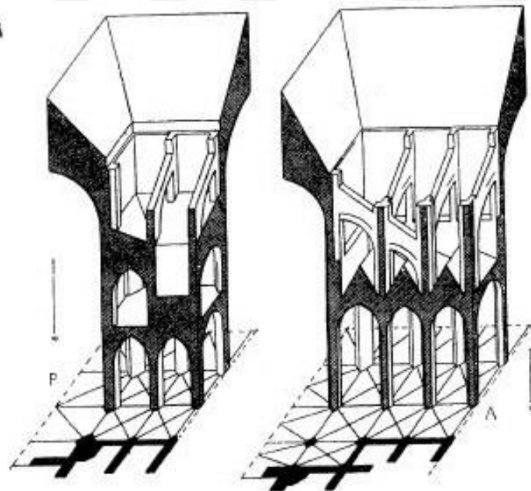
Figure 4.1.2. Sections of Amiens Cathedral by Choisy, Histoire de l'Architecture , 1899.
