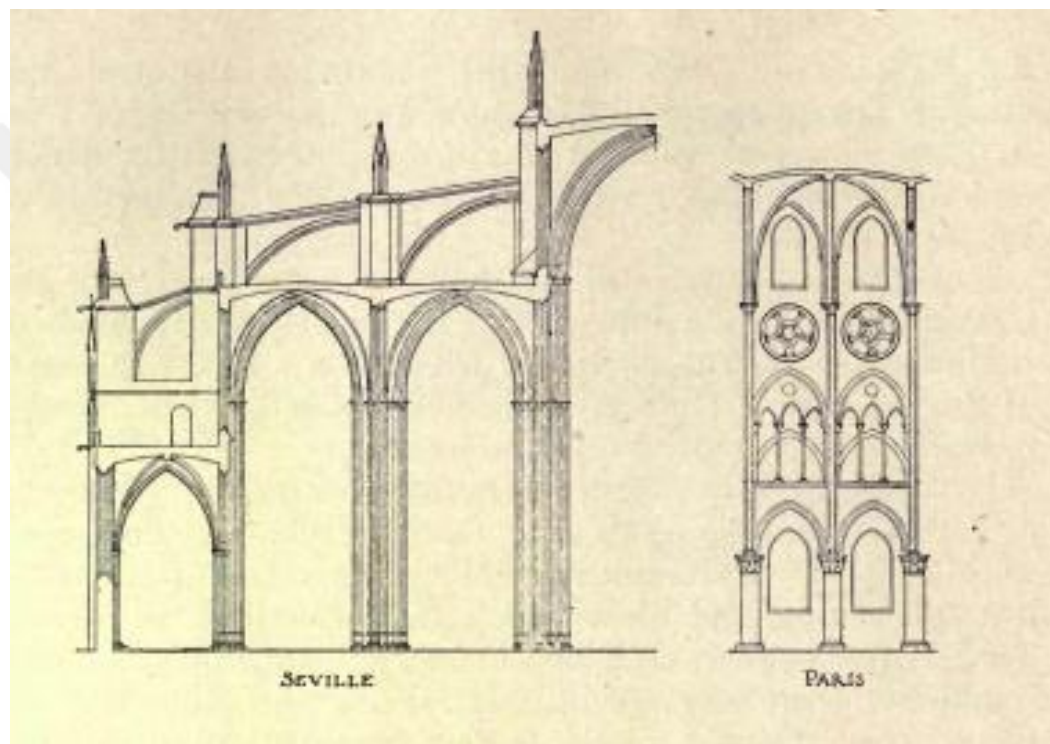
Figure 4.5.4. Sections and Systems of Gothic Buildings.
