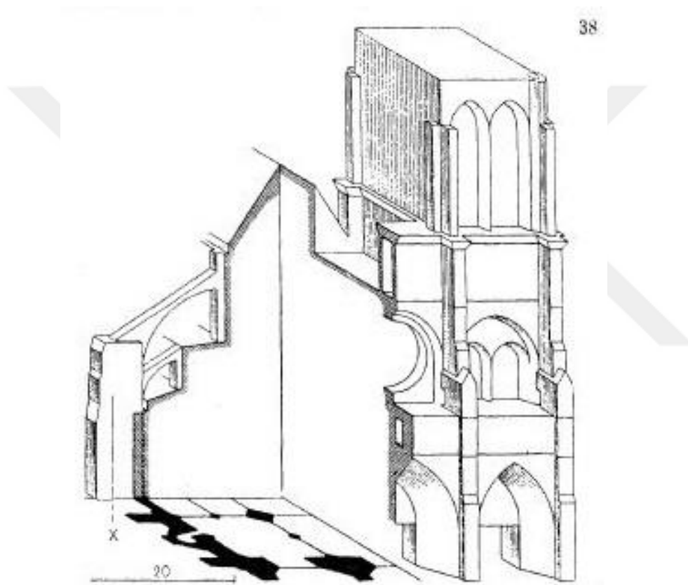
Figure 4.1.3. Partial section of Notre-Dame de Paris by Choisy, 1899
