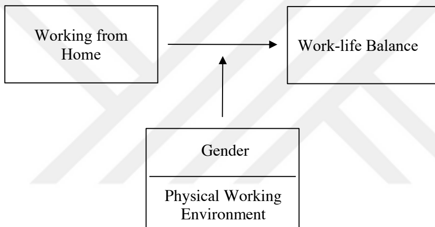
Figure 2. Conceptual model 2
