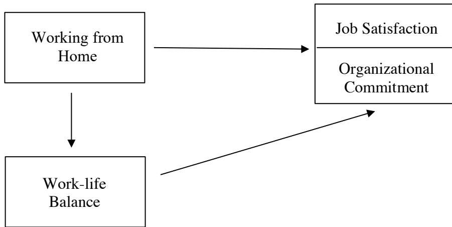
Figure 1. Conceptual model 1
