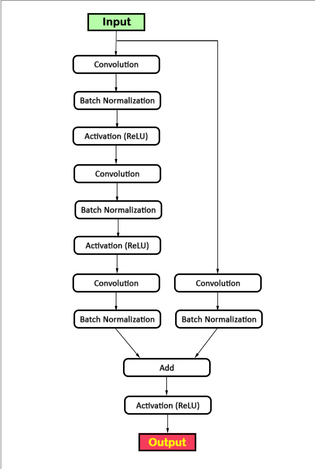
Figure 3.7: Symbolic Representation of A Convolution Block
