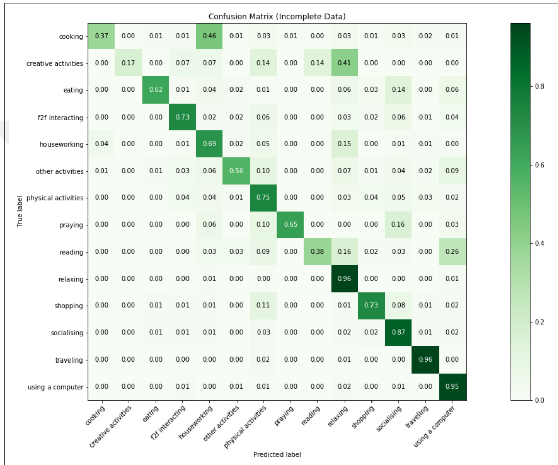
Figure 4.6: Confusion Matrix for 16-Class Incomplete Test Set
