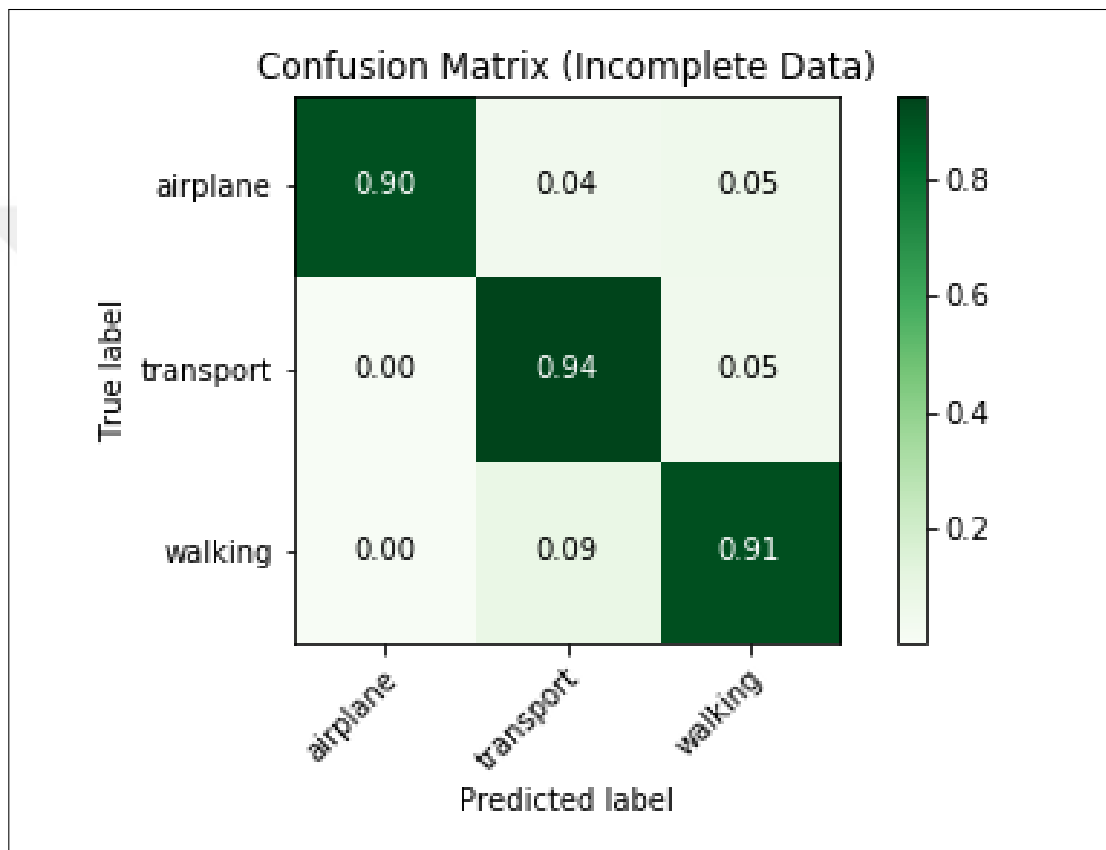
Figure 4.4: Confusion Matrix for 3-Class Incomplete Test Set
