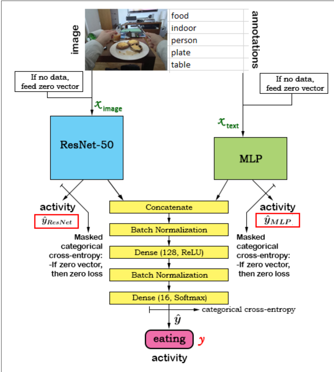
Figure 3.10: Structure of the Multi-Loss Combined Model
