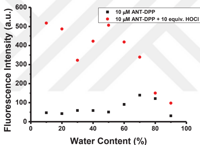
Figure 3.3. Water content solvent system, ANT-DPP (10 \mu\text{M} ) towards addition of HOCl (100 \mu\text{M} ), ( \lambda_{\text{ex}} : 380nm, \lambda_{\text{em}} : 460nm, 25 ^{\circ}\text{C} )
