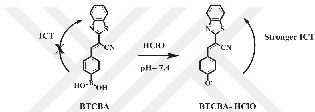
Figure 1.11. Sensing Mechanism of BTCBA based on ICT Mechanism
