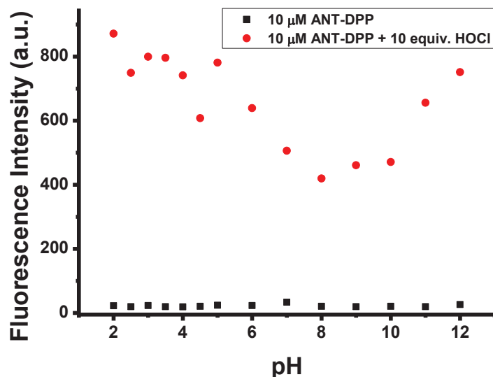
Figure 3.4. pH screening of ANT-DPP (10 \mu M) towards addition of HOCl (100 \mu M) in CH 3 CN/HEPES (1:1, v:v), ( \lambda_{ex} : 380nm, \lambda_{em} : 460nm, 25°C)
