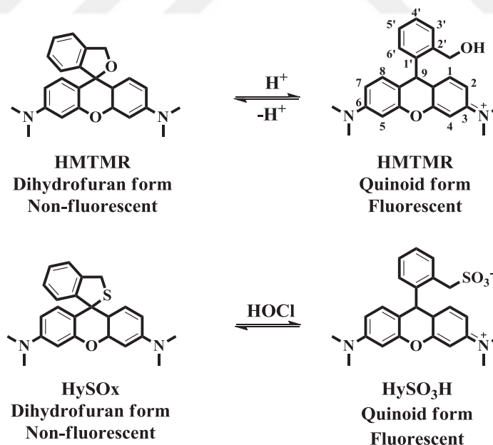
Figure 1.6. Sensing representation of probe and HOCl
