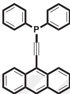
Figure 2.5. (anthracen-9-ylethynyl)diphenylphosphine
