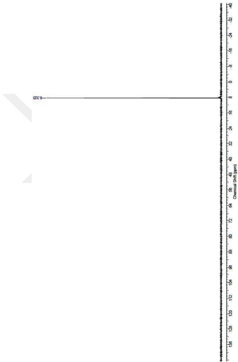
Figure A 6. ^{31}\text{P} NMR of ANT-DPPO
