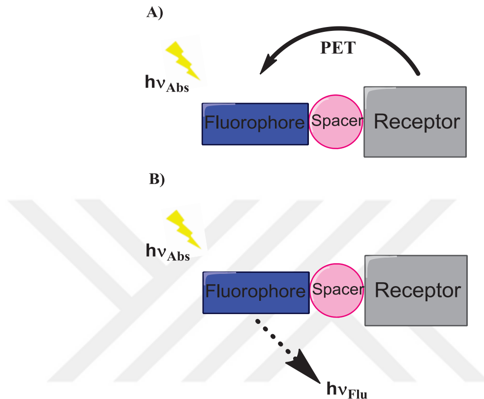
Figure 1.3. Representation of PET mechanism. A) "off" state B) "on" state
