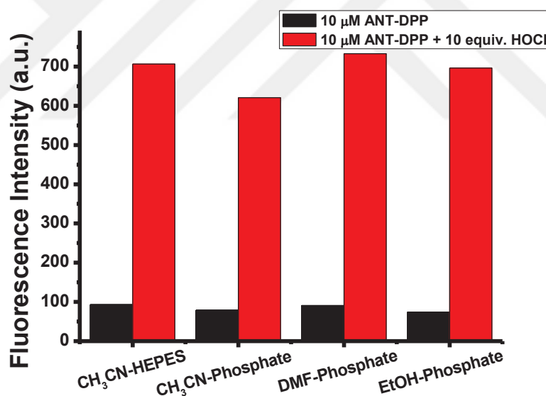
Figure 3.2. Solvent screening of ANT-DPP (10μM) towards addition of HOCl (100μM), ( \lambda_{\text{ex}} : 380nm, \lambda_{\text{em}} : 460nm, 25°C)
