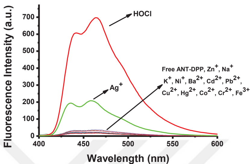
Figure 3.11. Metal scanning of ANT-DPP (10 \mu M) upon addition of other metals (200 \mu M) + HOCl (100 \mu M) in CH 3 CN/HEPES (1:1, v:v), ( \lambda_{\text{ex}} : 380nm, \lambda_{\text{em}} : 460nm, 25°C)
