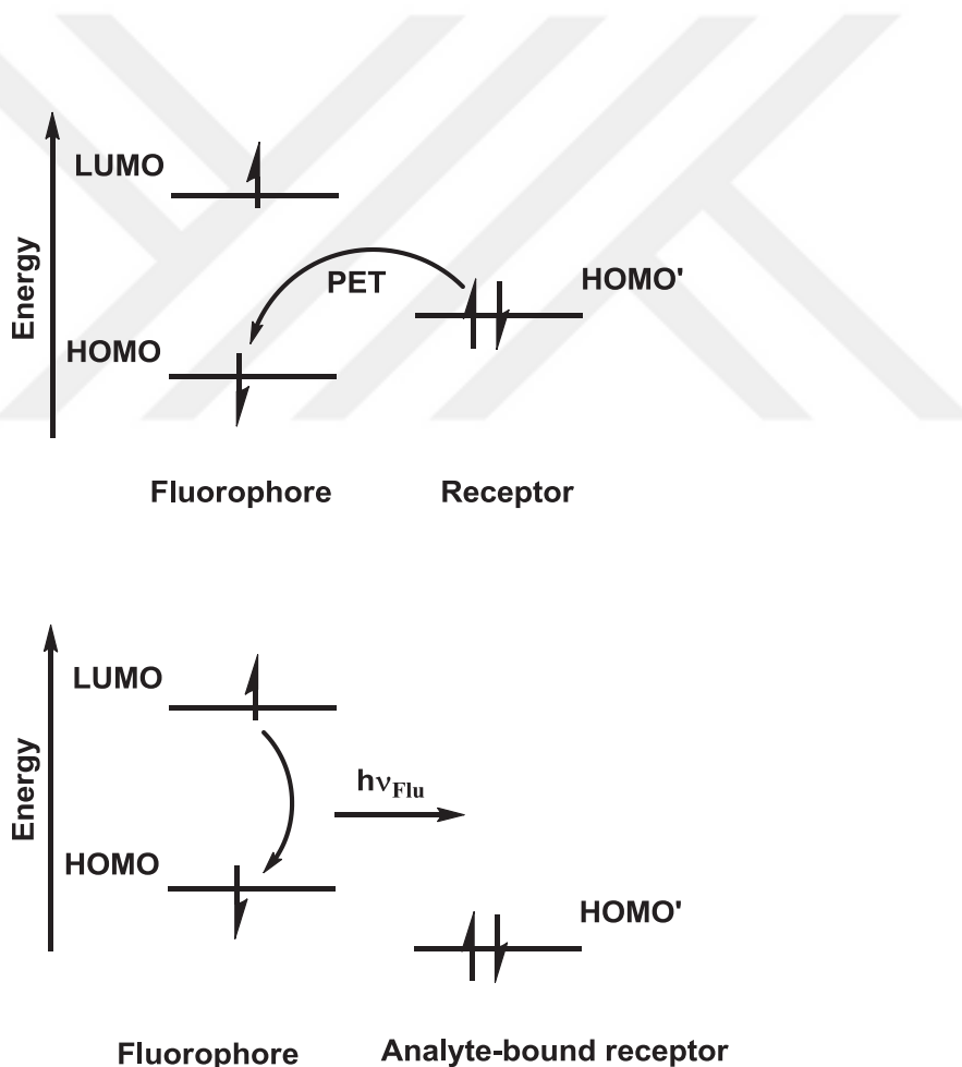
Figure 1.4. Representation of molecular orbital diagrams of fluorophores and receptor.
