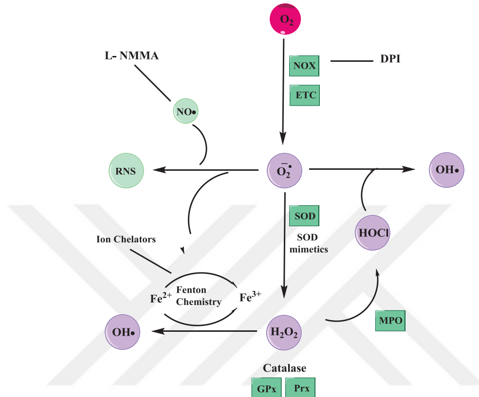
Figure 1.1: Physiological ROS homeostasis Network
