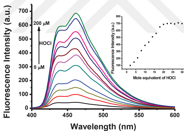
Figure 3.6. Fluorescence titration of ANT-DPP (10 \mu M) upon addition of HOCl (from 0 \mu M to 200 \mu M) in CH 3 CN/HEPES (1:1, v:v), ( \lambda_{\text{ex}} : 380nm, \lambda_{\text{em}} : 460nm, 25°C)
