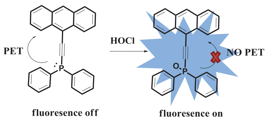
Figure 3.1. Reaction-based detection of HOCl
