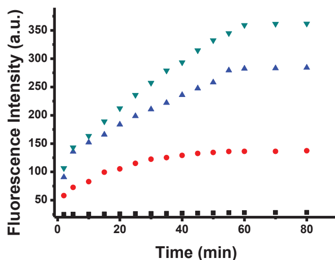
Figure 3.5. Time profile of ANT-DPP (10 \mu M) towards addition of HOCl (1 \mu M, 3 \mu M, 5 \mu M) in CH 3 CN/HEPES (1:1, v:v), ( \lambda_{\text{ex}} : 380nm, \lambda_{\text{em}} : 460nm, 25°C)
