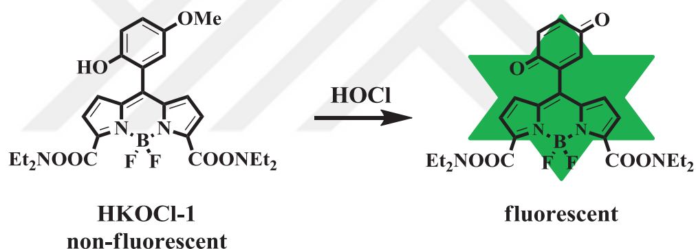
Figure 1.7. Demonstration of sensing mechanism
