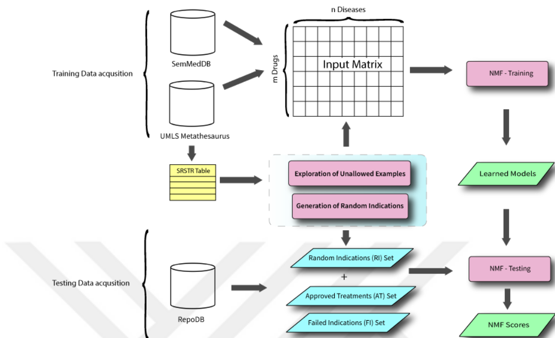
Figure 4.1: Schematic summary of the proposed NMF based CDR experiments
