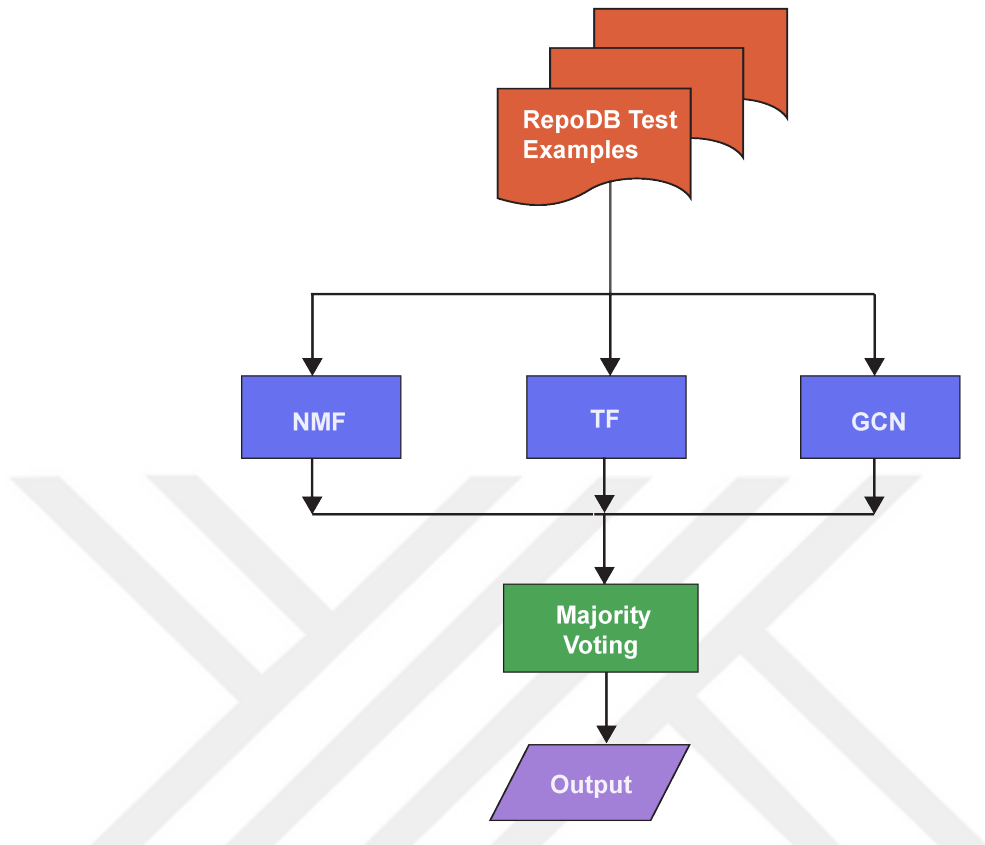
Figure 5.4: The ensemble model structure combining NMF, TF, and GCN models
