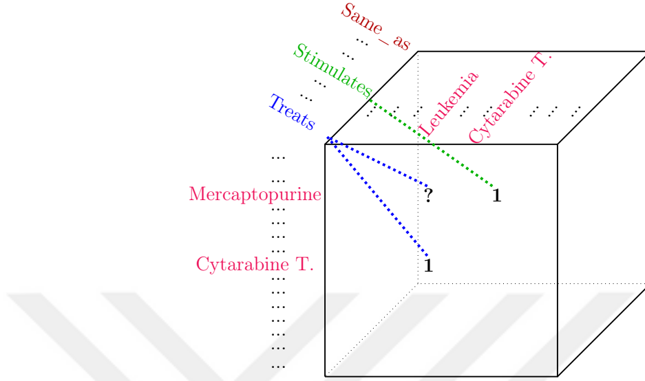
Figure 5.1: Third order tensor structure representation ( \mathcal{X}^{I \times J \times K} ) for embedding biomedical predications.
