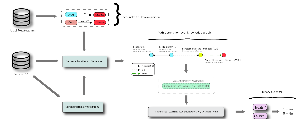
Figure 3.3: Schematic of graph pattern based relation prediction
