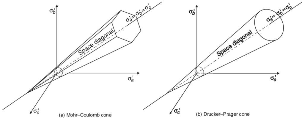
Figure 2.1. Mohr-Coulomb and Drucker-Prager Failure Surfaces Comparison (Potts et al., 2002)
