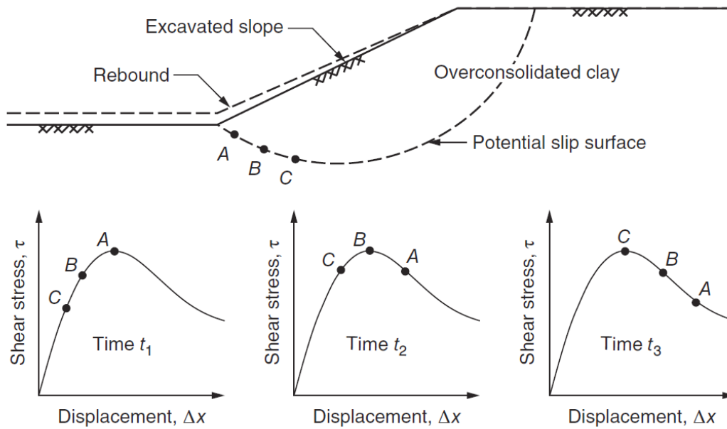
Figure 2.6. Progressive Failure of an Over-Consolidated Clay Slope (Duncan et al., 2014)
