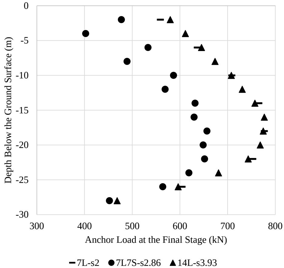
Figure 3.7. Anchor Loads at Last Serviceability Stages
