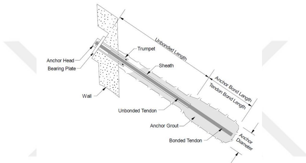
Figure 2.11. Typical Structure of Temporary Ground Anchor (Sabatini et al., 1999)
