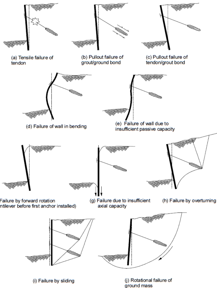
Figure 2.12. Failure Modes of Anchored Retaining Walls (Sabatini et al., 1999)
