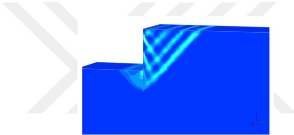
Figure 3.14. Incremental Deviatoric Strains of 14L-s3.93-3D Model
