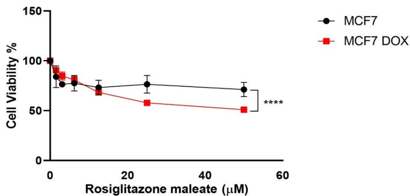
Figure 0-20 PPARG expression and effect of Rosiglitazone on cell death in MCF7 and MCF7 DOX cells.
