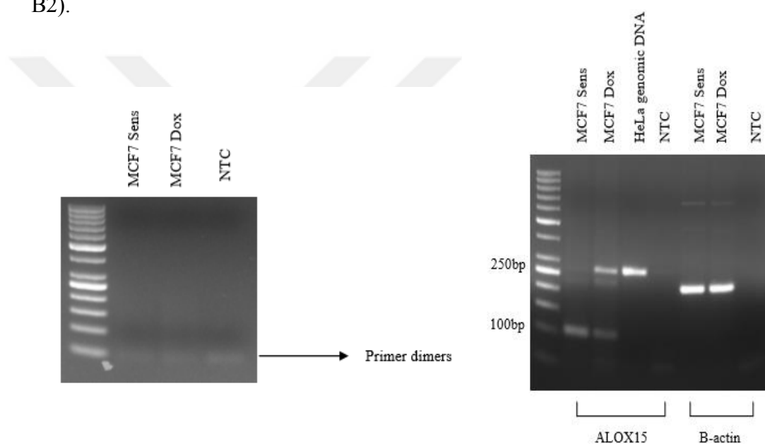
Figure B.0-2 Conventional PCR studies for assessing possible genomic DNA contamination in DNase-treated RNA samples (left) and for showing that firstly used ALOX15 primers amplified more than one PCR bands, one of which overlaps with that of intronic-region containing genomic DNA control (right).
