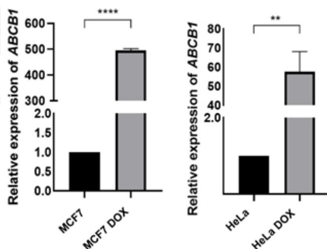
Figure 0-13 ABCB1 expression in MCF7 DOX and HeLa DOX cells compared to their sensitive counterparts (** p < 0.01 ; **** p < 0.0001 ).
