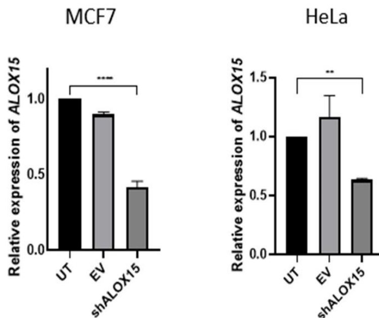
Figure 0-10 Downregulation of 15-LOX-1 by designed shRNA vector in the presence of untreated and EV controls.
