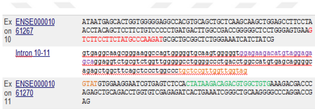
Figure B.0-1 The sequence showing primer pair in the first qRT-PCR studies. Red sequence: Forward primer; green sequence: Reverse primer. Sequence obtained from Ensembl.org (ENST00000293761.7).
