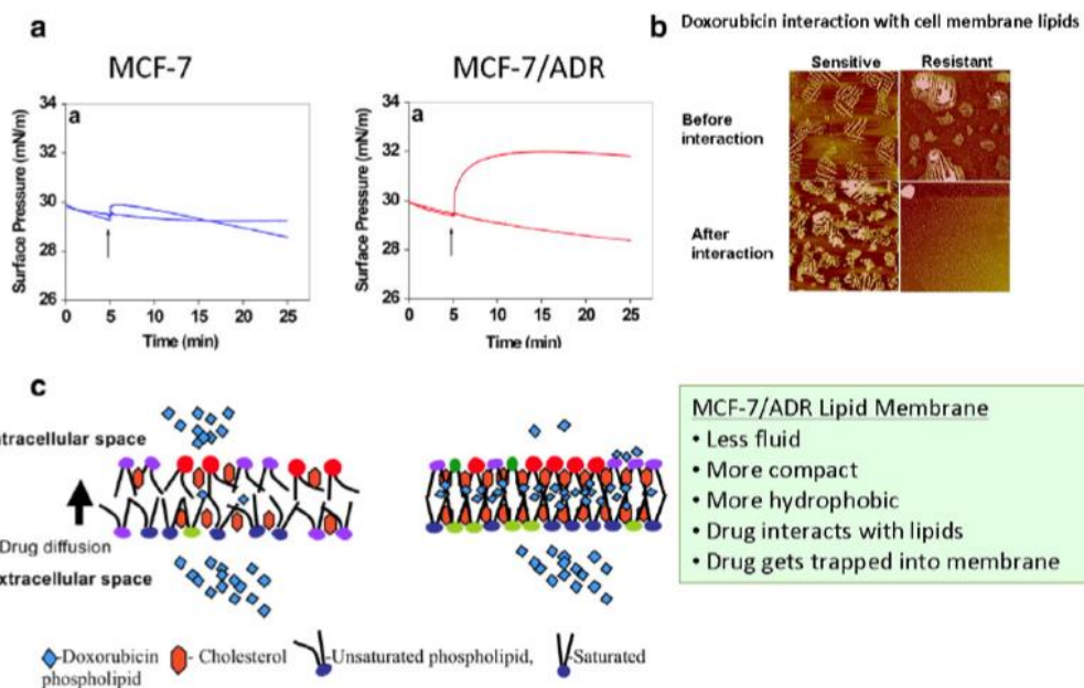
Figure 1-3 Membrane biophysics in sensitive and doxorubicin-resistant MCF7 cells. a) Doxorubicin interacted strongly with lipids in doxorubicin-resistant MCF7 cells, which was also confirmed by b) AFM images. c) Illustration of doxorubicin trapping in the lipid bilayer and the mechanisms related to lipid bilayer-dependent resistance status of doxorubicin-resistant cell line (Peetla et al., 2013).
