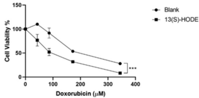
Figure 0-23 Effect of 13(S)-HODE treatment on response to doxorubicin in MCF7 DOX (top) and HeLa DOX (bottom). Cells were treated with doxorubicin at increasing concentrations and 13(S)-HODE, and cell viabilities were determined by MTT assay. Data were analysed by non-linear regression. *** p < 0.001 .
