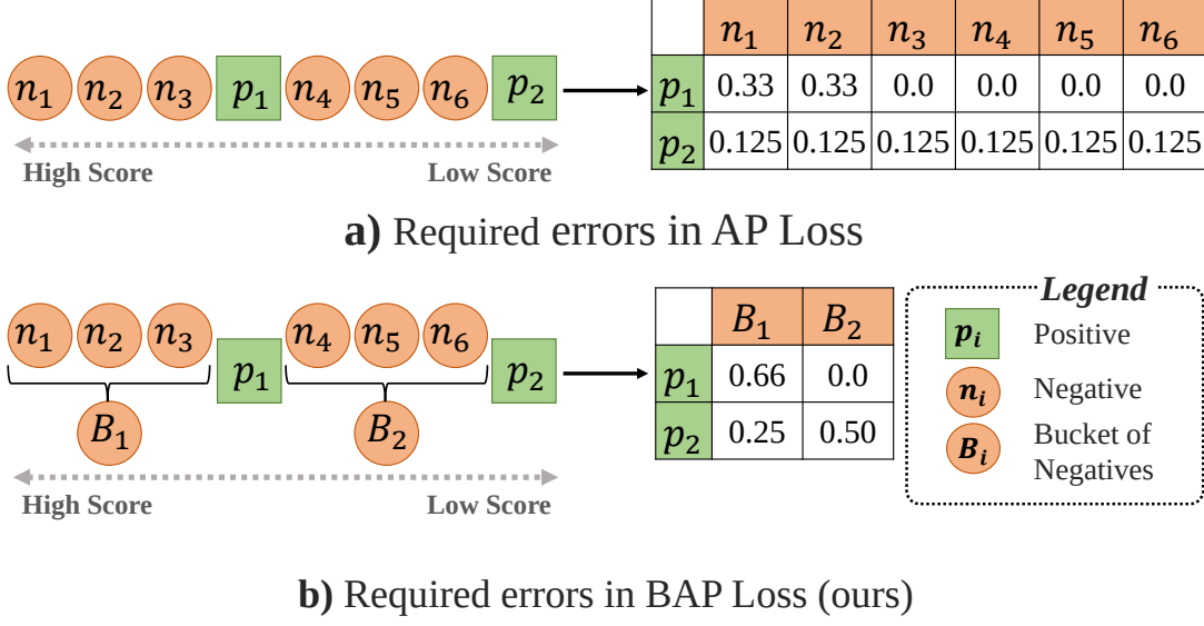
Figure 1.3: (a) Existing ranking-based losses (i.e., AP Loss [1, 2]) incur significant overhead owing to pairwise comparisons between positives and negatives. (b) We propose bucketing negatives to decrease the number of comparisons, and hence the complexity. Under certain assumptions, our bucketing approach provides equal gradients with conventional ranking-based losses such as AP Loss in (a). [Figure from our ECCV 2024 paper [3]]
