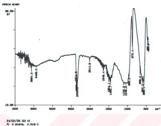
Figure 9.27. FTIR spectrum of the sample calcined at 500°C for 4 hours
