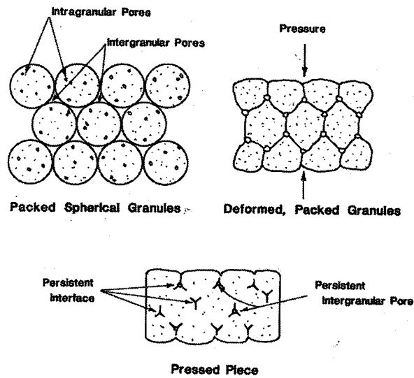
Figure 6.6. Change in granule shape and bimodal pore size distribution during compaction [23]
