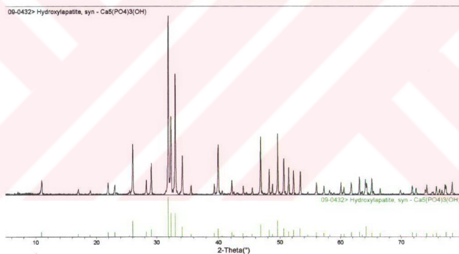
Figure 9.33. X-ray spectrum of the sample calcined at 700°C for 4 hours
