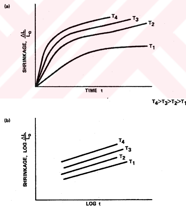
Figure 7.7. Typical sintering rate curves showing the effects of temperature and time
