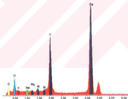
Figure 9.14. EDAX spectrum of the hydroxyapatite powder obtained using 2. Route (deproteinization in NaOH and calcination)
