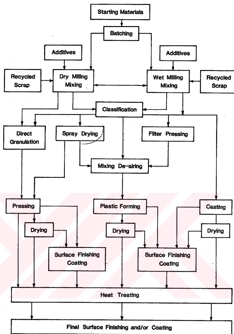
Figure A.1. A General processing flow diagram illustrating processing paths from raw materials to the fired product [23]
