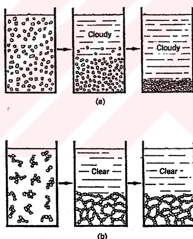
Figure 5.5. Sedimentation behavior for (a) deflocculated and (b) coagulated suspensions [23]
