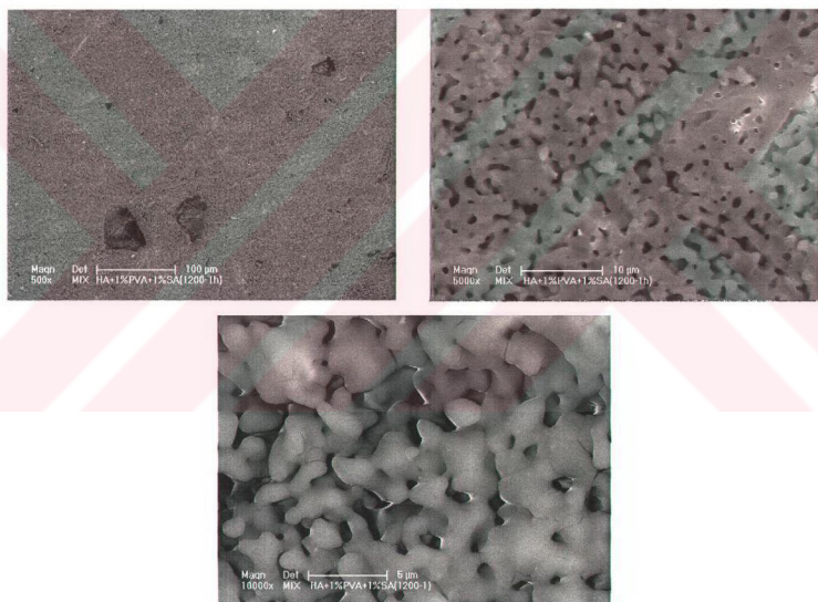
Figure 9.56. Hydroxyapatite + 1 % polyvinyl alcohol + 1 % stearic acid sintered at 1200 °C for 1 hour
