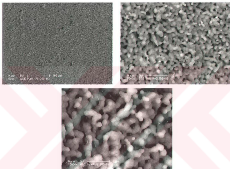
Figure 9.51. Pure hydroxyapatite sintered at 1200 °C for 4 hours
