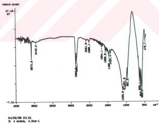
Figure 9.5. FTIR spectrum of the hydroxyapatite powder obtained using 3. Route (only calcination)
