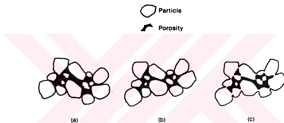
Figure 7.1. Changes that occur during the initial stage of sintering.
