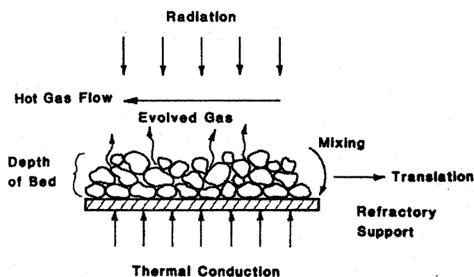
Figure 4.1. Thermal transport, gas flow, and particle movement during rotary calcination [23]
