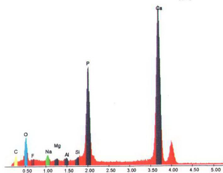
Figure 9.13. EDAX spectrum of the hydroxyapatite powder obtained using 1. Route (degassing in hexane, deproteinization in NaOH and calcination)
