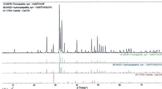
Figure 9.36. X-ray spectrum of the sample calcined at 850°C for 8 hours
