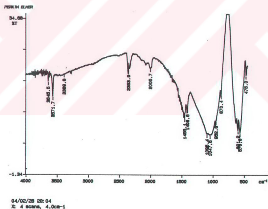
Figure 9.3. FTIR spectrum of the hydroxyapatite powder obtained using 1. Route (degassing in hexane, deproteinization in NaOH and calcination)
