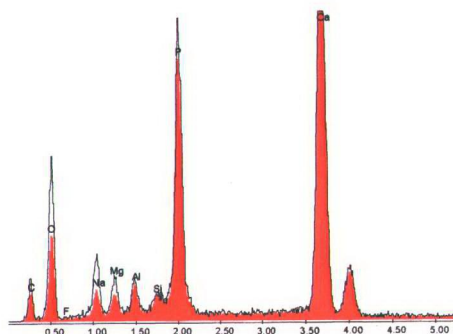
Figure 9.19. Comparison of the EDAX spectra of the light (ghost line) and dark regions (color line) seen in the ESEM images of the sample held in NaOH for 2 months
