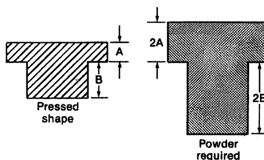
Figure 6.5. Schematic illustrating the different distances a punch must move to accomplish uniform compaction of the powder. Based on a powder with a compaction ratio of 2:1 [22]
