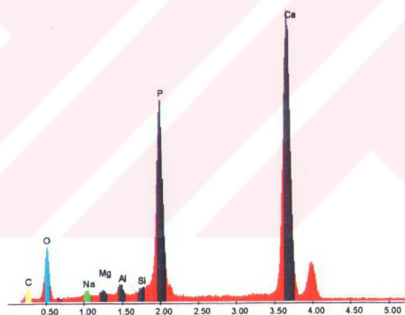
Figure 9.41. EDAX spectrum of the sample calcined at 850°C for 8 hours
