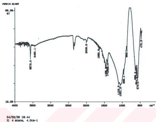
Figure 9.6. FTIR spectrum of the hydroxyapatite powder through a long-term (2 months) deproteinization in NaOH and calcination
