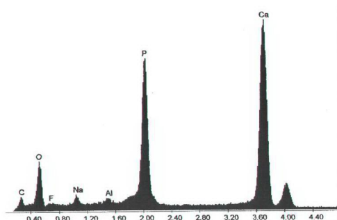
Figure 9.17. EDAX spectrum of the commercially available hydroxyapatite powder from Aldrich Chemical Company Inc. [19]
