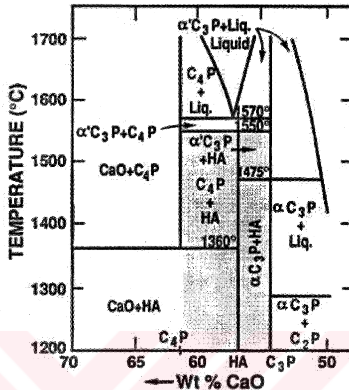
Figure 3.1. Phase equilibrium diagram of calcium phosphates in a water atmosphere.
