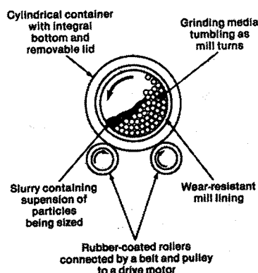
Figure 5.2. Schematic cross section showing the key elements of a typical ball mill [22]
