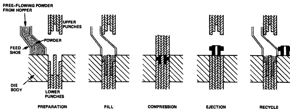
Figure 6.1. Schematic illustrating automated uniaxial pressing [22]
