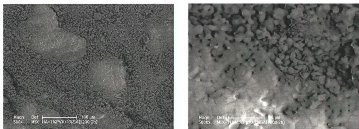
Figure 9.55. Hydroxyapatite + 1 % polyvinyl alcohol + 1 % stearic acid sintered at 1200 °C for 2 hours
