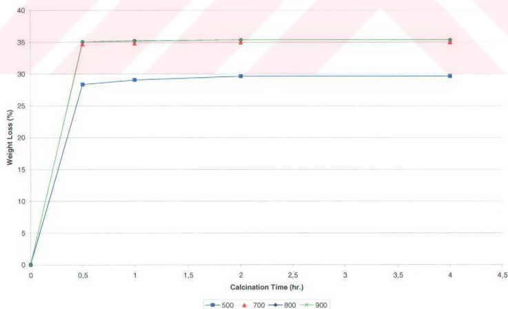
Figure 9.25. Per cent wt. loss vs. calcination time at different calcination temperatures
