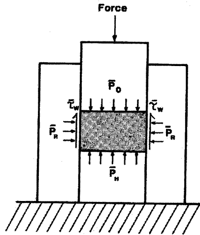
Figure 6.7. Mean stresses on the compact during unidirectional compaction [23]
