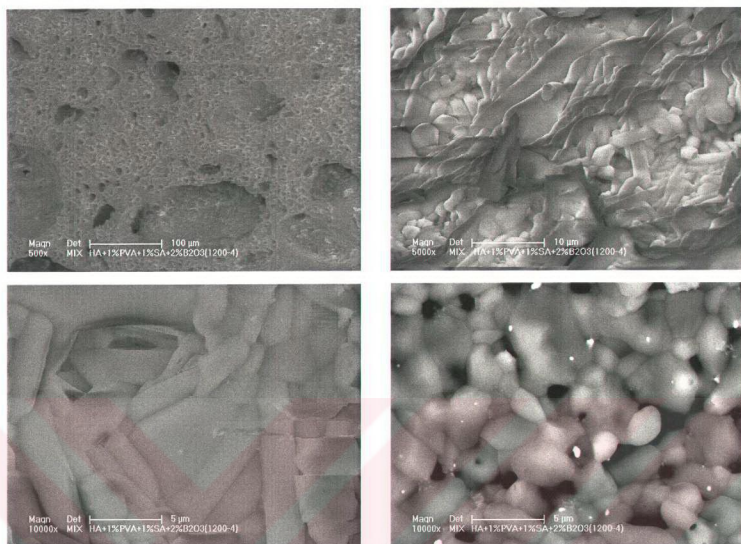
Figure 9.58. Hydroxyapatite + 1 % polyvinyl alcohol + 1 % stearic acid + 2 % boron oxide sintered at 1200 °C for 4 hours
