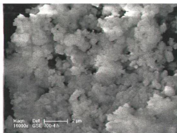
Figure 9.43. ESEM image of the sample calcined at 700°C for 4 hours
