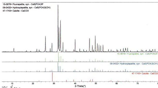
Figure 9.10. X-ray spectrum of the hydroxyapatite powder obtained using 3. Route (only calcination)
