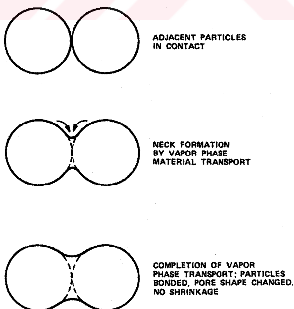
Figure 7.4. Schematic of vapor-phase material transport [22]
