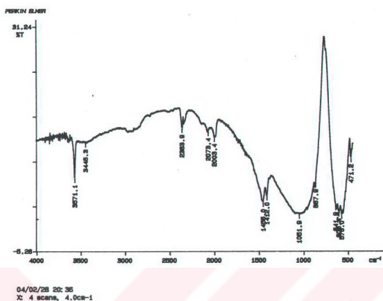
Figure 9.4. FTIR spectrum of the hydroxyapatite powder obtained using 2. Route (deproteinization in NaOH and calcination)
