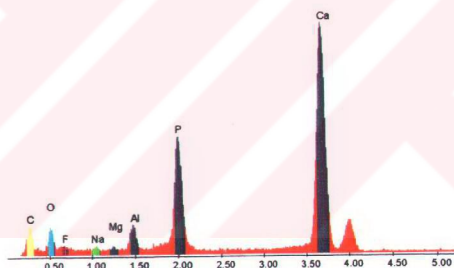
Figure 9.37. EDAX spectrum of the sample calcined at 500°C for 4 hours
