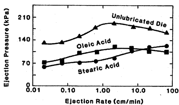
Figure 6.4. Effect of lubrication on ejection pressure for an alumina compact with a polyvinyl alcohol binder (23 °C) [23]
