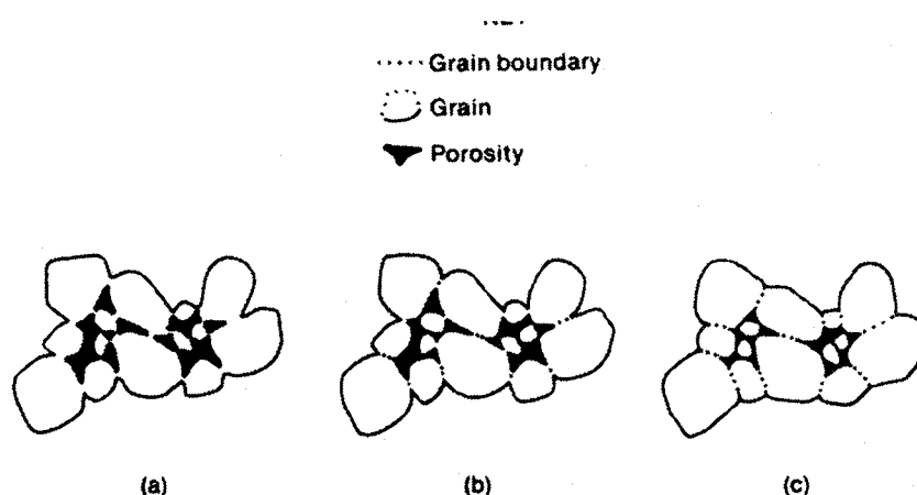
Figure 7.2. Changes that occur during the intermediate stage of sintering.
