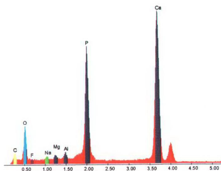
Figure 9.38. EDAX spectrum of the sample calcined at 700°C for 4 hours
