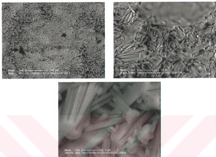
Figure 9.60. Hydroxyapatite + 1 % polyvinyl alcohol + 1 % stearic acid + 10 % boron oxide sintered at 1200 °C for 4 hours
