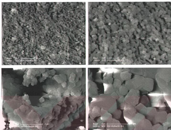
Figure 9.20. ESEM image of the hydroxyapatite powder obtained using 1. Route (degreasing in hexane, deproteinization in NaOH and calcination)
