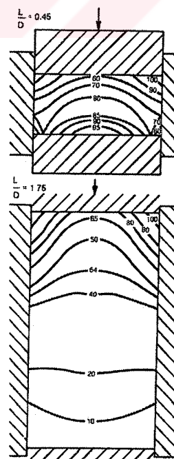
Figure 6.9. Pressure variations in uniaxial pressing due to die-wall friction and particle-particle friction, which lead to nonuniform density of the pressed compact [22]
