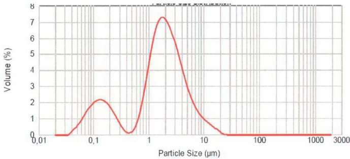
Figure 9.49. Particle size distribution of the hydroxyapatite powder after 6 hours of grinding
