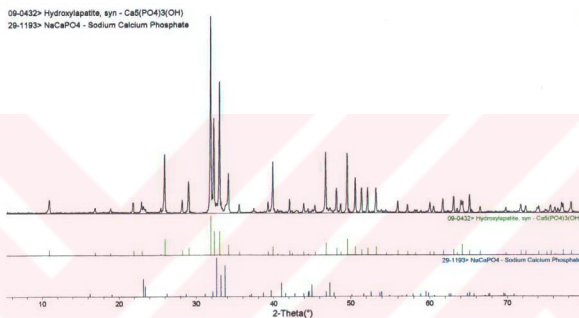
Figure 9.8. X-ray spectrum of the hydroxyapatite powder obtained using 1. Route (degreasing in hexane, deproteinization in NaOH and calcination)
