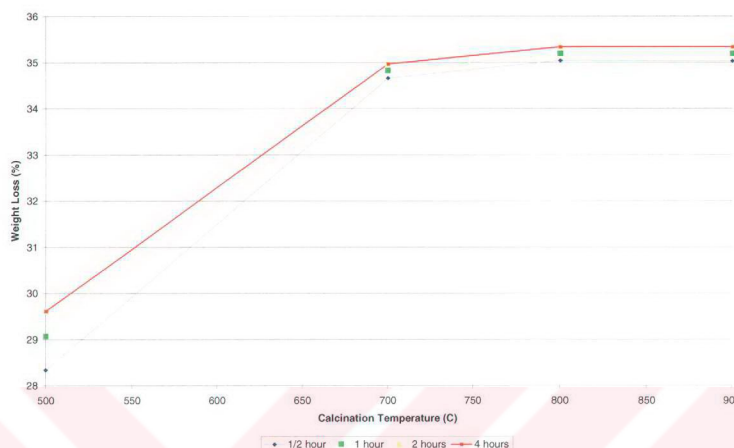
Figure 9.26. Per cent wt. loss vs. calcination temperature at different calcination times
