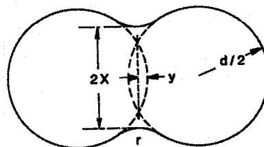
Figure 7.6. Two-sphere initial-stage sintering model [23]
