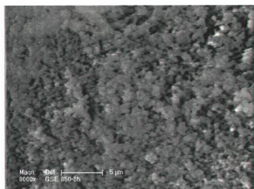
Figure 9.46. ESEM image of the sample calcined at 850°C for 8 hours
