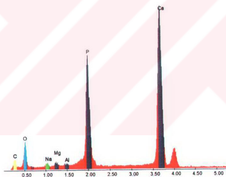
Figure 9.39. EDAX spectrum of the sample calcined at 800°C for 4 hours
