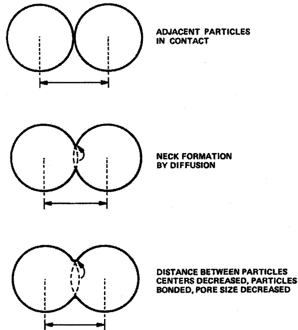
Figure 7.5. Schematic of solid-state material transport [22]
