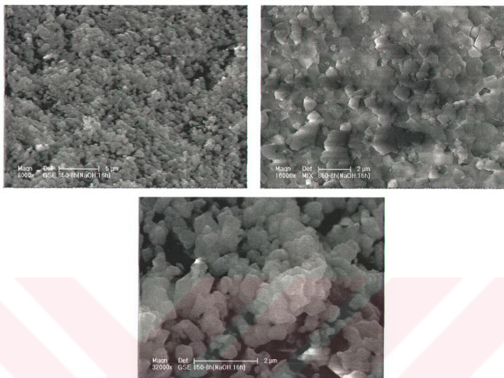
Figure 9.21. ESEM image of the hydroxyapatite powder obtained using 2. Route (deproteinization in NaOH and calcination)
