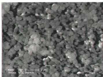
Figure 9.44. ESEM image of the sample calcined at 800°C for 4 hours
