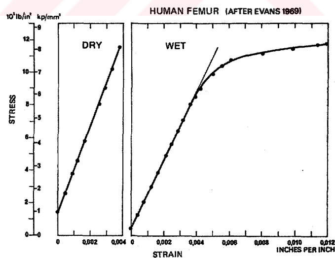
Figure B.3. Stress-strain curves of human femoral bone [47]
