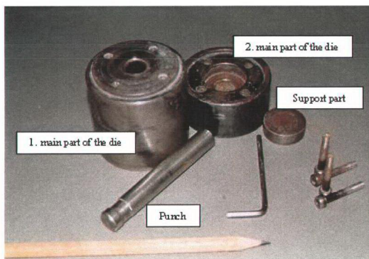
Figure 8.3. Die used to prepare the specimens [43]
