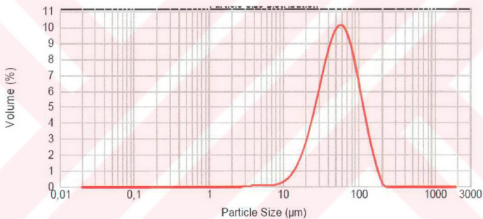
Figure 9.50. Particle size distribution of polymethylmethacrylate prior to grinding
