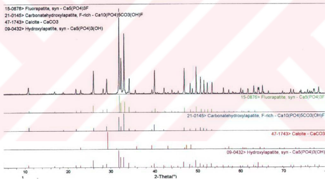
Figure 9.35. X-ray spectrum of the sample calcined at 900°C for 4 hours
