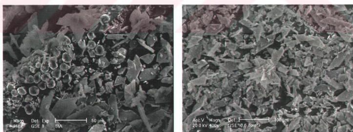
Figure 9.24. ESEM image of the commercially available hydroxyapatite powder from Aldrich Chemical Company Inc. [19]
