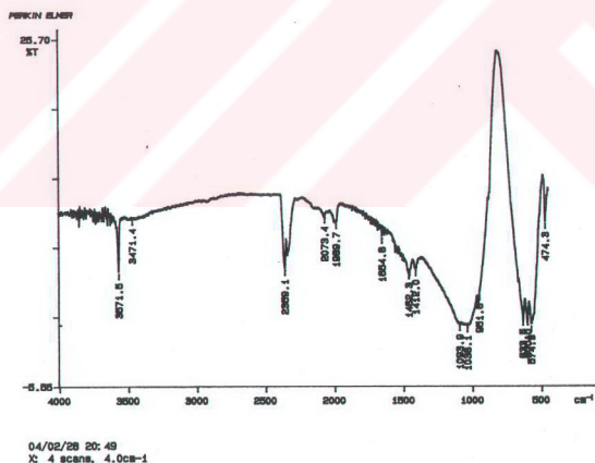
Figure 9.30. FTIR spectrum of the sample calcined at 900°C for 4 hours
