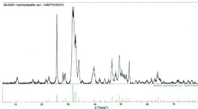
Figure 9.12. X-ray spectrum of the commercially available hydroxyapatite powder from Aldrich Chemical Company Inc.
