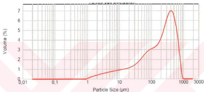
Figure 9.47. Particle size distribution of the hydroxyapatite powder prior to grinding
