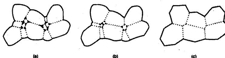
Figure 7.3. Changes that occur during the final stage of sintering.
