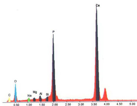
Figure 9.15. EDAX spectrum of the hydroxyapatite powder obtained using 3. Route (only calcination)
