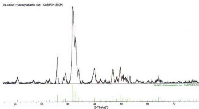
Figure 9.32. X-ray spectrum of the sample calcined at 500°C for 4 hours
