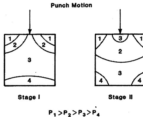
Figure 6.8. General pressure profiles for unidirectional pressing [23]
