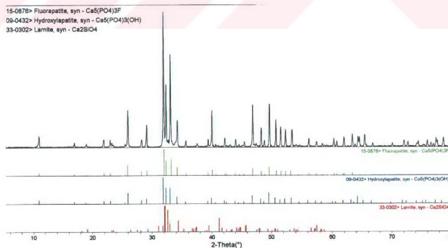
Figure 9.9. X-ray spectrum of the hydroxyapatite powder obtained using 2. Route (deproteinization in NaOH and calcination)
