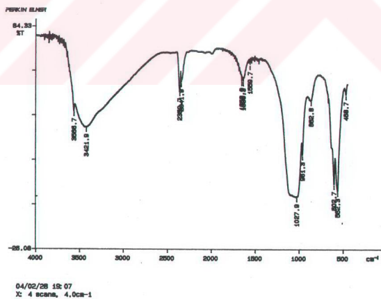
Figure 9.7. FTIR spectrum of the commercially available hydroxyapatite powder from Aldrich Chemical Company Inc.
