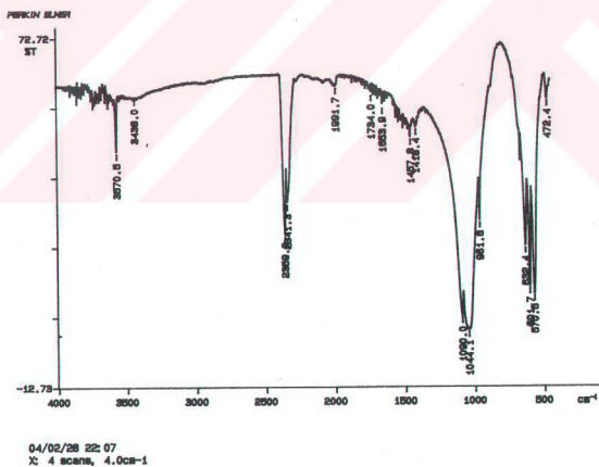
Figure 9.28. FTIR spectrum of the sample calcined at 700°C for 4 hours
