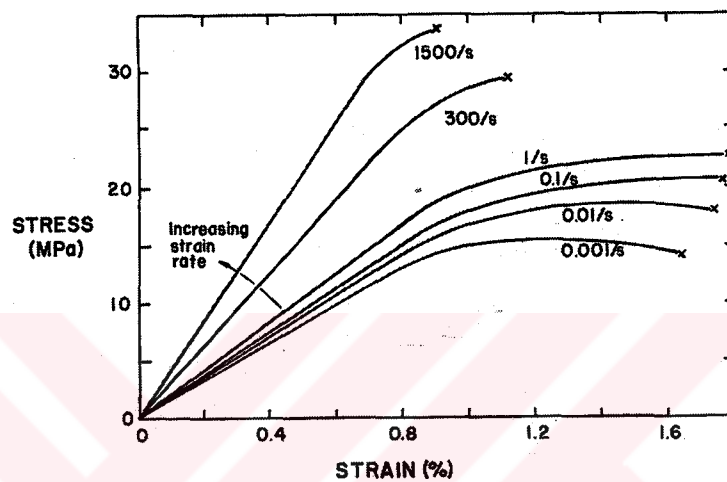
Figure B.4. Stress as a function of strain and strain rate for human compact bone [1]
