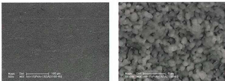
Figure 9.53. Hydroxyapatite + 1 % polyvinyl alcohol + 1 % stearic acid sintered at 1100 °C for 4 hours
