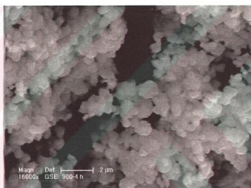
Figure 9.45. ESEM image of the sample calcined at 900°C for 4 hours
