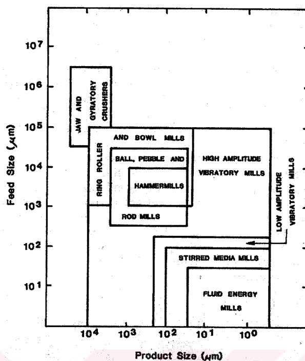
Figure 5.1. Nominal feed and product mean size capabilities of industrial equipment
