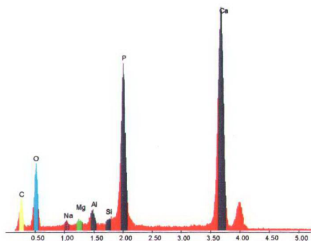
Figure 9.40. EDAX spectrum of the sample calcined at 900°C for 4 hours
