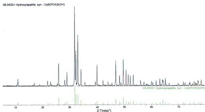
Figure 9.34. X-ray spectrum of the sample calcined at 800°C for 4 hours
