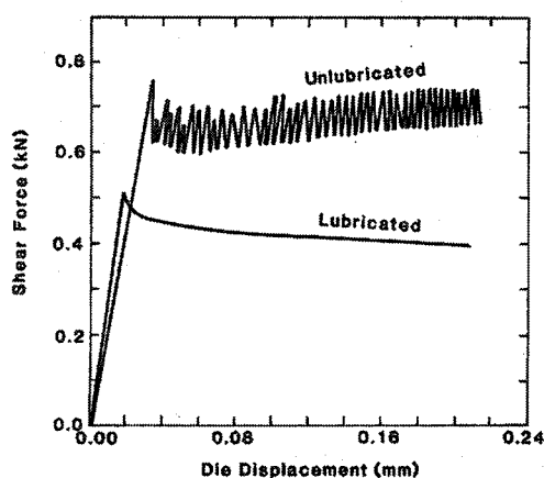
Figure 6.2. Regular and slip-stick shear produced on displacing the die while the compact is compressed [23]
