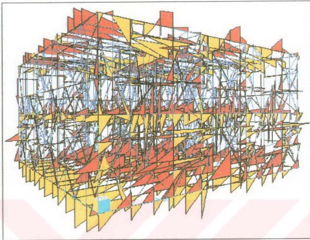
Figure 5.10 Typical Moment Diagram of Himiş Structure Under Lateral Forces
