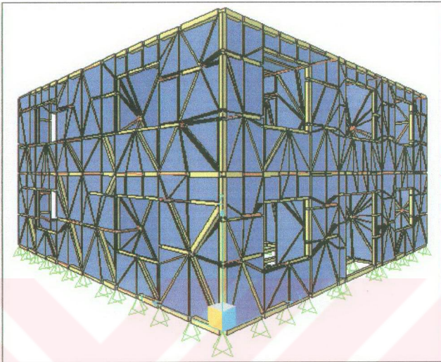
Figure 5.6 Undeformed Shape of Himiş Structure Without Infill Material
