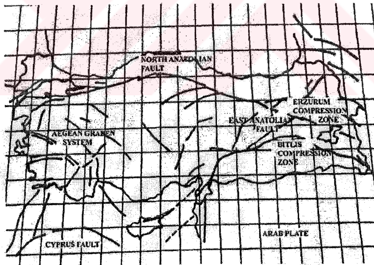
Seismic Plates Around Turkey (Barbieri, Lichtenegger & G. Calabresi, 2004)
