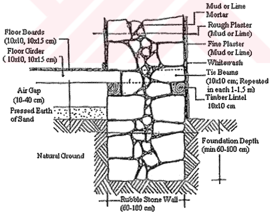
Heightened Floor, Inserted Into The Wall (Modified from Şahin, 1995)
