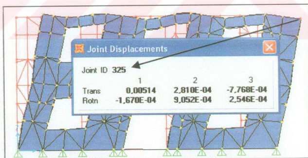
Figure 5.9 Deformed Shape of Hmuş Type of Building
