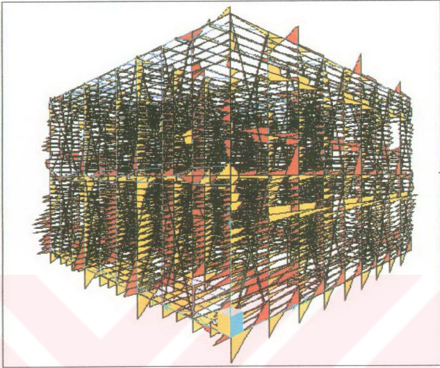
Figure 5.20 Typical Moment Diagram of Bağdadi Structure With Infill Under Lateral Forces
