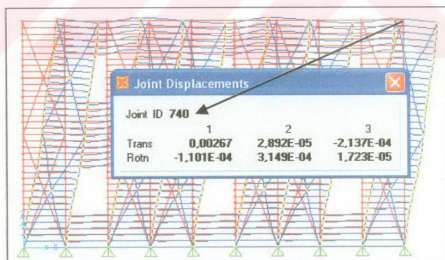
Figure 5.15 Deformed Shape of Bağdadi Structure Without Infill
