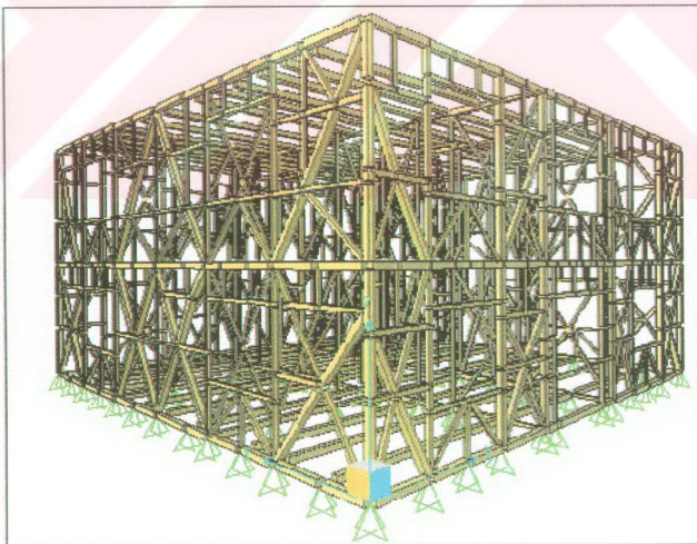
Figure 5.7 Undeformed Shape of Himiş Structure With Infill Material
