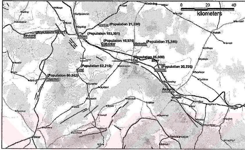
Figure 4.12 Damage Distribution of Sultandağı Earthquake (Erdik, Sesetyan, Demircioğlu, Celep, Biro, Üçkan, 2002)
