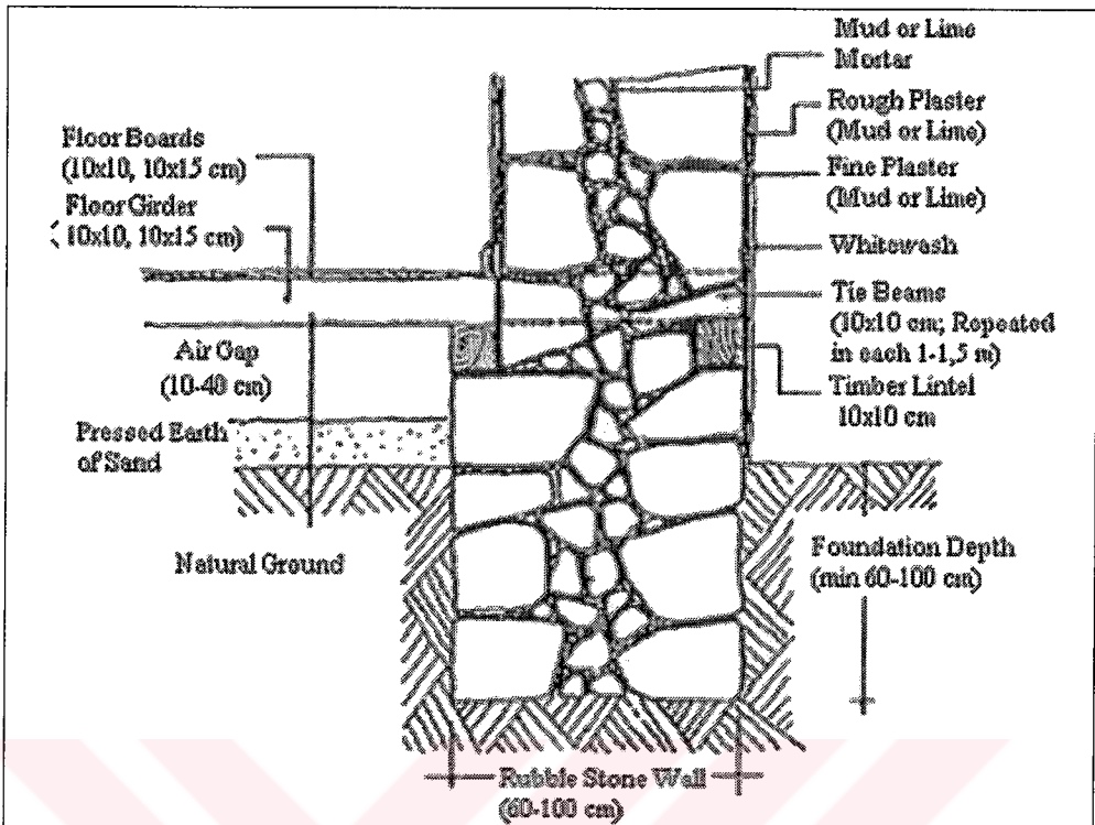
Heightened Floor, Supported by Stone Plint (Modified from Şahin, 1995)
