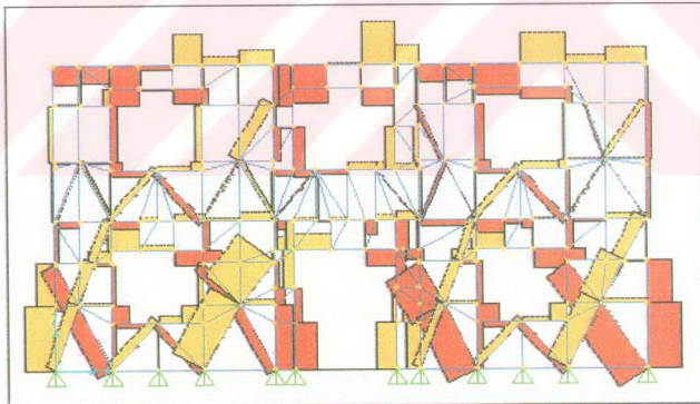
Figure 5.11 Typical Axial Force Distribution of Himiş Structure Under Lateral Forces
