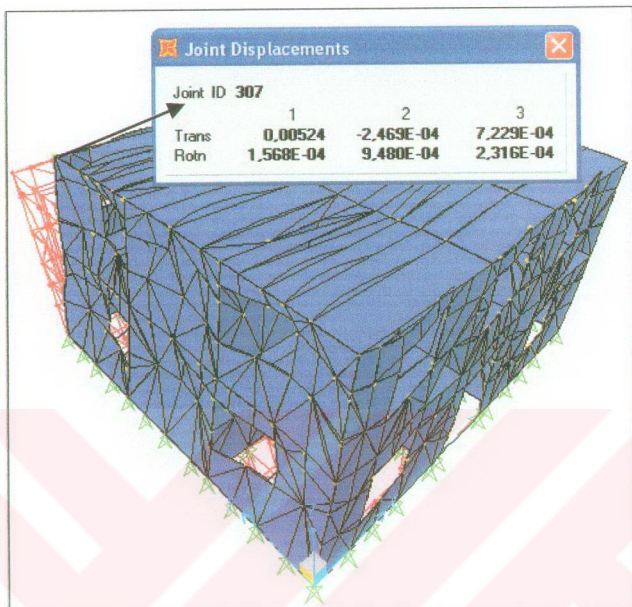
Figure 5.8 Deformed Shape of Hmuş Type of Building
