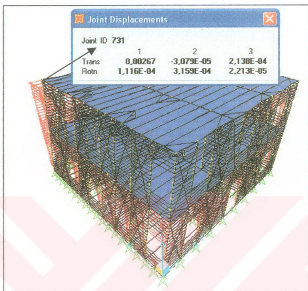
Figure 5.14 Deformed Shape of Bağdadi Structure Without Infill
