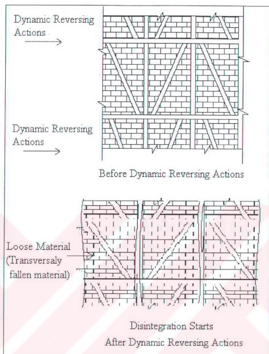
Figure 5.22 Deformation in Himiş Structure
