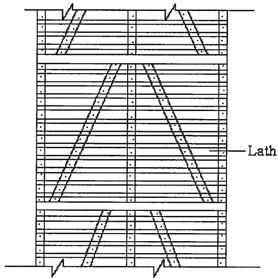
Bagdadi Construction System (Modified From Bayülke, 1934)
