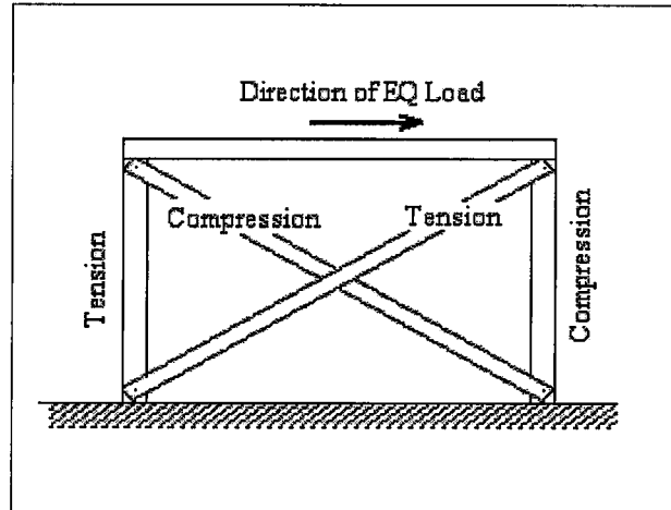
Figure 4.6 X Bracing
