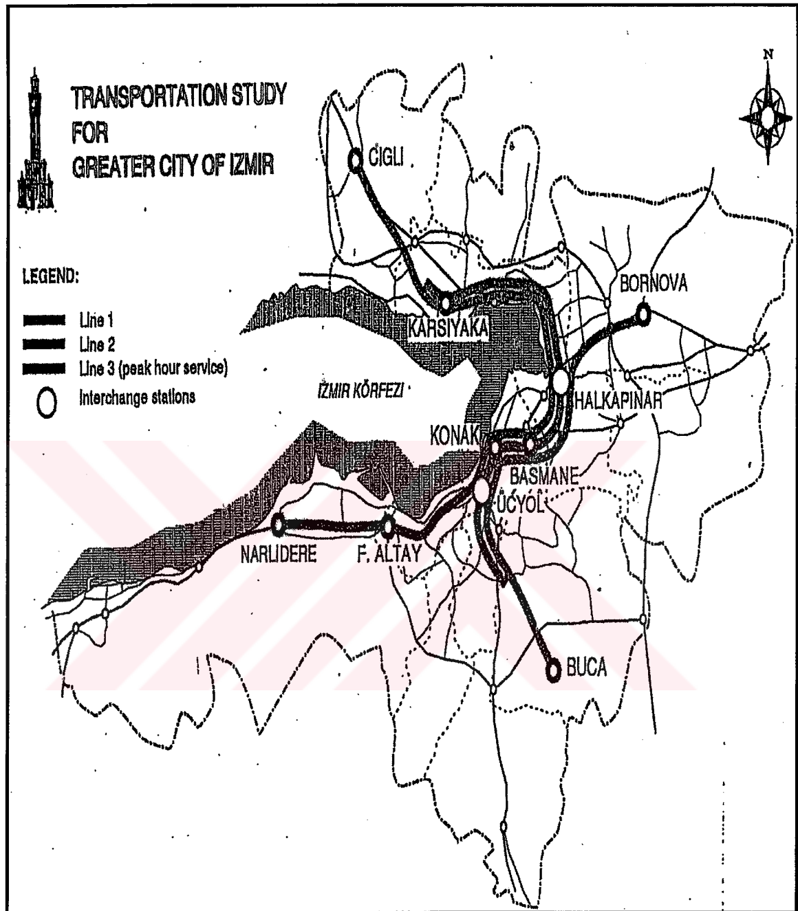
Figure 6. Proposed Subway Routes for İzmir
