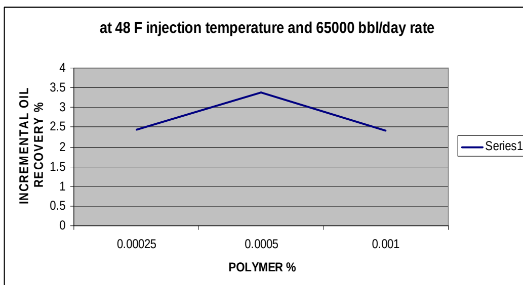
Figure 6.10 Incremental oil recovery versus polymer concentration at 48 F o
