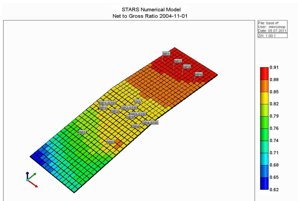
Figure 5.10 Net-to-gross distributions
