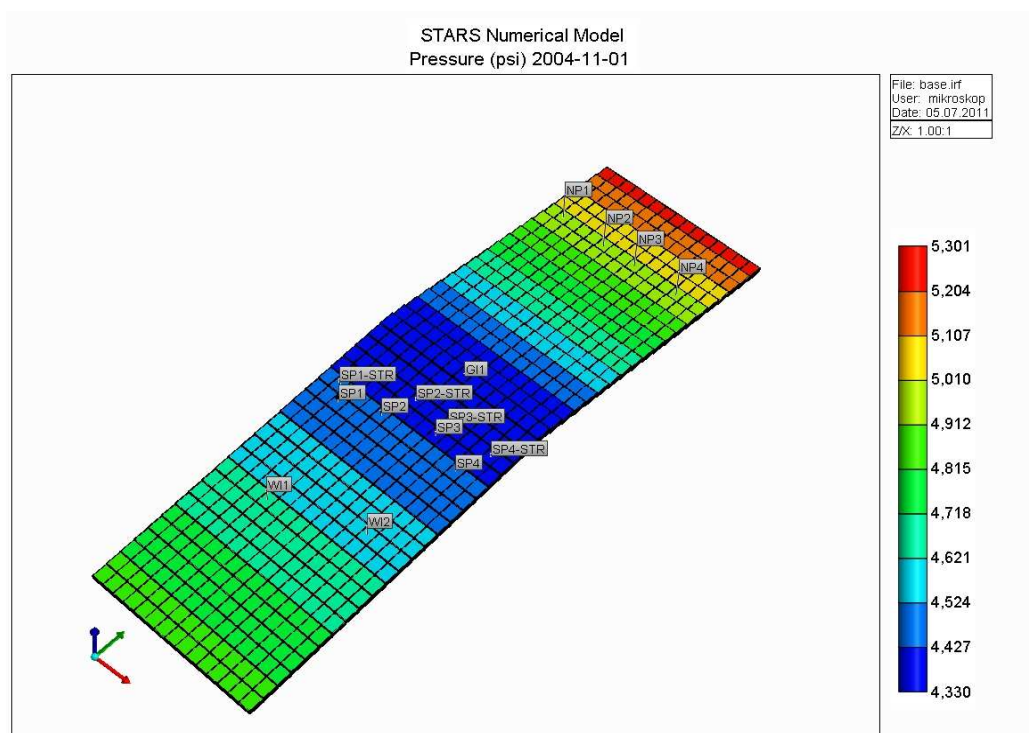
Figure 5.5 Initial pressure distributions of sector model
