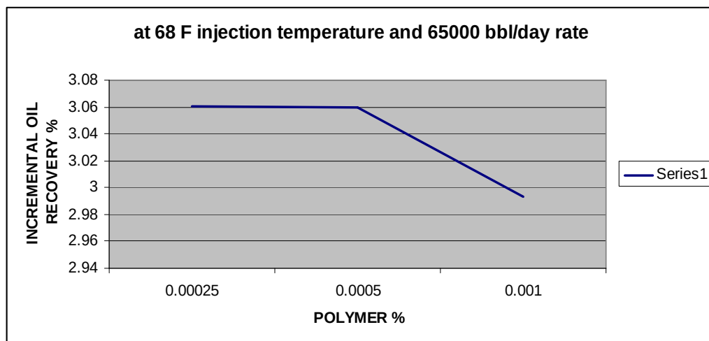
Figure 6.6 Incremental oil recovery versus polymer concentration at 68 F o
