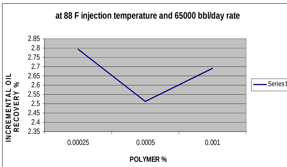
Figure 6.8 Incremental oil recovery versus polymer concentration at 88 F o
