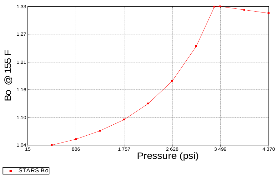
Figure C.4 Oil formation volume factor at 155°F
