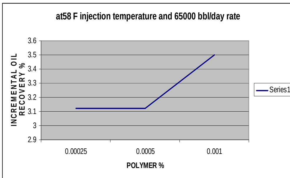
Figure 6.9 Incremental oil recovery versus polymer concentration at 58 F o
