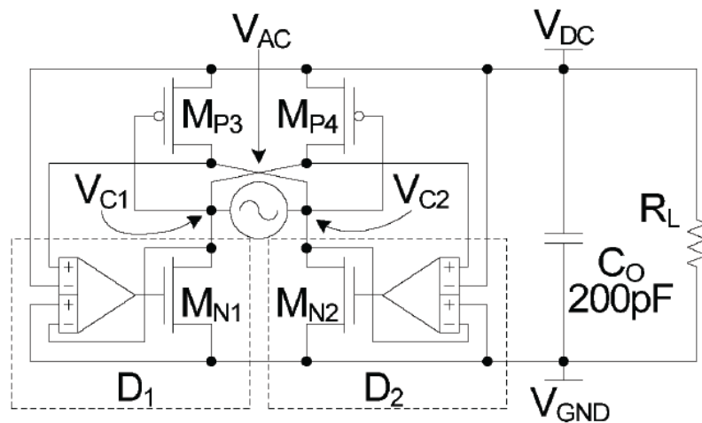
Figure 2.7: The 4-input comparator-based active rectifier utilizing RCC switching [36].
