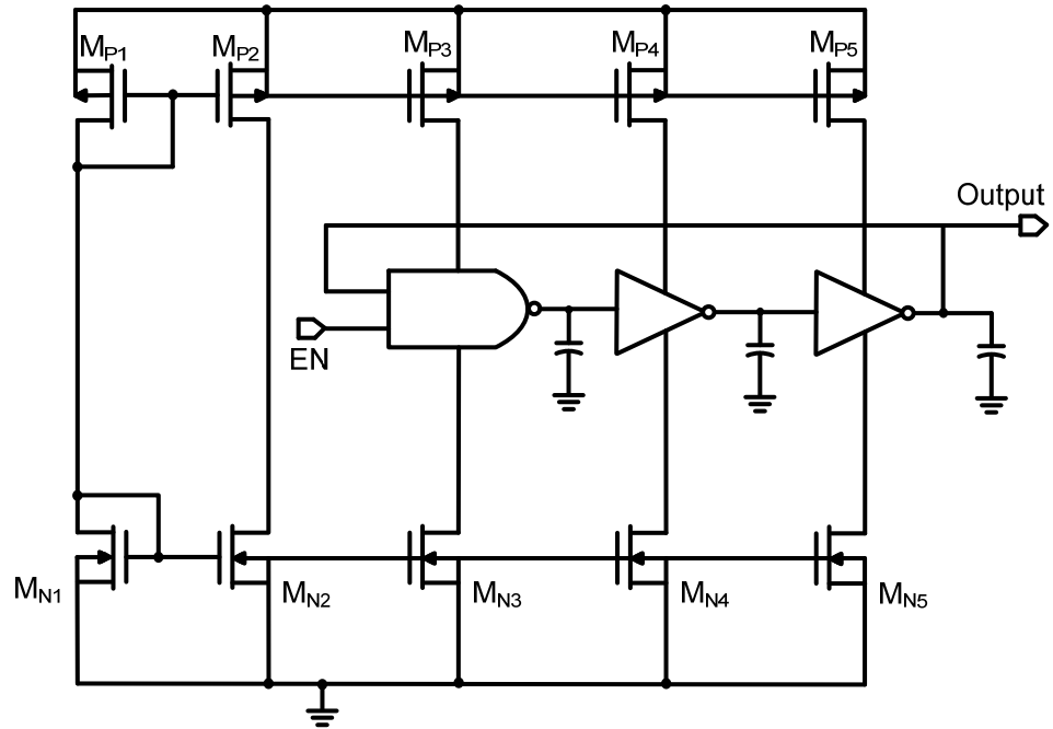
Figure 4.5: The current-starved ring oscillator designed in TSMC 90 nm CMOS process.
