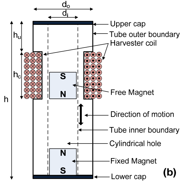
Figure 5.21: (a) The system block diagram, (b) the schematic of the energy harvester module.
