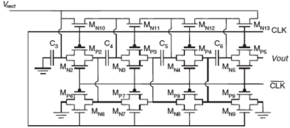
Figure 2.10: The switched capacitor DC-DC converter proposed in [44].
