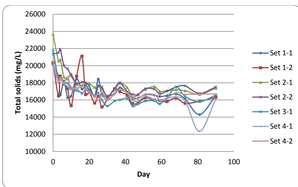
Figure 4-17: TS vs time for 2.5 L anaerobic batch reactors
