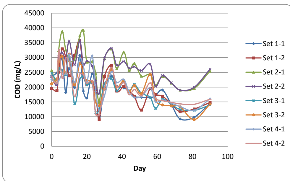
Figure 4-20: COD vs time for 2.5 L anaerobic batch reactors
