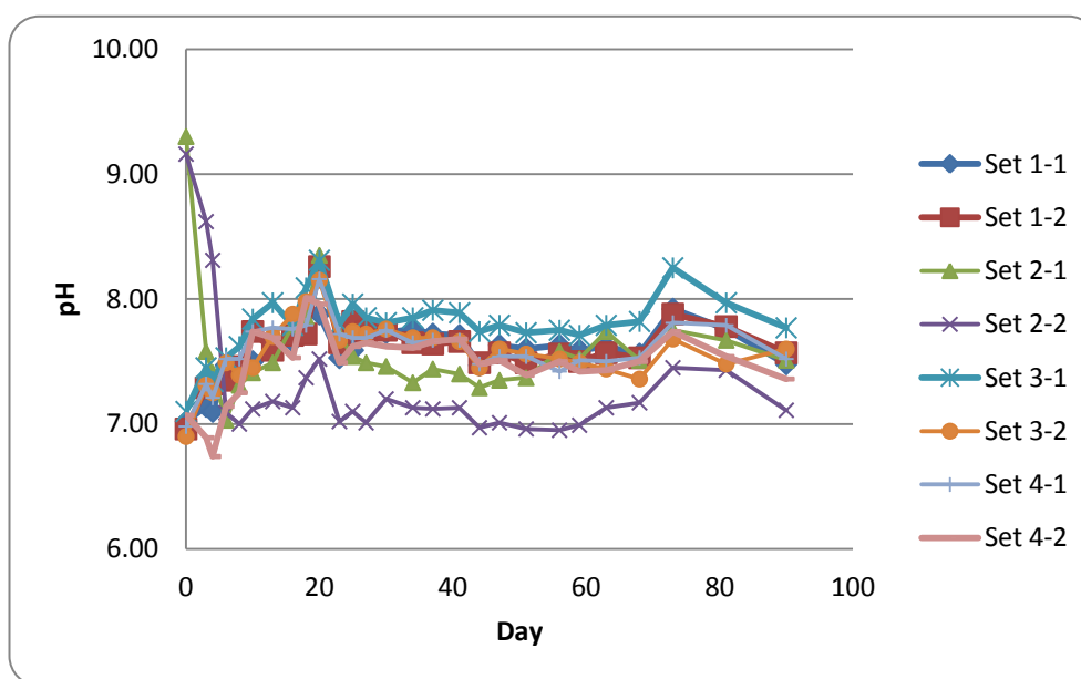
Figure 4-16: pH vs time for 2.5 L anaerobic batch reactors
