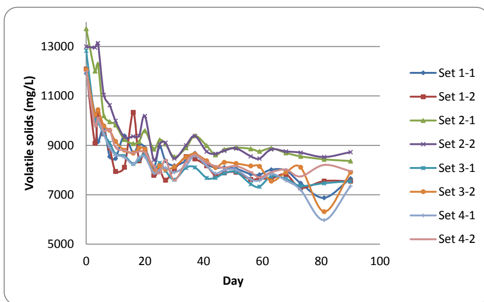
Figure 4-18: VS vs time for 2.5 L anaerobic batch reactors
