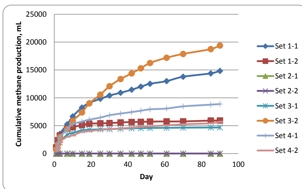
Figure 4-14: Cumulative methane production vs. time for 2.5 L anaerobic batch reactors – all reactors included
