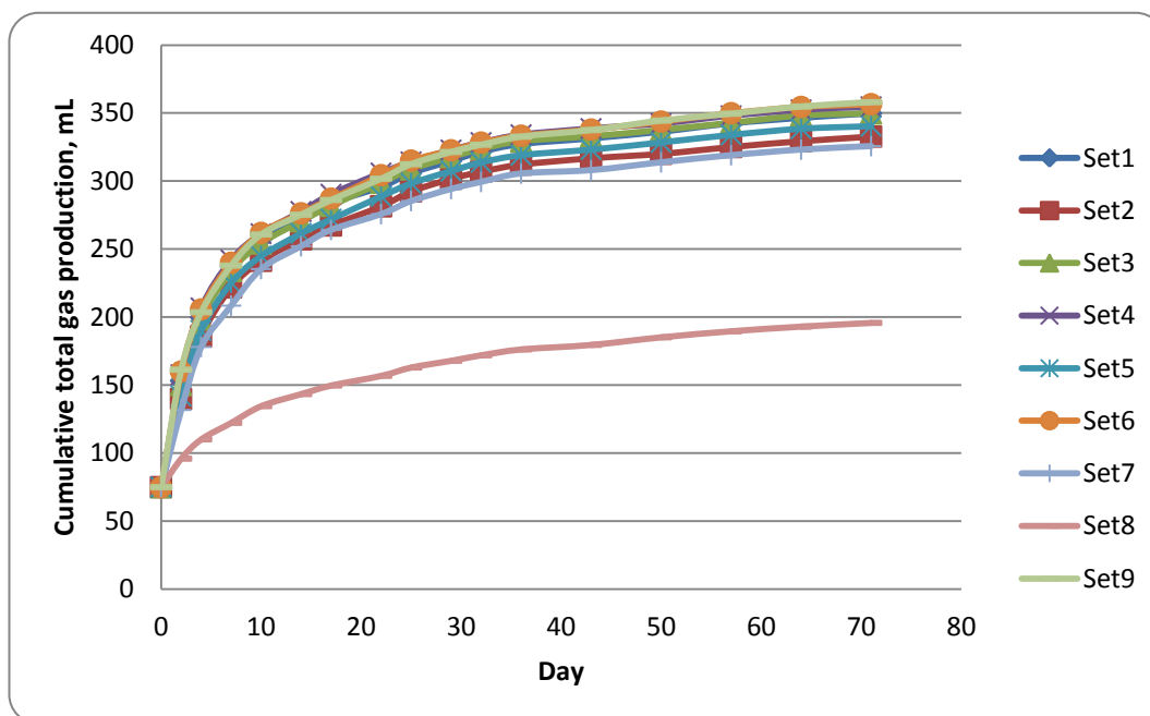
Figure 4-8: Cumulative total gas production vs. time for NP (branched)
