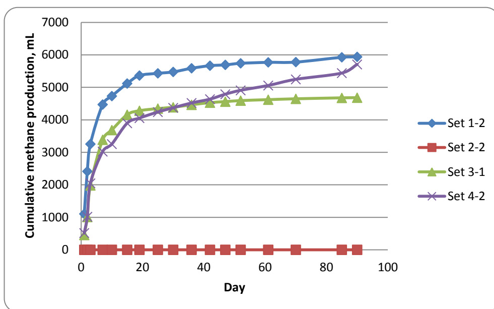
Figure 4-15: Cumulative methane production vs. time for 2.5 L anaerobic batch reactors – excluding suspected leaking reactors
