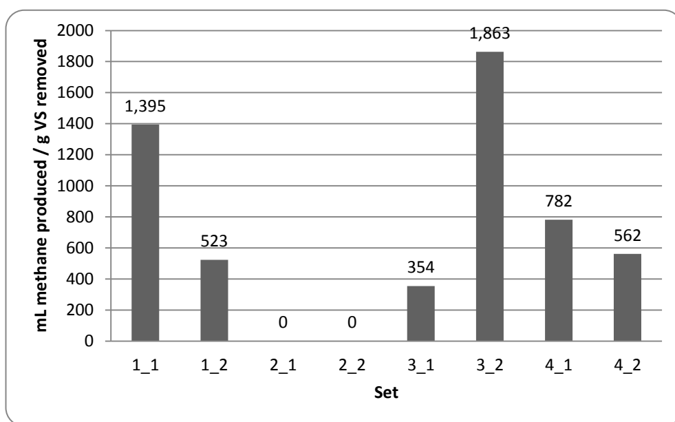
Figure 4-19: mL CH 4 produced per g VS removal for 2.5 L anaerobic batch reactors
