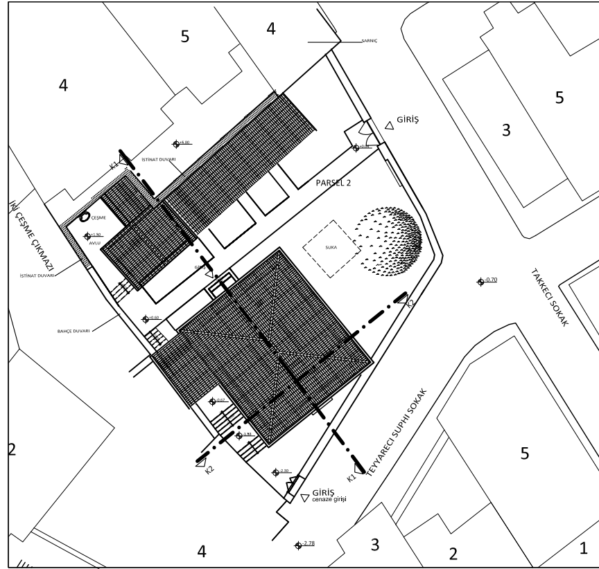
VAZİYET PLANI 1/200
