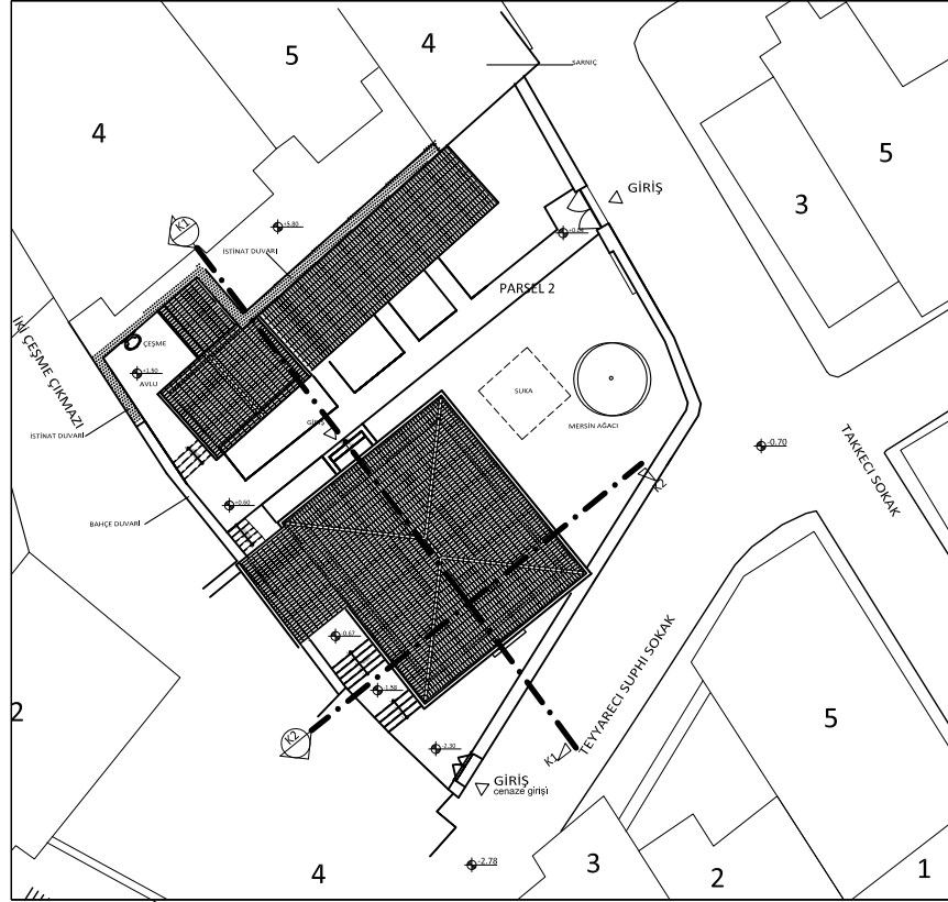
VAZİYET PLANI 1/200
