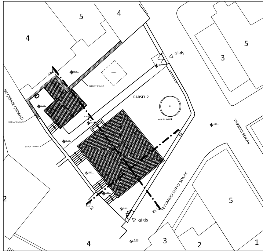
VAZİYET PLANI 1/200
