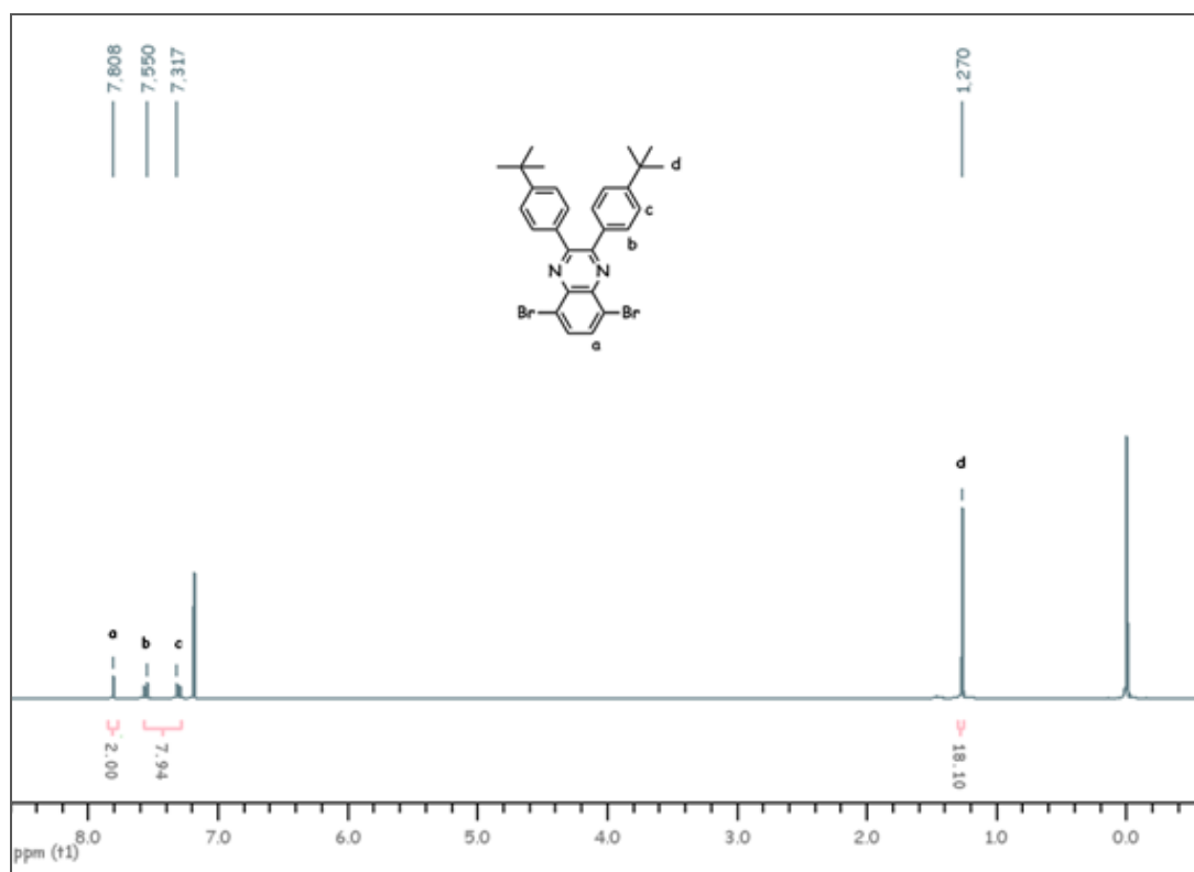
Figure A.2 ^1\text{H} -NMR spectrum of 5,8-dibromo-2,3-bis(4- tert -butylphenyl)quinoxaline (3)
