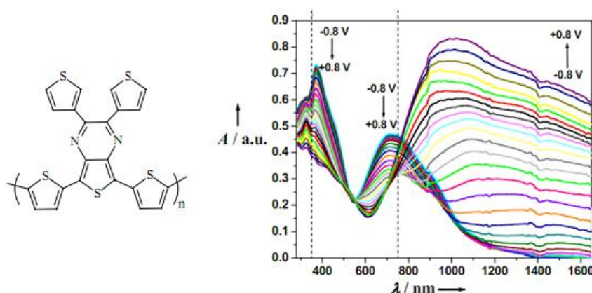
Figure 1.17 The structure and absorption spectrum of PDDTP
