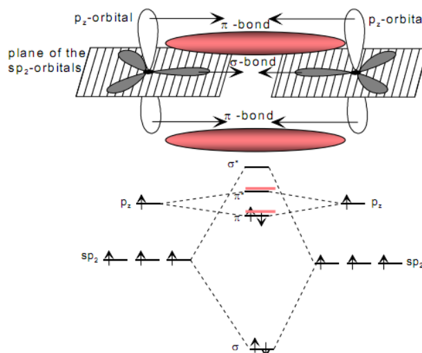
Figure 1.5 The representation of overlapping in n orbitals
