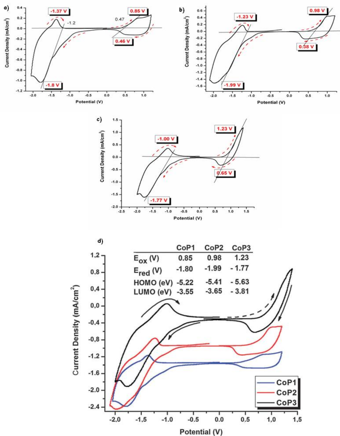
Figure 3.3 CVs and onset potentials of a) CoP1, b) CoP2, c) CoP3 and d) oxidation/reduction potentials and HOMO-LUMO levels of polymer films vs. \text{Fc}/\text{Fc}^+ in 0.1 M \text{TBAPF}_6/\text{ACN} .
