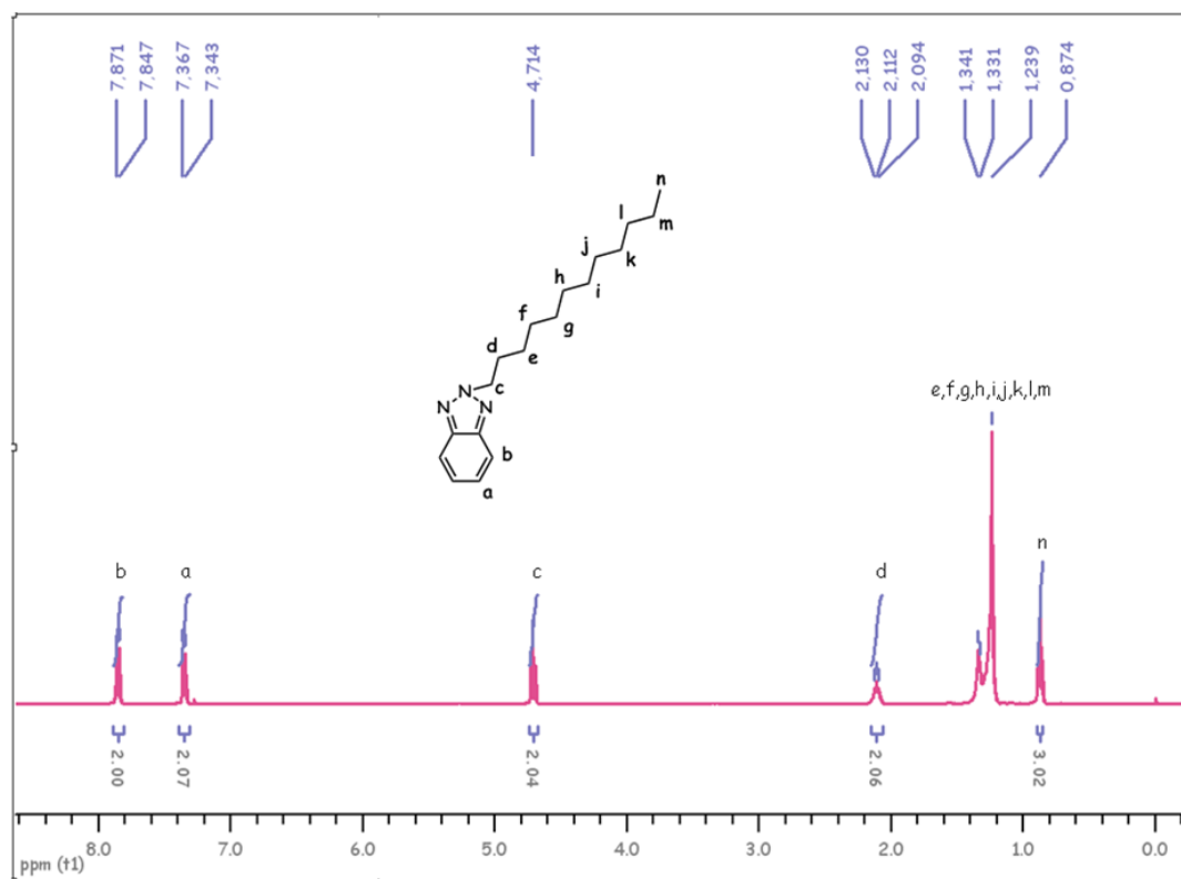
Figure A.5 ^1\text{H} -NMR spectrum of 2-dodecyl-2H-benzo[d][1,2,3]triazole (6)
