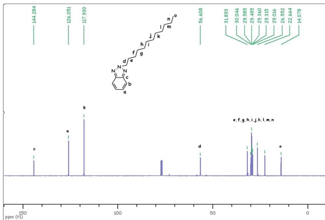
Figure A.6 ^{13}\text{C} -NMR spectrum of 2-dodecyl-2H-benzo[d][1,2,3]triazole (6)
