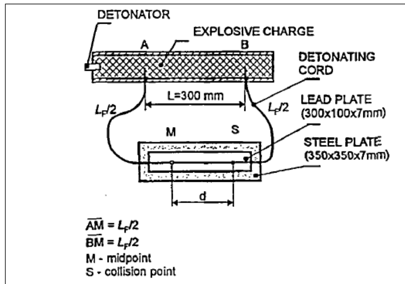
Figure 2.14 Determination of detonation velocity by Dautriché's method (Suceska, 1995)
