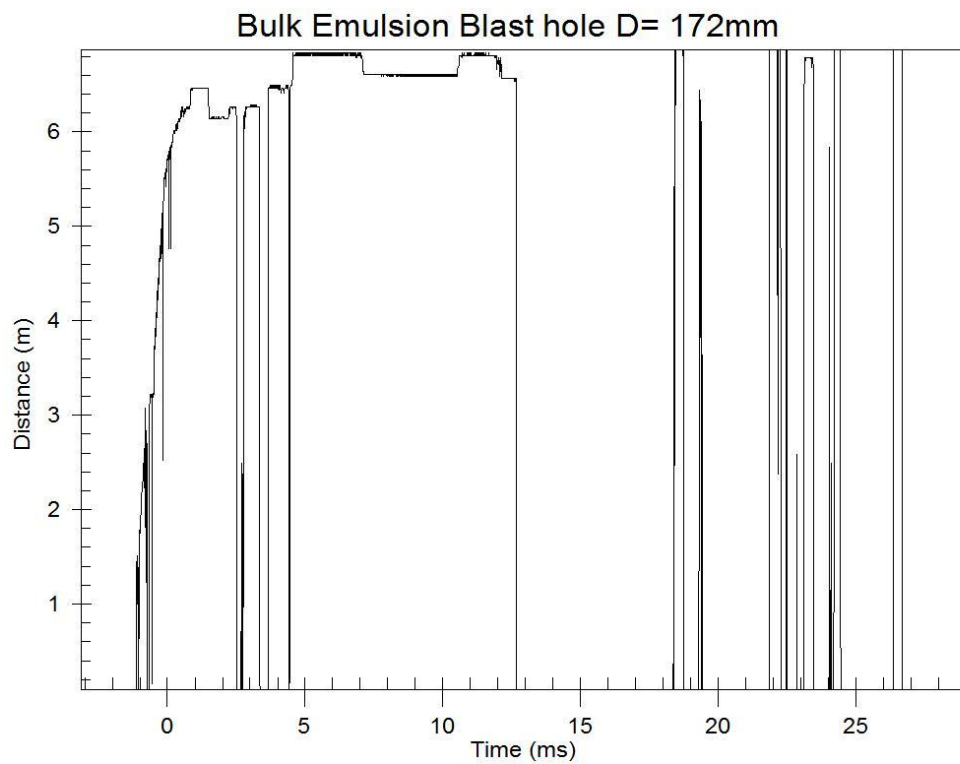
Figure B.21 The original VOD graph for blast pattern 3706-1
