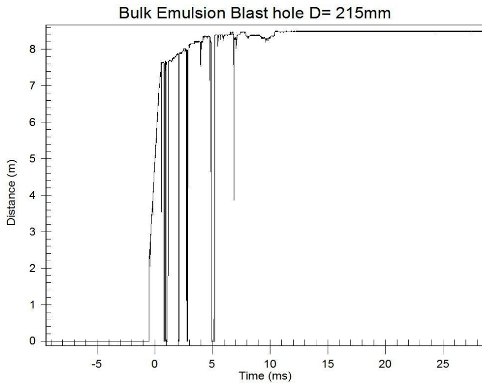
Figure B.15 The original VOD graph for blast pattern 3786-52
