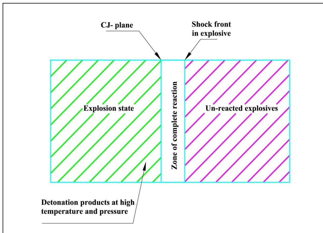
Figure 2.8 Features of ideal detonation process of explosive (Brinkmann, 1990)
