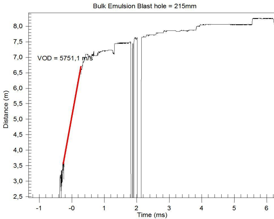
Figure B.14 VOD result for blast pattern 3834-300a
