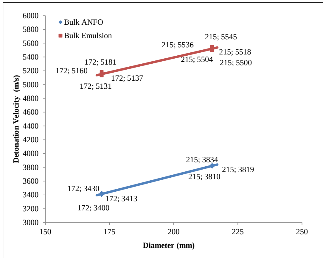
Figure 4.3 Effect of explosive type on VOD in ore metasomatite
