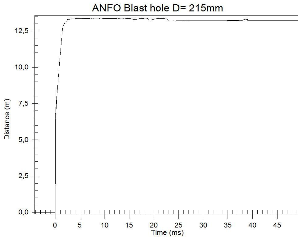
Figure A.11 The original VOD graph for blast pattern 4082-299
