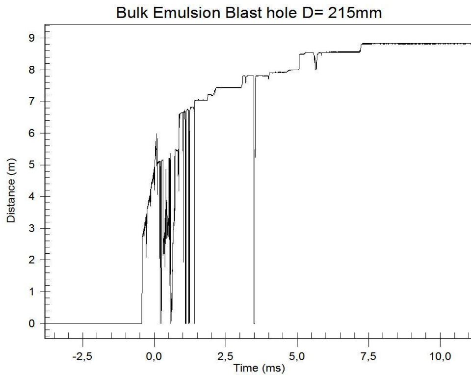
Figure B.33 The original VOD graph for blast pattern 3786-53
