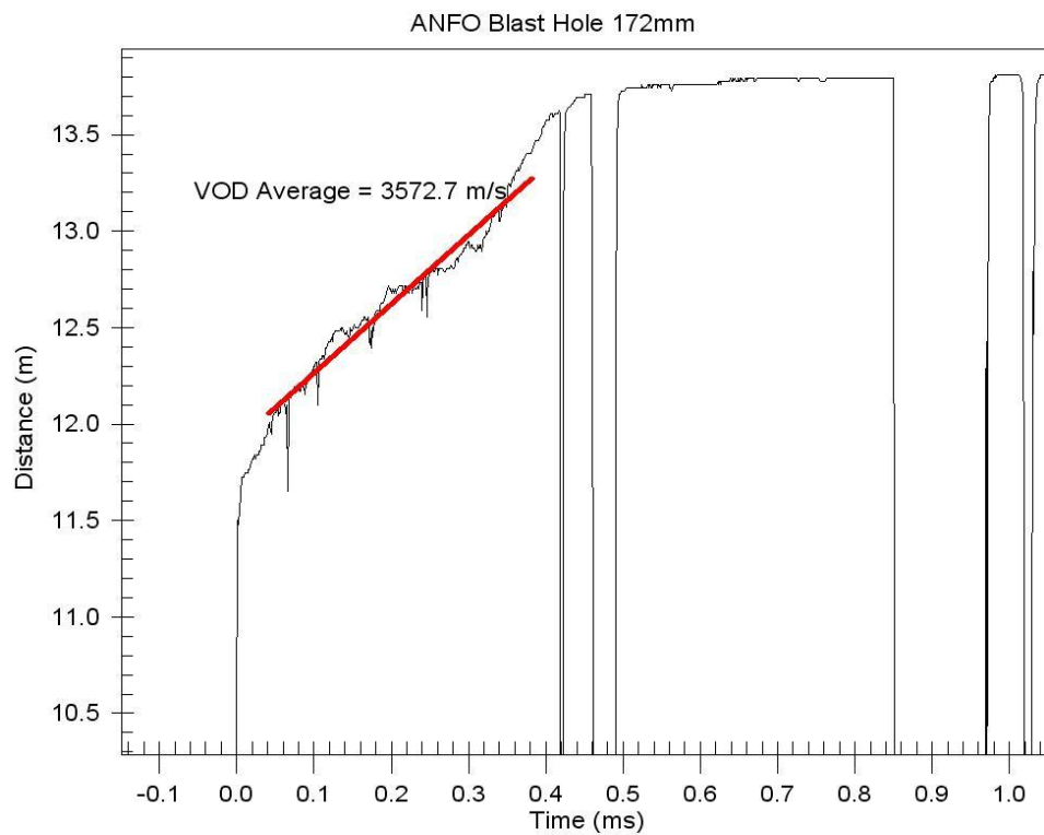
Figure A.4 VOD result for blast pattern 3834-107
