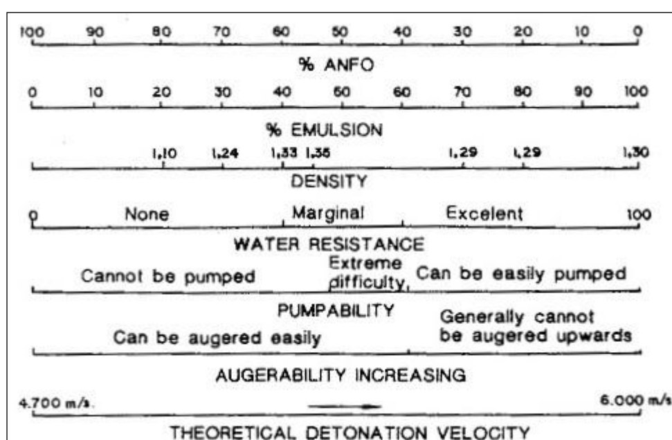
Figure 3.14 Charging and main characteristics of different types of blends (Jimeno and Carcedo, 1995)
