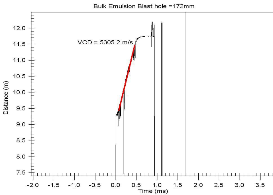
Figure B.8 VOD result for blast pattern 3842-145
