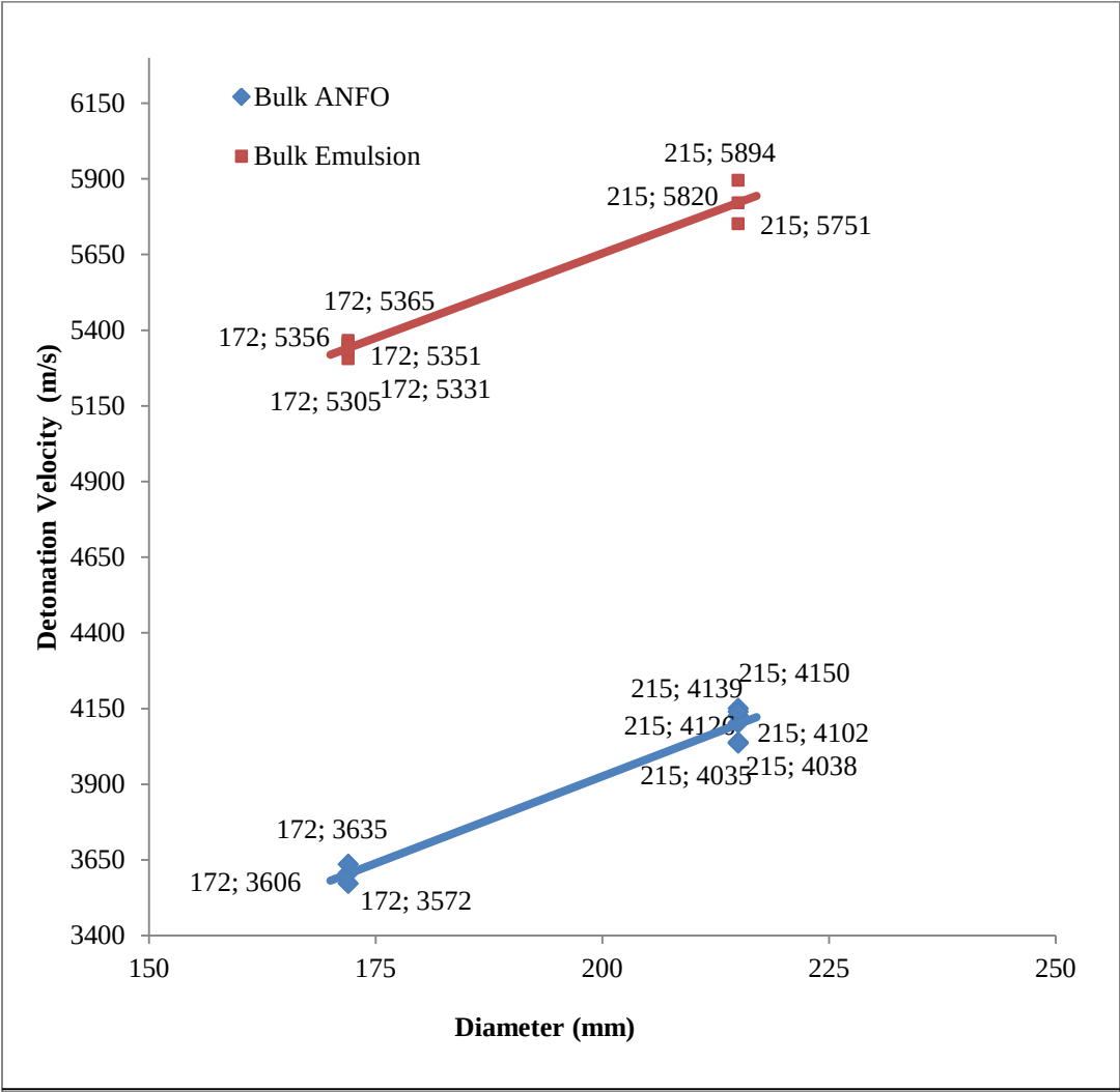
Figure 4.2 Effect of explosive type on VOD in Phyllite
