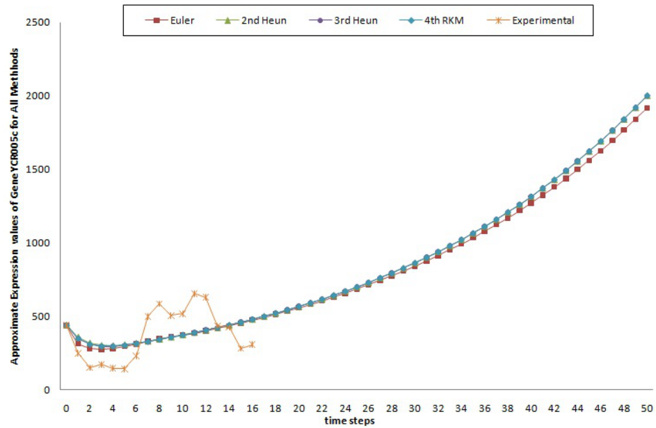
Figure 4.86: Results of all 4 schemes for Gene YCR005c by considering original model
