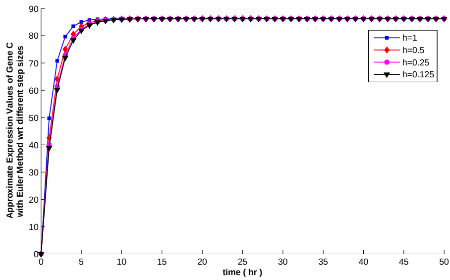
Figure 4.8: Results of Gene C using different step-sizes with Euler method
