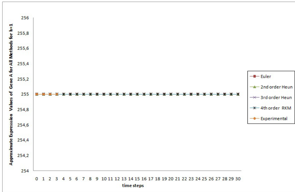
Figure 4.2: Results of Gene A using different methods for fixed data and fixed step-size
