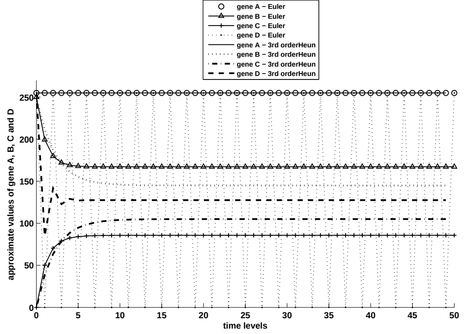
Figure 4.1: Approximate results of gene-expressions of all genes by using Euler's and 3^{rd} -order Heun's methods.
