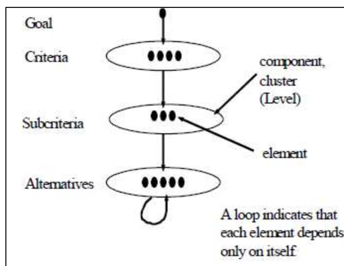
Figure 4.1. Linear Hierarchy (Saaty, 2008)
