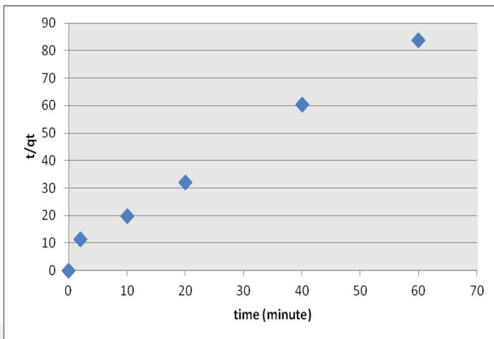
Figure 4.19 : The pseudo-second-order model plots of BPA by resin1
