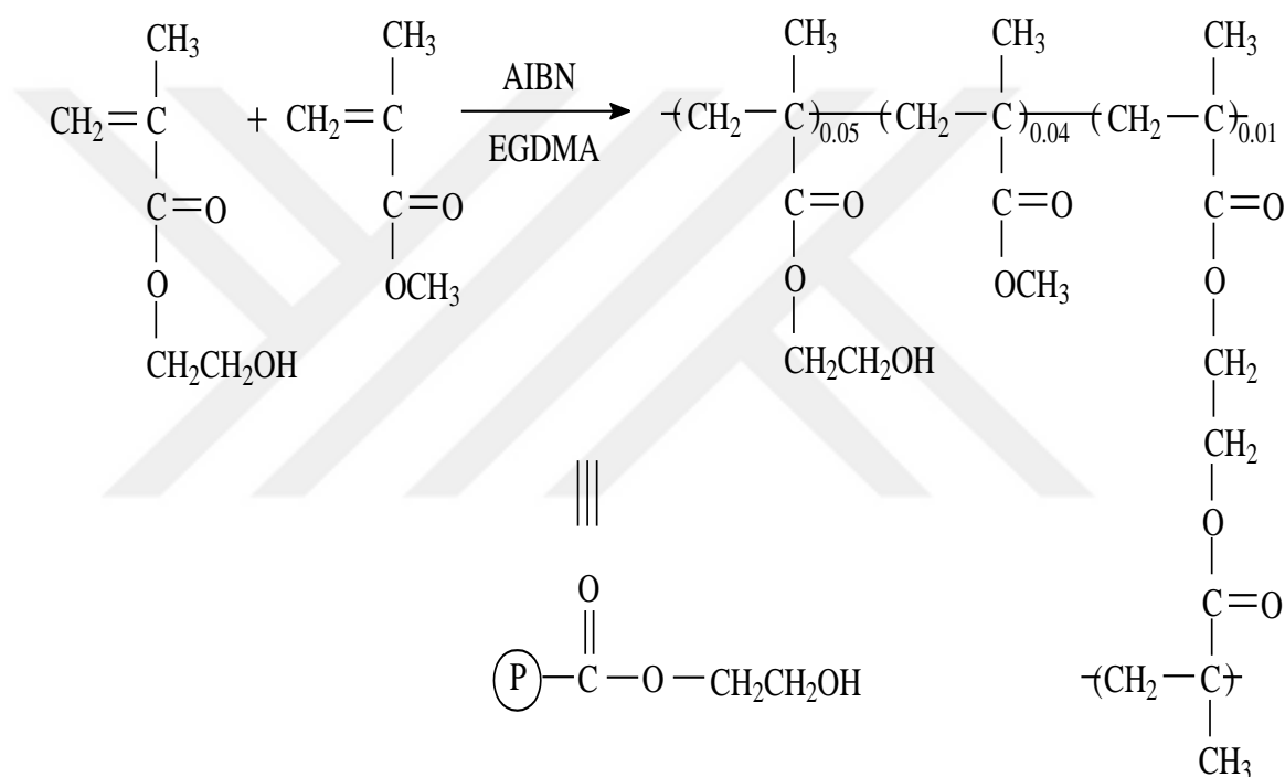
Figure 4.1 : Crosslinked poly (HEMA-co-MMA) beads.
