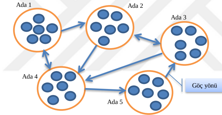
Şekil 2.8 : Ada modeli (Island/Coarse-Grained).
