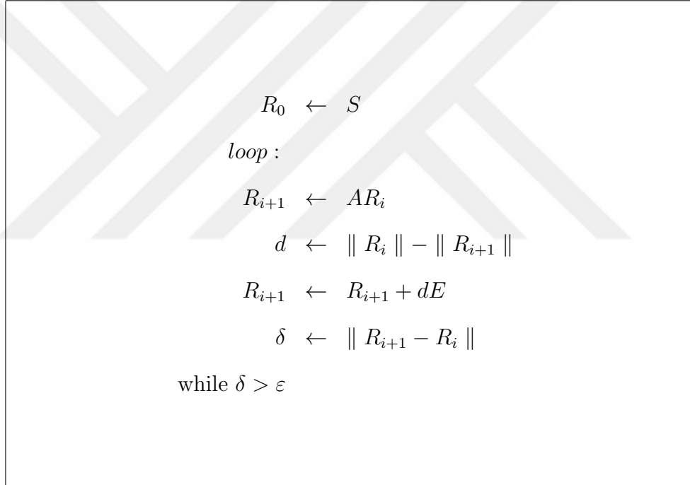
Figure 3.2. PageRank algorithm.
