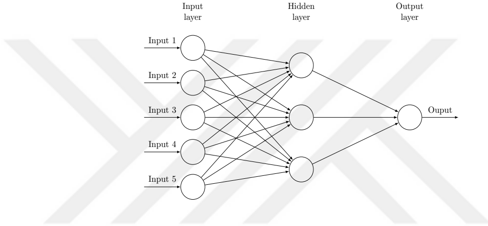
Figure 3.5. A multilayer perceptron.
