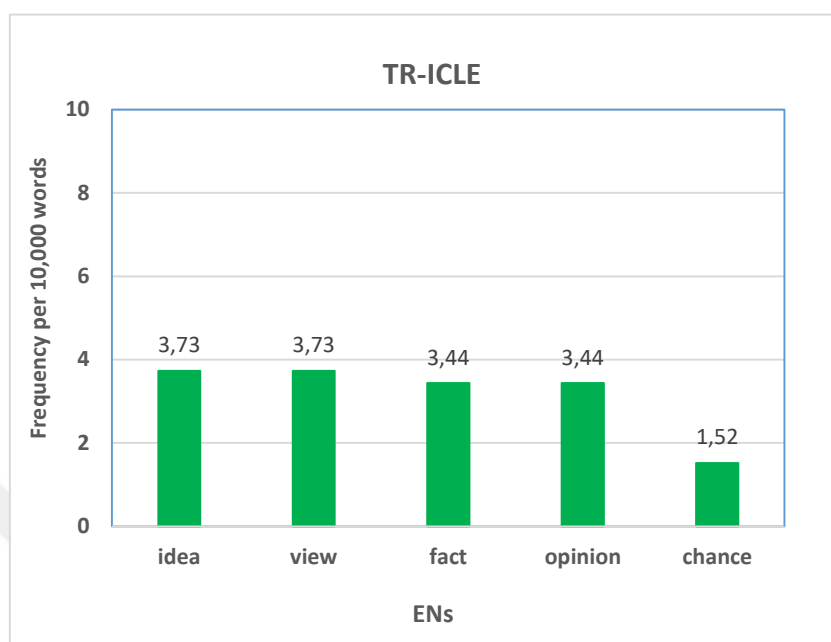
Figure 4.29. Top five ENs in TR-ICLE
