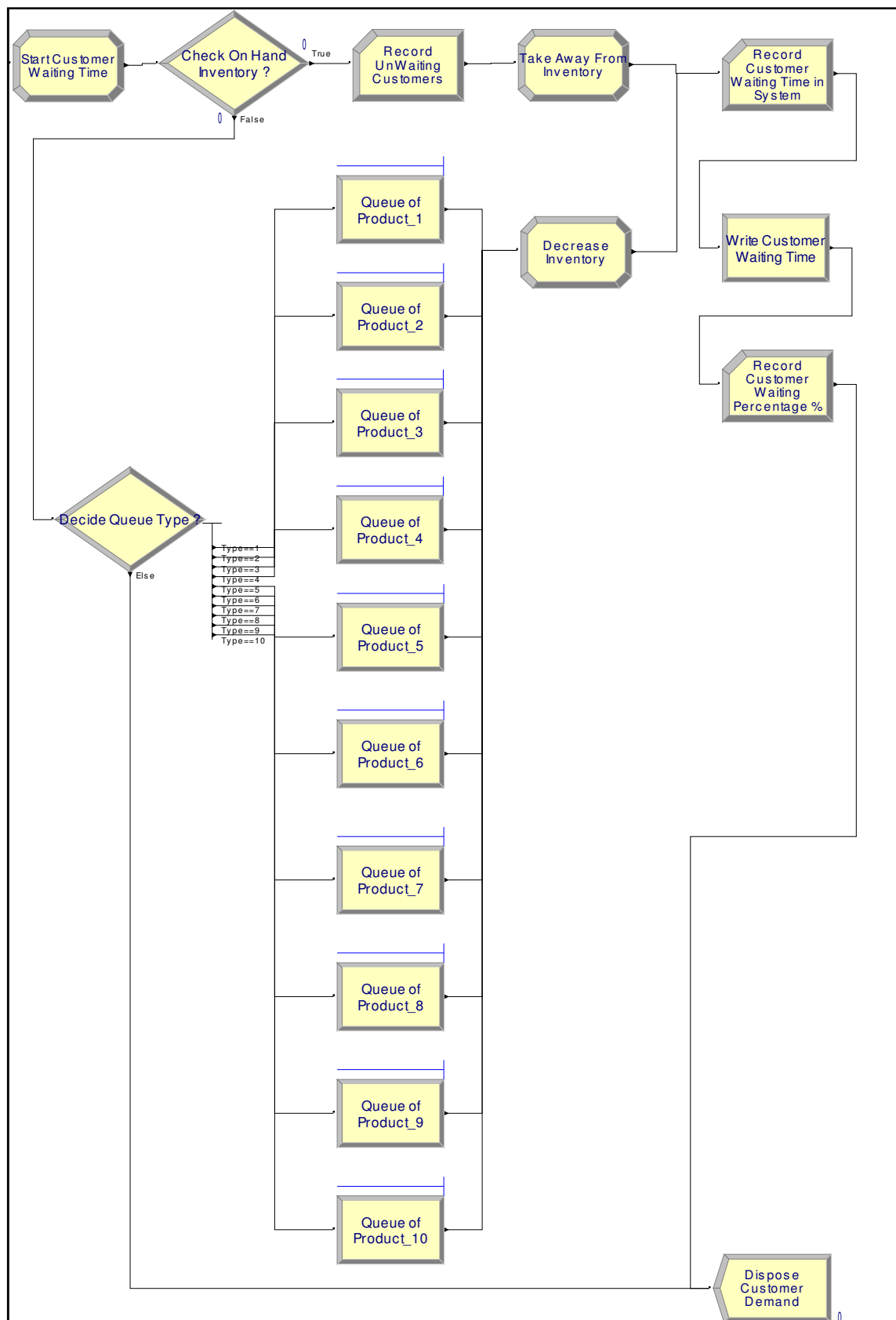
Figure 5.15. Demand management segment
