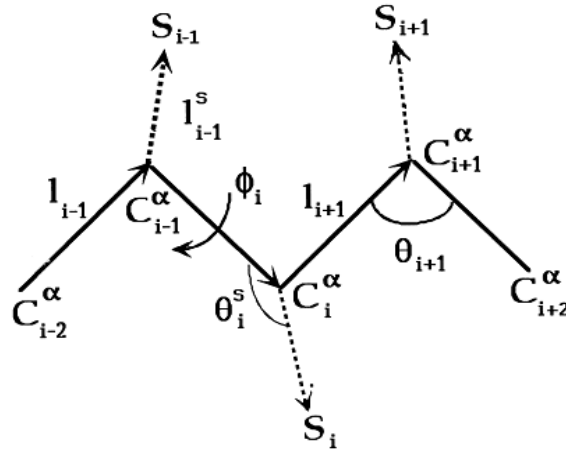
Figure 3.1. Schematic representation of the virtual bond model
