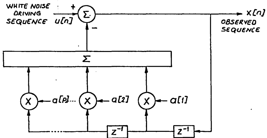
Figure 3.1.1. Autoregressive model of random process
