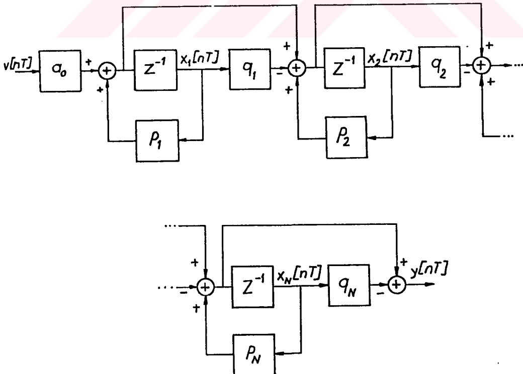
Figure 3.6.6. Cascade form realization of transfer function G(z)
