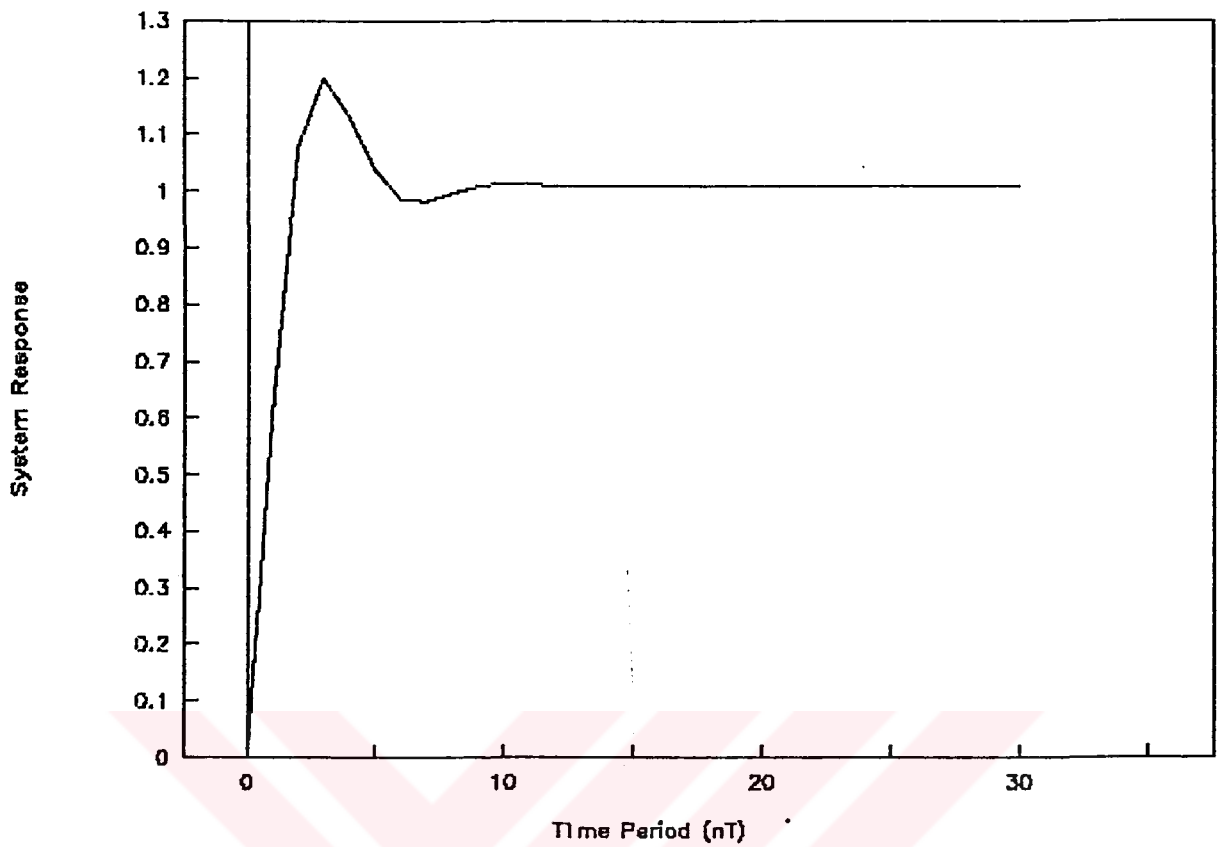
Figure 5.5. Step response of Real transfer function for the first test case
