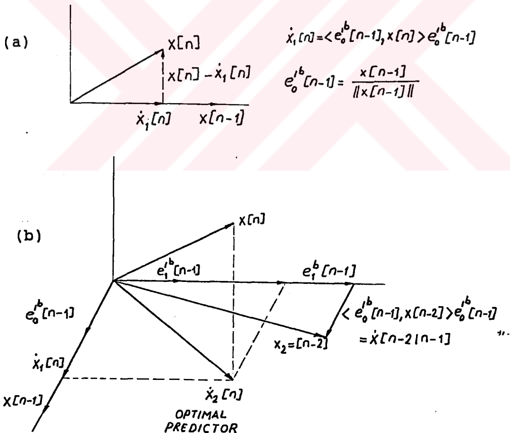
Figure 3.1.4. Vector space interpretation of linear prediction (a) First prediction (b) Second order predictor
