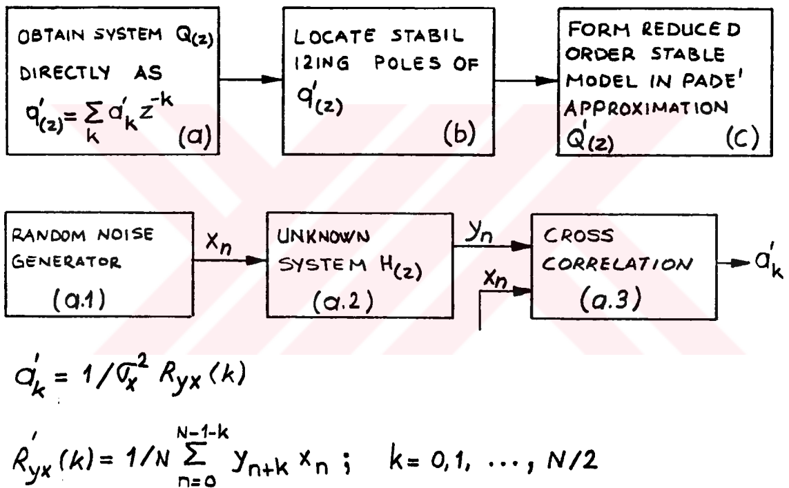
Figure 3.4.2. Pade' approximation Biyiksiz approach
