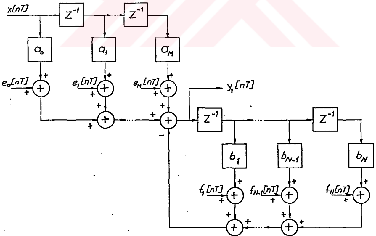
Figure 4.3.1. Noise in a type 0 direct form recursive filter realization caused by fixed point finite word length arithmetic
