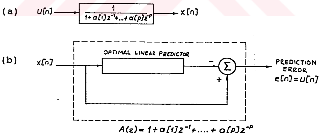
Figure 3.1.3. Filtering interpretation of linear prediction (a) AR model of order p . (b) Prediction error filter
