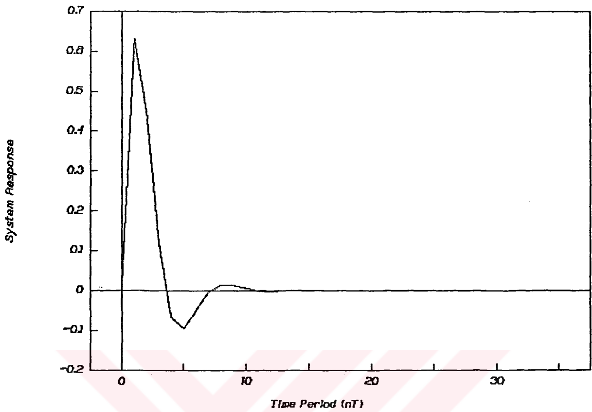
Figure 5.1. Impulse response of Real transfer functions of the first test case
