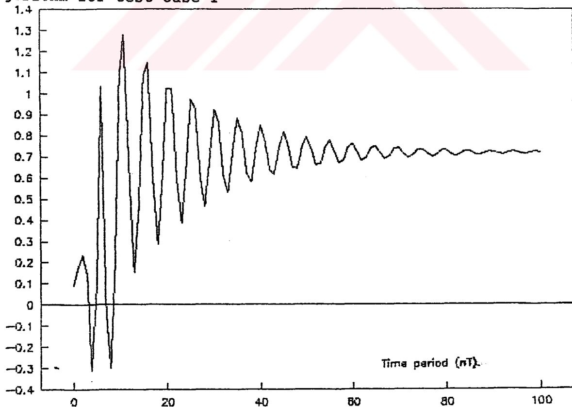
Figure 5.12. Step response of higher order ARMA MYWE algorithm for test case 1
