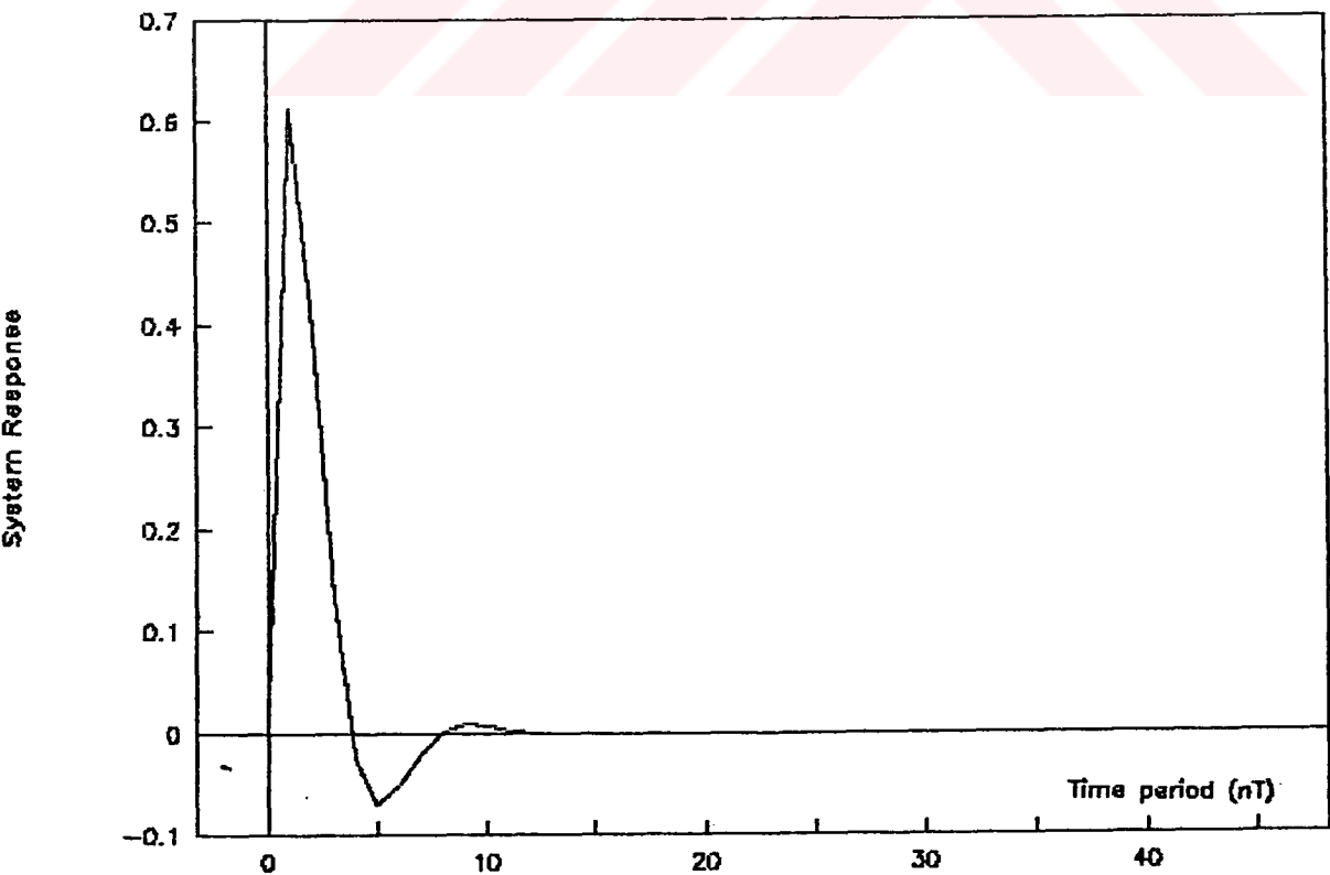
Figure 5.20. Impulse response of Pade' transfer function for the test case 2
