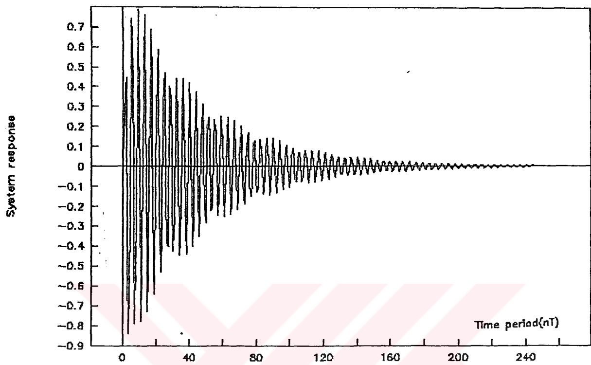
Figure 5.19. Impulse response of real transfer function for the test case 2
