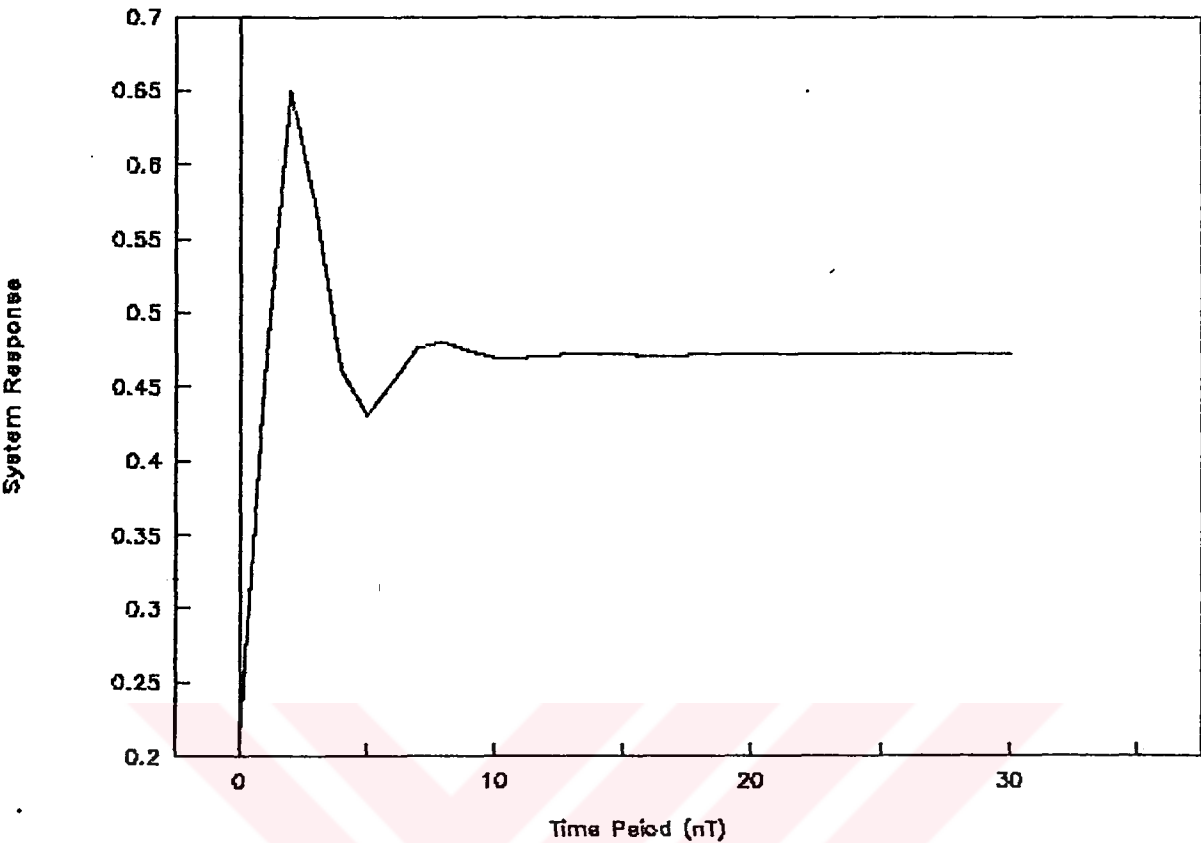
Figure 5.7. Step response of ARMA MYWE transfer function for the first test case
