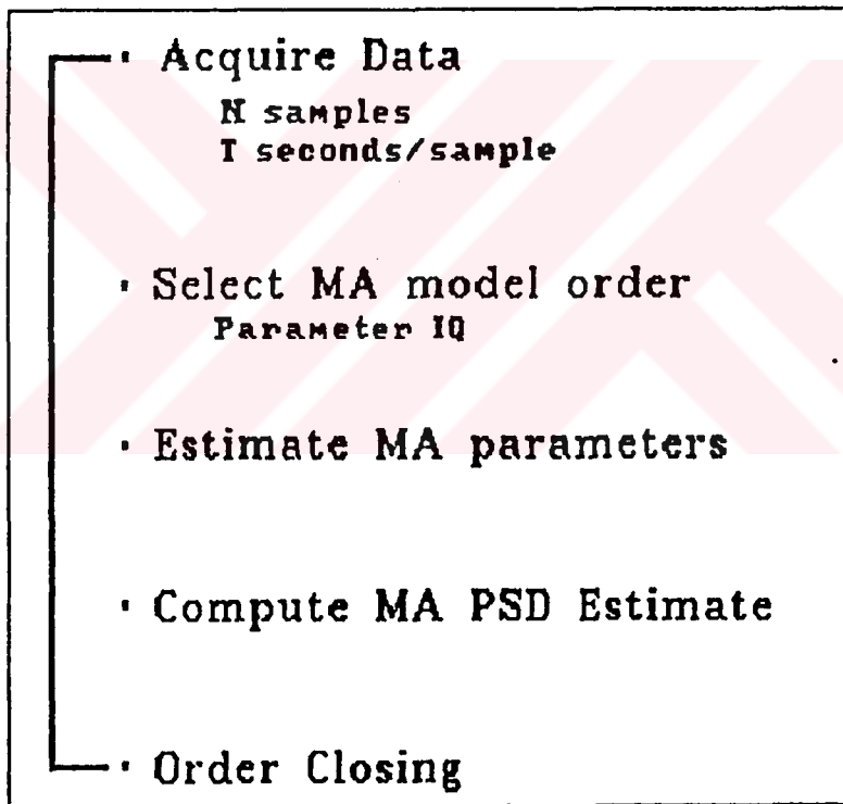
Figure 3.2.2. Summary of MA modelling technique
