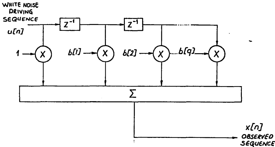
Figure 3.2.1. Moving Average model of random process
