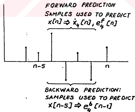
Figure 3.1.5. Illustration of forward and backward prediction
