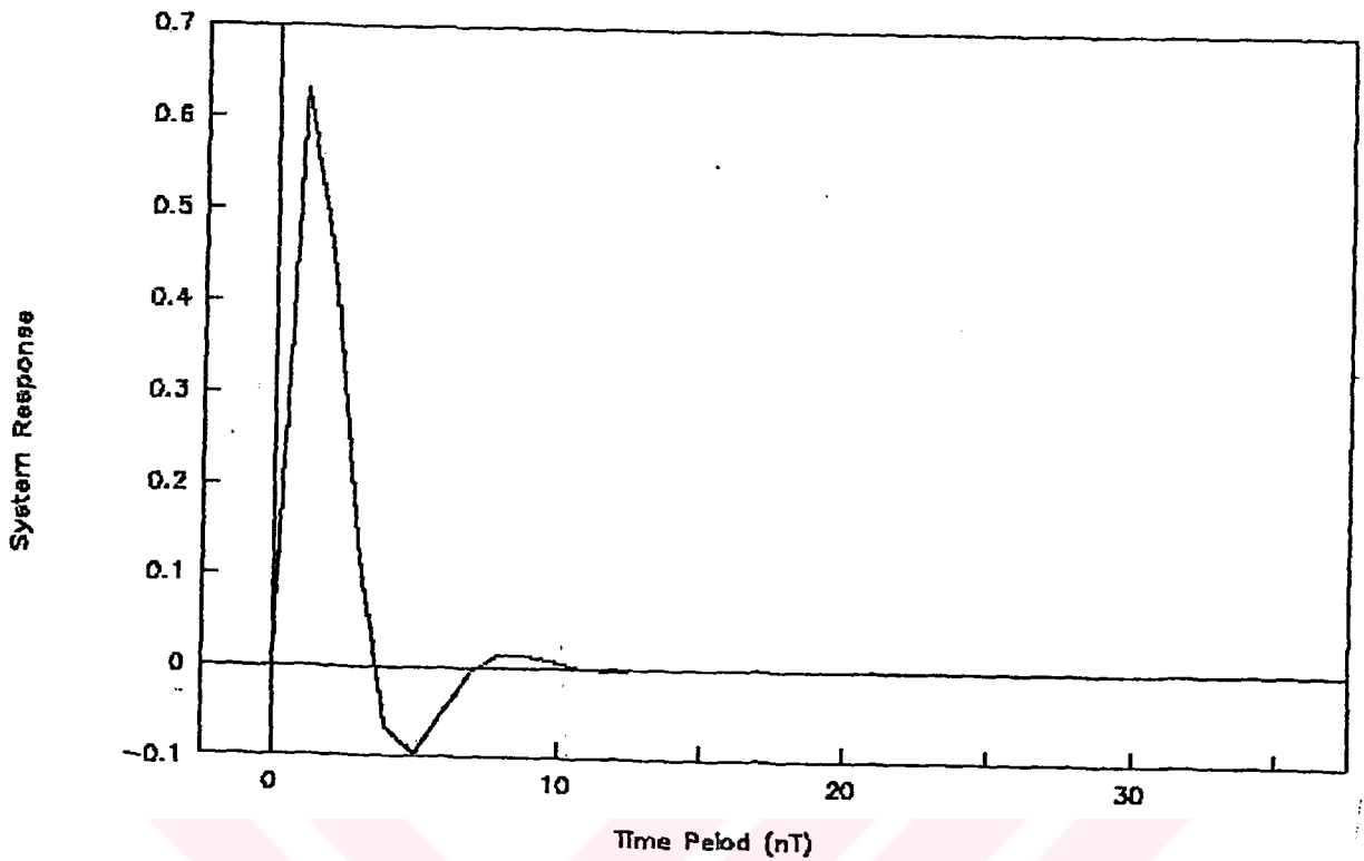
Figure 5.3. Impulse response of ARMA MYWE transfer function for the first test case
