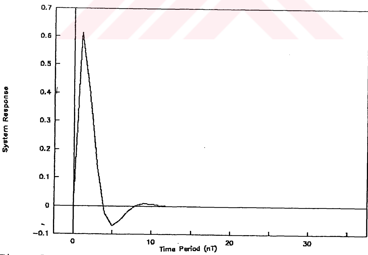
Figure 5.2. Impulse response of Pade' transfer function of the first test case
