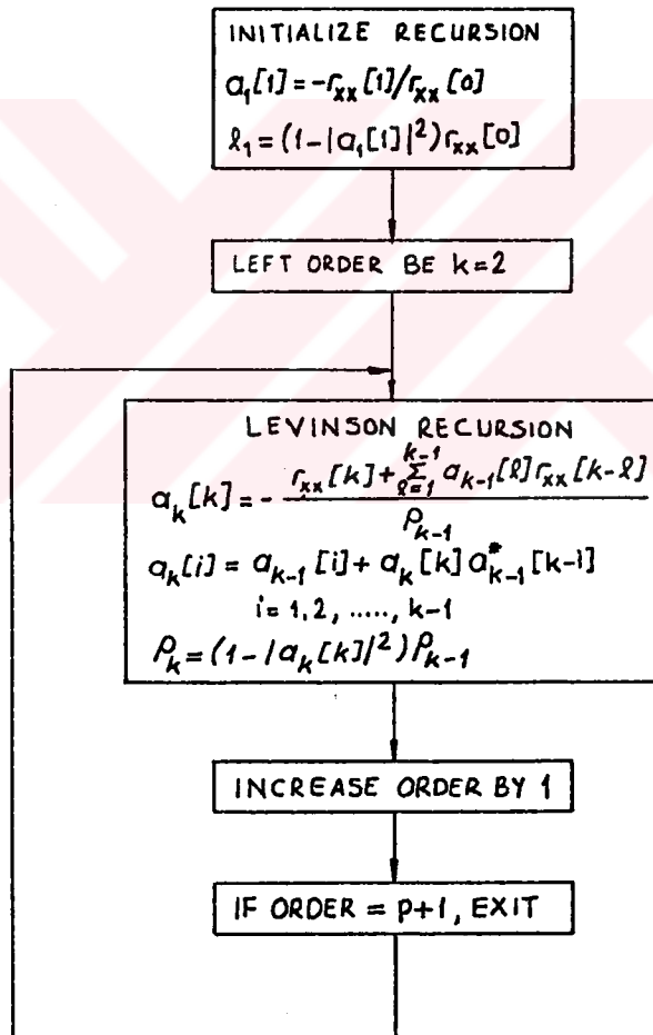
Figure 3.1.6. Summary of Levinson recursion
