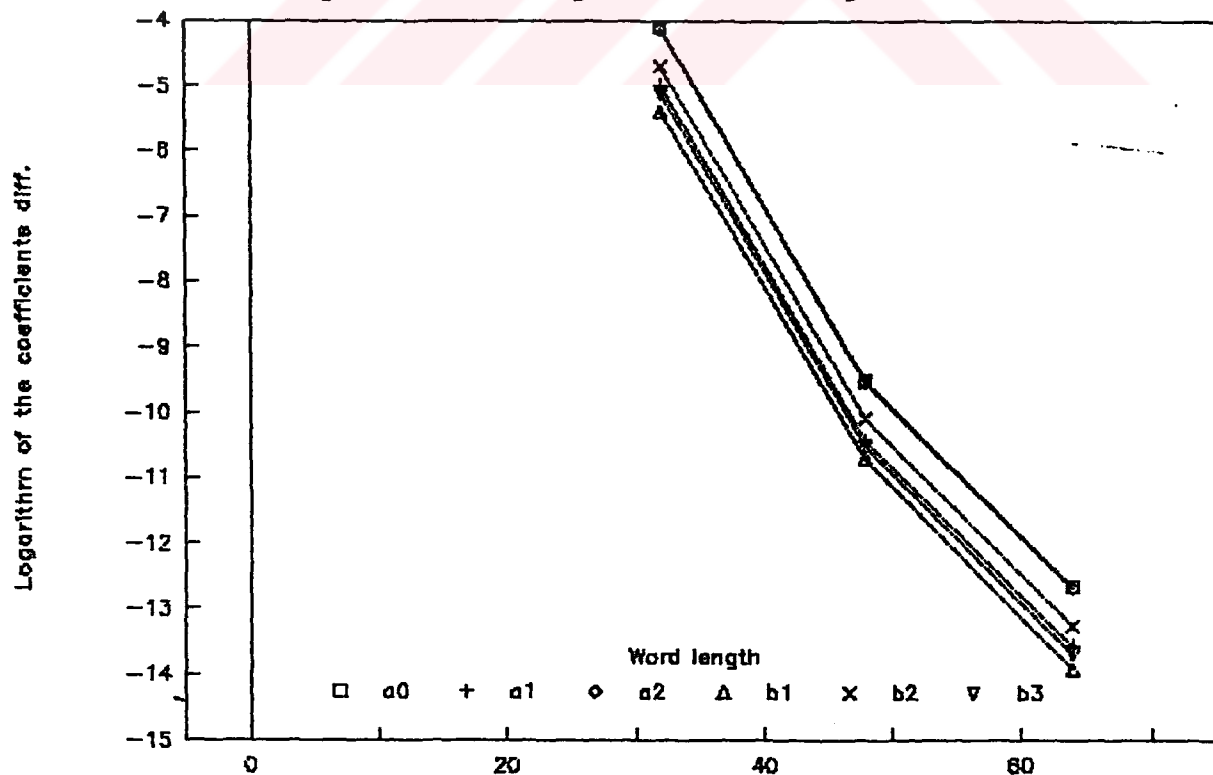
Figure 5.31. ARMA MYWE transfer function: Logarithm of coefficient errors according to the change of word length
