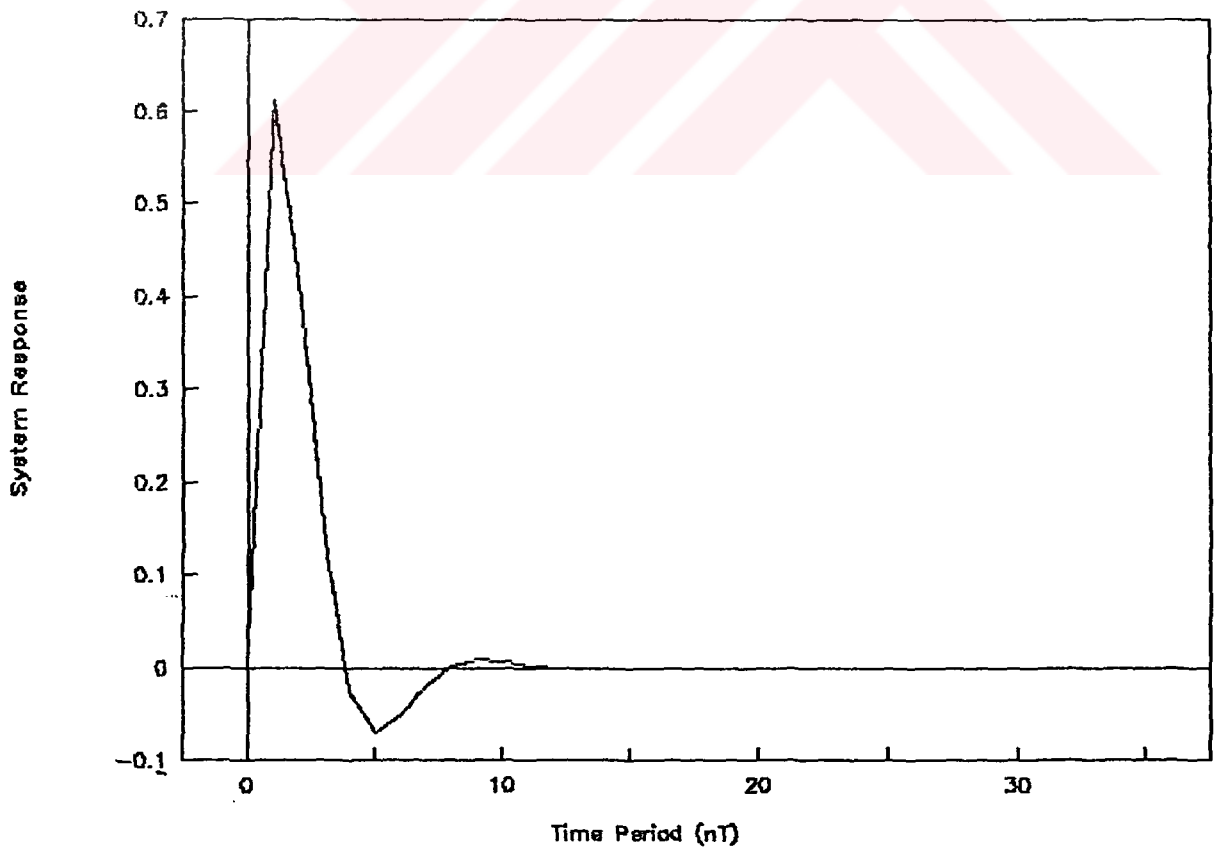
Figure 5.4. Impulse response of ARMA AKAIKE transfer function for the first test case
