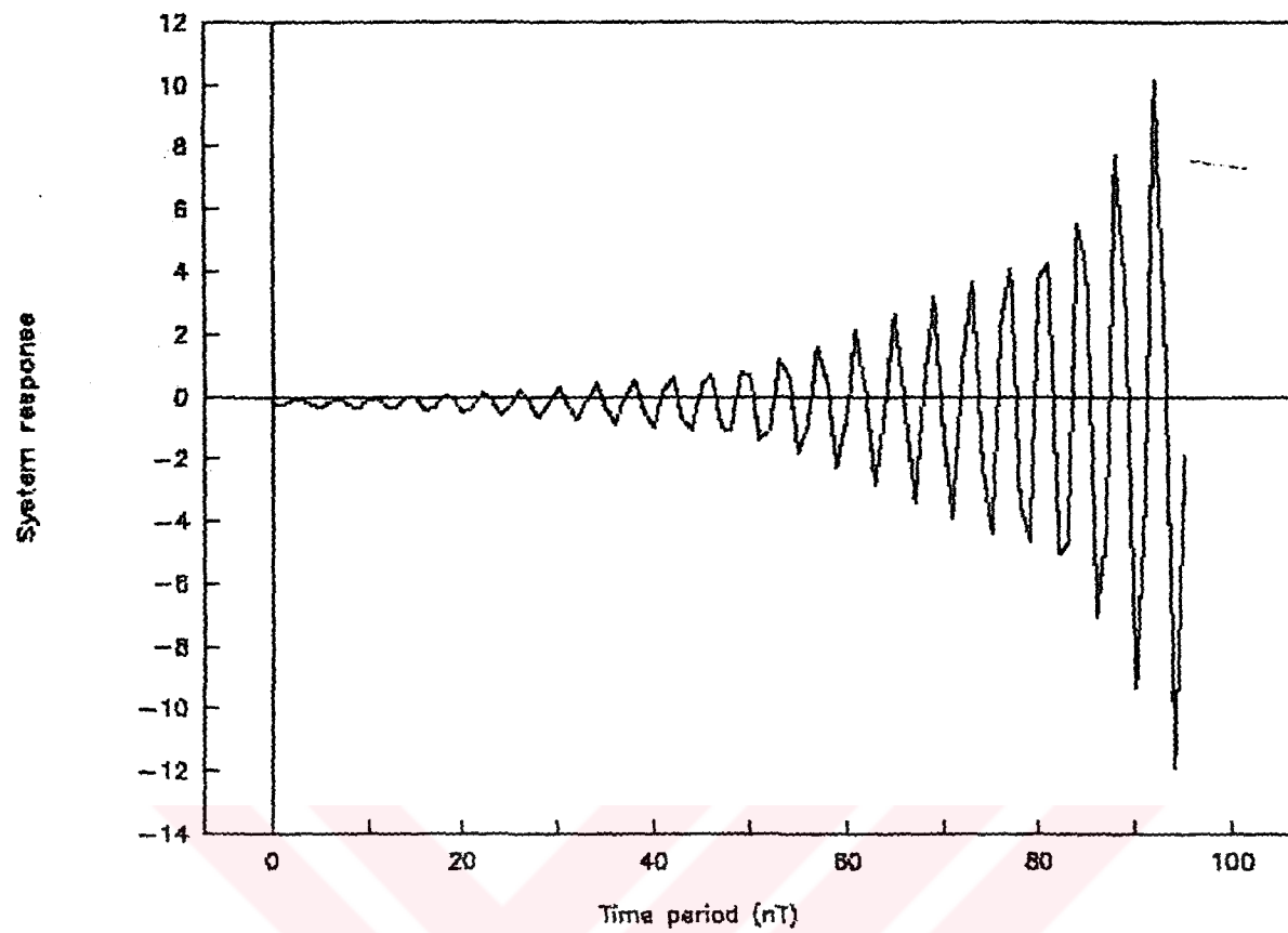
Figure 5.25. Step response of ARMA MYWE transfer function for the test case 2
