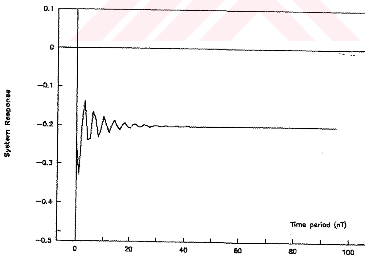
Figure 5.26 Step response of ARMA AKAIKE transfer function for the test case 2
