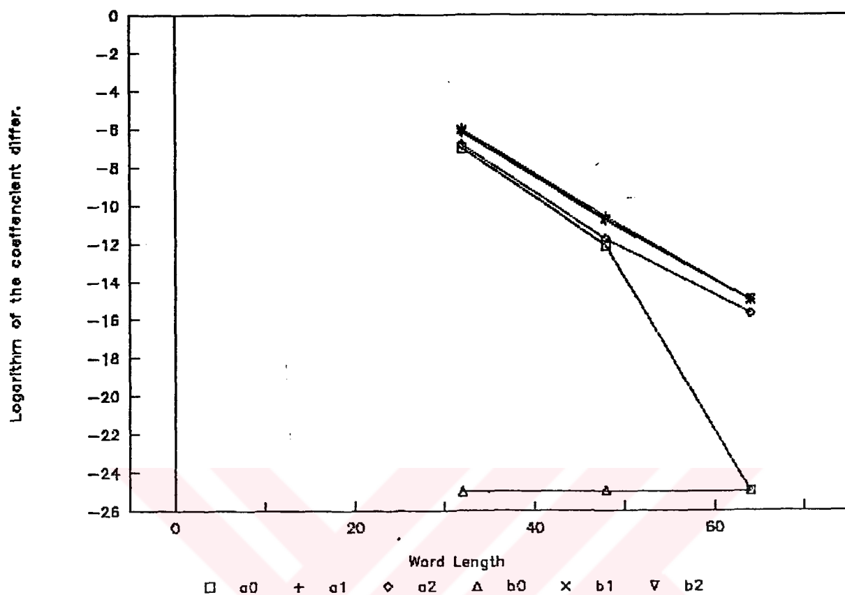
Figure 5.17 ARMA MYWE transfer function : Logarithm of coefficient errors according to the change of word length
