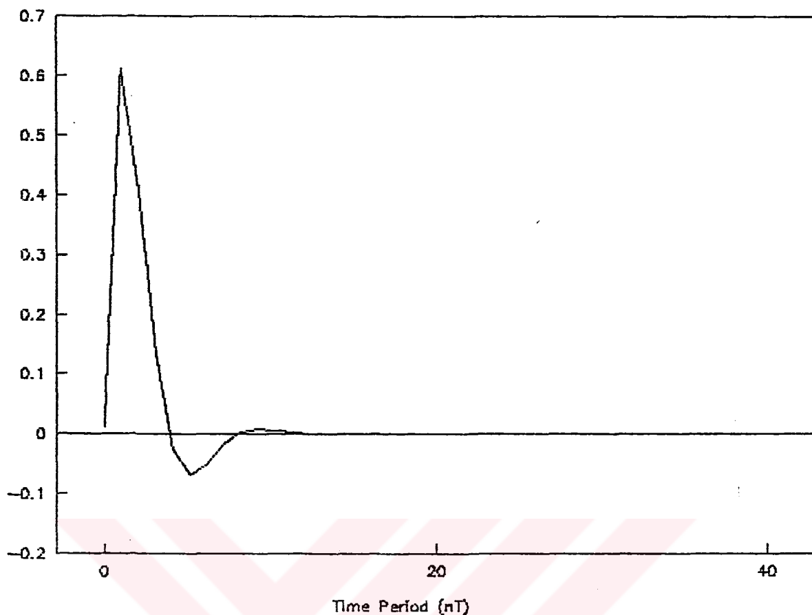
Figure 5.10. Impulse response of higher order ARMA AKAIKE algorithm for test case 1
