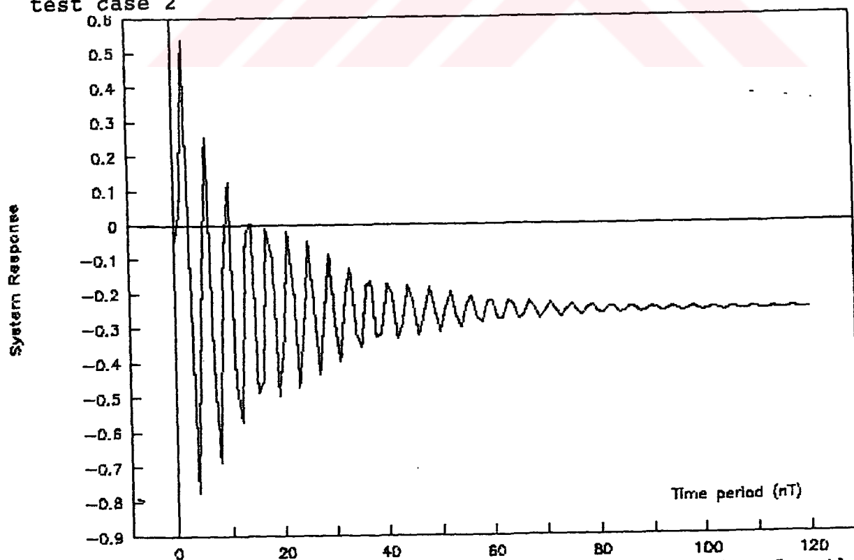
Figure 5.24. Step response of Pade' transfer function for the test case 2
