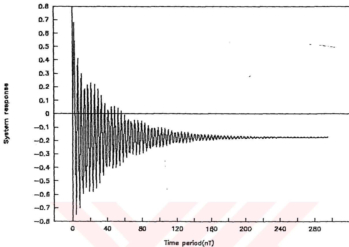
Figure 5.23 Step response of Real transfer function for the test case 2
