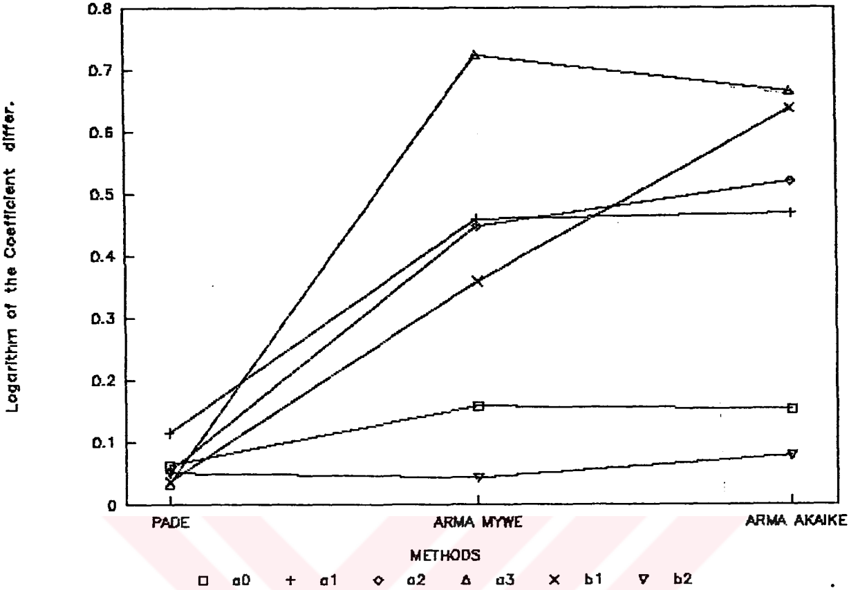
Figure 5.28 Coefficients error of simulated methods according to the extended data representation type
