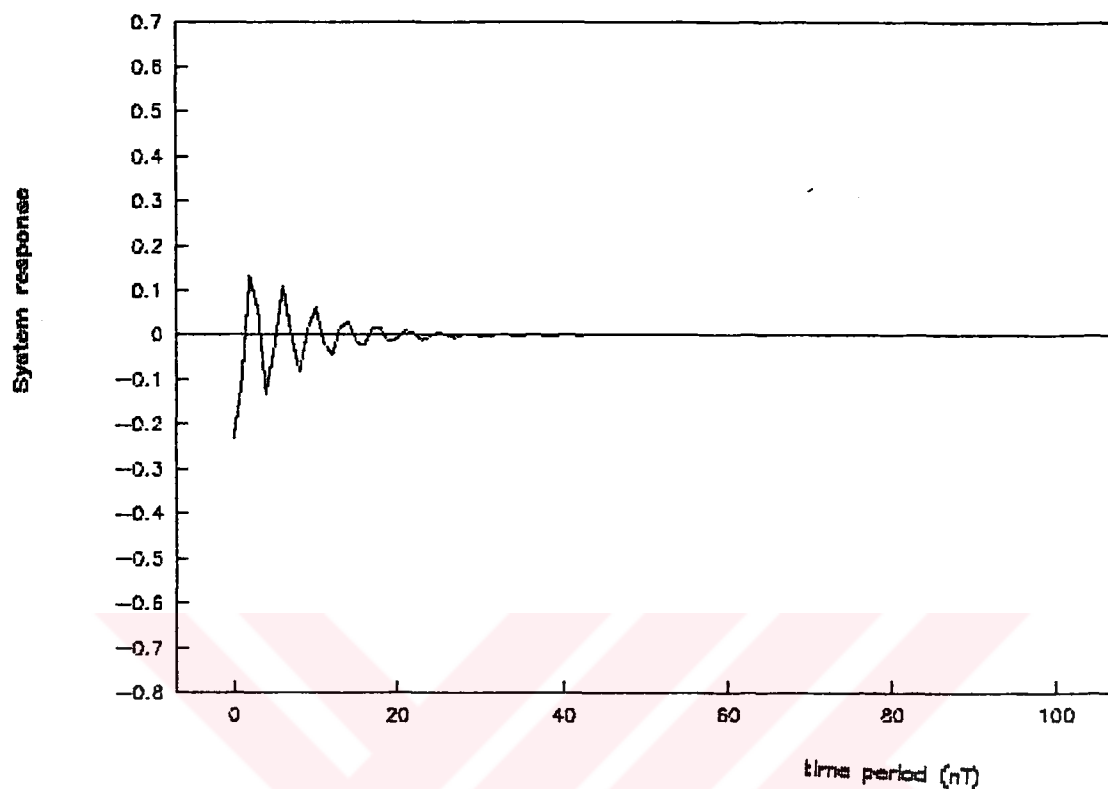
Figure 5.21. Impulse response of ARMA MYWE transfer function for the test case 2
