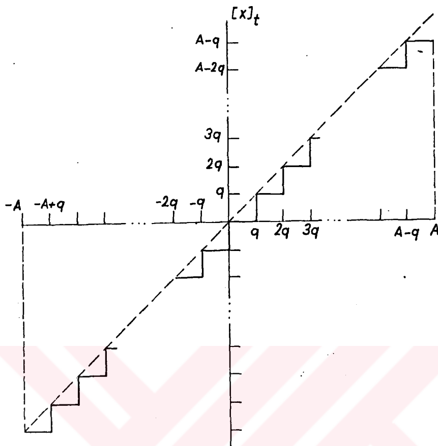
Figure 4.1.1. Truncation of two's complement numbers
