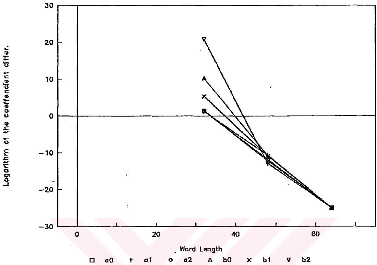
Figure 5.15 Real transfer function : Logarithm of coefficient errors according to the change of word length
