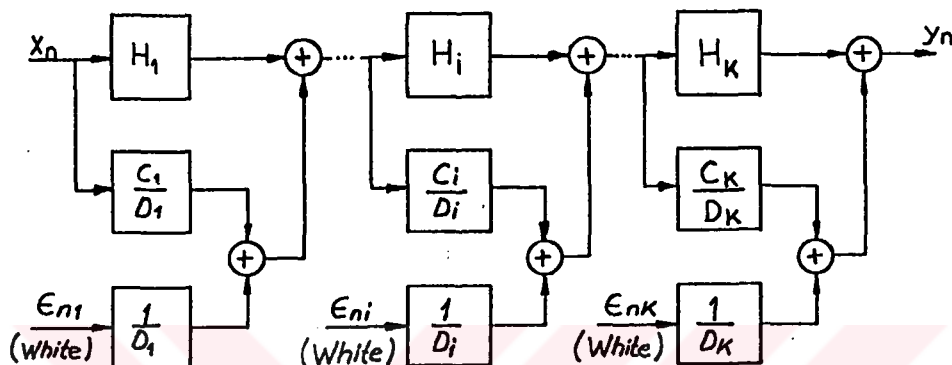
Figure 4.3.4. Round-off error accumulation for cascade form
