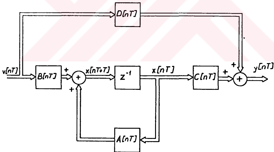
Figure 3.6.1. Pictorial representation of the state and output equations for a uniformly sampled, linear, discrete-time systems
