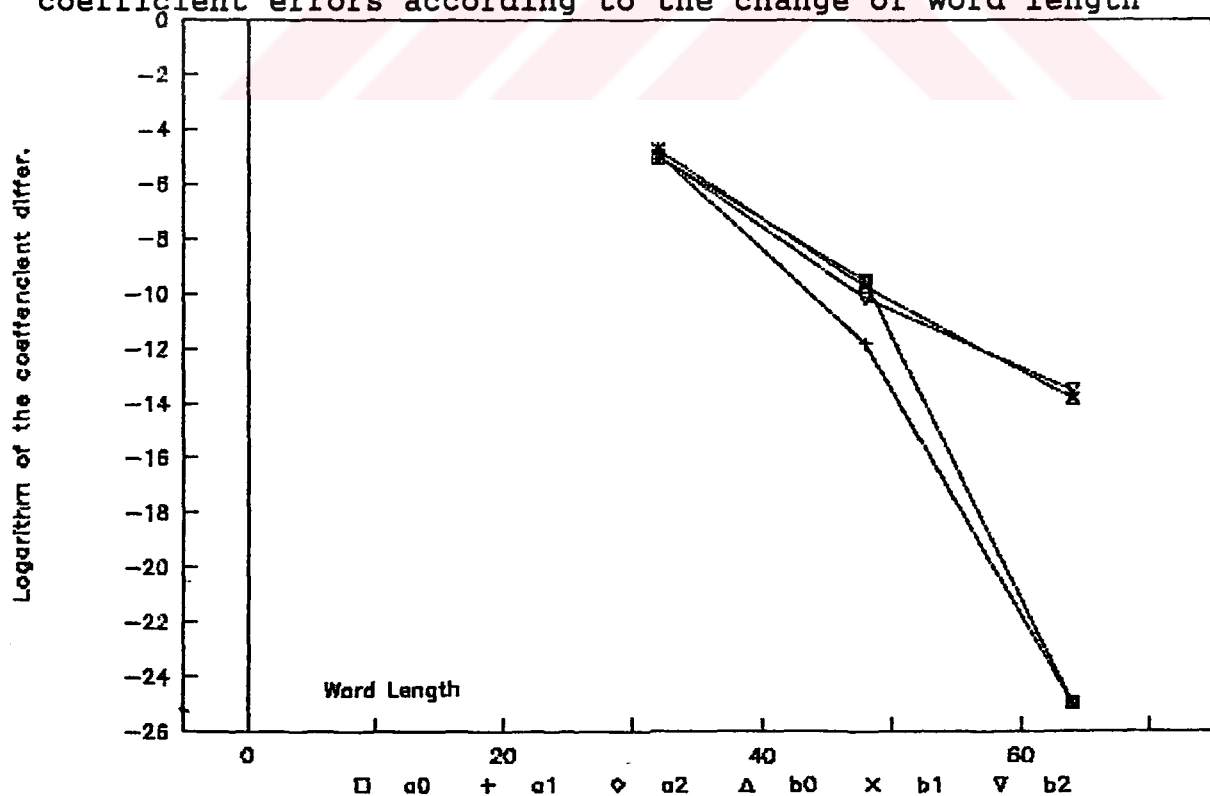
Figure 5.18 ARMA AKAIKE transfer function : Logarithm of coefficient errors according to the change of word length
