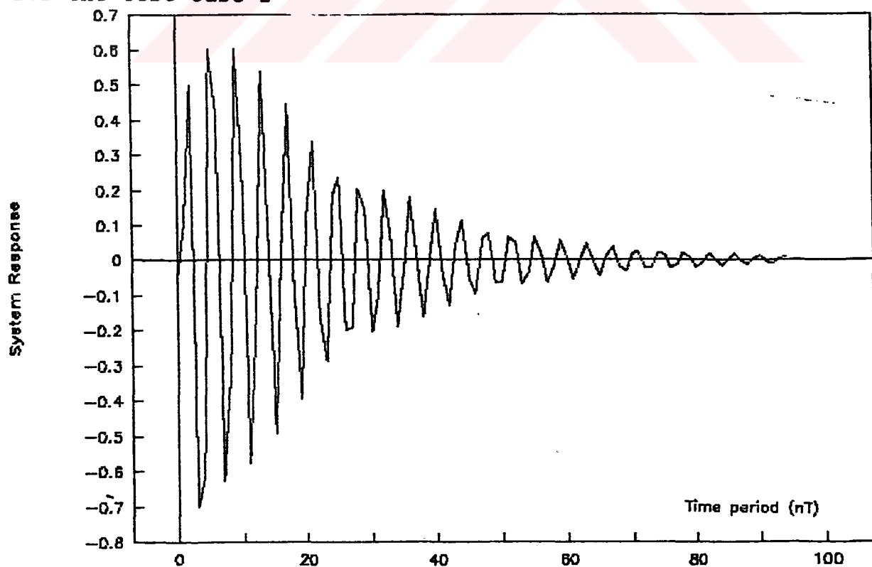
Figure 5.22 Impulse response of ARMA AKAIKE transfer function for the test case 2
