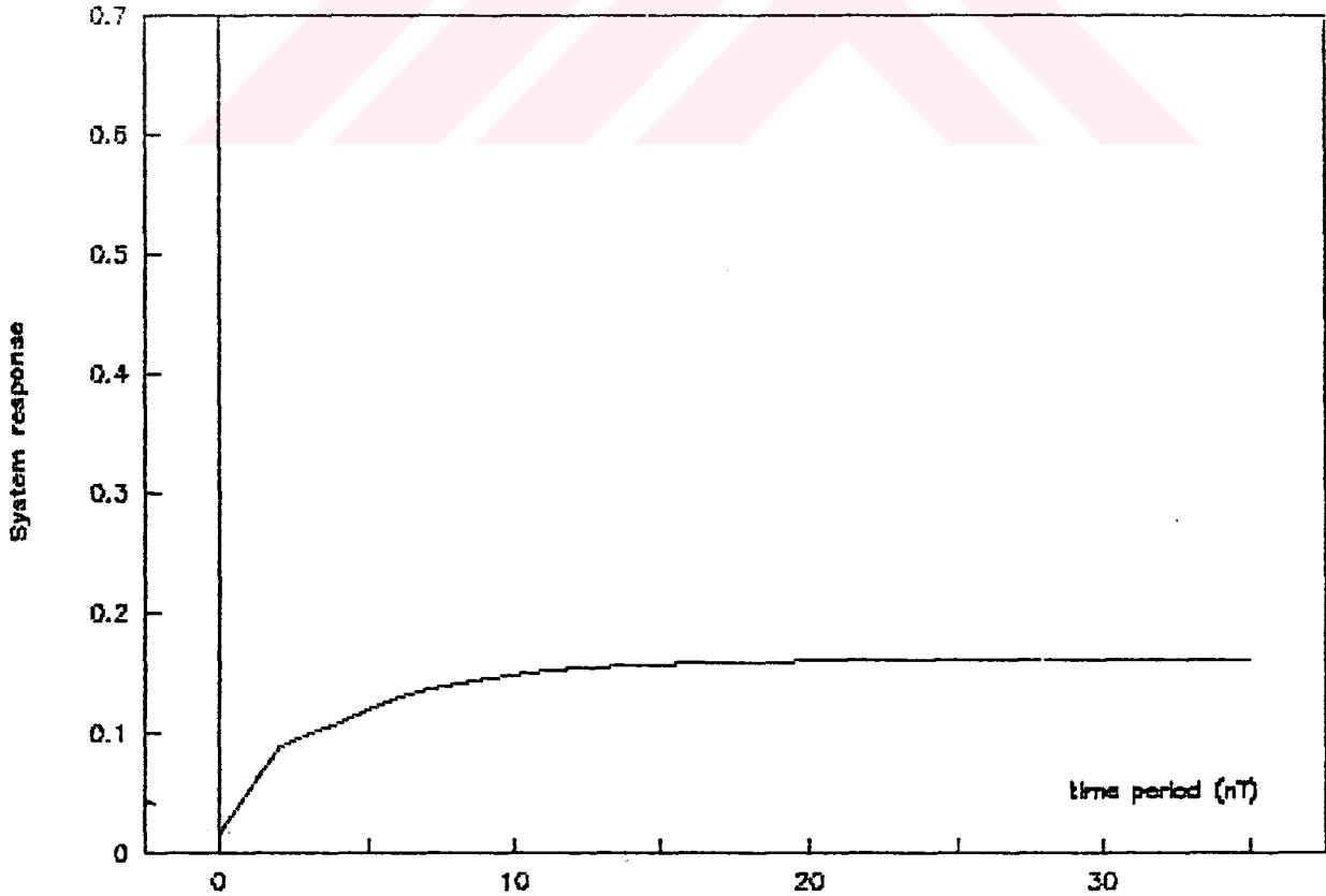
Figure 5.8. Step response of ARMA AKAIKE transfer function for the first test case
