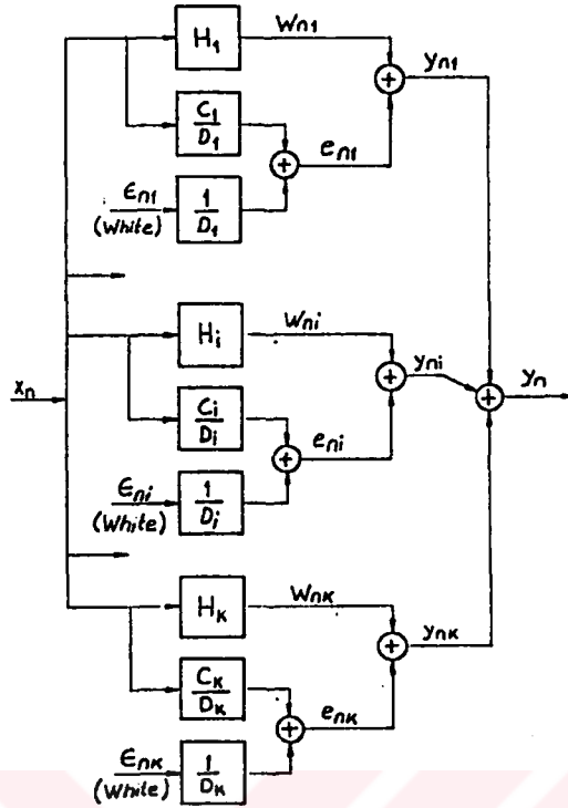
Figure 4.3.3. Round-off error accumulation for parallel form
