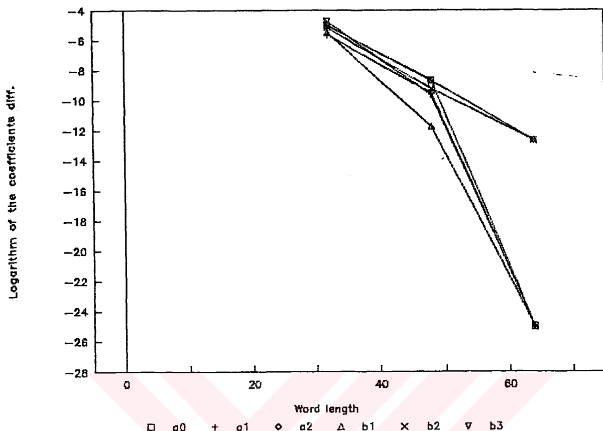
Figure 5.32. ARMA AKAIKE transfer function : Logarithm of coefficient errors according to the change of word length
