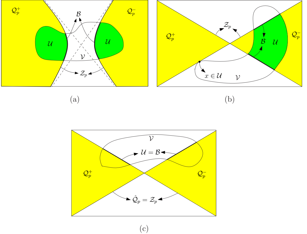
Figure B.3. An illustration of Lemma 7.3.4 for \pi(P) = 1 and two components under the condition \mathcal{U} \not\subseteq \mathcal{Q}_p^+ , \mathcal{U} \not\subseteq \mathcal{Q}_p^- : (a) for an inequality constraint, \mathcal{U} does not have a supporting halfspace at a point of \mathcal{B} , (b) for an inequality constraint, it has a single supporting halfspace; (c) for an equality constraint, it has two supporting halfspaces
