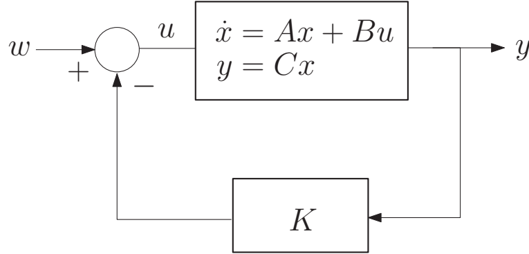
Figure 2.4. An LTI system subject to static linear output feedback
