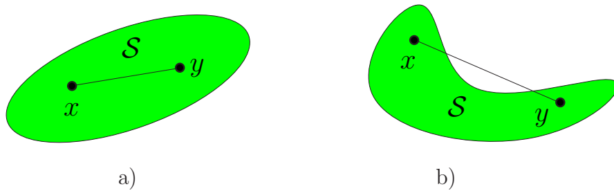
Figure 3.1. a) Convex set; b) nonconvex set
