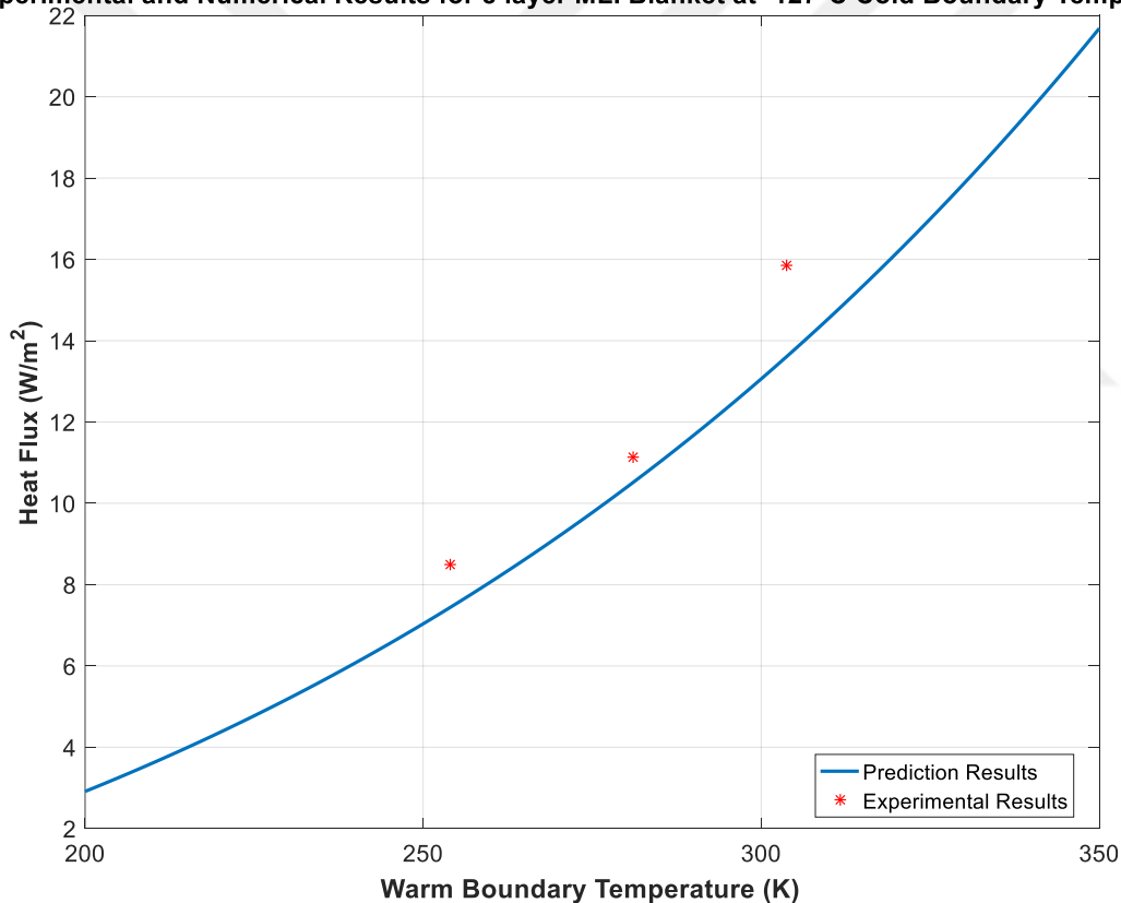
Figure 5.11: Experimental and Numerical Results for 8 layer MLI Blanket at -127°C Cold Boundary Temperature
