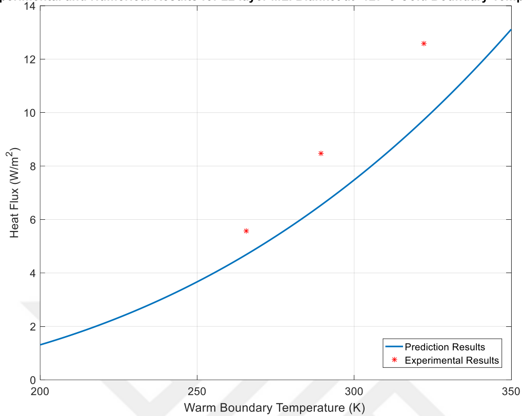
Figure 5.8: Experimental and Numerical Results for 22 layer MLI Blanket at -127°C Cold Boundary Temperature
