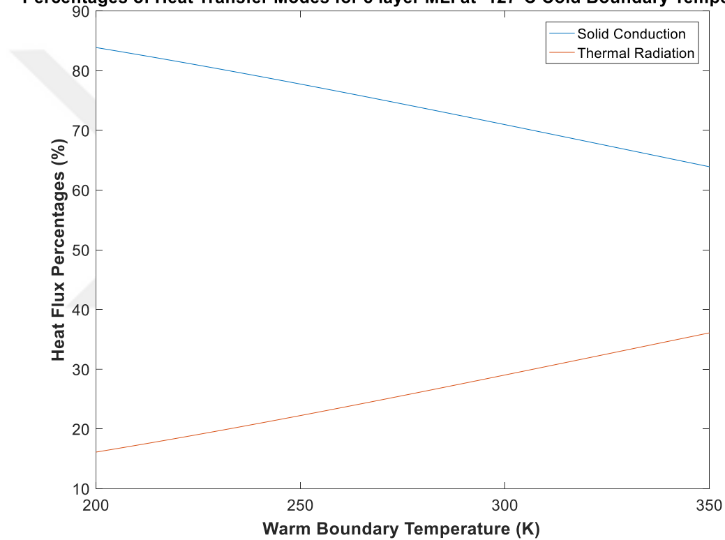
Percentages of Heat Transfer Modes for 8 layer MLI at -127°C Cold Boundary Temperature
