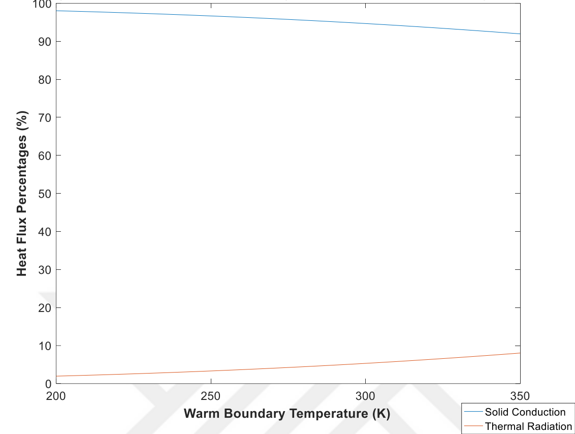
Percentages of Heat Transfer Modes for 22 layer MLI at -127°C Cold Boundary Temperature
