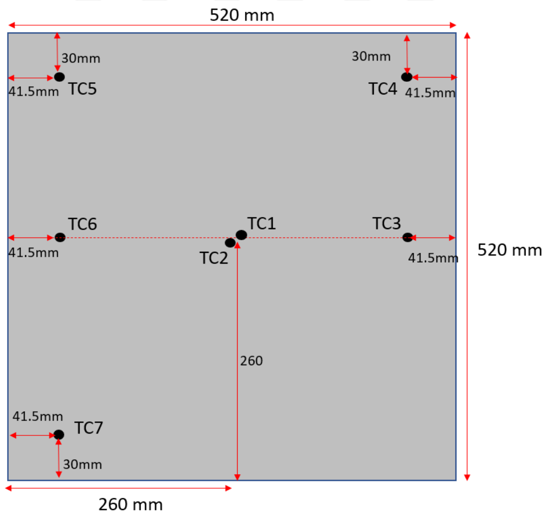
Figure 4.4: Thermocouple Layout
