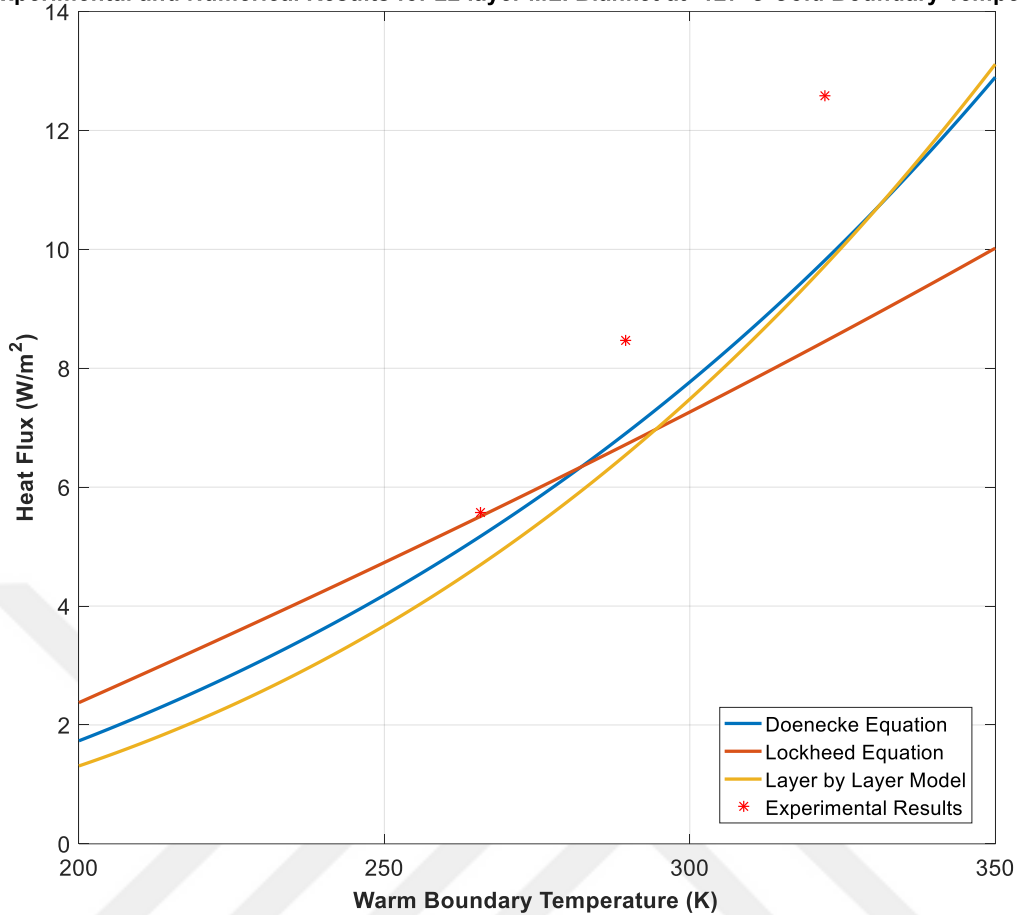
Experimental and Numerical Results for 22 layer MLI Blanket at -127°C Cold Boundary Temperature
