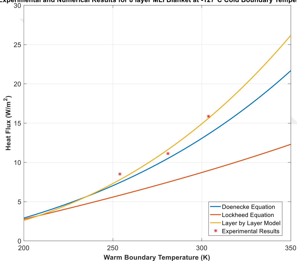
Experimental and Numerical Results for 8 layer MLI Blanket at -127°C Cold Boundary Temperature
