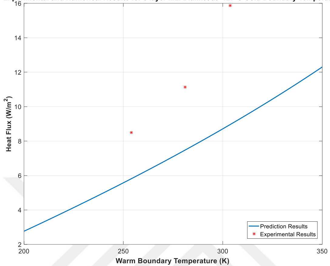
Figure 5.19: Experimental and Numerical Results for 8 layer MLI Blanket at -127°C Cold Boundary Temperature
