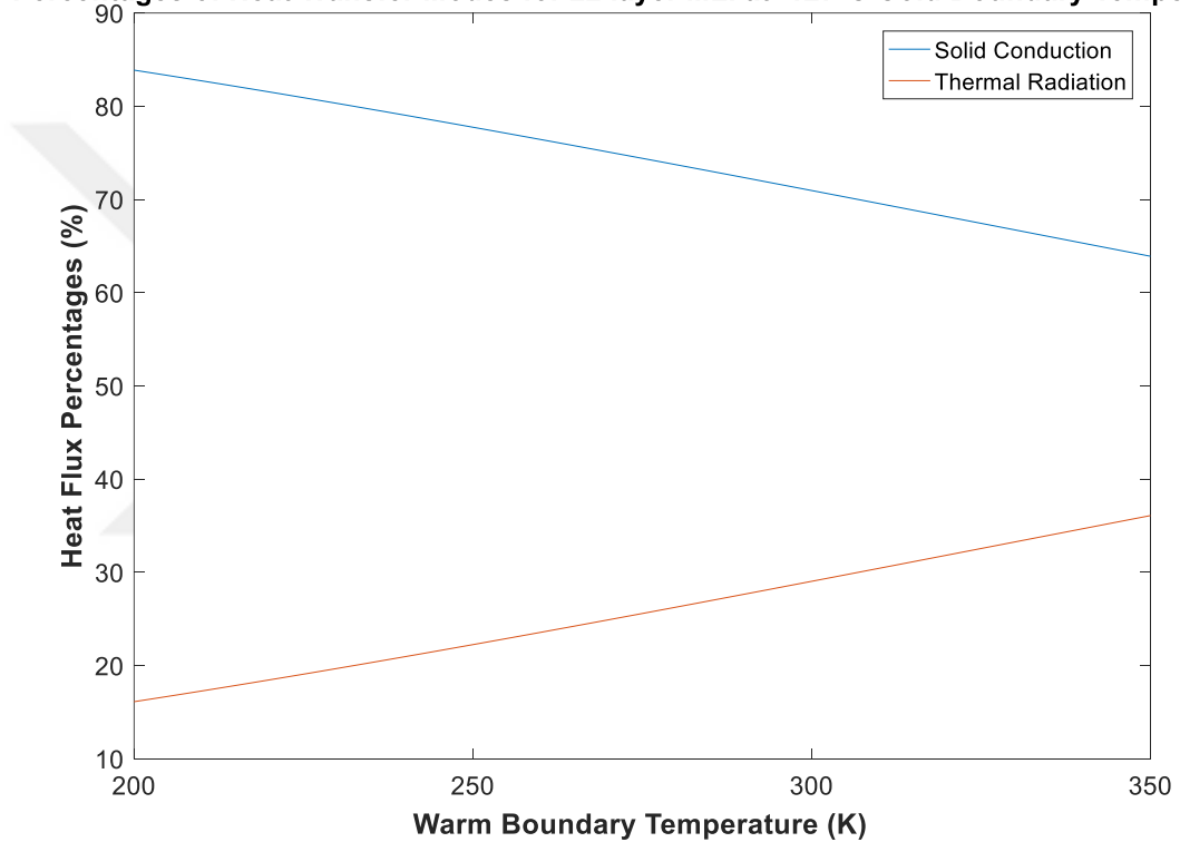
Figure 5.14: Heat Transfer Mode Participation Percentages for 22 layer MLI blanket at -127°C
