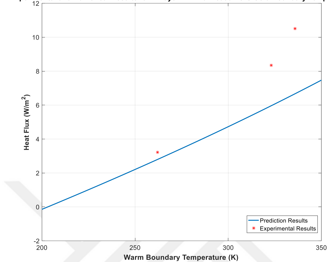
Figure 5.25: Experimental and Numerical Results for 22 layer MLI Blanket at -75°C Cold Boundary Temperature
