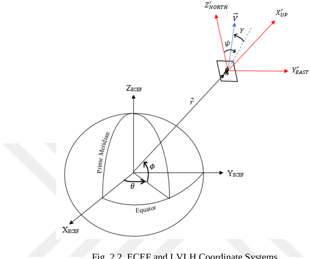
Fig. 2.2 ECEF and LVLH Coordinate Systems
