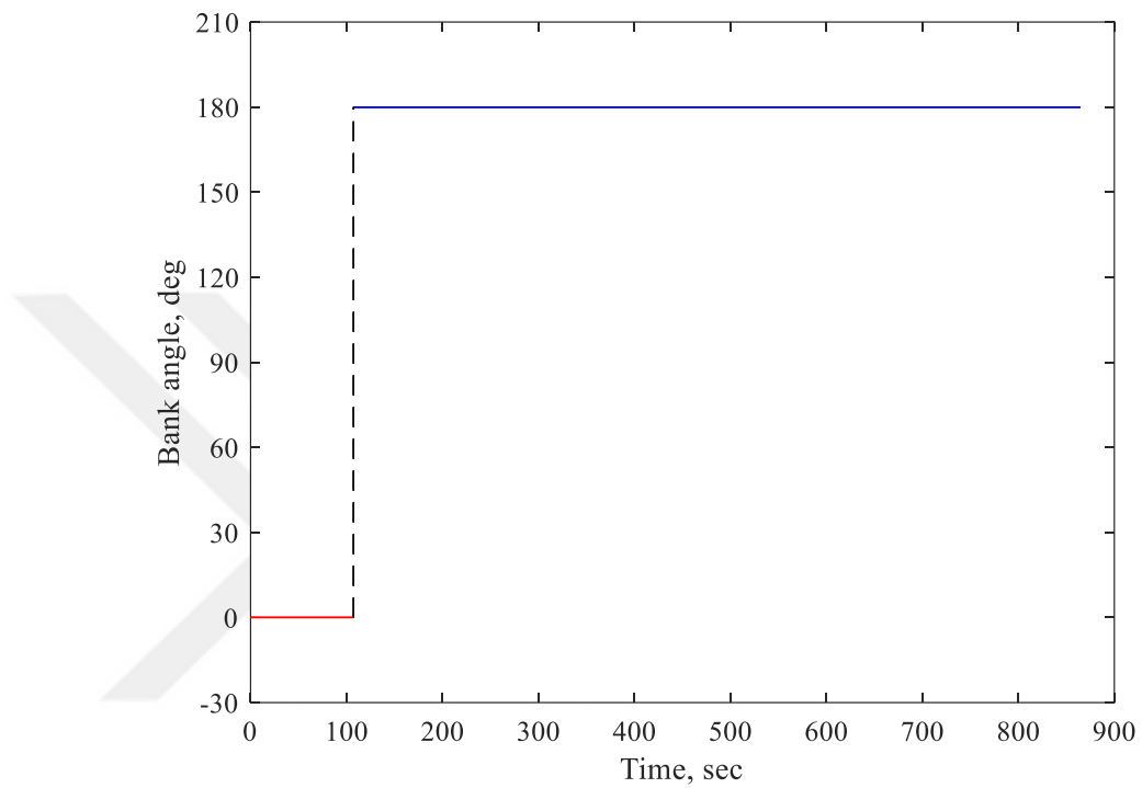
Fig. 3.1 Bank Angle vs. Time for Optimal Bang-Bang Control Problem
