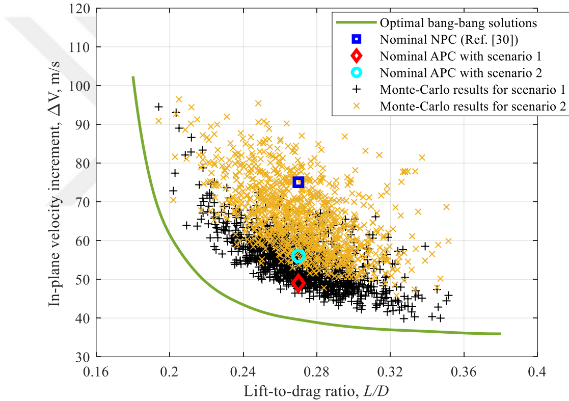
Fig. 5.28 Aerocapture In-plane Maneuver \Delta V vs. Lift-to-Drag Ratio
