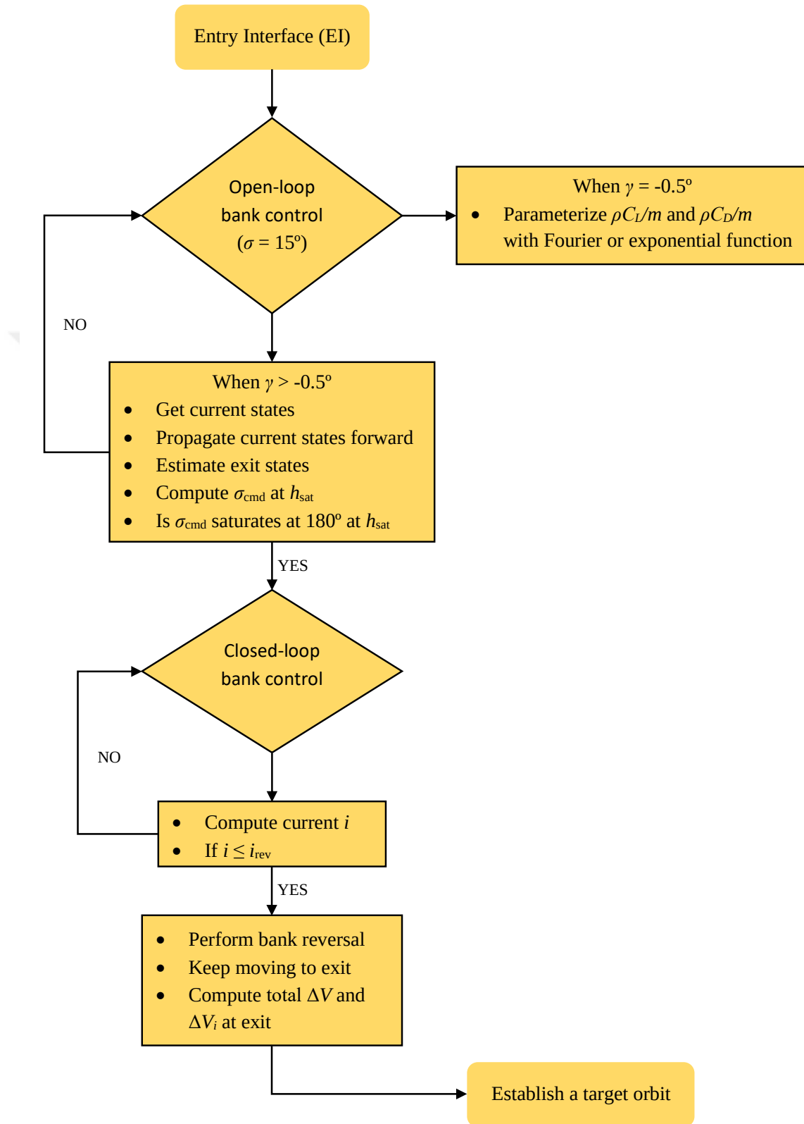
Fig. 4.8 Schematic Flowchart of Analytical Aerocapture Guidance
