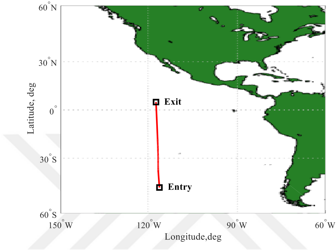
Fig. 5.7 Ground Track of Atmospheric Flight Phase for Scenario 1 on a Mercator Map
