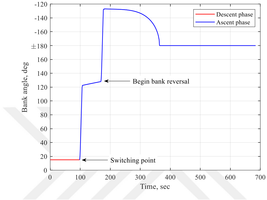
Fig. 5.6 Nominal Bank Angle Time History for Scenario 1
