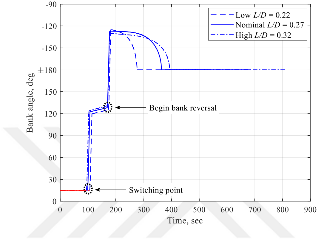
Fig. 4.6 Bank Angle Time History for Three Sample L/D Ratios
