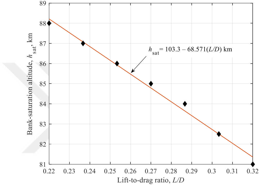
Fig. 4.4 Linear Least-Square Fitting for h_{\text{sat}}
