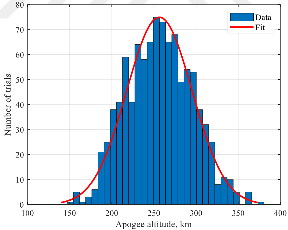
Fig. 5.25 Histogram of Apogee Altitude from 1000 Trails for Scenario 2
