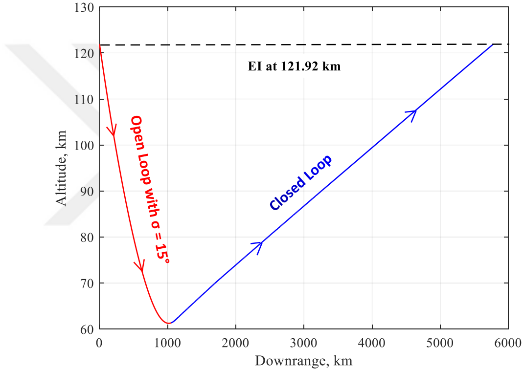
Fig. 4.1 Nominal Aerocapture Trajectory
