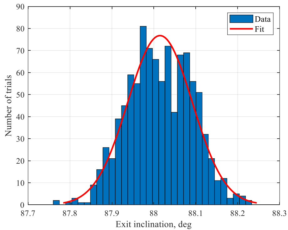
Fig. 5.14 Histogram of Exit Inclination from 1000 Trails for Scenario 1
