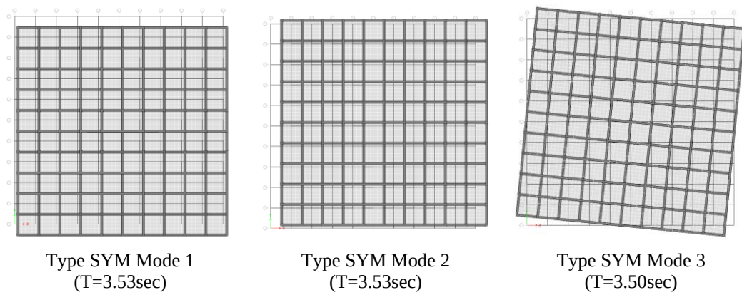
Figure 3.11. Mode shapes of SYM model set (Plan view of 8 th story)
