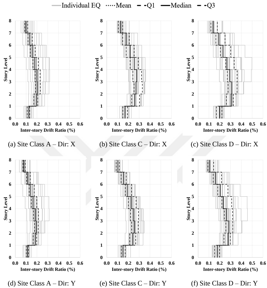
Figure A.8. IDR profiles for building case “U3”
