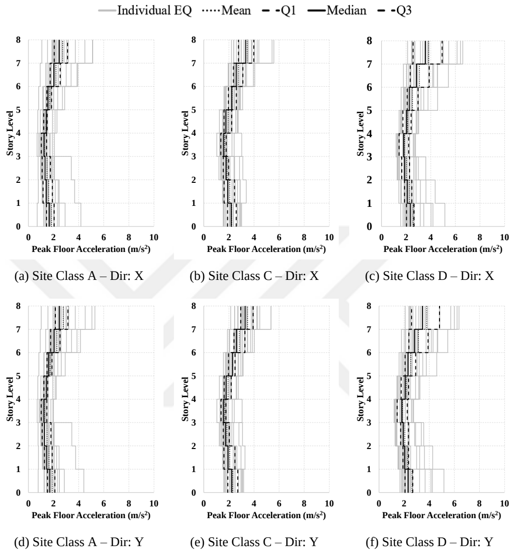
Figure A.21. PFA profiles for building case “U2”
