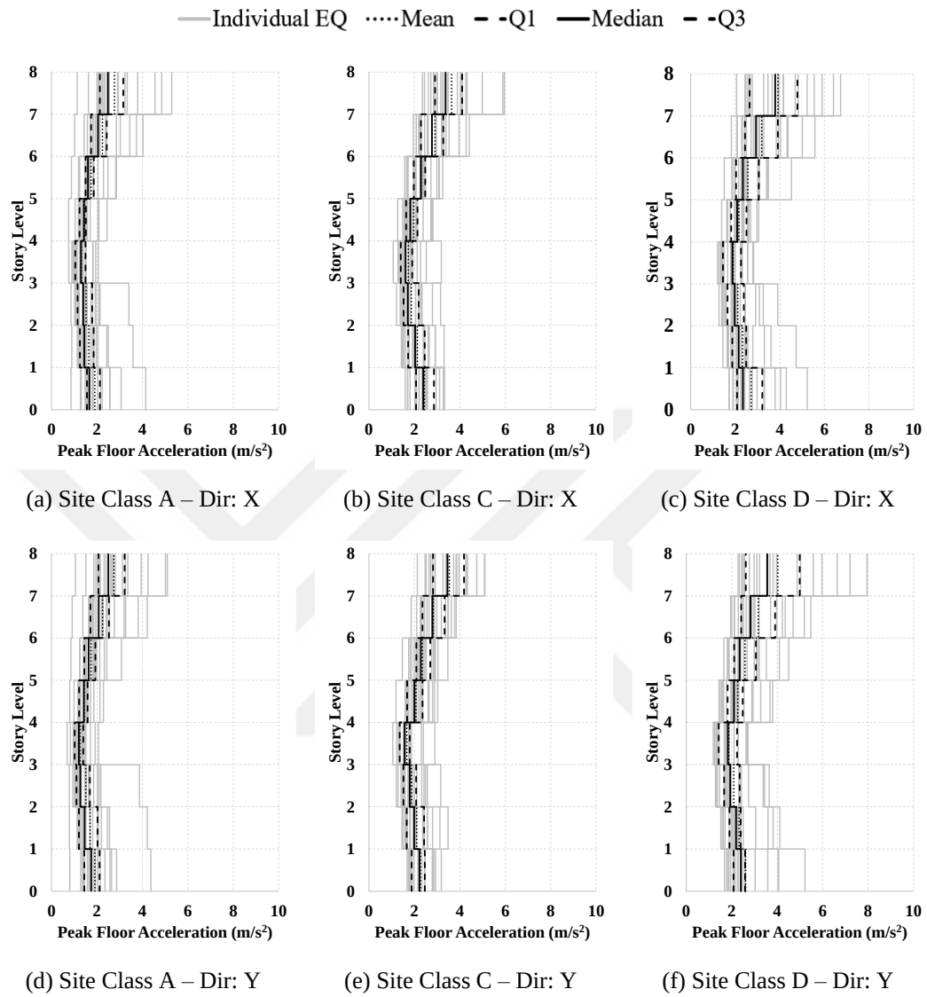
Figure A.23. PFA profiles for building case “U4”
