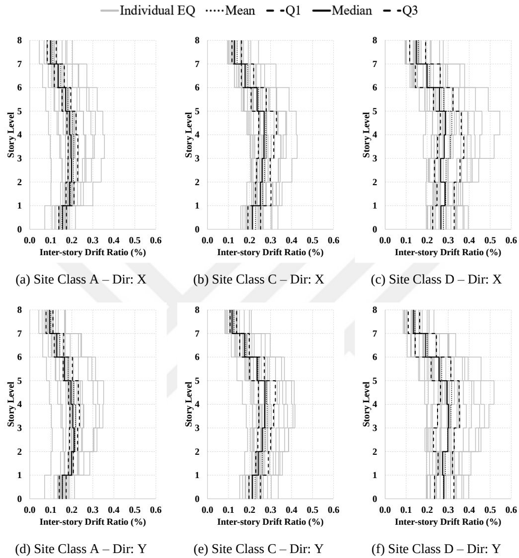
Figure A.4. IDR profiles for building case “T3”
