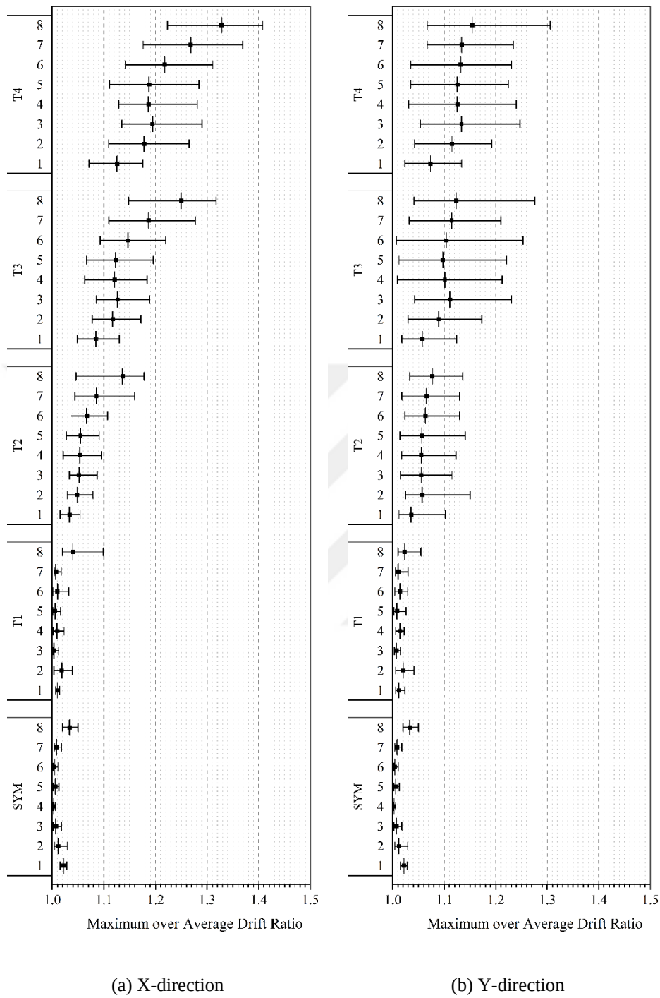
Figure 5.4. Variation of maximum drift to average drift ratios for T-shaped models (Site Class D)
