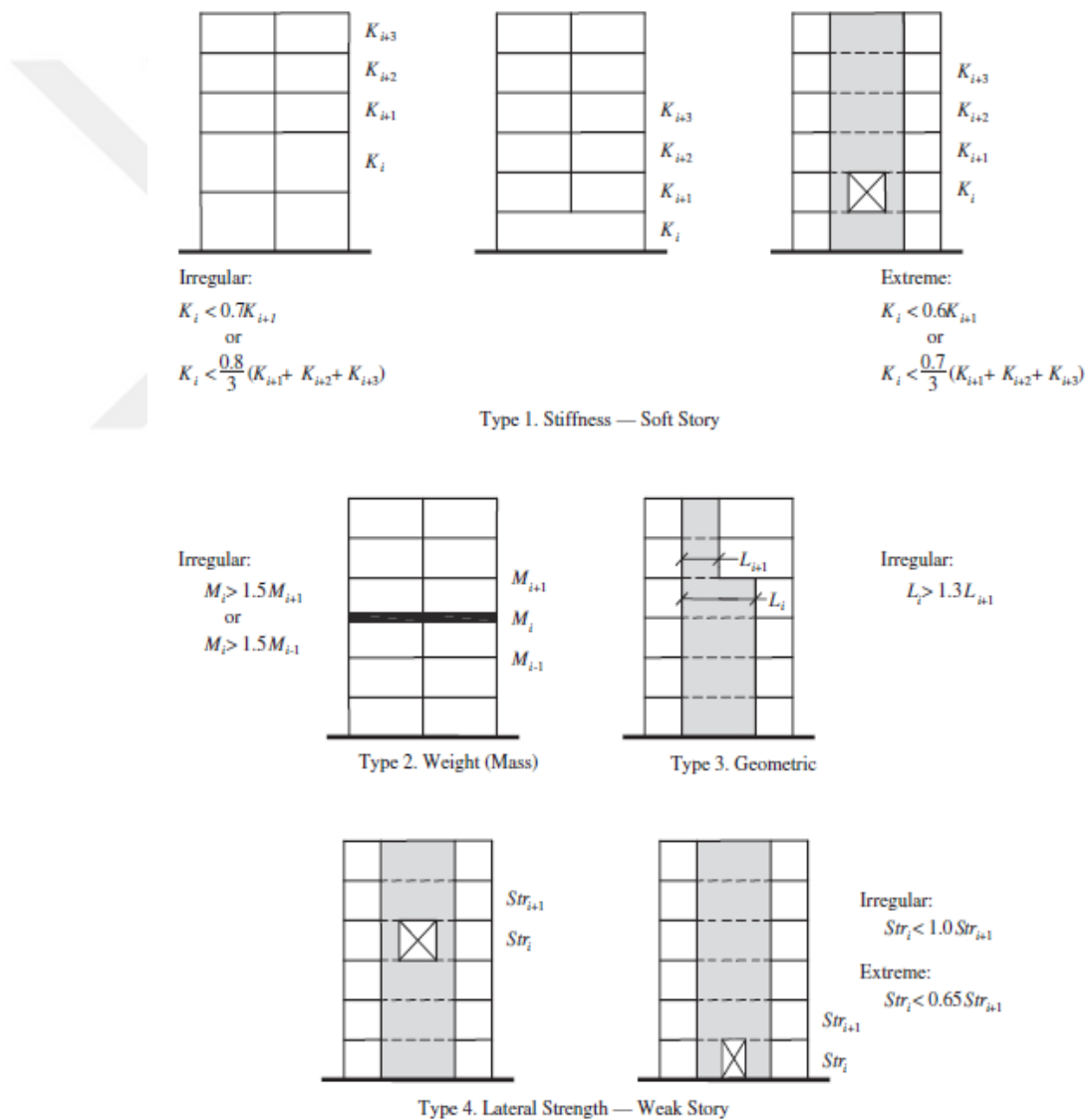
Figure 1.5. Vertical Irregularity in ASCE/SEI 7.22 C12.3-2
