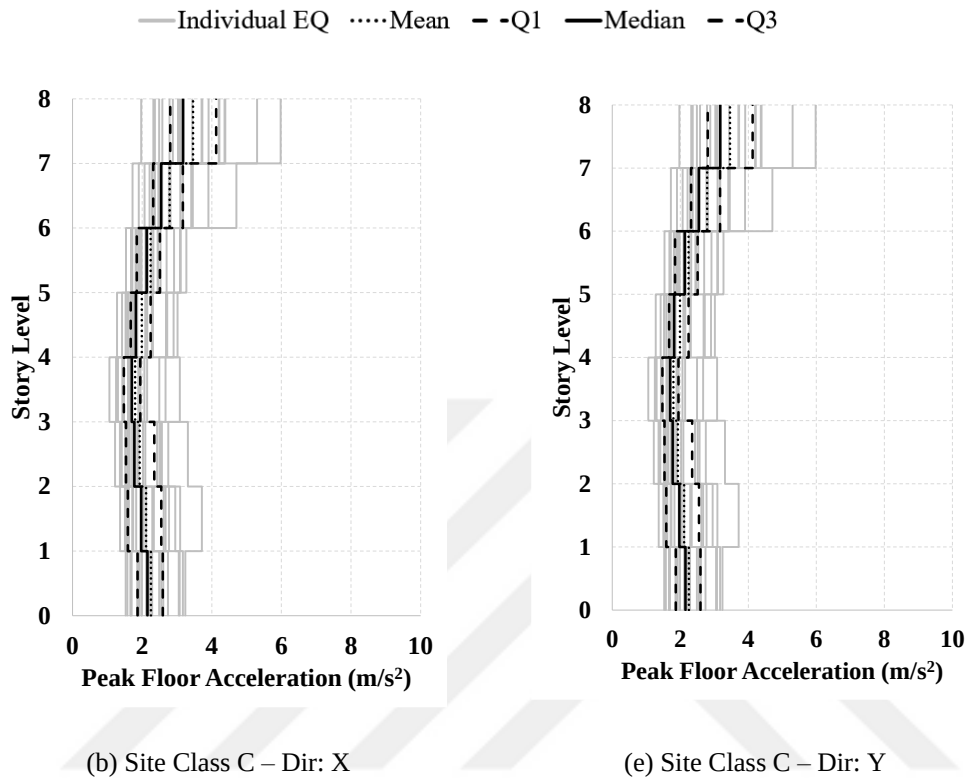
Figure 4.11. PFA profiles for building case “Symmetric” Site Class C
