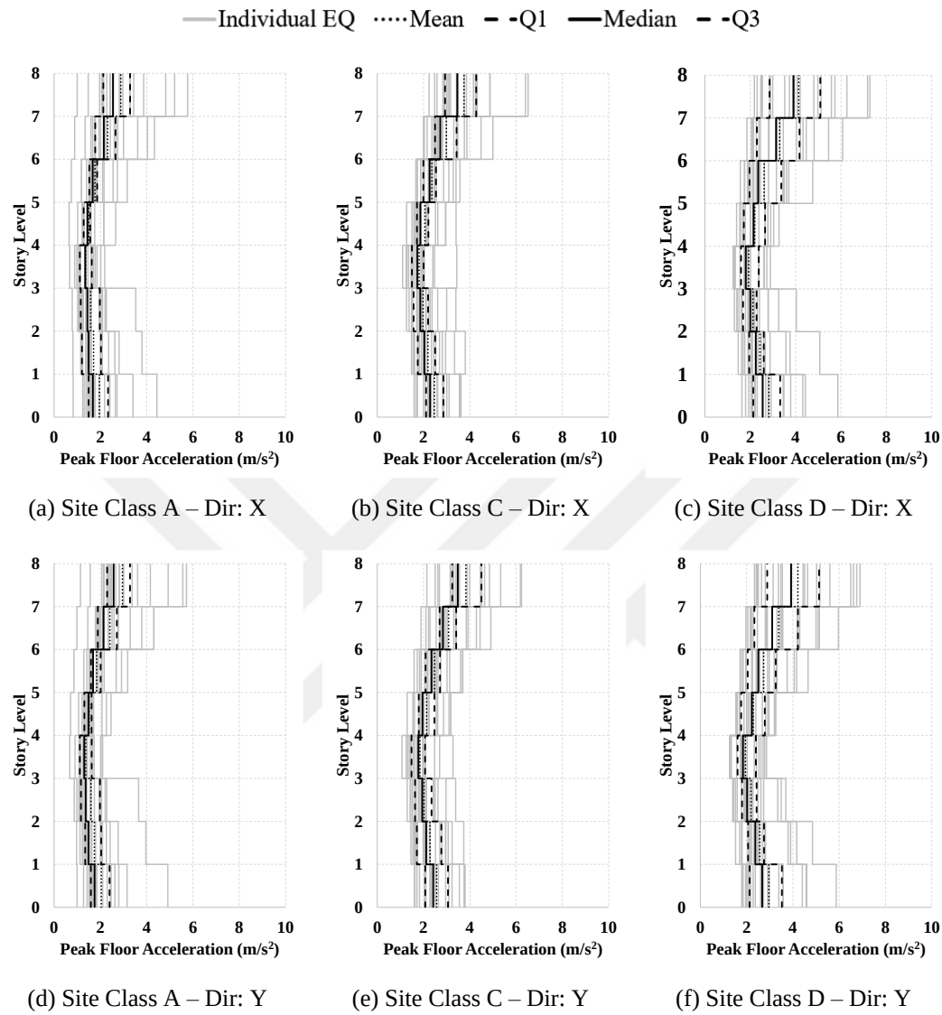
Figure A.18. PFA profiles for building case “T3”
