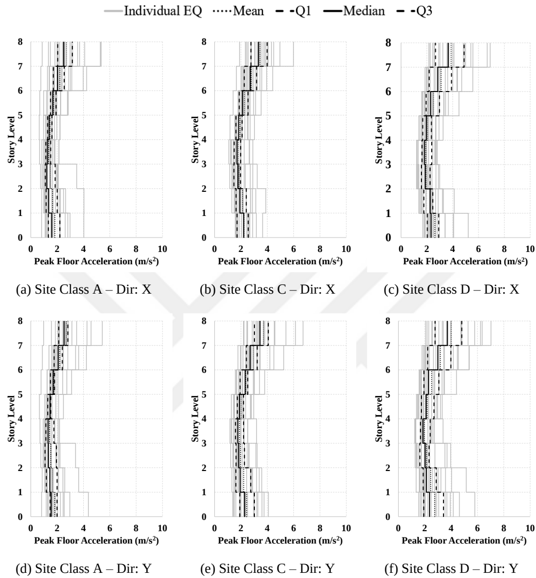
Figure A.16. PFA profiles for building case “T1”
