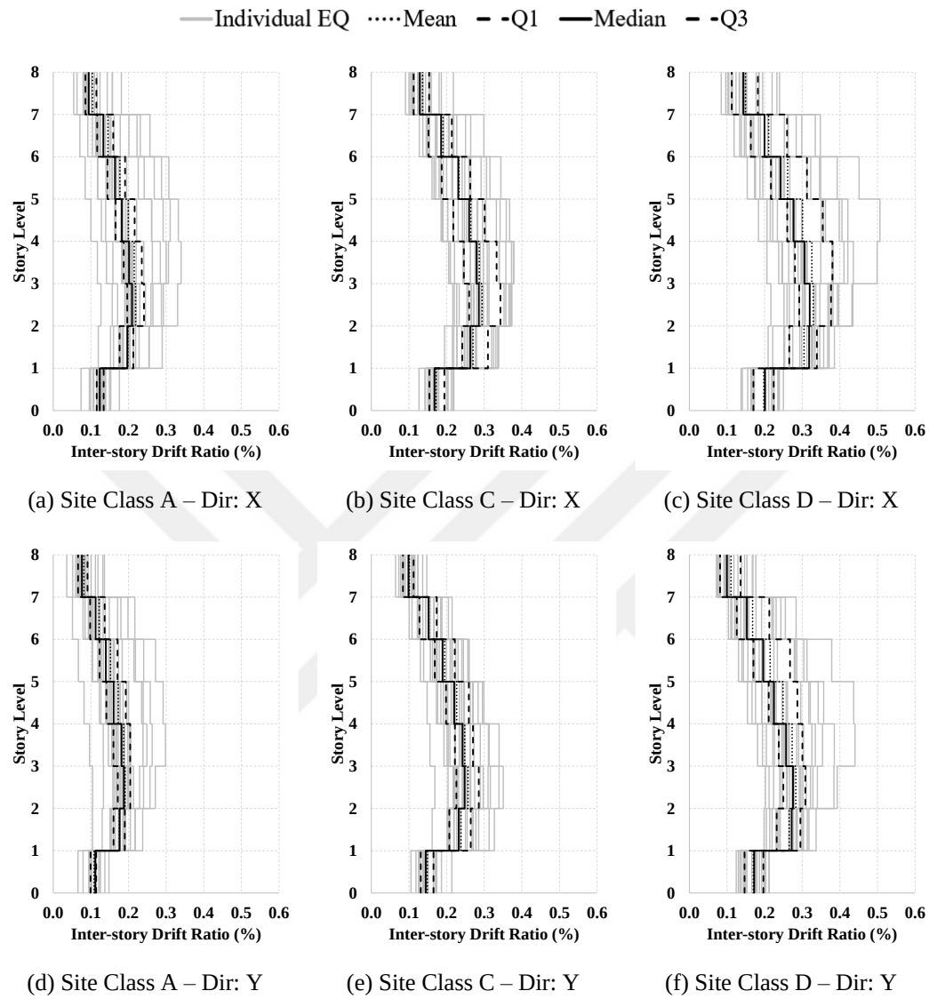
Figure A.14. IDR profiles for building case “U4 Group 5”
