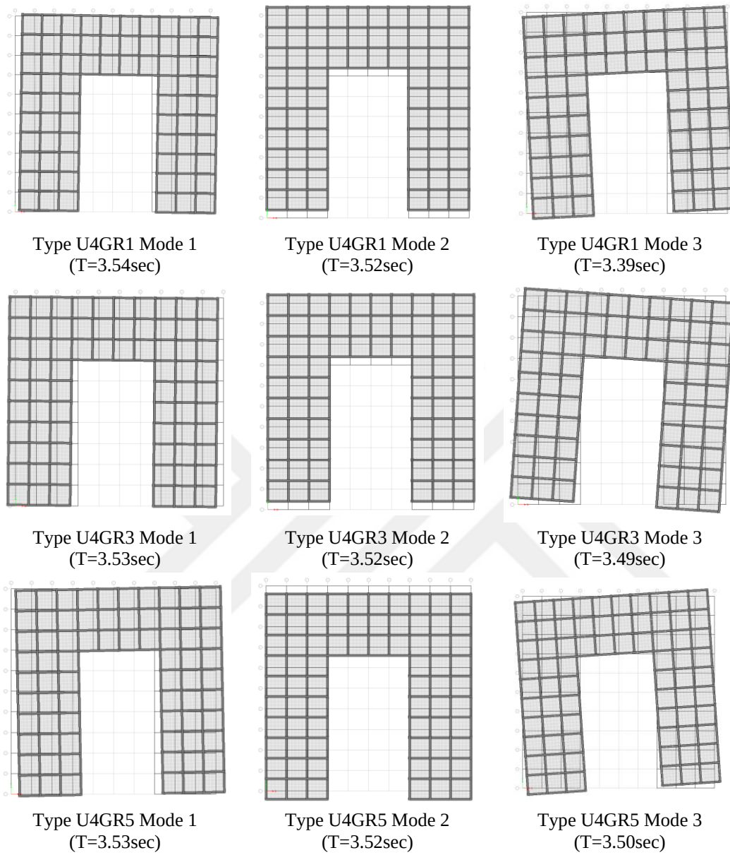
Figure 3.13. Mode shapes of isolator group effect model set (Plan view of 8 th story)
