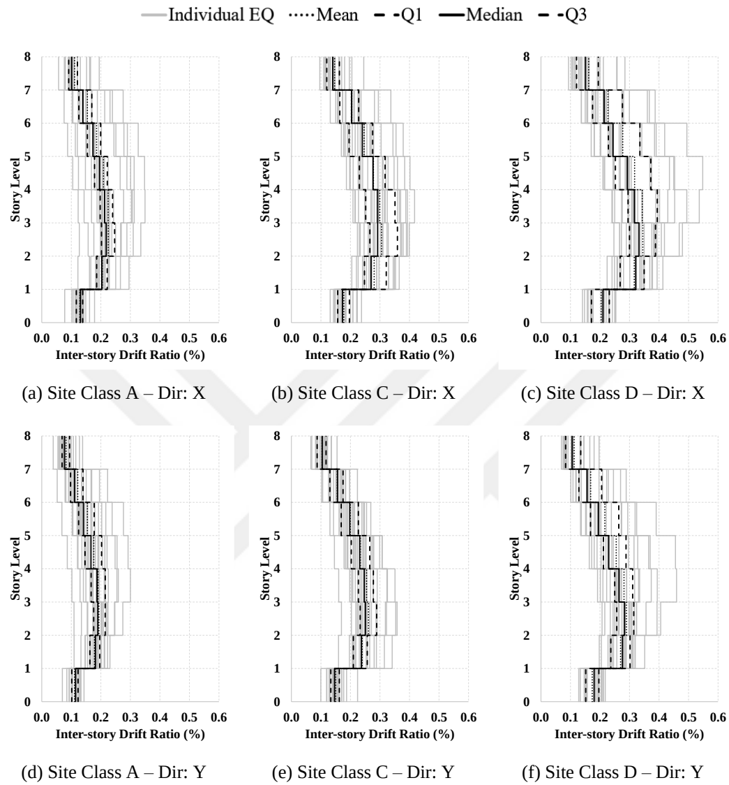
Figure A.12. IDR profiles for building case “U4 Mass”
