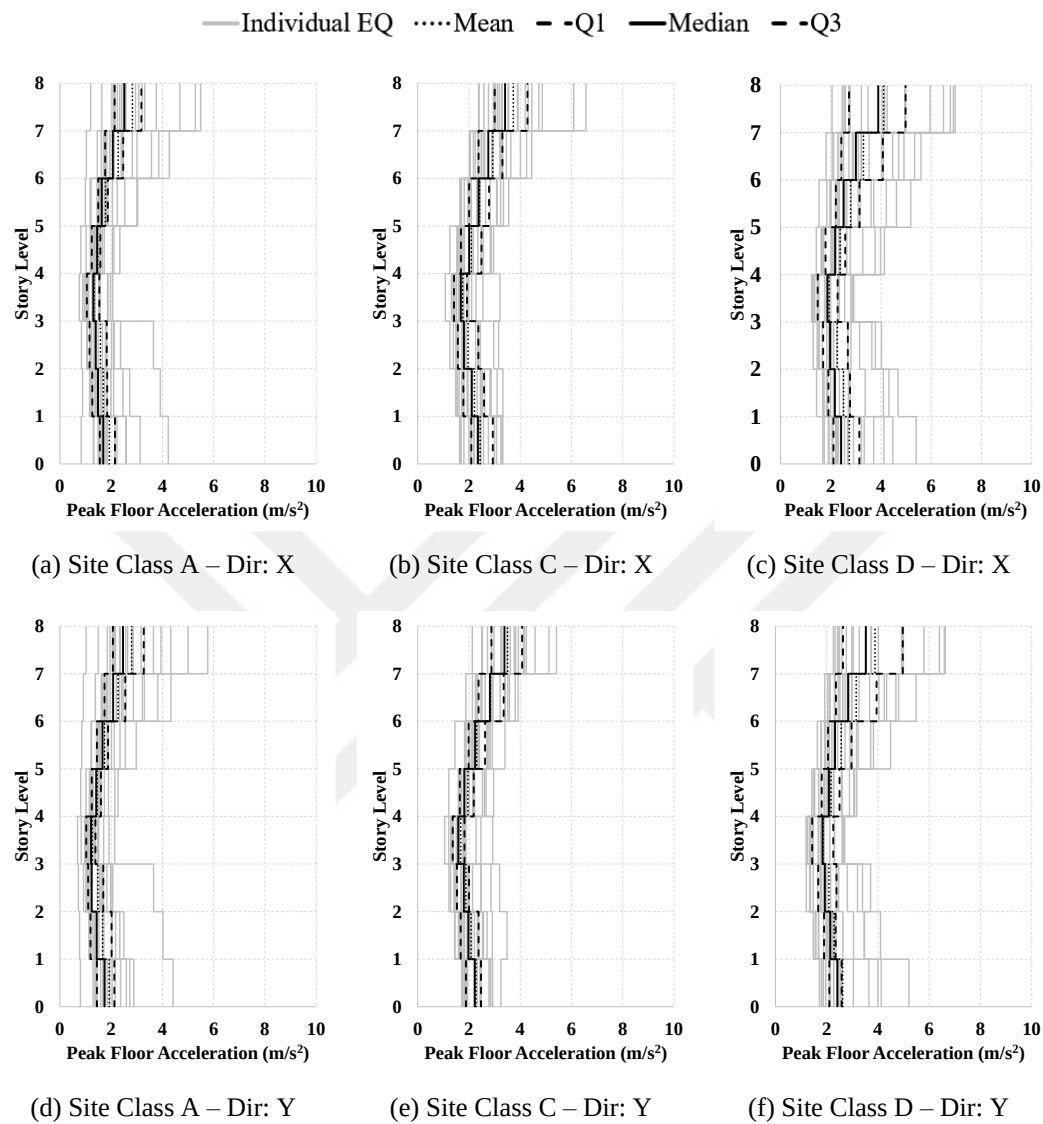
Figure A.28. PFA profiles for building case “U4 Group 5”
