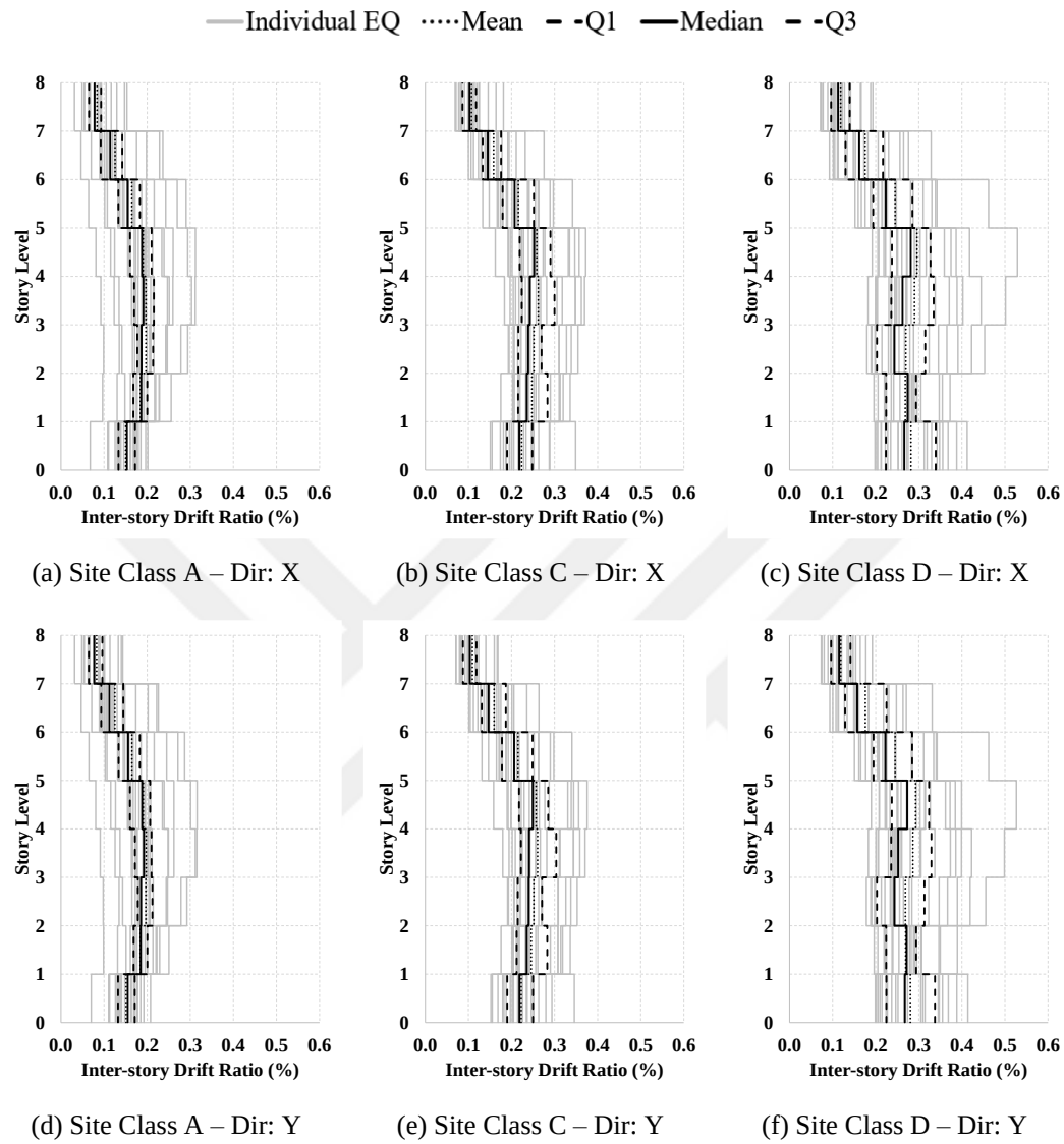
Figure A.10. IDR profiles for building case “Symmetric Mass”
