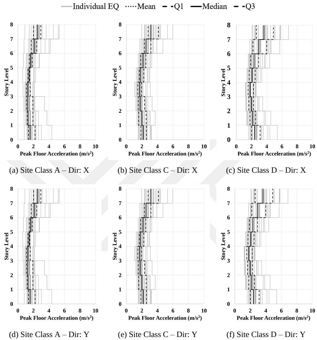
Figure A.15. PFA profiles for building case “Symmetric”
