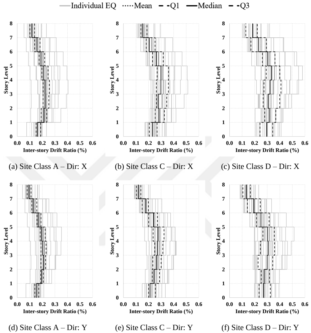
Figure A.5. IDR profiles for building case “T4”
