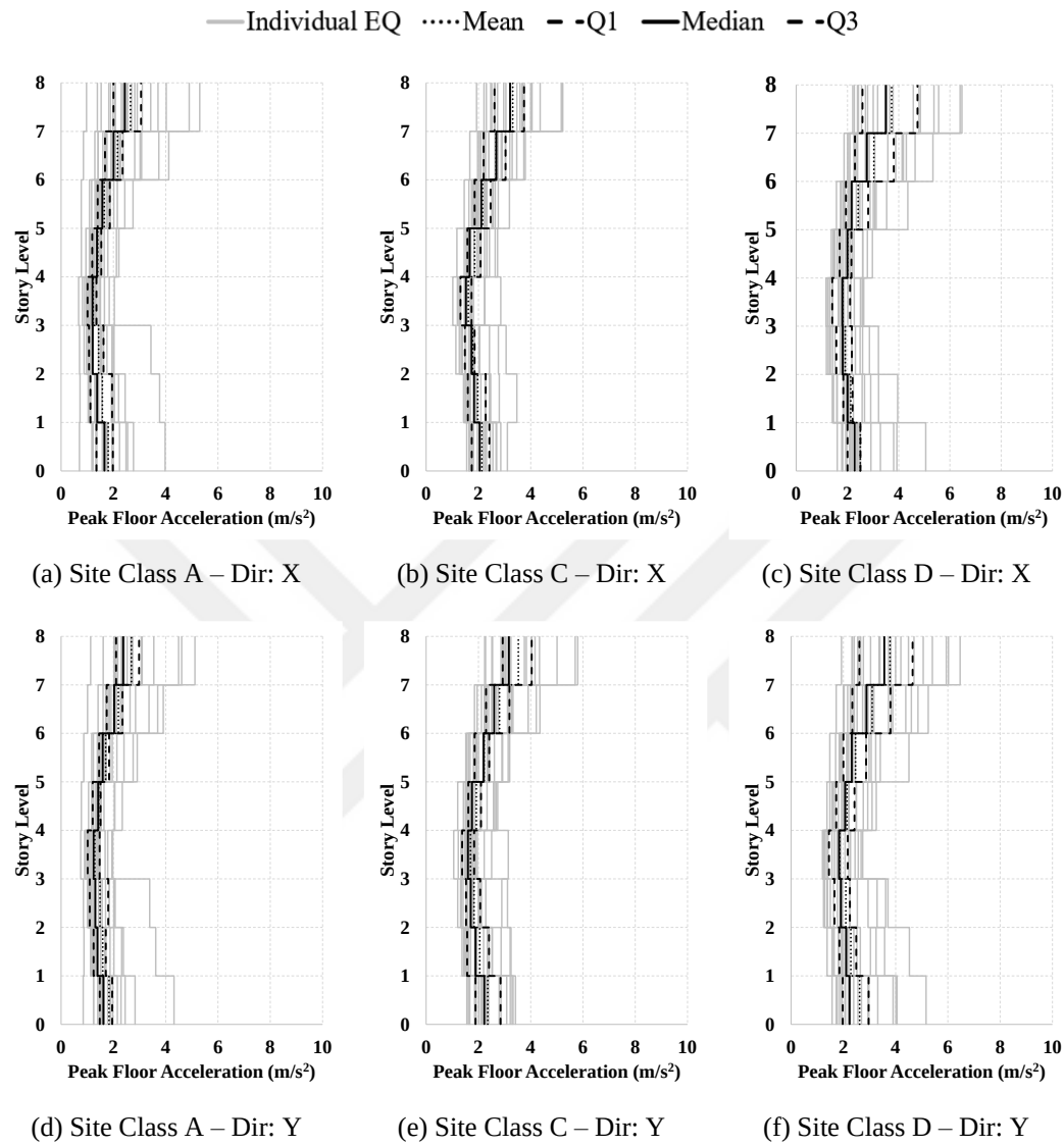
Figure A.20. PFA profiles for building case “U1”
