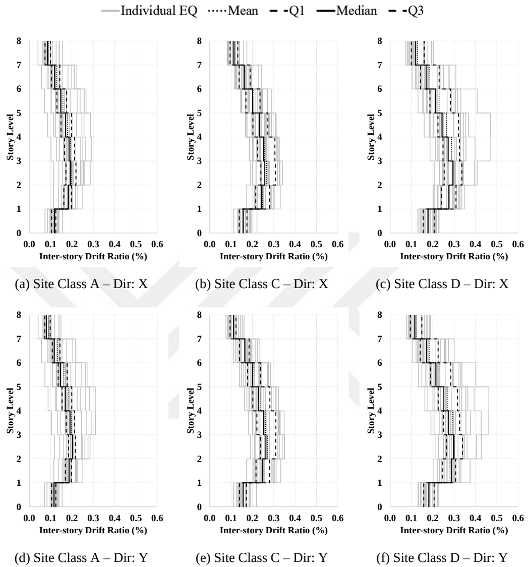
Figure A.7. IDR profiles for building case “U2”
