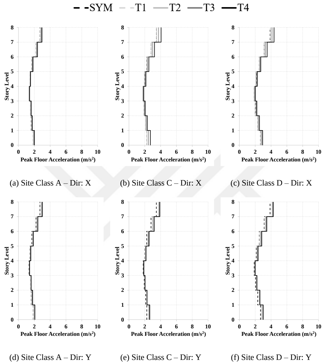
Figure 5.5. Comparison of PFA profiles for T-shaped models
