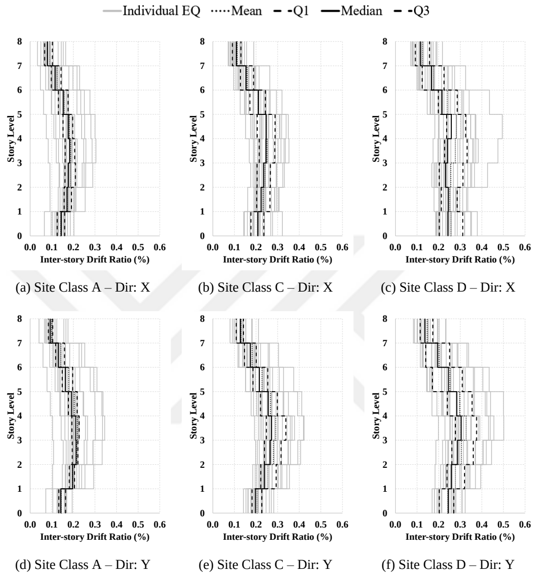
Figure A.3. IDR profiles for building case “T2”
