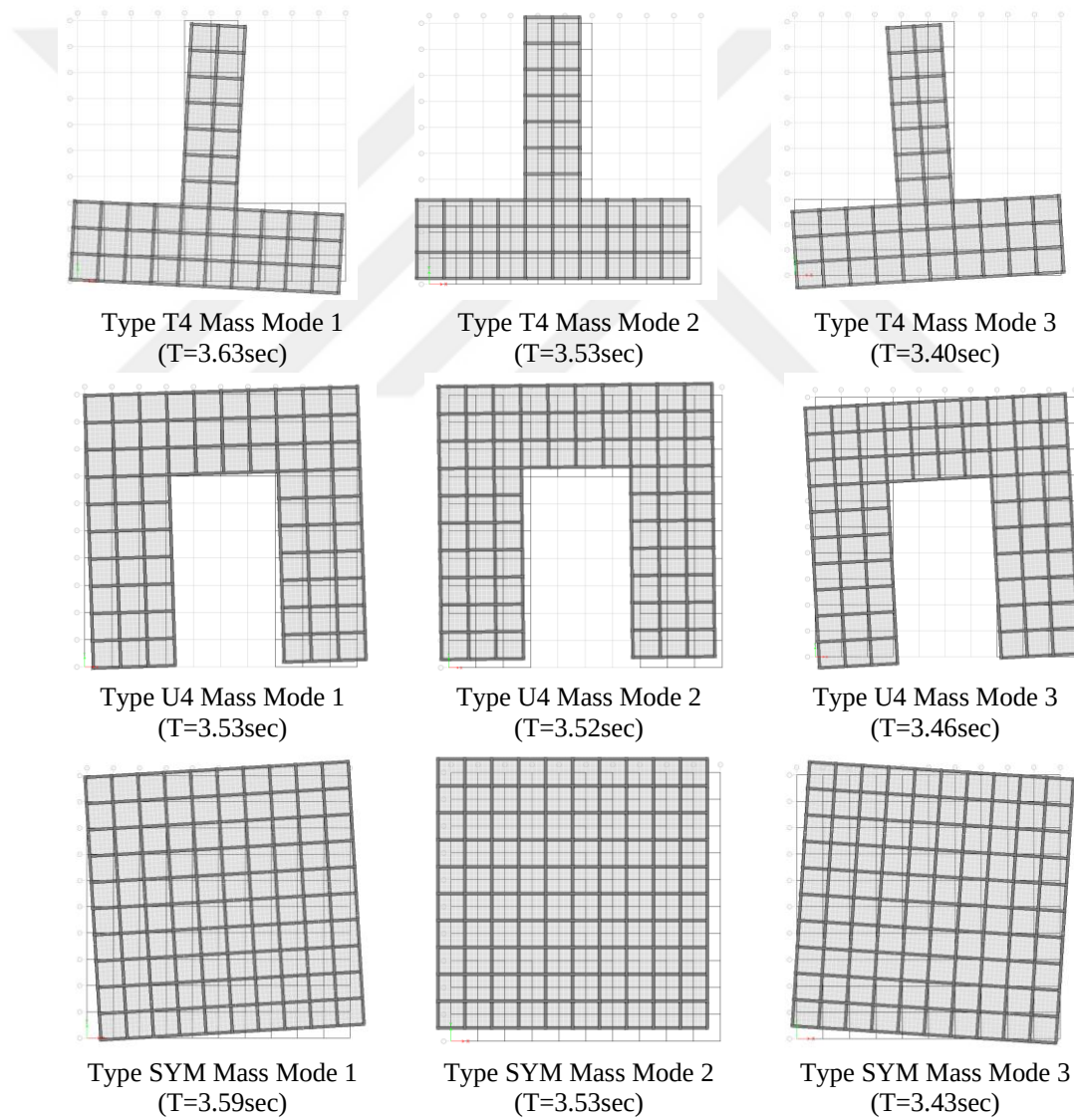
Figure 3.12. Mode shapes of mass concentrated model set (Plan view of 8 th story)
