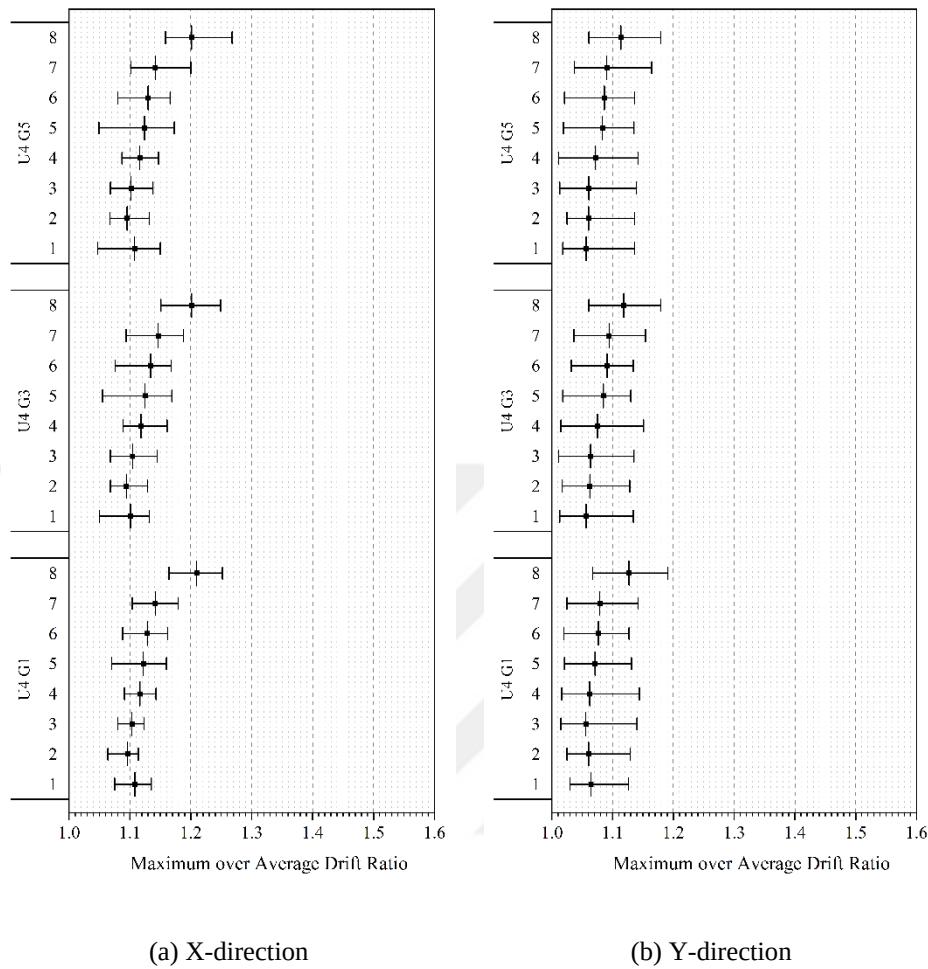
Figure 5.28. Variation of CM maximum drift to average drift ratios for U4 – Group 1, 3 and 5 models (Site Class C)
