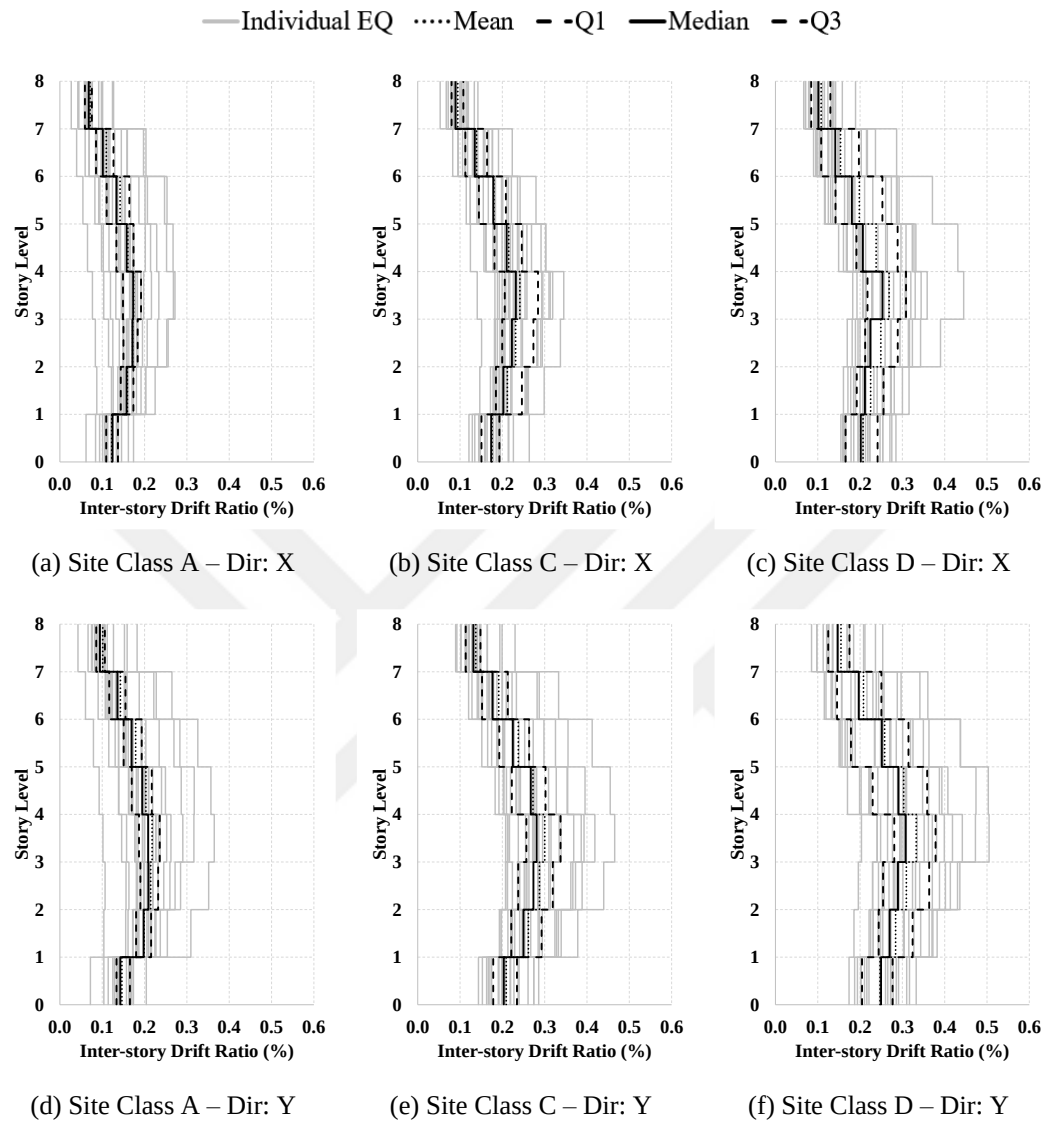
Figure A.2. IDR profiles for building case “T1”
