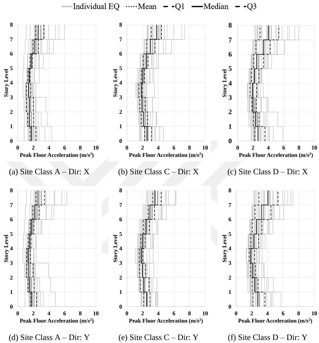
Figure A.19. PFA profiles for building case “T4”
