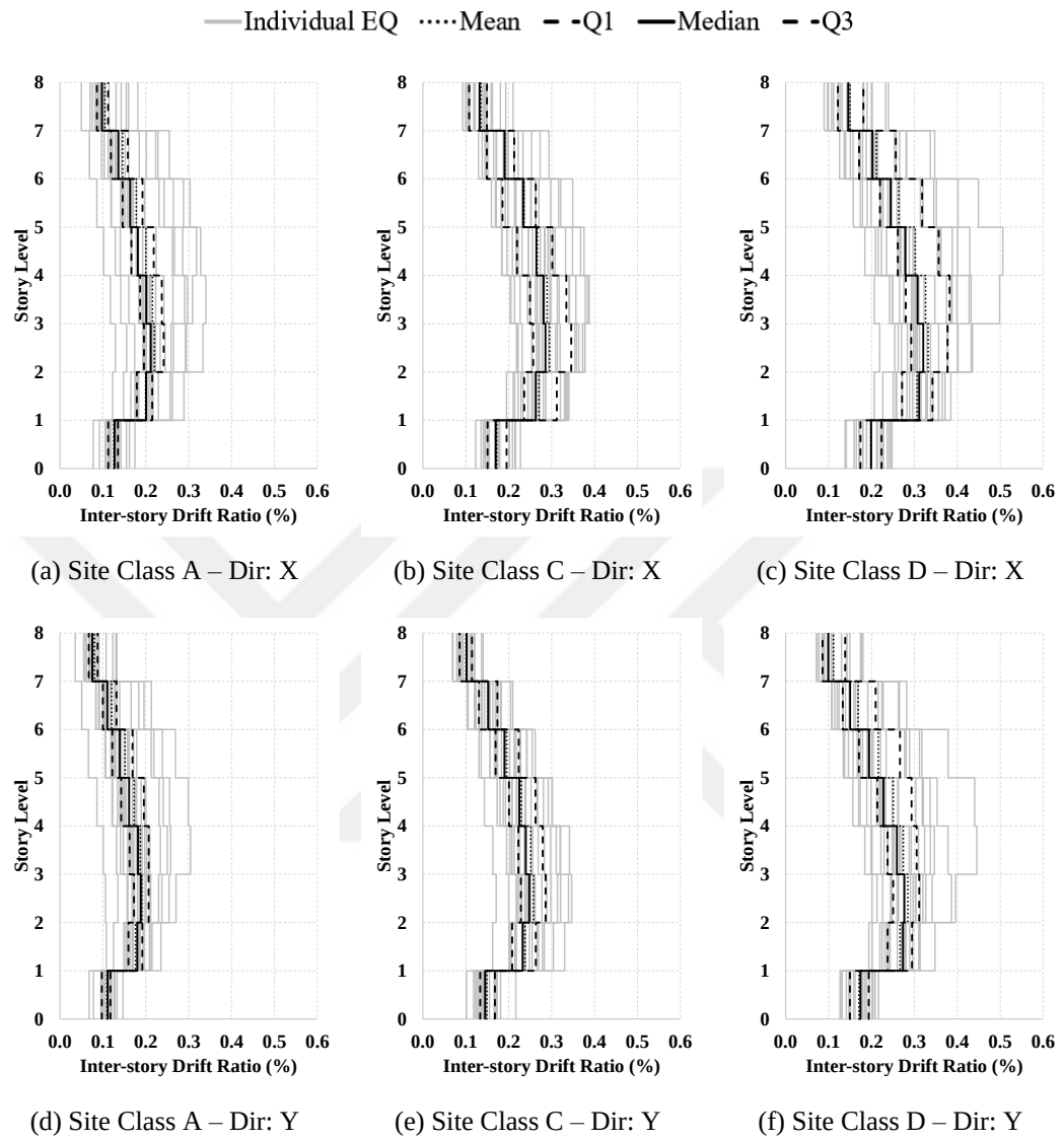
Figure A.9. IDR profiles for building case “U4”
