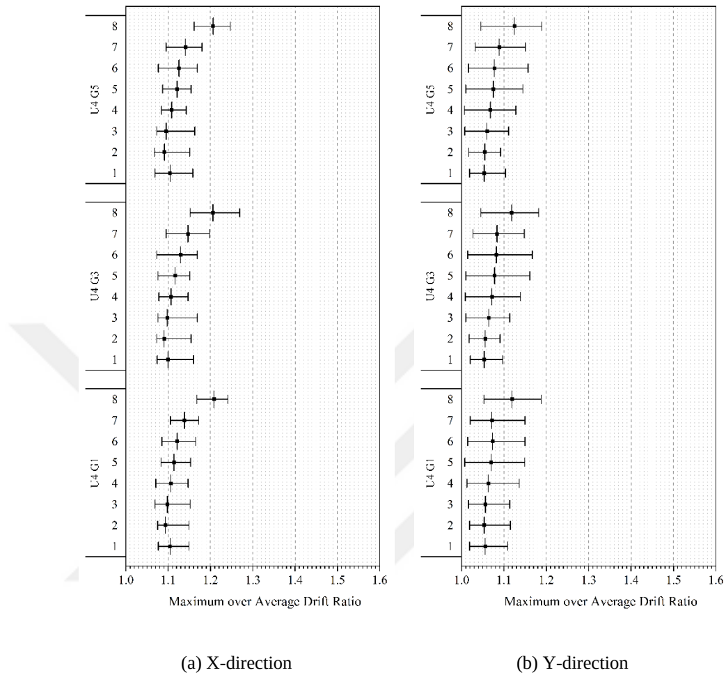
Figure 5.29 Variation of CM maximum drift to average drift ratios for U4 – Group 1, 3 and 5 models (Site Class D)
