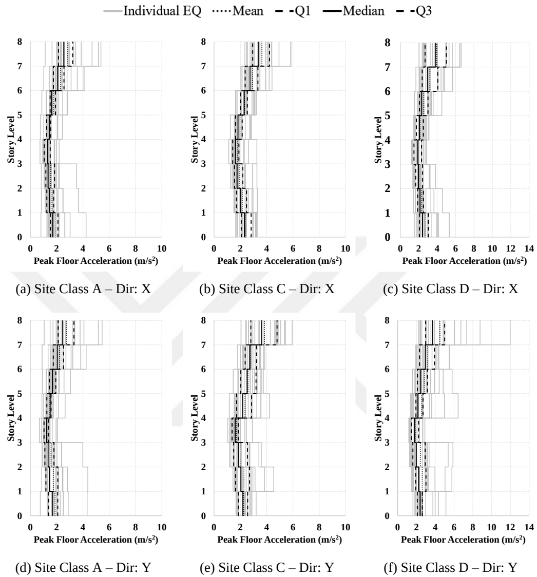
Figure A.27. PFA profiles for building case “U4 Group 1”
