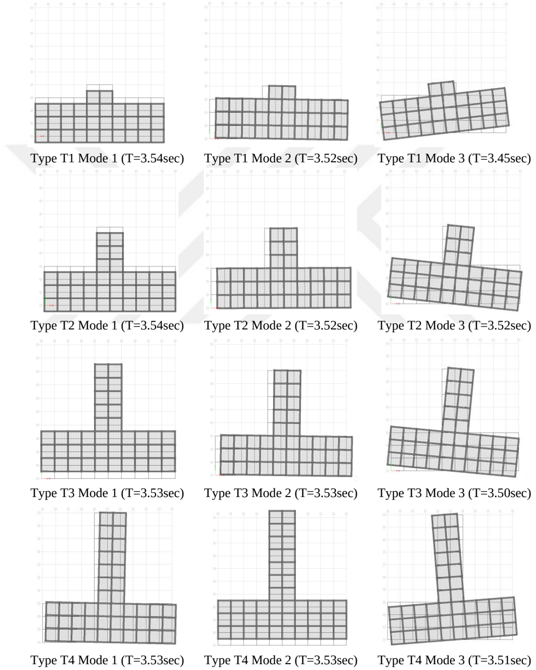
Figure 3.9. Mode shapes of T-shaped model set (Plan view of 8 th story)
