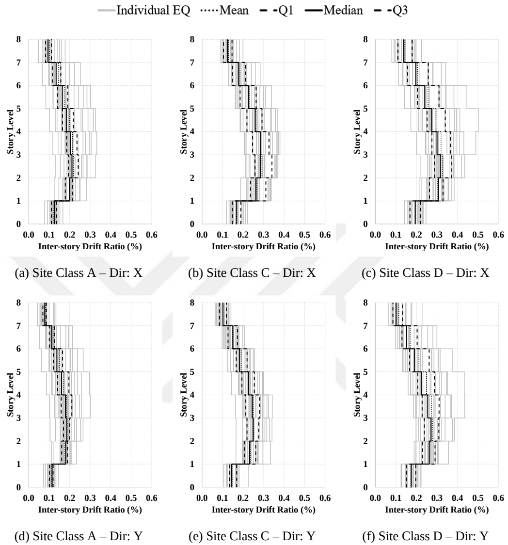
Figure A.13. IDR profiles for building case “U4 Group 1”
