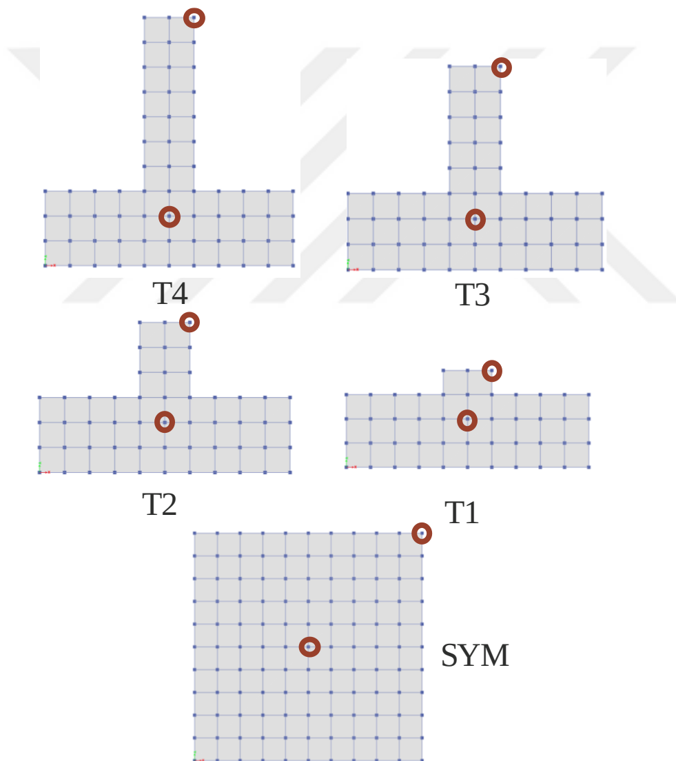
Figure 4.9. Monitored joints for T- and Symmetrical-shaped buildings
