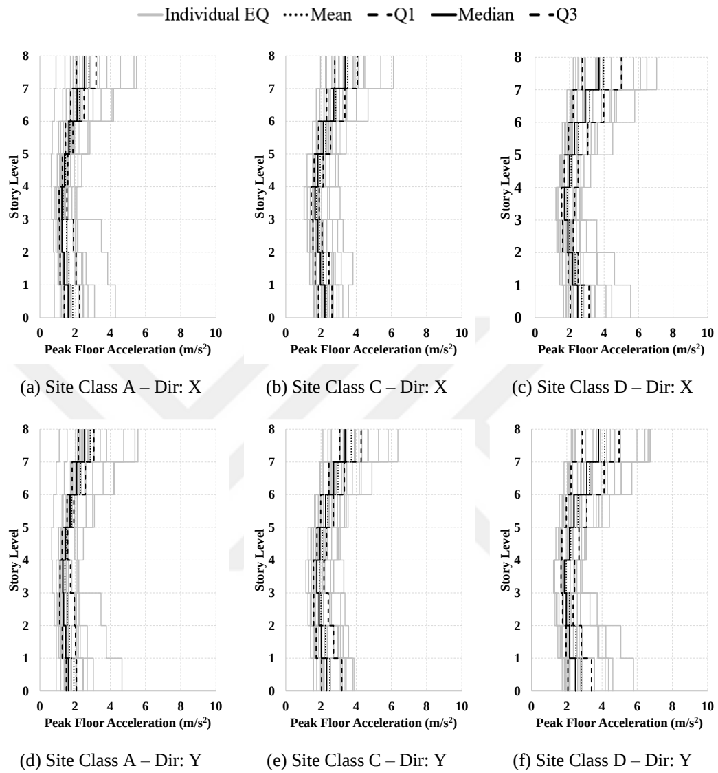
Figure A.17. PFA profiles for building case “T2”
