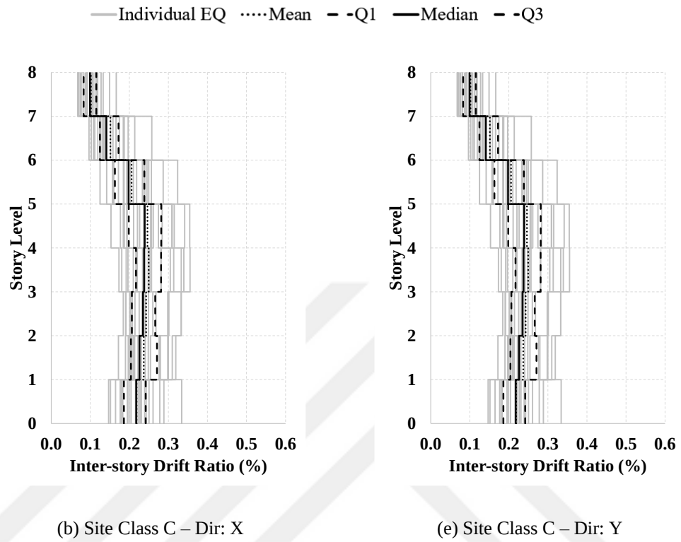
Figure 4.7. IDR profiles for building case “Symmetric” Site Class C
