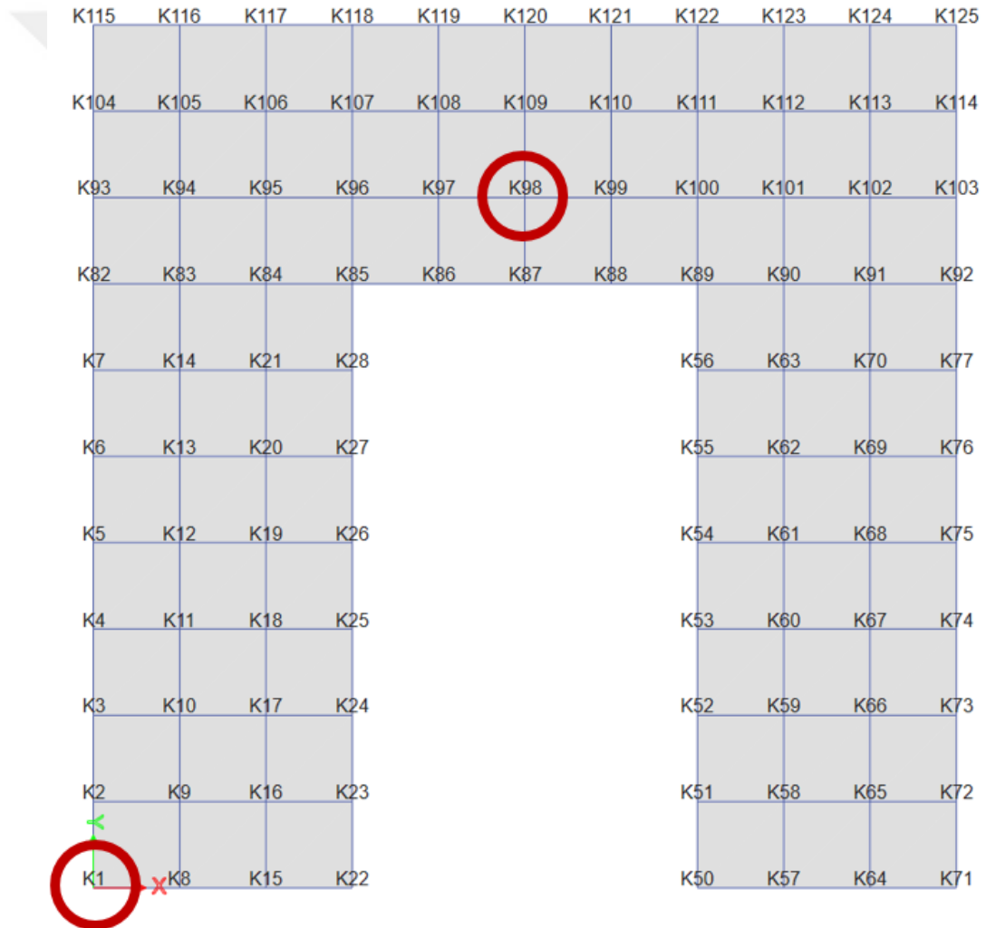
Figure 5.31. Monitored isolator locations on the plan
