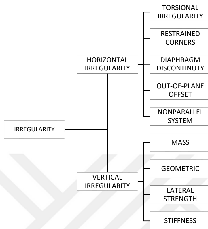
Figure 1.1. Irregularity classification chart ASCE/SEI 7.22 C12.3
