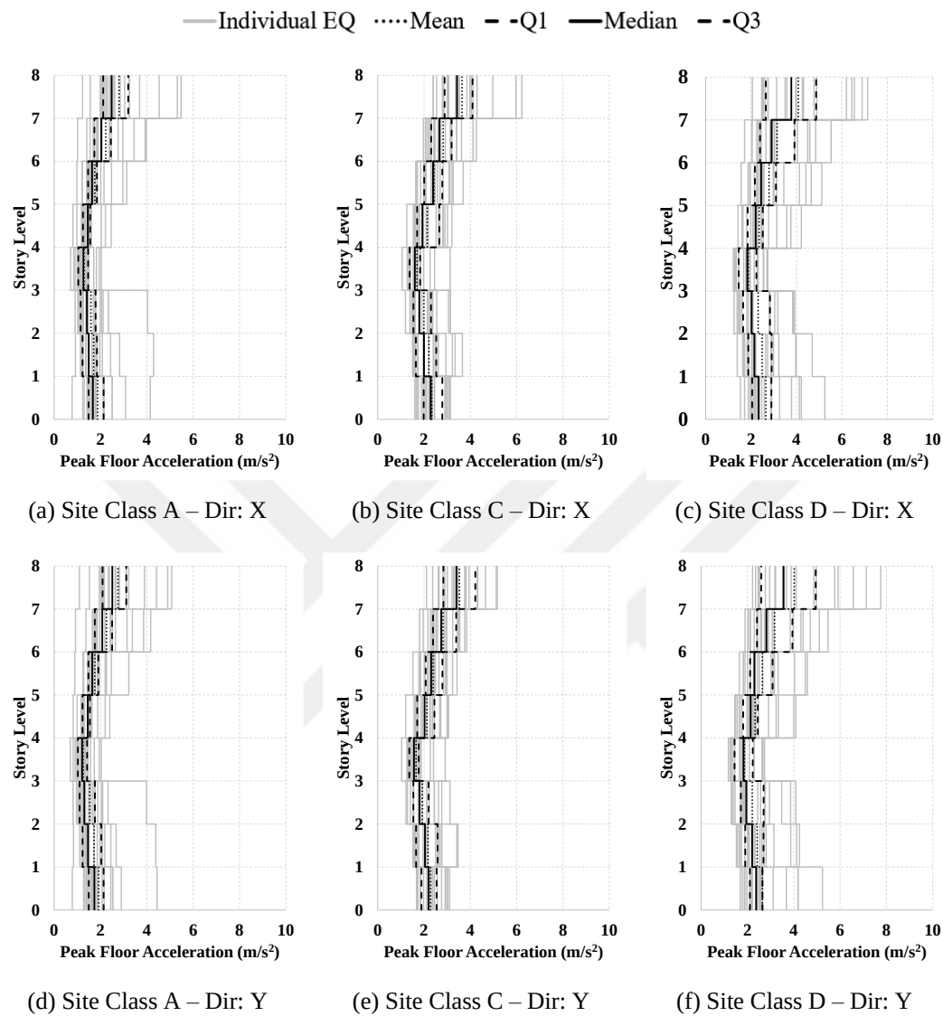
Figure A.22. PFA profiles for building case “U3”
