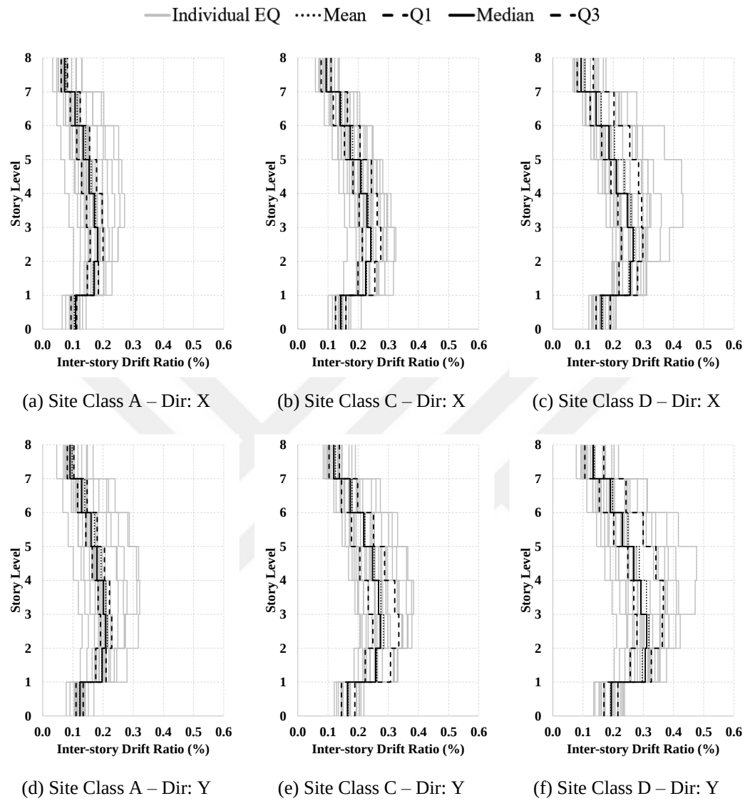
Figure A.6. IDR profiles for building case “U1”
