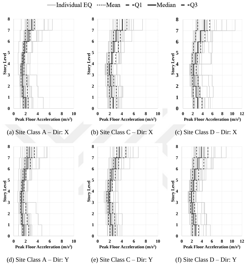
Figure A.25. PFA profiles for building case “T4 Mass”
