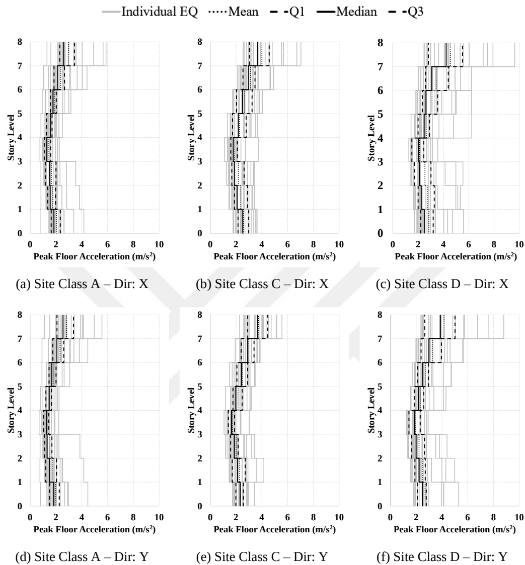
Figure A.26. PFA profiles for building case “U4 Mass”
