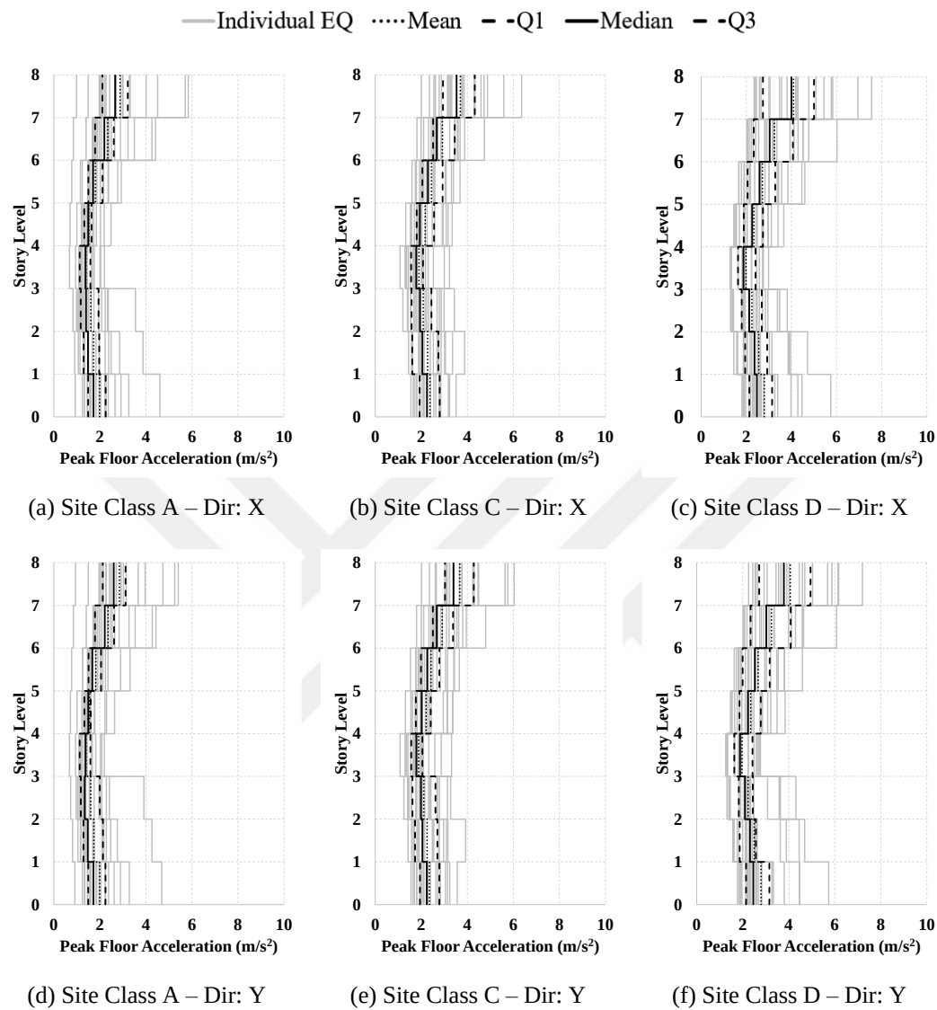
Figure A.24. PFA profiles for building case “Symmetric Mass”
