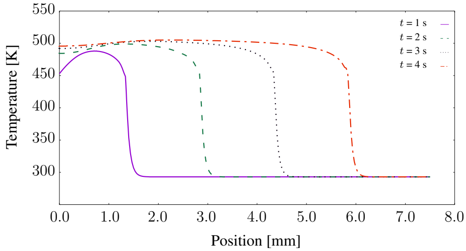
Figure 5.12: The temperature variation with respect to position
