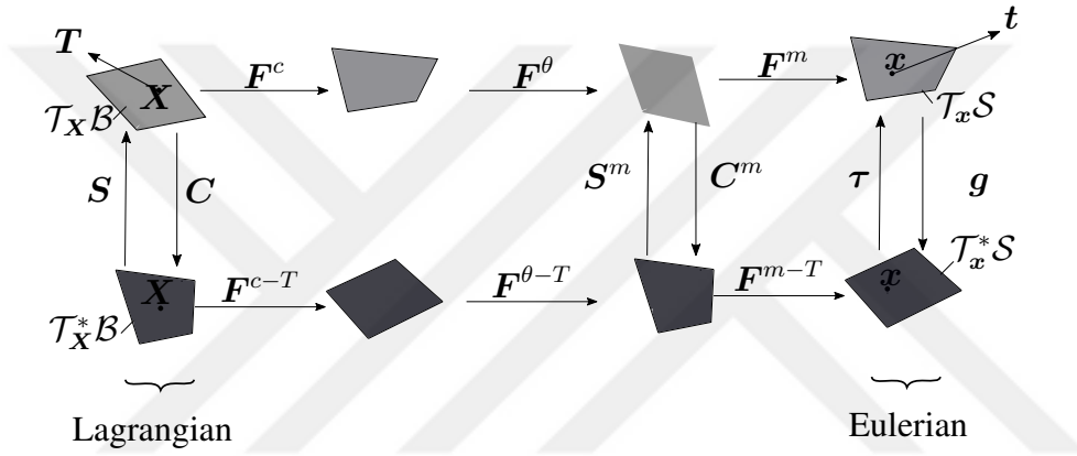
Figure 3.2: Schematic representation of the commutative diagram
