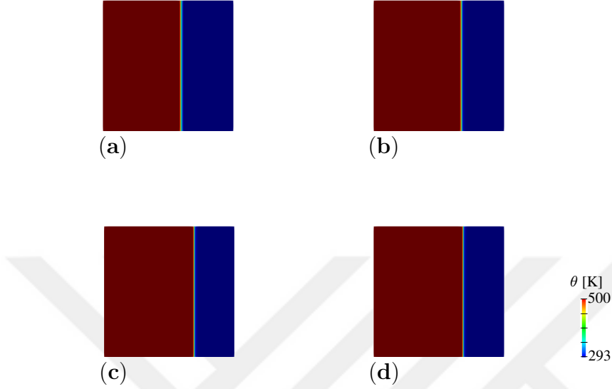
Figure 5.2: The spatial convergence analyzes of the 2D model domain. a) h = 0.15 mm, b) h = 0.075 mm, c) h = 0.033 mm, d) h = 0.025 mm at t = 3.5 s
