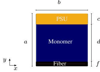
Figure 5.15: Dimension of the 2-D geometry for the composite model problem
