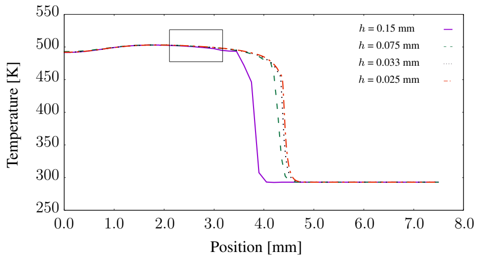
Figure 5.3: The spatial convergence analyses of the 2D model domain
