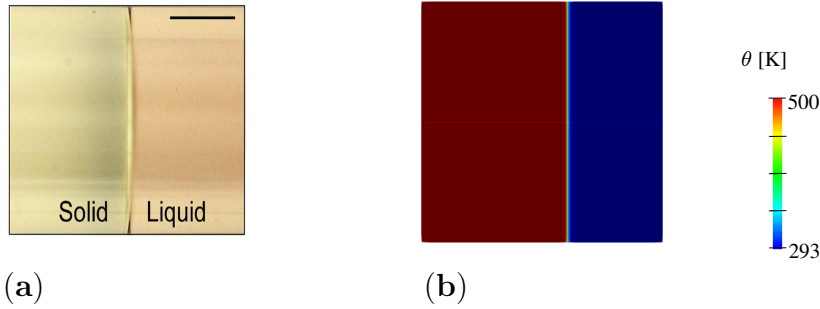
Figure 5.11: The comparison between the experimental result [3] and numerical result
