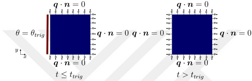
Figure 5.9: Boundary condition for the 2D model problem
