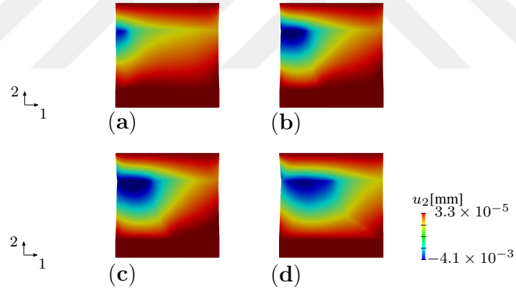
Figure 5.48: Displacement simulation u_2 for material frontally polymerized at a) t = 0.2 s, b) t = 0.6 s, c) t = 1.0 s, d) t = 1.4 s.
