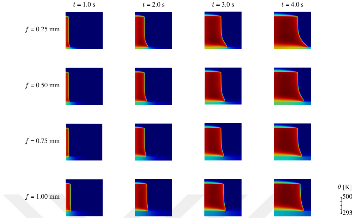
Figure 5.16: Temperature variation in the composite with distinct fiber fractions and at different times
