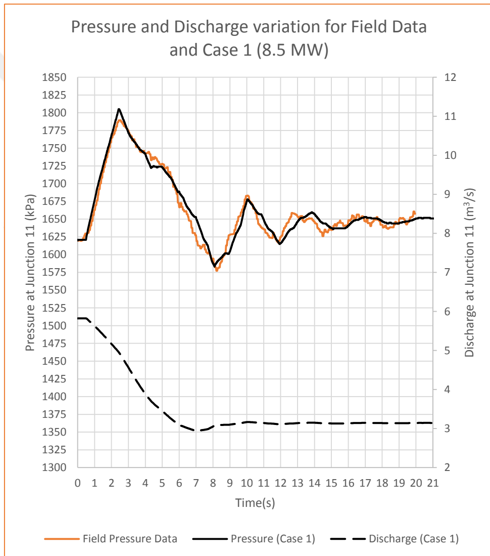
Figure 5.8 Comparison of Pressure Variation between Field data (8.5 MW Test) and Case 1 with Flow Variation
