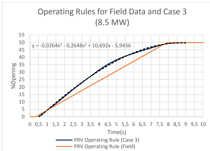
Figure 5.19 Comparison of PRV Operating Rules in Case 3 and measured data for 8.5 MW Test
