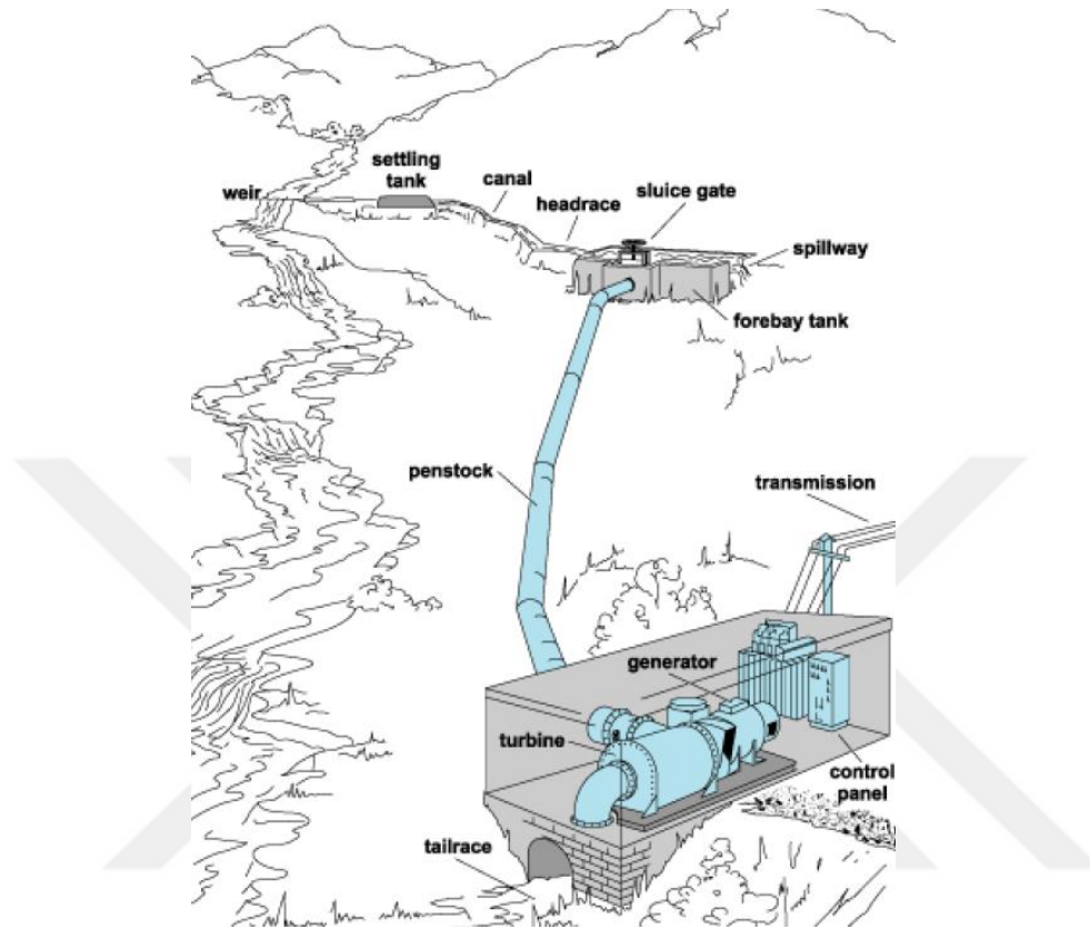
Figure 2.1 Illustration of a Run-of-river HPP (Dursun, 2013)
