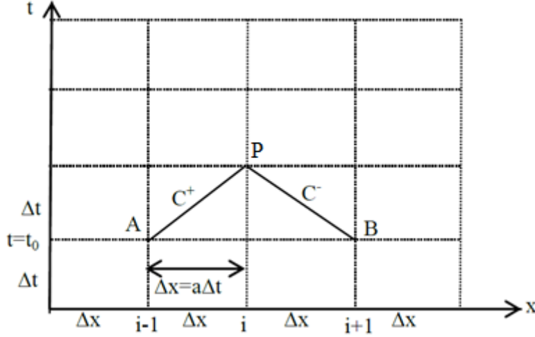
Figure 3.9 Characteristics Lines in x-t solution domain
