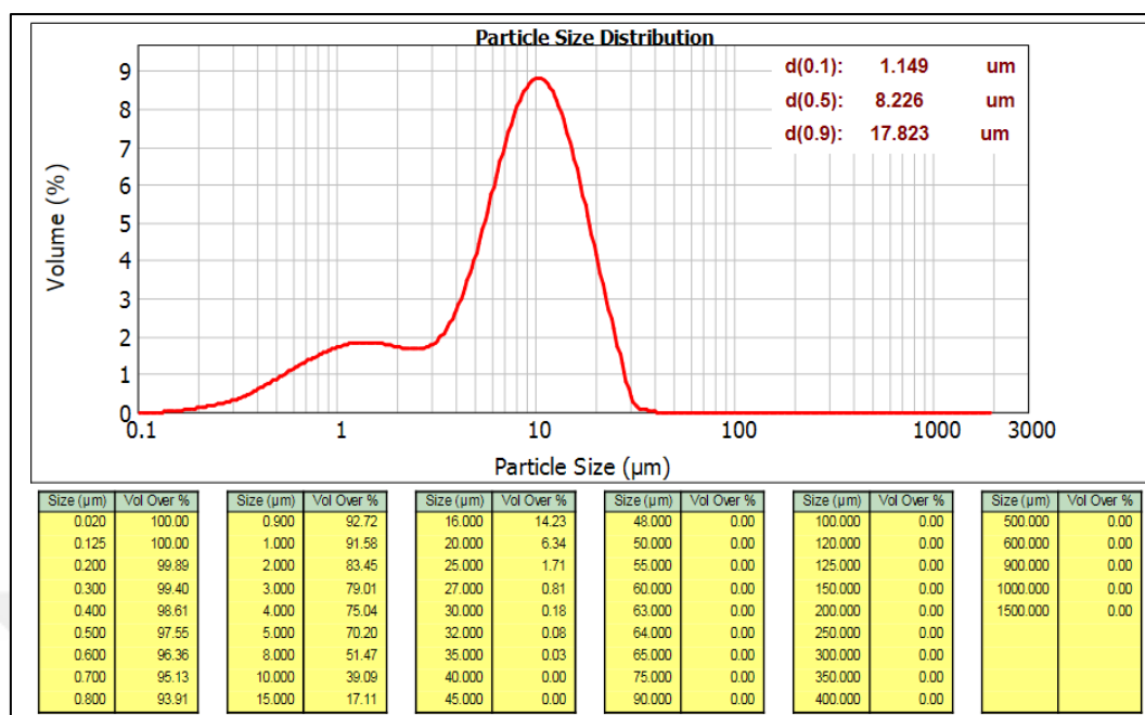
Figure C.5 The result of particle size analysis of PCC product (marble origin) produced by using 5% \text{Ca}(\text{OH})_2 concentration at 5 bar \text{CO}_2 pressure
