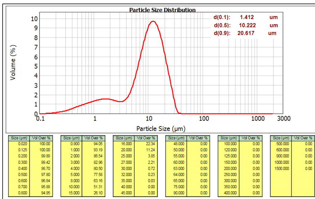
Figure C.7 The result of particle size analysis of PCC product (marble origin) produced by using 10% \text{Ca}(\text{OH})_2 concentration at 5 bar \text{CO}_2 pressure
