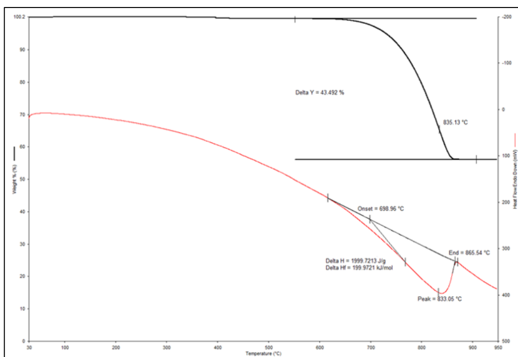
Figure 3.4 TG-DSC profile of the limestone
