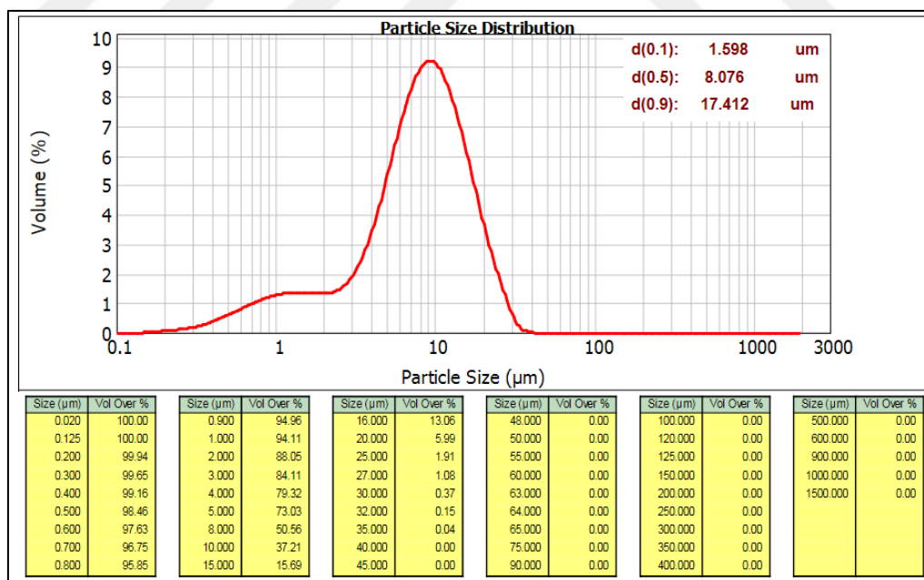
Figure C.2 The result of particle size analysis of PCC product (limestone origin) produced by using 5% \text{Ca}(\text{OH})_2 concentration at 10 bar \text{CO}_2 pressure
