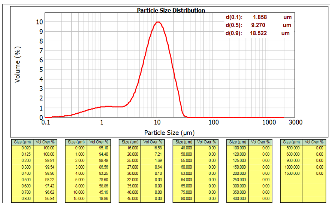
Figure C.3 The result of particle size analysis of PCC product (marble origin) produced by using 10% \text{Ca}(\text{OH})_2 concentration at 10 bar \text{CO}_2 pressure
