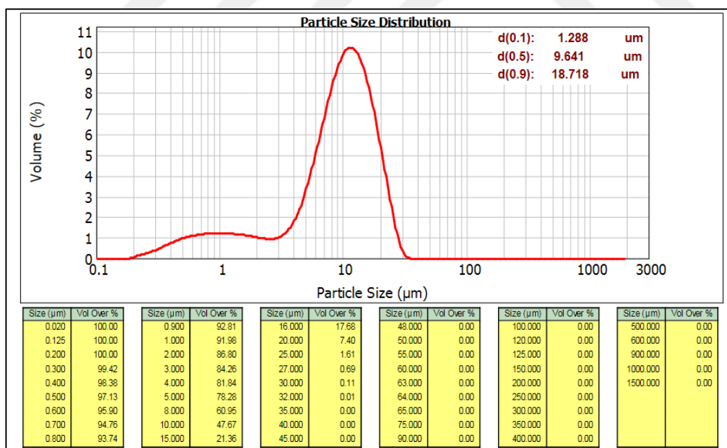
Figure C.4 The result of particle size analysis of PCC product (limestone origin) produced by using 10% \text{Ca}(\text{OH})_2 concentration at 10 bar \text{CO}_2 pressure
