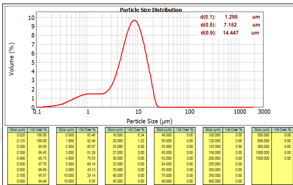
Figure C.1 The result of particle size analysis of PCC product (marble waste origin) produced by using 5% \text{Ca}(\text{OH})_2 concentration at 10 bar \text{CO}_2 pressure
