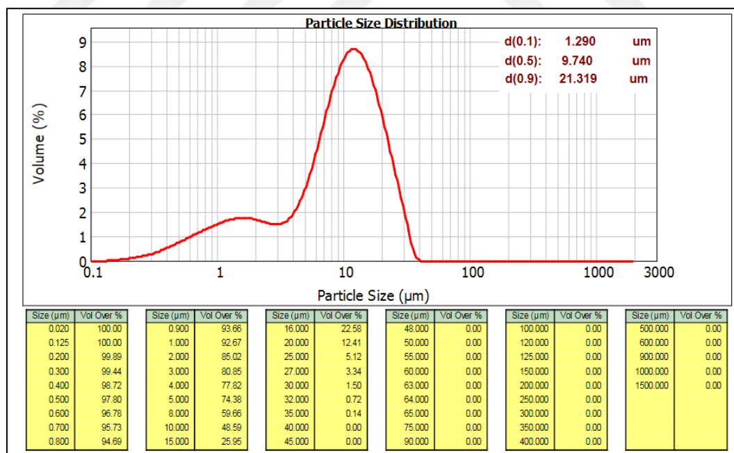
Figure C.6 The result of particle size analysis of PCC product (limestone origin) produced by using 5% \text{Ca}(\text{OH})_2 concentration at 5 bar \text{CO}_2 pressure
