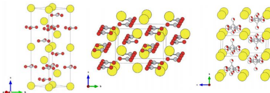
Unit cell
