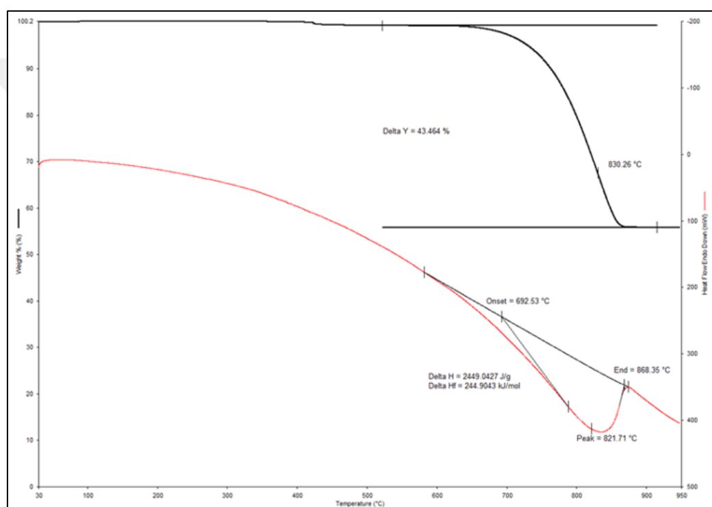
Figure 3.3 TG-DSC profile of the marble waste
