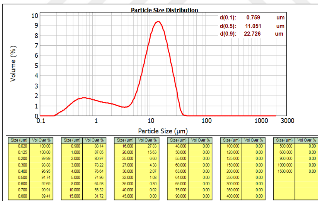
Figure C.8 The result of particle size analysis of PCC product (limestone origin) produced by using 10% \text{Ca}(\text{OH})_2 concentration at 5 bar \text{CO}_2 pressure
