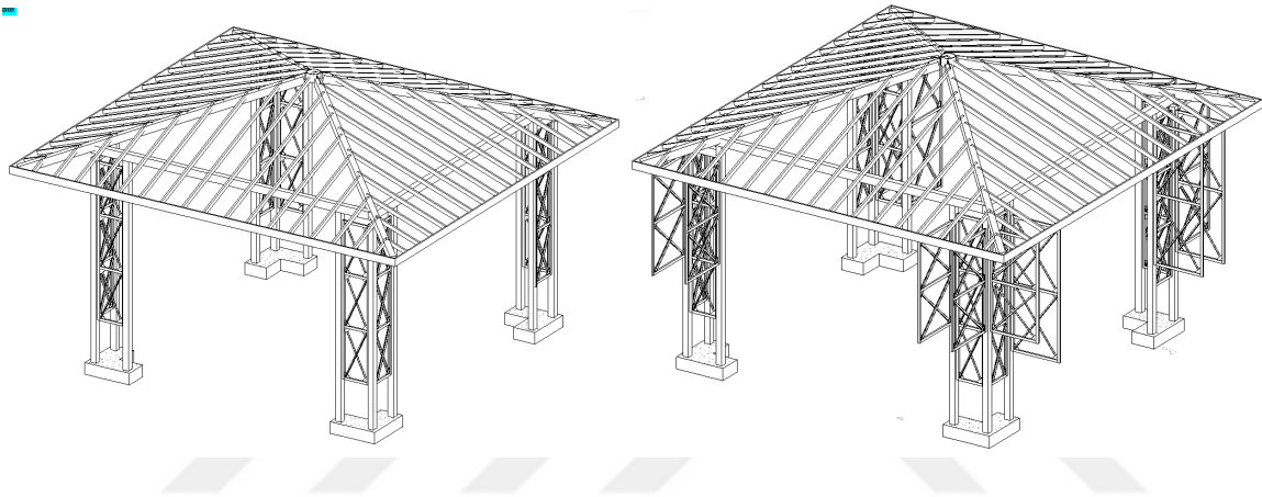
Figure 4.38. Soğukluk roof structure exported from Revit, (a) Roof structure only, (b) Structure with side carriers
