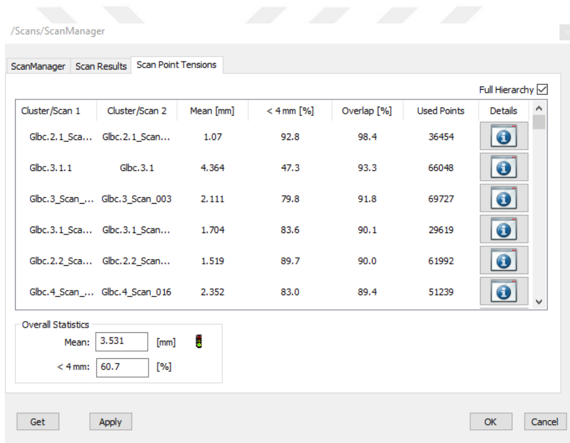
Figure 4.3. Point cloud registration result (standard deviation)
