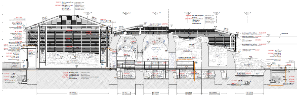
Figure 4.34. Combined drawings of the restoration project
