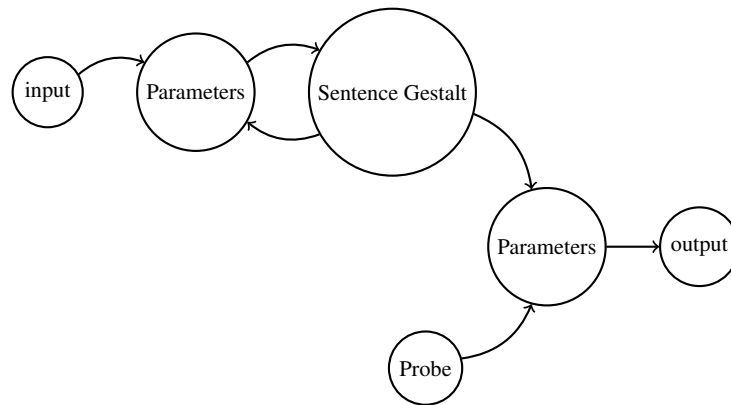
Figure 5.16: McClelland model
