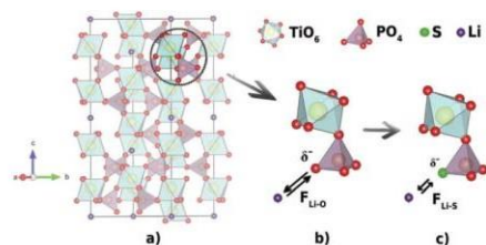
Fig. 9 (a) NASICON crystal structure of LATP, (b) atomic local environment of bare-LATP and (c) atomic local environment of sulfur-doped LATP, where the sulfur atoms are replaced with oxygen atoms.
