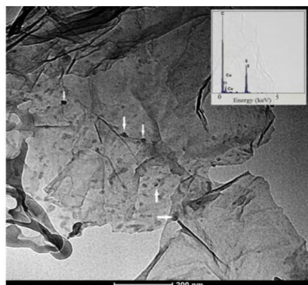
Figure 4. TEM analysis of rGO/S composite with EDS in the inset.
