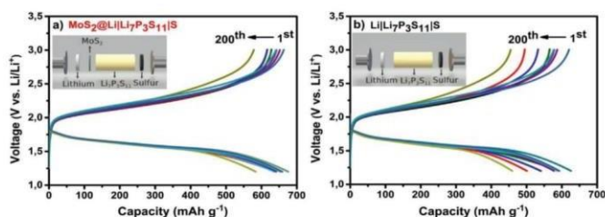
Figure 6. Galvanostatic charge–discharge analysis of all solid state a) \text{MoS}_2@\text{Li}/\text{Li}_7\text{P}_3\text{S}_{11}/\text{S} and b) \text{Li}/\text{Li}_7\text{P}_3\text{S}_{11}/\text{S} cells.
