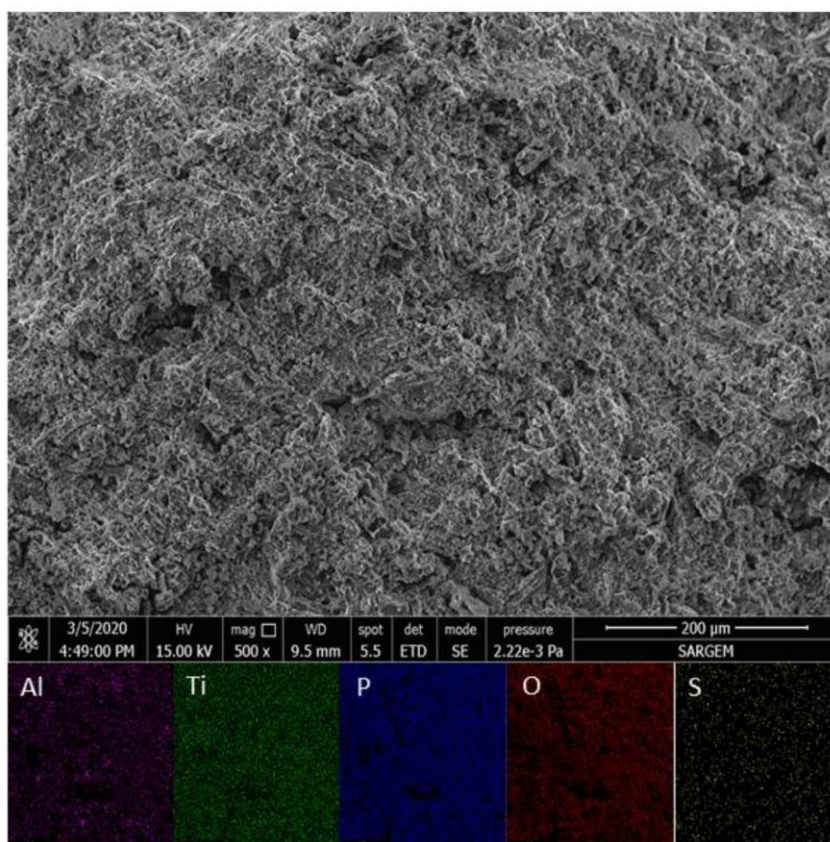
Fig S5: Fracture surface FESEM image and corresponding EDS mapping of LAMP-005S.
