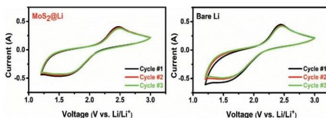
Figure 5. CV analysis of all solid state a) \text{MoS}_2@\text{Li}/\text{Li}_7\text{P}_3\text{S}_{11}/\text{S} and b) \text{Li}/\text{Li}_7\text{P}_3\text{S}_{11}/\text{S} cells.
