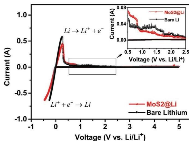
Figure 3. CV analysis of \text{MoS}_2\text{@Li}/\text{Li}_7\text{P}_3\text{S}_{11}/\text{SUS} and \text{Li}_7\text{P}_3\text{S}_{11}/\text{SUS} cells.
