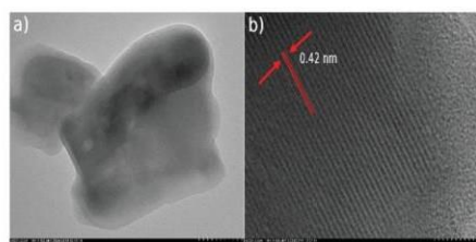
Fig. 6 TEM analysis of bare LATP powders (a) low magnification and (b) HRTEM analysis of bare-LATP.
