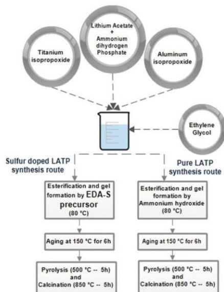
Fig. 1 Synthetic route to pure-LATP and the sulfur-doped LATP.
