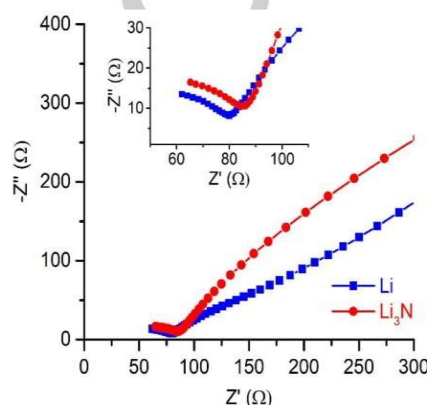
Figure 8. Impedance analysis of the cell with pure Lithium and \text{Li}_3\text{N} protected Li used as anode where \text{Li}_7\text{P}_3\text{S}_{11} and (\text{rGO/S/CB/ Li}_7\text{P}_3\text{S}_{11}) used as solid electrolyte and cathode respectively
