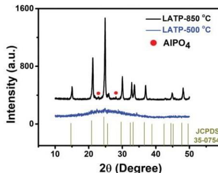
Fig. 2 XRD analysis of heat-treated LATP at 500 °C and 850 °C for 5 h.
