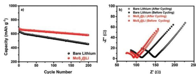
Figure 7. Cycle analysis of all solid state a) MoS 2 @Li/Li 7 P 3 S 11 /S and Li/Li 7 P 3 S 11 /S cells and, b) Nyquist plots for MoS 2 @Li/Li 7 P 3 S 11 /S and Li/Li 7 P 3 S 11 /S cells before and after galvanostatic cycling.
