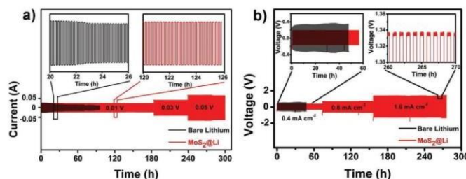
Figure 4. a) Chronoamperometry analysis of symmetric cells assembled with bare lithium and \text{MoS}_2\text{@Li} as anode at different voltages and b) chronovoltammetry analysis of symmetric cells assembled with bare lithium and \text{MoS}_2\text{@Li} as anode at different current densities.
