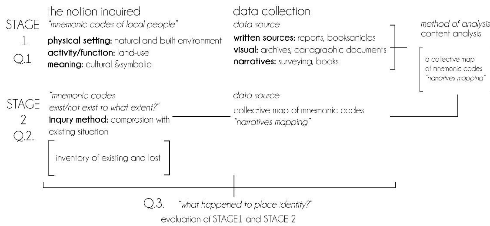
Figure 10 Methodological Framework
