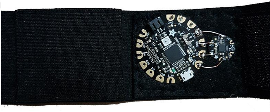
Figure 4.10 The placement of the 9-DOF IMU (The sensor is on the right)
