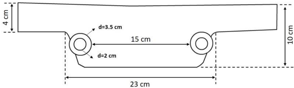
Figure 4.15 The dimensions of the interactive belt
