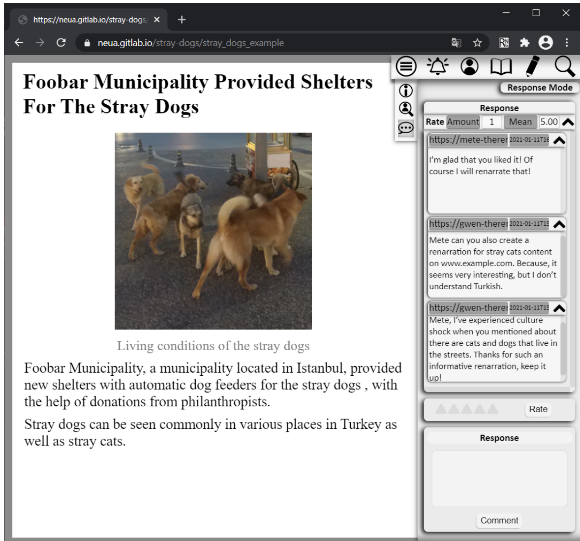
Figure 7.41. Response UI of RNEx for the stray dogs web page
