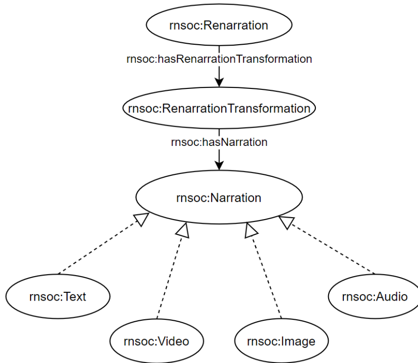
Figure 5.9. Narration class and its significant relations
