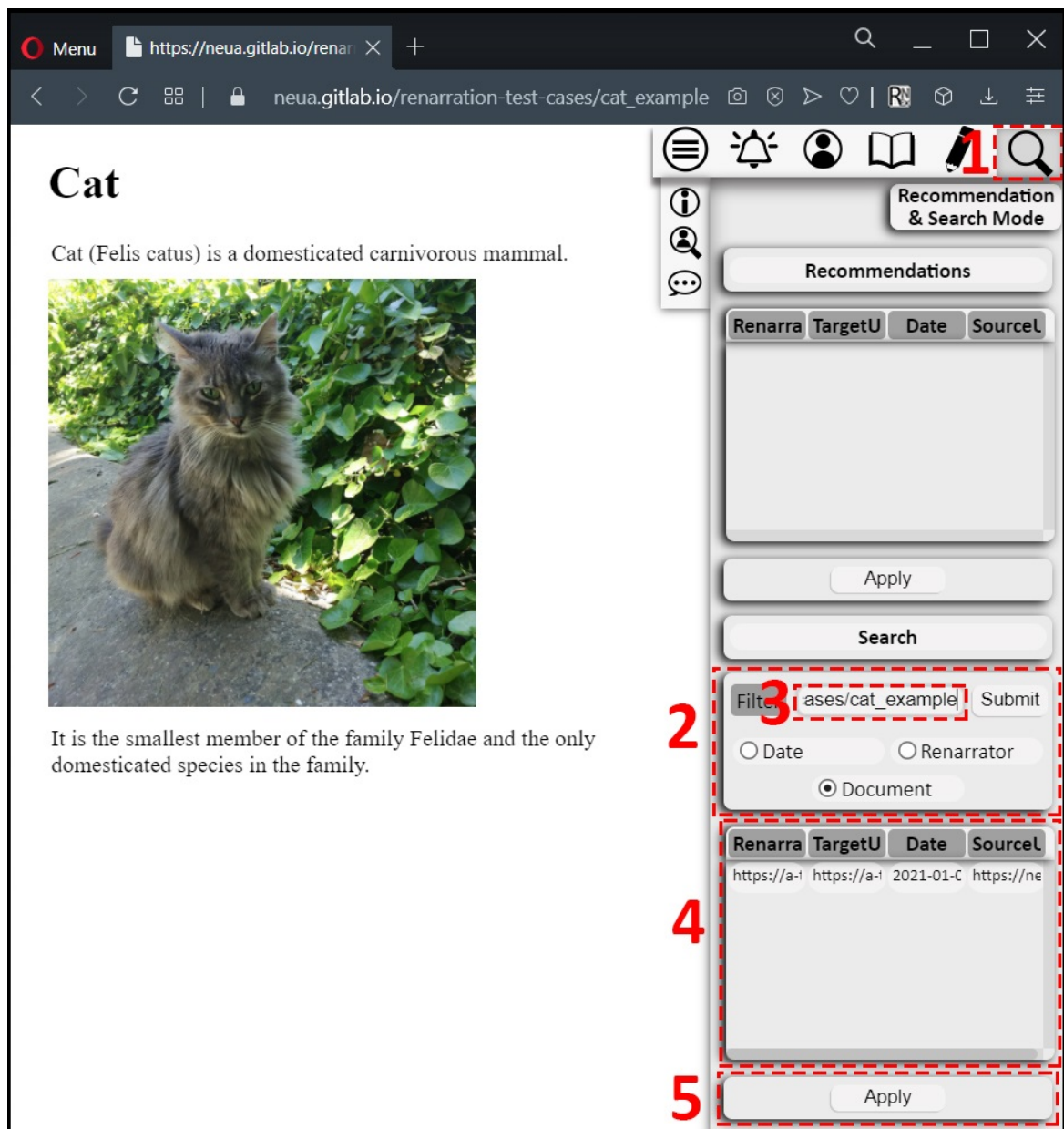
Figure 6.23. Searching functionality of the prototype
