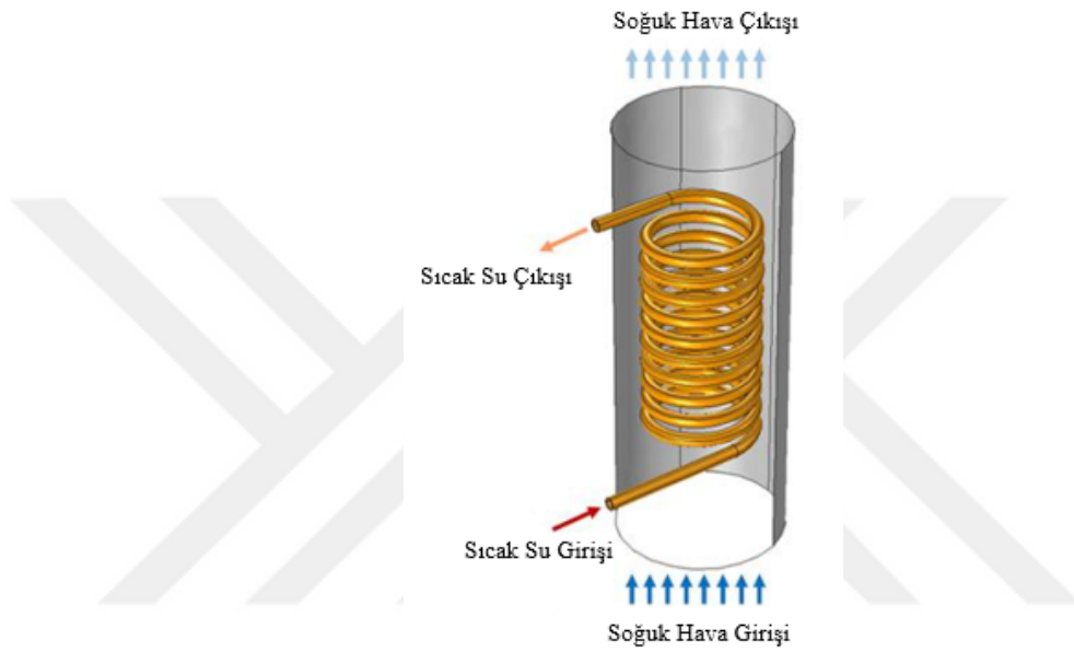
řekil 3.9. Spiral borulu ısı deęiřtiricisi (“Modeling a Coil Heat Exchanger COMSOL”, 2021).
