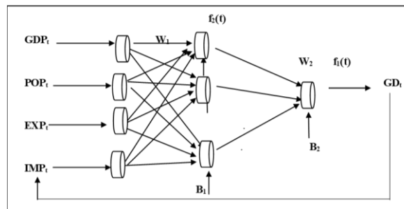
Figure 21: ANN Model with Single Layer Four Inputs
