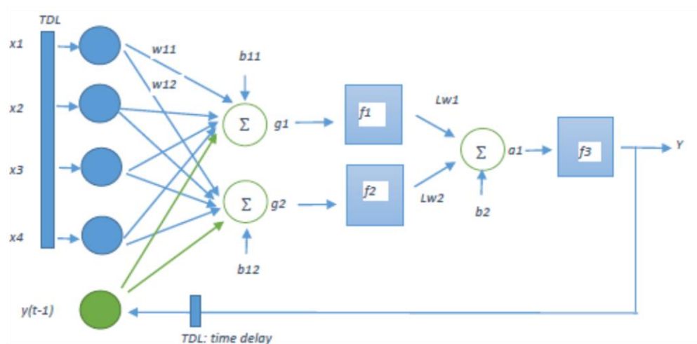
Figure 26 : ANN Schema with Weights and Bias
