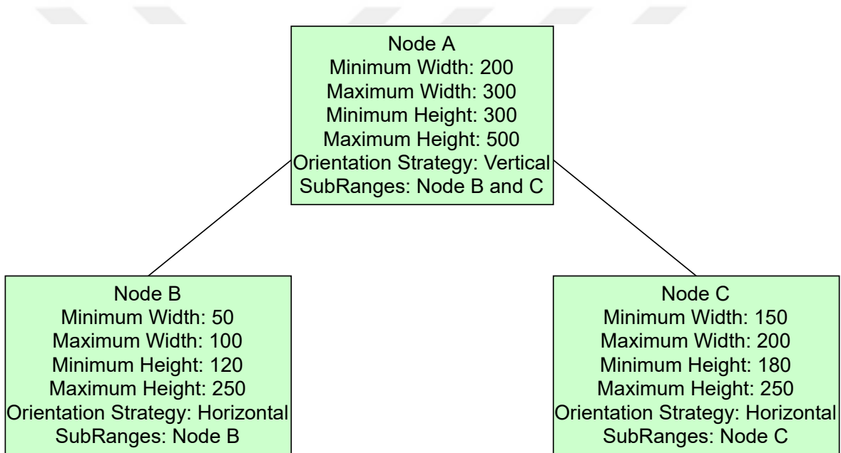
FIGURE 3.1. WidthHeightRange example
