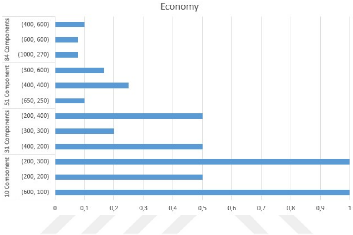
FIGURE 6.31. Economy parameter results for each resolution.
