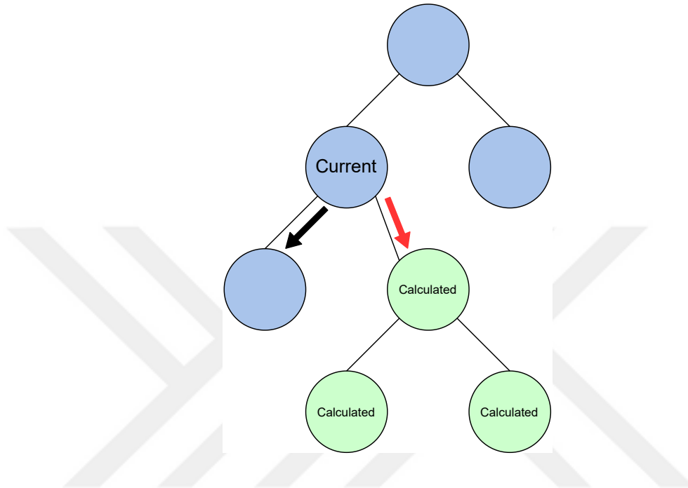
FIGURE 3.7. Green circles represent the calculated nodes which have their memoization fields filled and blue circles represent non calculated nodes
