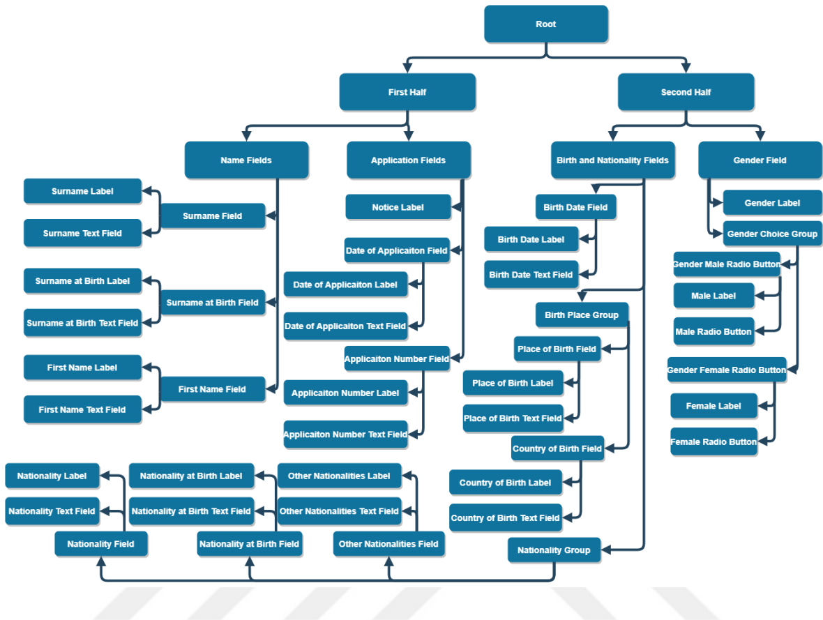
FIGURE 6.6. Layout 2, composed of 51 components, which are 28 UI components and 23 containers
