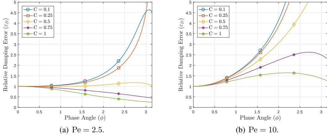
Figure 5.1. Relative damping error for various values of Courant numbers, using SD-FEM in space and Crank-Nicolson method in time.
