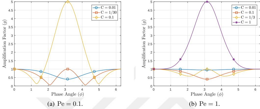
Figure 4.2. Amplification factor using SGFEM in space and forward Euler method in time for various choices of Courant numbers.
