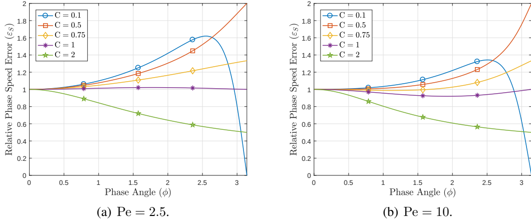
Figure 5.3. Relative phase speed error for various values of Courant numbers using SDFEM in space and Crank-Nicolson method in time.
