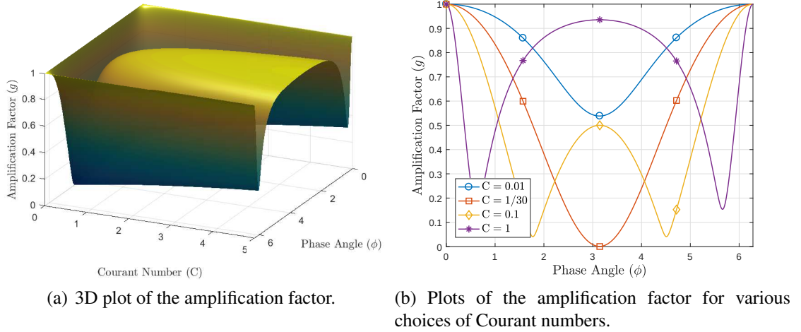
Figure 4.3. Amplification factor for \text{Pe} = 0.1 using SGFEM in space and Crank-Nicolson method in time.
