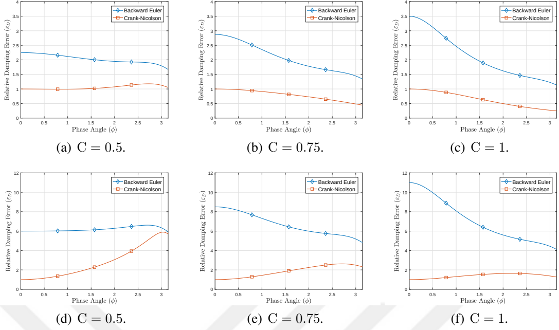
Figure 5.5. Comparison of relative damping errors of the time integrators for convective-diffusive case: Pe = 2.5 on the above and Pe = 10 on the below.
