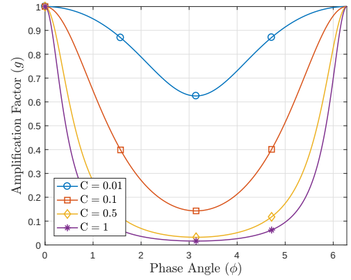
(b) Plots of the amplification factor for various choices of Courant numbers.
