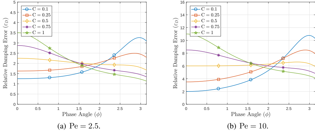
Figure 5.2. Relative damping error for various values of Courant numbers, using SD-FEM in space and backward Euler method in time.
