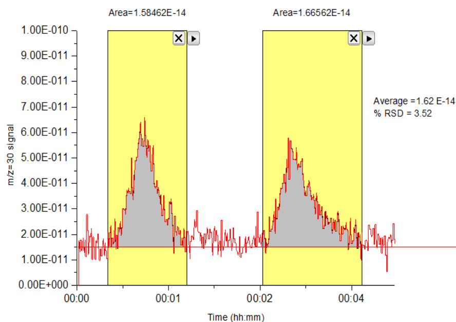
Figure A. 18: Integrated area of the m/z = 30 signal curve of HTCO analysis of 20 mg edta disodium salt 99ehydrate over 3 % Cu-7% Ce / \text{Al}_2\text{O}_3 catalyst sample at 700 °C in the presence of 500 sccm air flow
