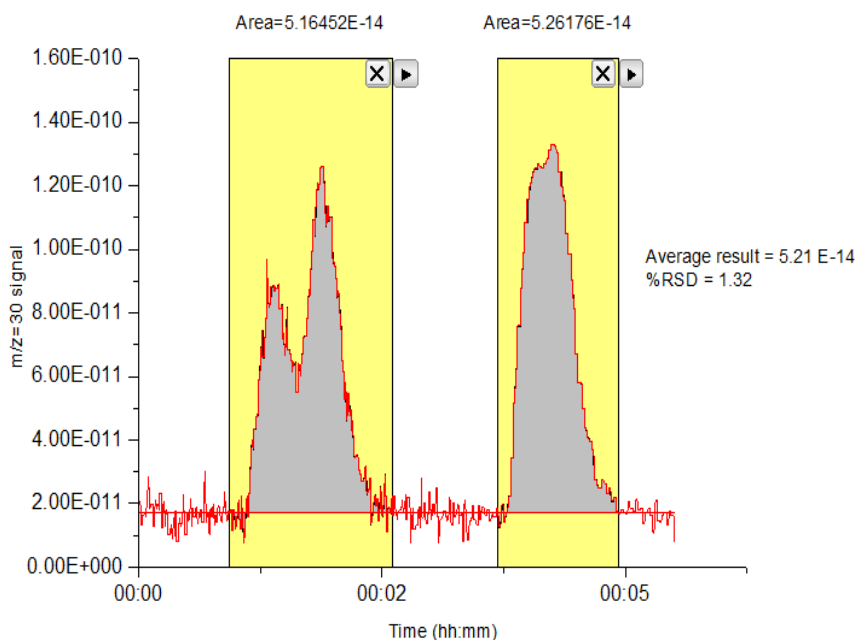
Figure A. 17: Integrated area of the m/z = 30 signal curve of HTCO analysis of 20 mg ammonium sulfate over 3 % Cu-7% Ce / \text{Al}_2\text{O}_3 catalyst sample at 700 °C in the presence of 500 sccm air flow
