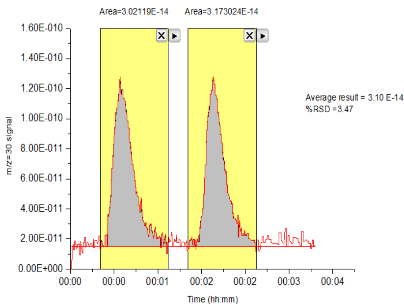
Figure A. 15: Integrated area of the m/z = 30 signal curve of HTCO analysis of 5 mg urea over 3 % Cu-7% Ce / \text{Al}_2\text{O}_3 catalyst sample at 700 °C in the presence of 500 sccm air flow
