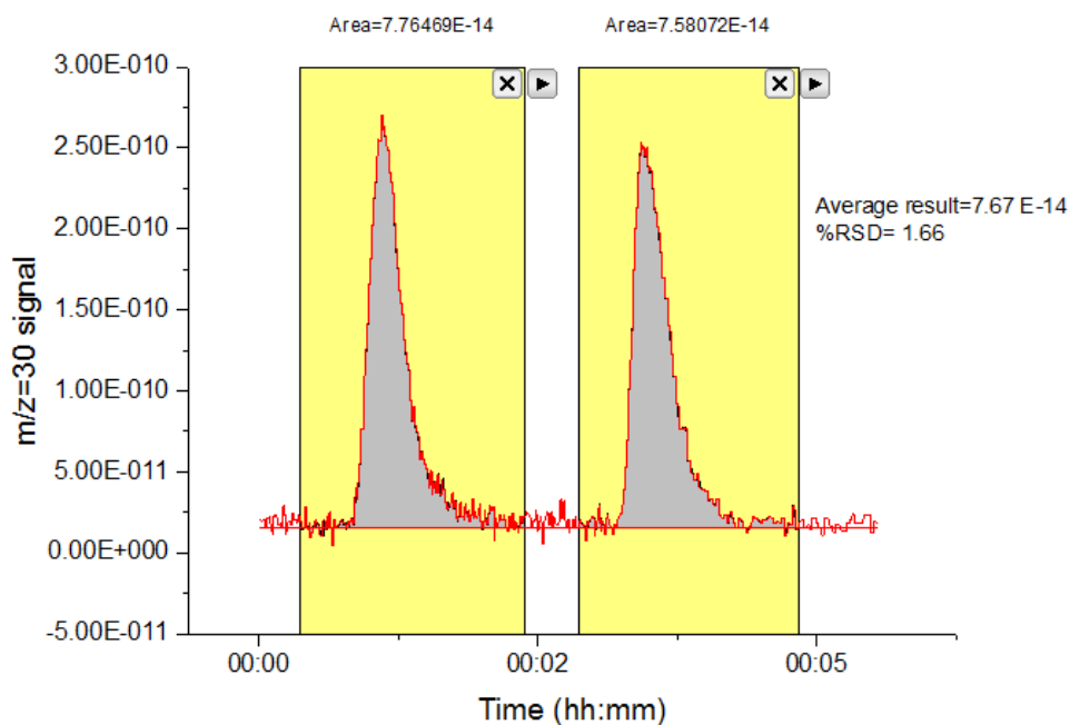
Figure A. 31: Integrated area of the m/z = 30 signal curve of HTO analysis of 20 mg ammonium nitrate over 1 % wt Pt / \text{Al}_2\text{O}_3 catalyst sample at 700 ^{\circ}\text{C} in the presence of 500 sccm air flow
