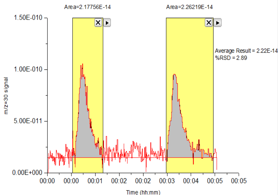
Figure A. 30: Integrated area of the m/z = 30 signal curve of HTO analysis of 600 \mu\text{l} of 2.5 % by volume pyridine solution over 1 % wt Pt / \text{Al}_2\text{O}_3 catalyst sample at 700 ^{\circ}\text{C} in the presence of 500 sccm air flow
