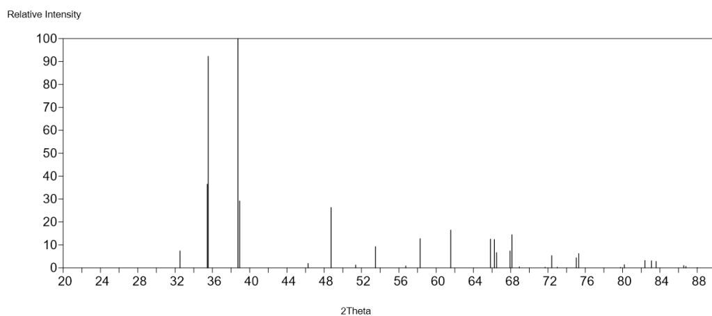
Figure C. 2: Reference XRD pattern of CuO structure obtained from ICDS PDF Card No.: 01-089-5897
