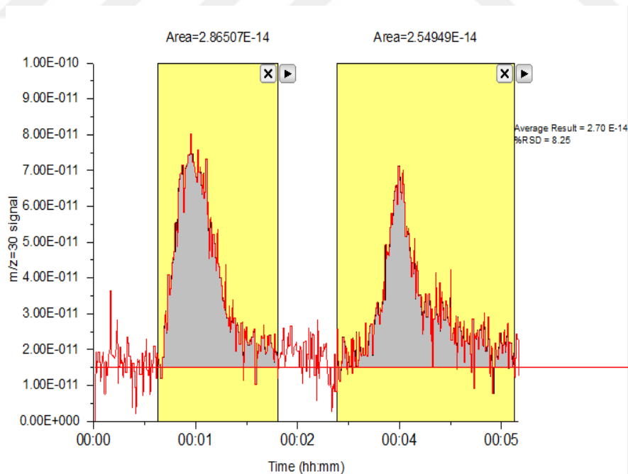
Figure A. 19: Integrated area of the m/z = 30 signal curve of HTCO analysis of 40 mg glutamic acid over 3 % Cu-7% Ce / \text{Al}_2\text{O}_3 catalyst sample at 700 °C in the presence of 500 sccm air flow
