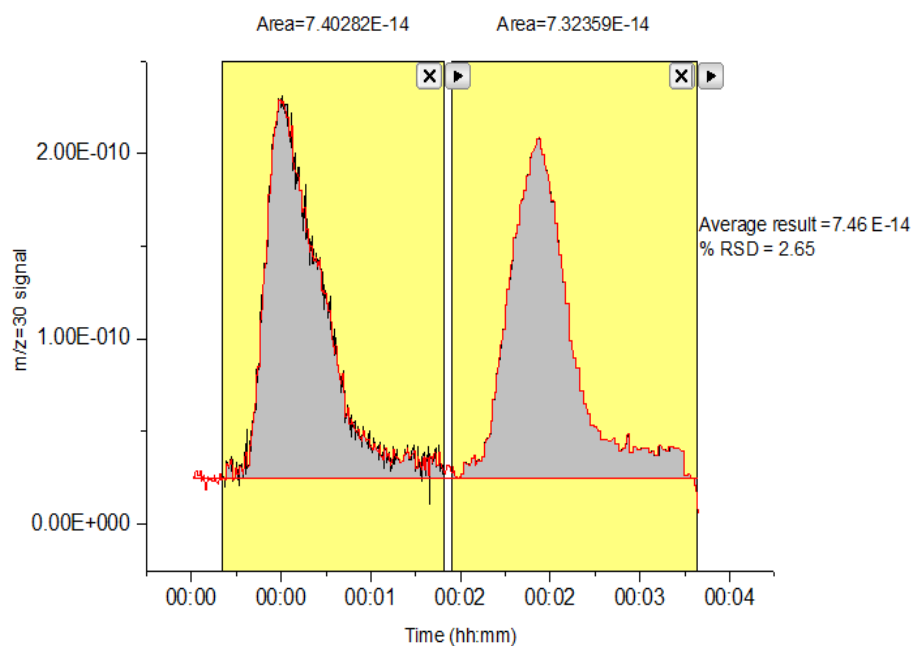
Figure A. 22: Integrated area of the m/z = 30 signal curve of HTCO analysis of 20 mg ammonium nitrate over 5 % wt Fe / \text{Al}_2\text{O}_3 catalyst sample at 700 °C in the presence of 500 sccm air flow
