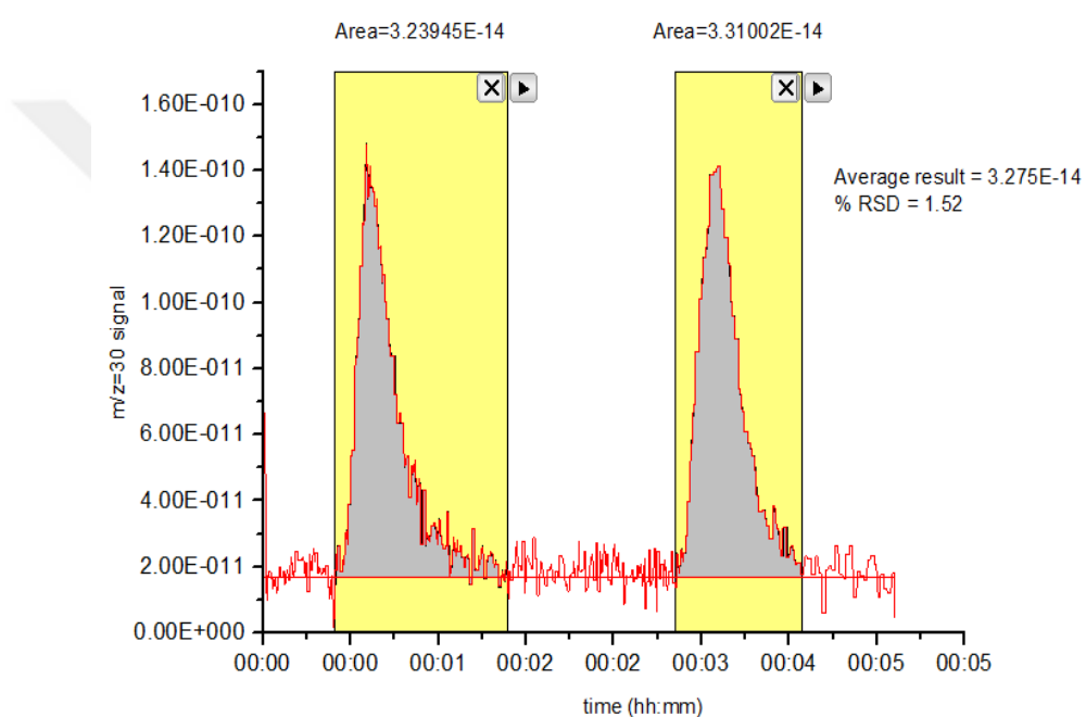
Figure A. 27: Integrated area of the m/z = 30 signal curve of HTCO analysis of 5 mg urea over 1 % wt Pt / \text{Al}_2\text{O}_3 catalyst sample at 700 °C in the presence of 500 sccm air flow
