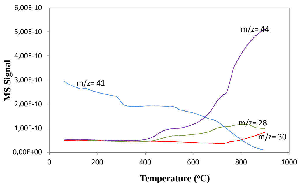
Figure 4. 9: MS trend of TPO of acetonitrile over \text{Al}_2\text{O}_3 support
