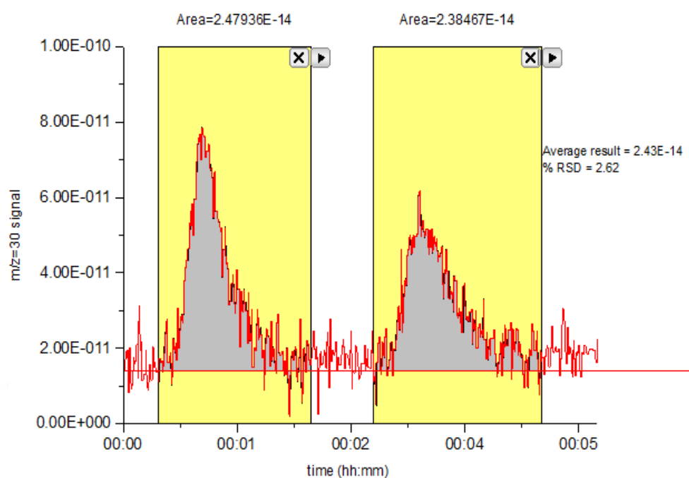
Figure A. 28: Integrated area of the m/z = 30 signal curve of HTCO analysis of 20 mg edta disodium salt dihydrate over 1 % wt Pt / \text{Al}_2\text{O}_3 catalyst sample at 700 °C in the presence of 500 sccm air flow
