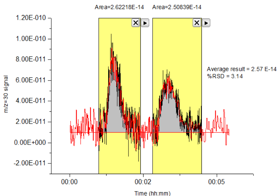
Figure A. 16: Integrated area of the m/z = 30 signal curve of HTCO analysis of 20 mg ammonium nitrate over 3 % Cu-7% Ce / \text{Al}_2\text{O}_3 catalyst sample at 700 °C in the presence of 500 sccm air flow
