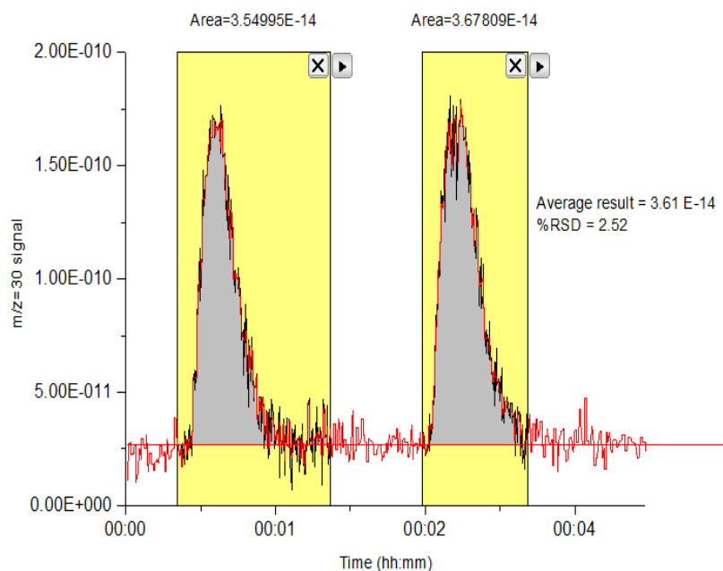
Figure A. 13: Integrated area of the m/z = 30 signal curve of HTCO analysis of 600 µl of 2.5 % by volume pyridine solution over 10 % Cu / Al 2 O 3 catalyst sample at 700 °C in the presence of 500 sccm air flow
