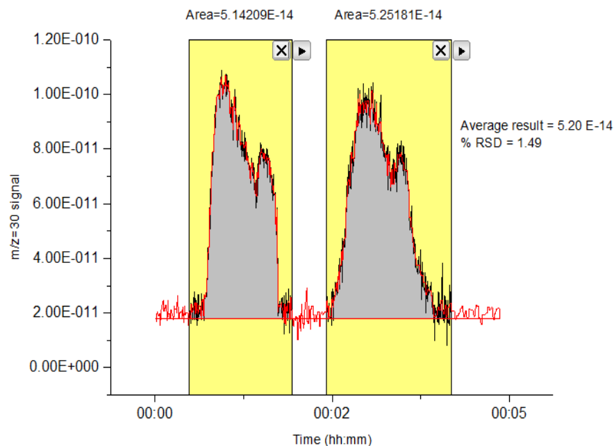
Figure A. 23: Integrated area of the m/z = 30 signal curve of HTCO analysis of 20 mg ammonium sulfate over 5 % wt Fe / \text{Al}_2\text{O}_3 catalyst sample at 700 °C in the presence of 500 sccm air flow
