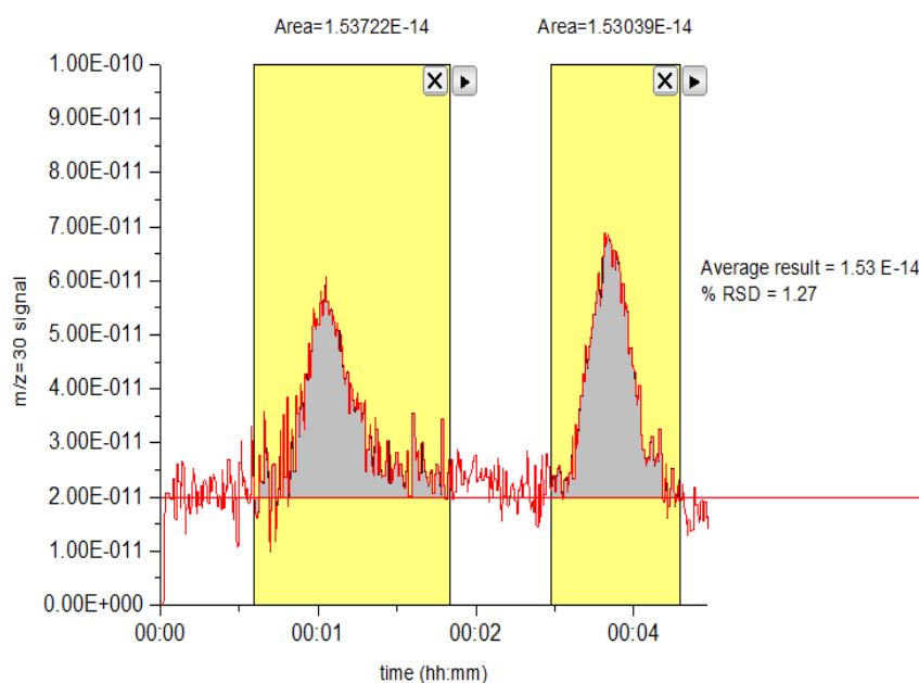
Figure A. 11: Integrated area of the m/z = 30 signal curve of HTCO analysis of 20 mg Edta disodium salt 94ehydrate over 10 % Cu / Al 2 O 3 catalyst sample at 700 °C in the presence of 500 sccm air flow
