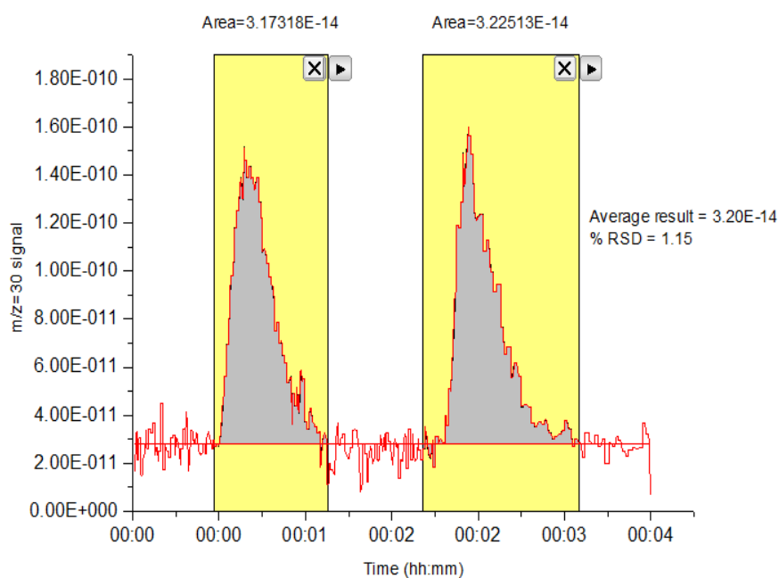
Figure A. 9: Integrated area of the m/z = 30 signal curve of HTCO analysis of 5 mg urea over 10 % Cu / \text{Al}_2\text{O}_3 catalyst sample at 700 °C in the presence of 500 sccm air flow
