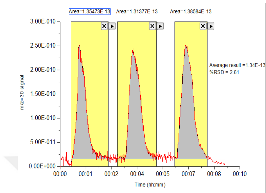
Figure A. 8: Integrated area of the m/z = 30 signal curve of three repetitive HTCO analysis of 60 mg (\text{NH}_4)_2\text{SO}_4 over 1 % wt Pt / \text{Al}_2\text{O}_3 Catalyst Sample at 700 °C in the presence of 500 sccm air flow
