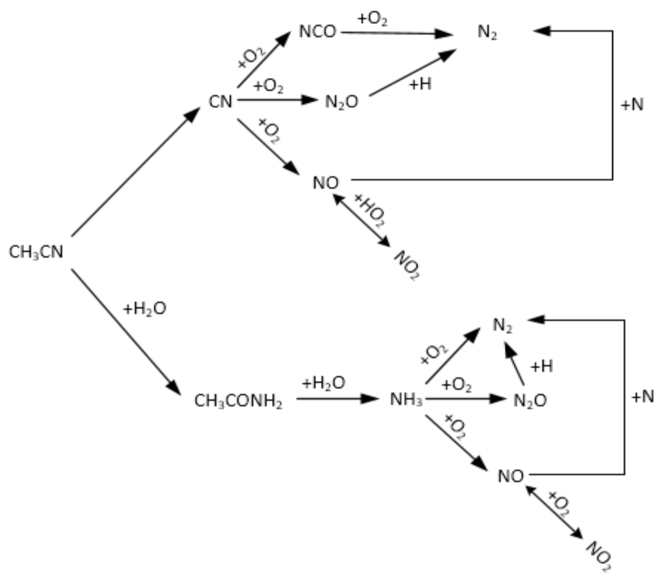
Figure 4. 8: Oxidation mechanisms of acetonitrile ( C_2H_3N )
