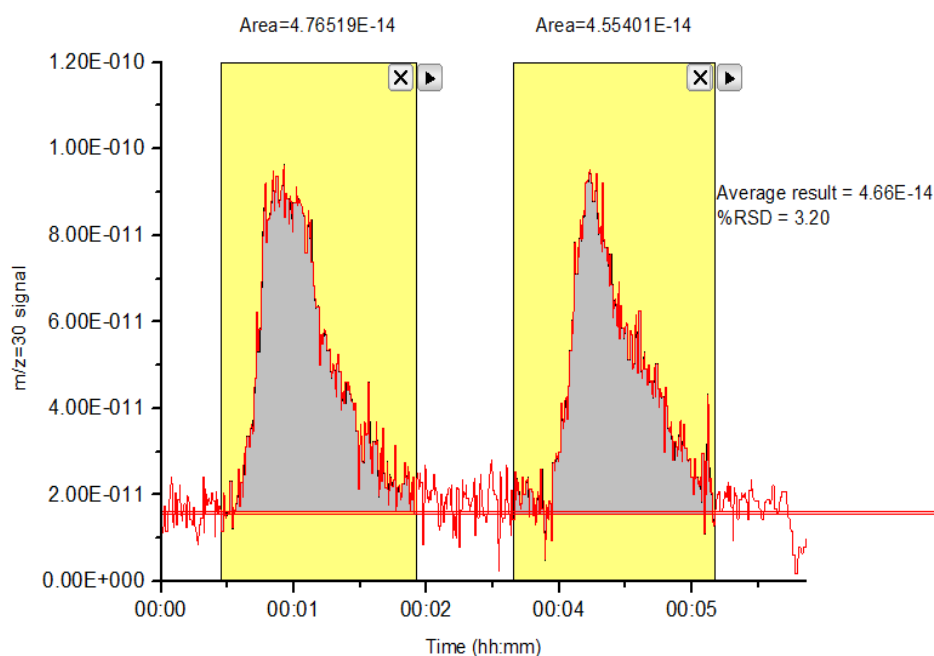
Figure A. 29: Integrated area of the m/z = 30 signal curve of HTCO analysis of 40 mg glutamic acid over 1 % wt Pt / \text{Al}_2\text{O}_3 catalyst sample at 700 °C in the presence of 500 sccm air flow
