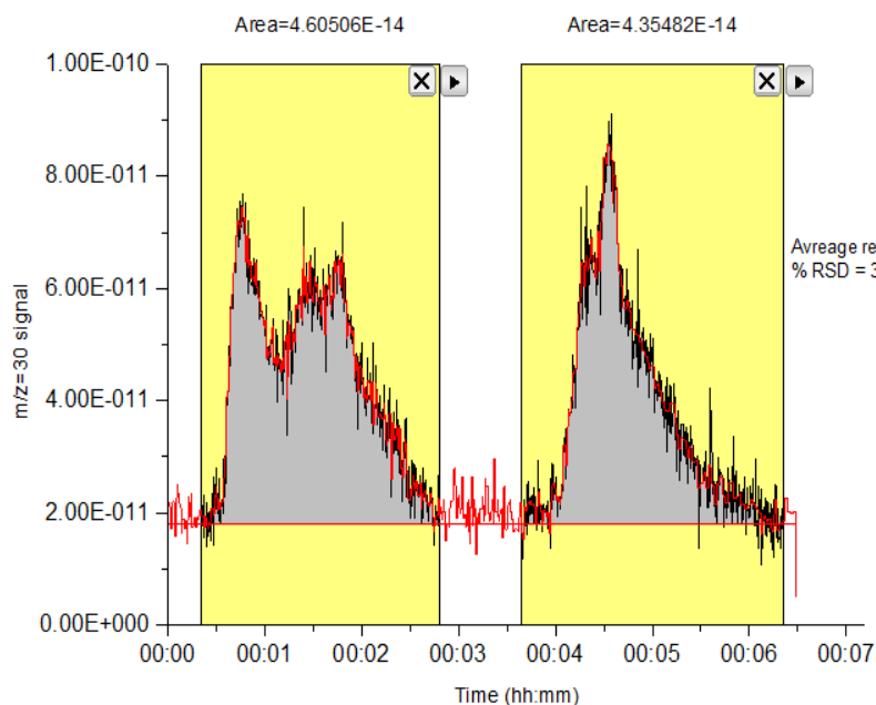
Figure A. 25: Integrated area of the m/z = 30 signal curve of HTCO analysis of 40 mg glutamic acid over 5 % wt Fe / Al_2O_3 catalyst sample at 700 °C in the presence of 500 sccm air flow
