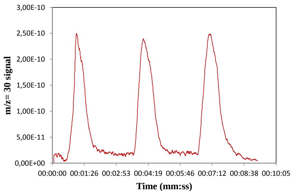
Figure A. 7: The m/z = 30 signal as a function of time of three repetitive HTCO analysis of 60 mg (\text{NH}_4)_2\text{SO}_4 over 1 % wt Pt / \text{Al}_2\text{O}_3 Catalyst Sample at 700 °C in the presence of 500 sccm air flow
