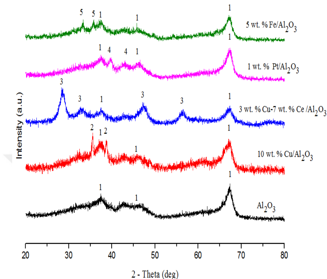
Figure 4. 1: XRD patterns of \text{Al}_2\text{O}_3 support and catalyst samples that are calcined at 700 °C under air flow (lines (1) attributed to \gamma\text{-Al}_2\text{O}_3 , lines (2) attributed to CuO, lines (3) attributed to \text{CeO}_2 , lines (4) attributed to Pt, lines (5) attributed to \alpha\text{-Fe}_2\text{O}_3 )
