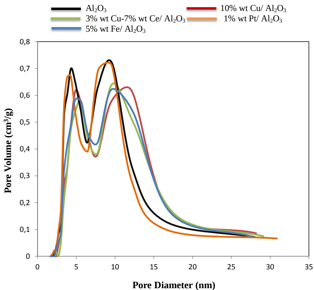
Figure 4. 3: Pore size distribution of \text{Al}_2\text{O}_3 support and catalyst samples
