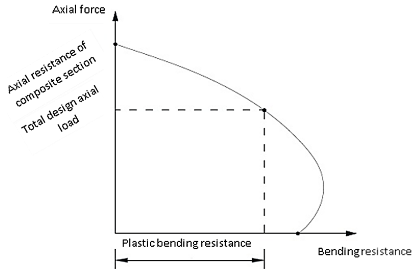
Figure 2.6 Interaction curve for combined compression and bending (Liew and Xiong, 2015)
