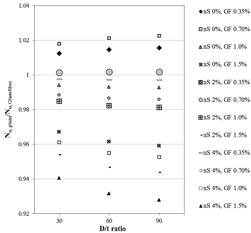
Figure 5.19 Effect of using GF on N_{u, DL/T} of the composite columns tested at 28 days for f_y of a) 185 MPa, b) 275 MPa and c) 450 MPa
