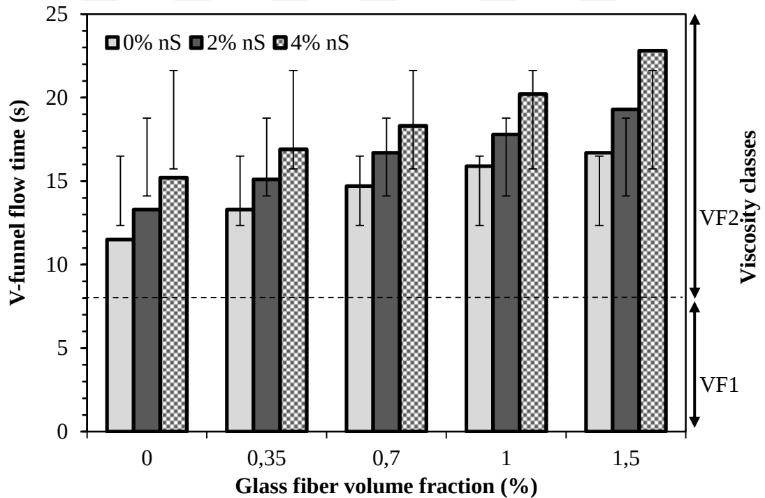
Figure 4.4 Variation of V-funnel flow time
