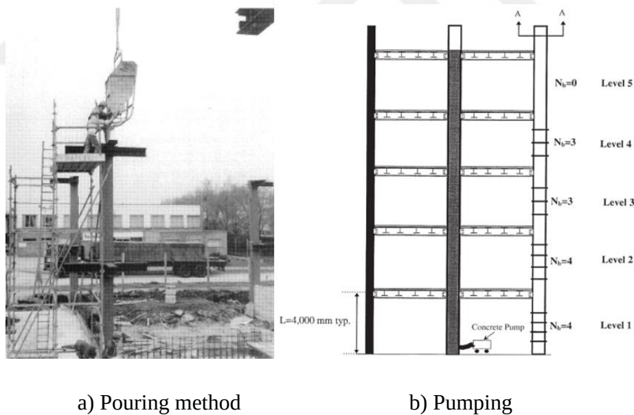
Figure 2.9 Procedure of filling concrete on site of CFST columns (Bergmann et al., 1995; Uy and Das, 1999)
