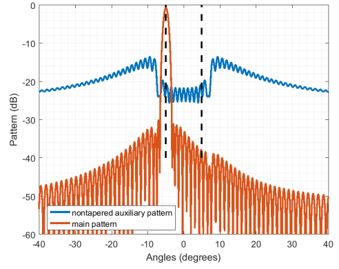
(d) Beamspace main and auxiliary patterns vs angles when D = 16
