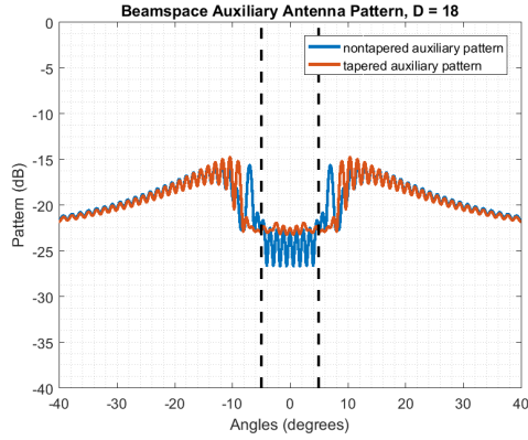
(e) Beamspace auxiliary patterns vs angles when D = 18
