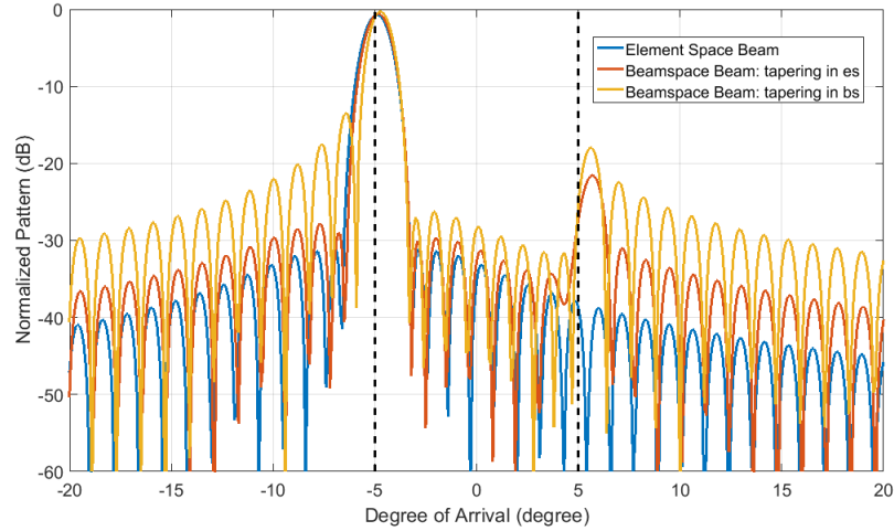
Figure 4.4: Receiver patterns of tapering methods, \phi_s is taken as -5^\circ .
