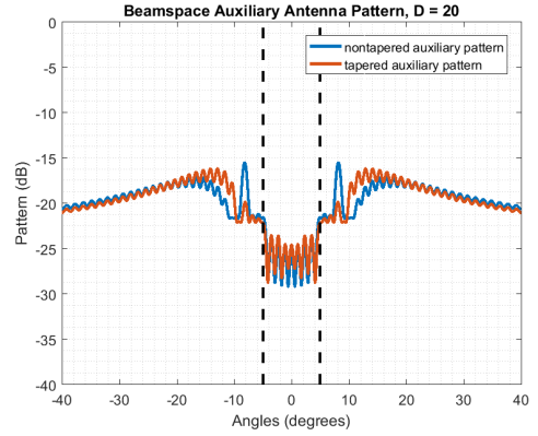
(f) Beamspace auxiliary patterns vs angles when D = 20
