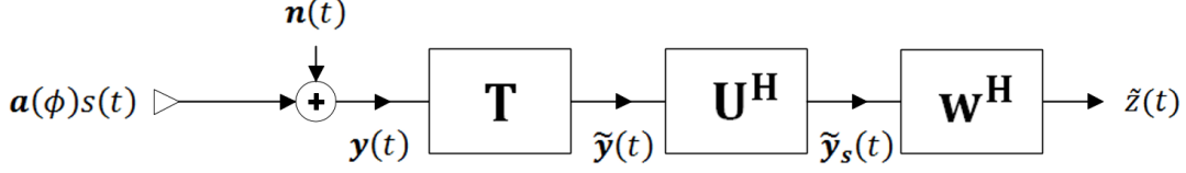
Figure 4.1: Processing chain for tapering before dimension reduction
