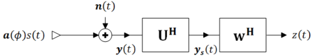
Figure 3.10: Processing chain of the beamspace beamforming.
