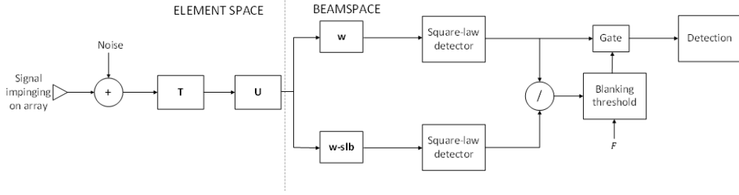
Figure 5.15: Sidelobe blanking structure in tapered beamspace.
