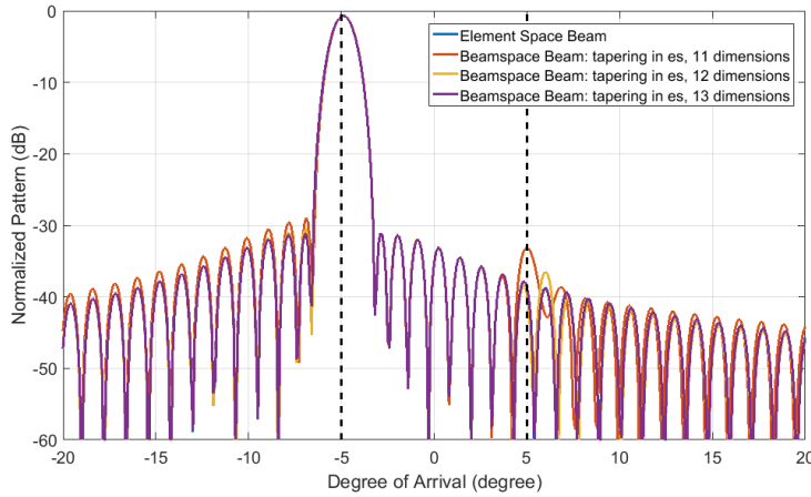
Figure 4.5: Receiver patterns of the tapering before dimension reduction method, \phi_s is taken as -5^\circ .
