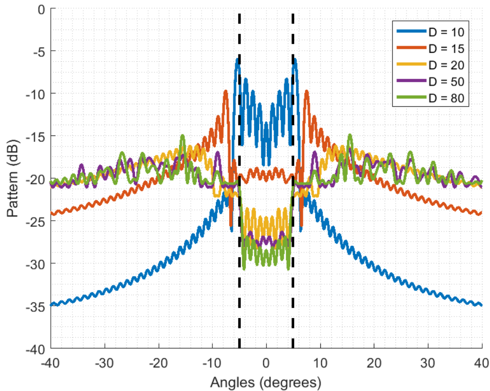
Figure 5.17: Designed auxiliary patterns in tapered beamspace for various number of dimensions.
