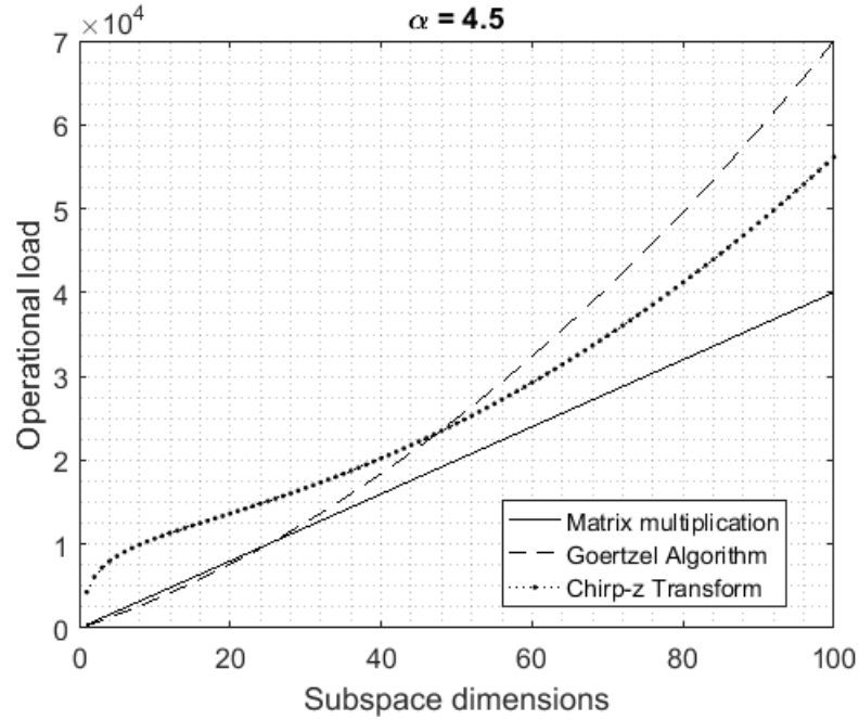
Figure 3.8: Computational complexity for DFT and eigenvector beamformers with orthogonalization process in beamspace.
