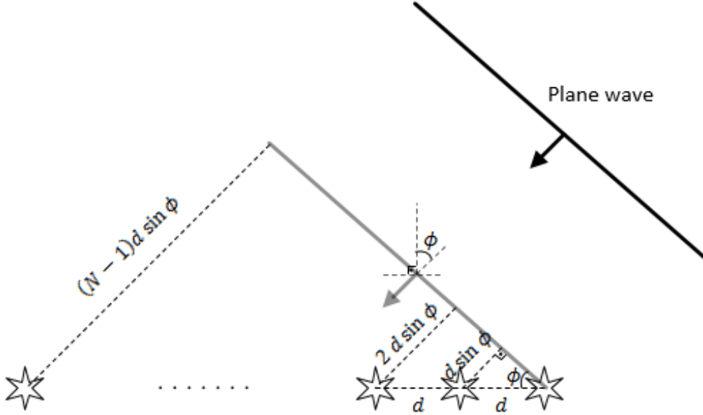
Figure 2.1: ULA with N elements.
