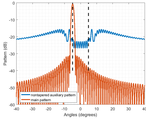
(e) Beamspace main and auxiliary patterns vs angles when D = 18
