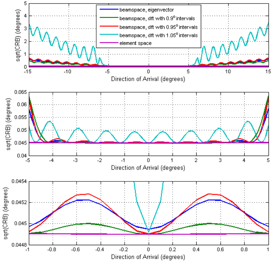
Figure 3.12: CRB analyses of the beamspace methods versus direction of arrival for SNR = 20 dB.
