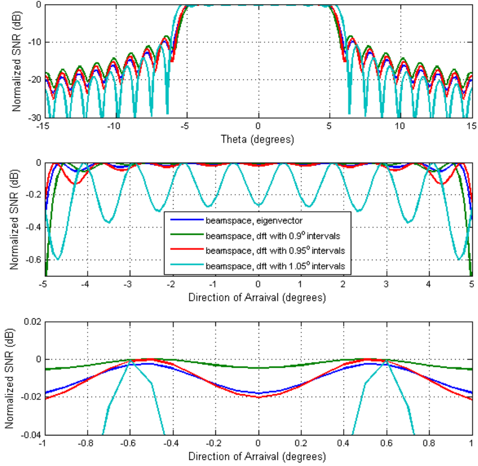
Figure 3.11: SNR performances of beamspace methods versus direction of arrival.
