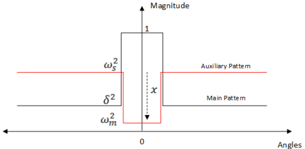
Figure 5.3: Proposed auxiliary channel pattern and main channel pattern.
