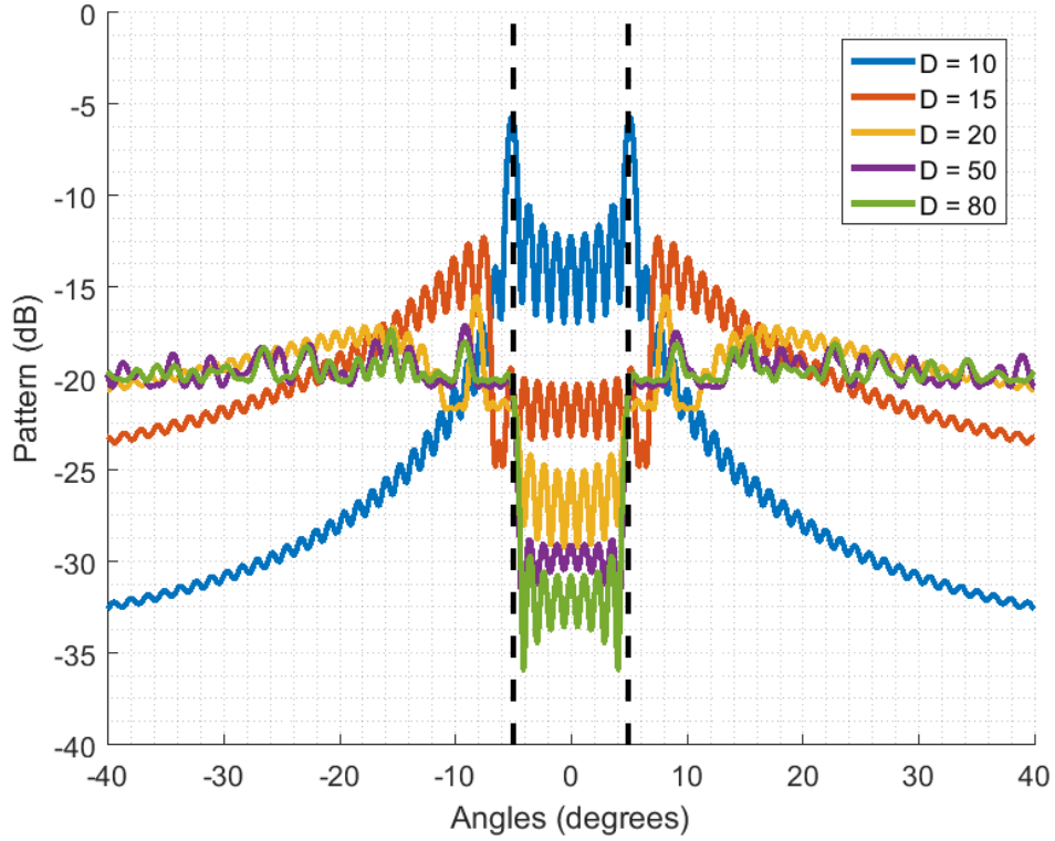
Figure 5.14: Designed auxiliary pattern in beamspace for various dimensions.
