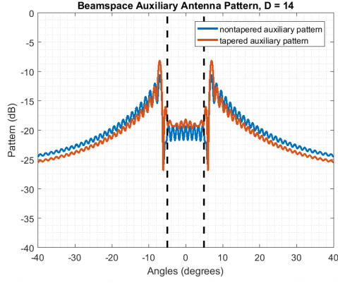
(c) Beamspace auxiliary patterns vs angles when D = 14
