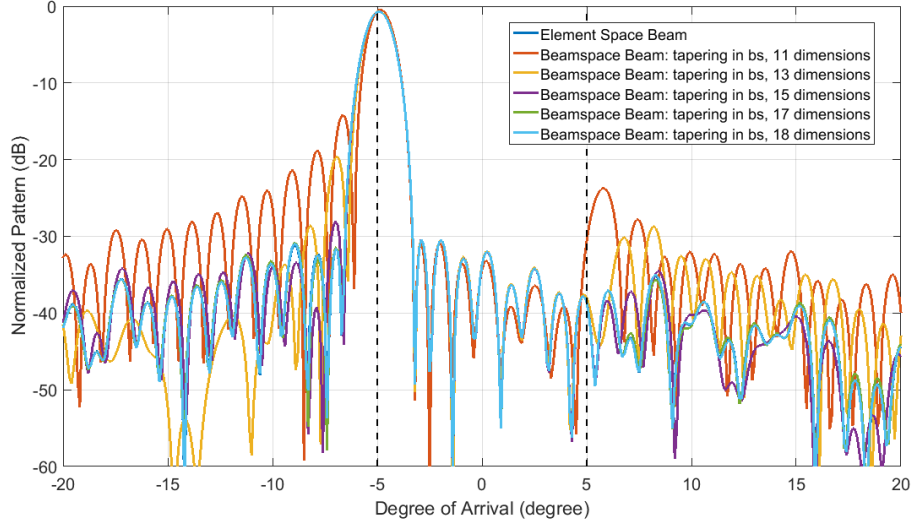
Figure 4.9: Receiver pattern of the tapering after dimension reduction method with random phase errors, \phi_s is taken as -5^\circ .
