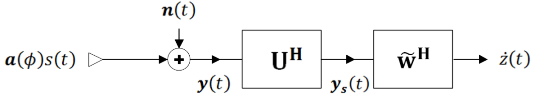
Figure 4.2: Processing chain of the tapering after dimension reduction method
