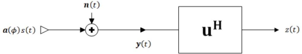
Figure 3.4: The spatial filtering operation
