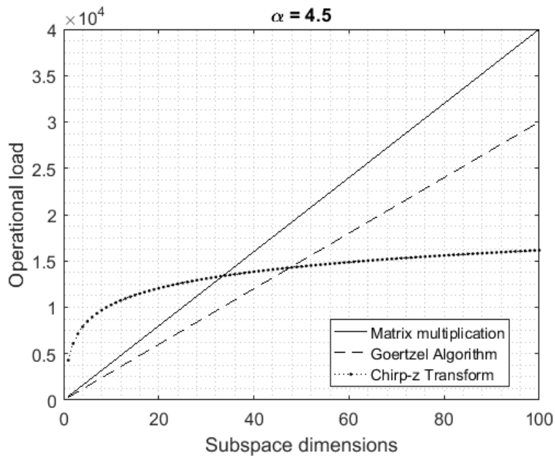
Figure 3.7: Computational complexity for DFT and eigenvector beamformers.
