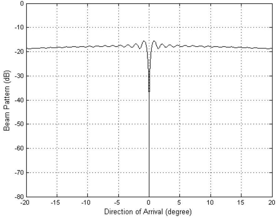
Figure 3.6: Beamspace beam pattern for the 2nd column of beamspace matrix.
