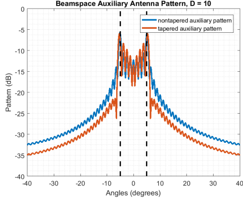
(a) Beamspace auxiliary patterns vs angles when D = 10
