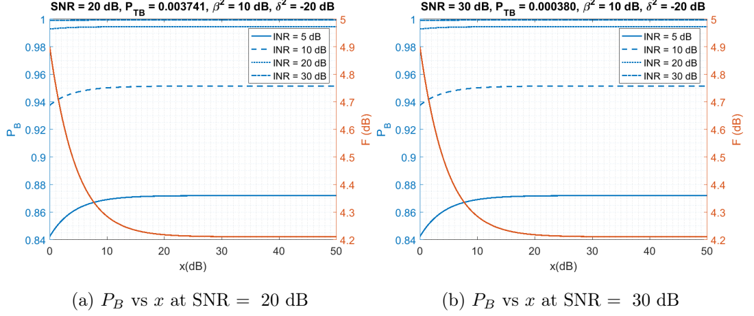
Figure 5.7: Probability of blanking, P_B , as a function of x for various INR. Left y-axis denotes the probability of blanking, P_B , and the right y-axis indicates the threshold values for the same x-axis.
