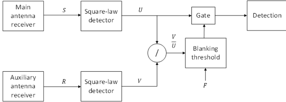
Figure 5.2: Basic sidelobe blanking system.
