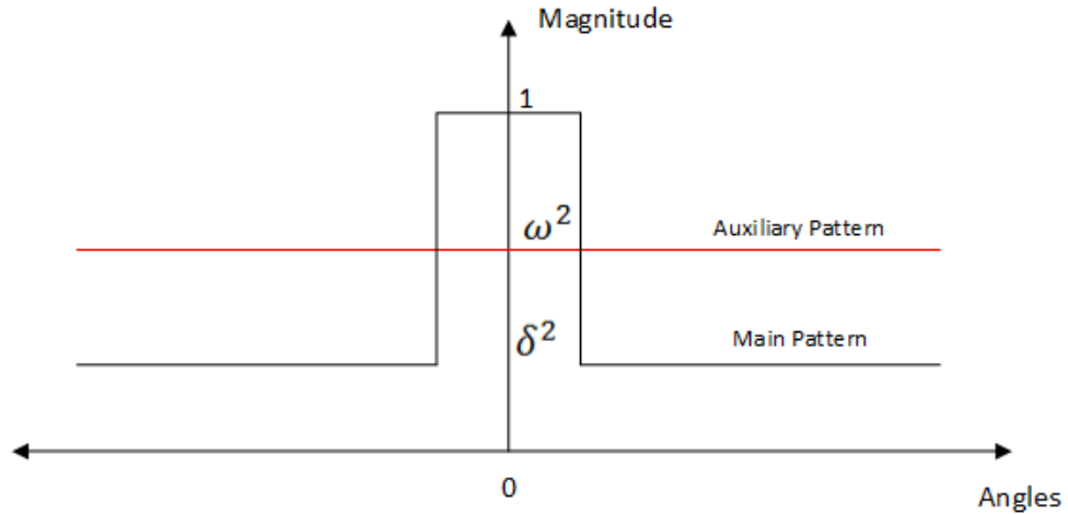
Figure 5.1: Ideal main and auxiliary pattern proposed by Maisel.
