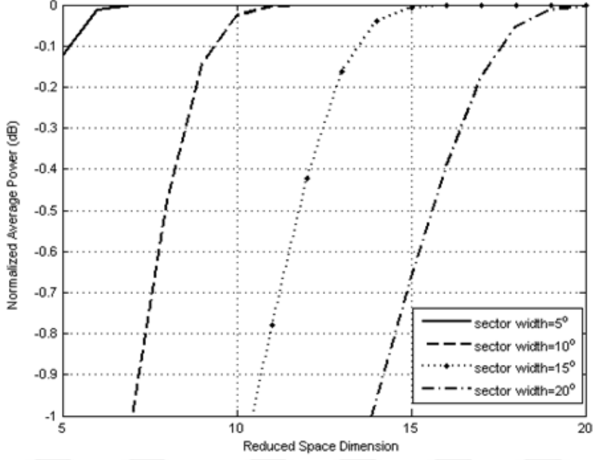
Figure 3.9: Average power for different sector widths and reduced space dimensions.
