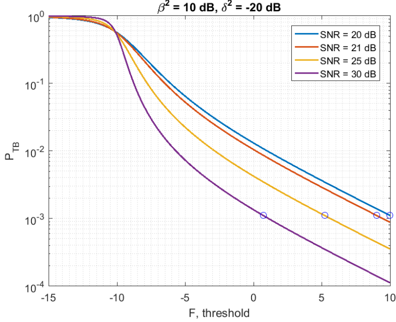
Figure 5.4: Probability of target blanking, P_{TB} , as a function of threshold, F .
