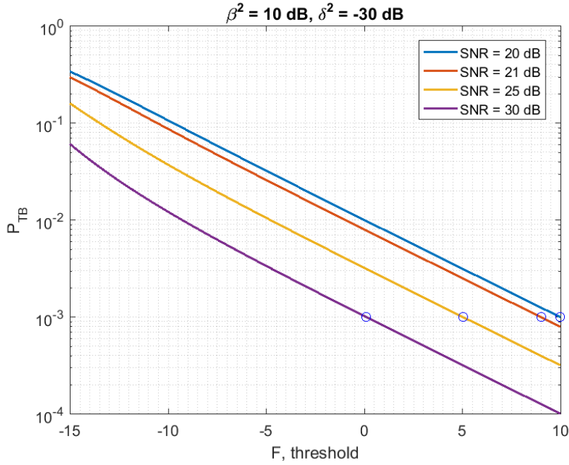
Figure 5.9: Probability of target blanking, P_{TB} , as a function of threshold, F .
