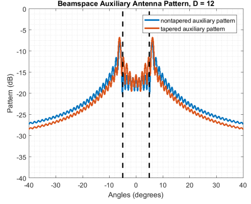
(b) Beamspace auxiliary patterns vs angles when D = 12
