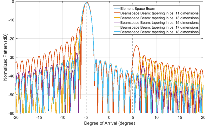
Figure 4.6: Receiver pattern of the tapering after dimension reduction method, \phi_s is taken as -5^\circ .
