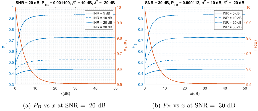
Figure 5.6: Probability of blanking, P_B , as a function of x for various INR. Left y-axis denotes the probability of blanking, P_B , and the right y-axis indicates the threshold values for the same x-axes.
