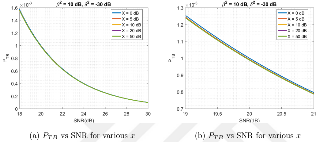
Figure 5.11: Probability of target blanking, P_{TB} , as a function of SNR, F .
