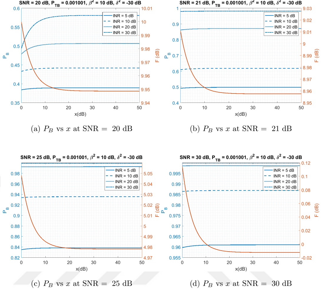
Figure 5.10: Probability of blanking, P_B , as a function of x for various INR. Left y-axes denotes the probability of blanking, P_B , and the right y-axes indicates the threshold values for the same x-axes.
