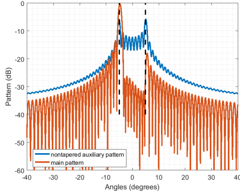
(a) Beamspace main and auxiliary patterns vs angles when D = 10
