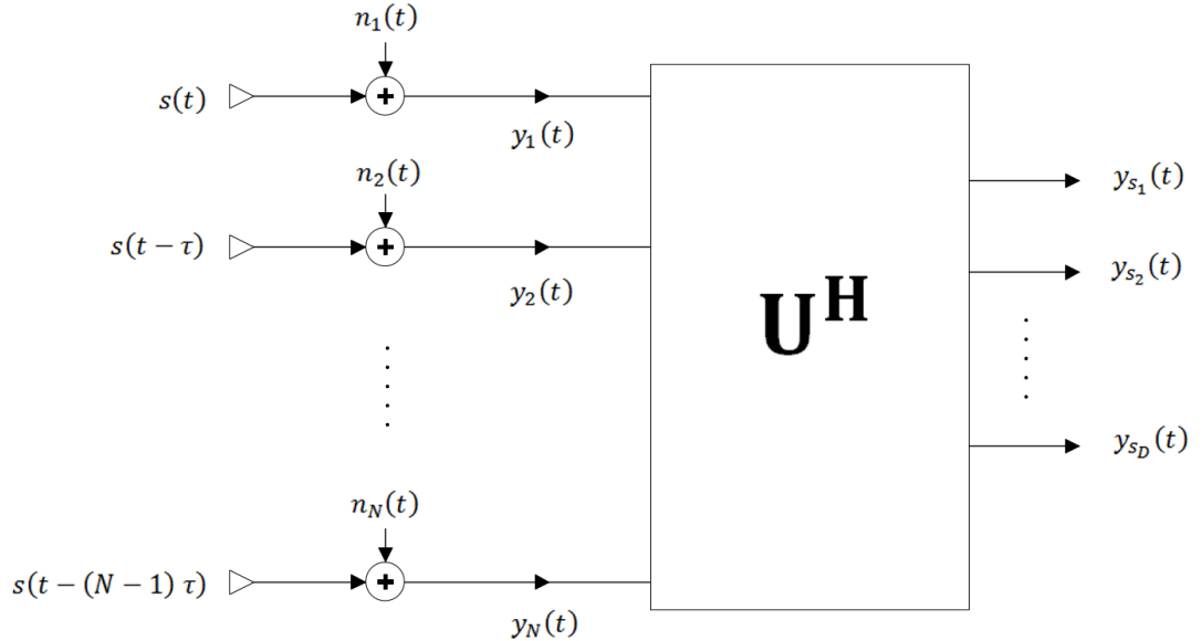
Figure 3.1: Beamspace processing chain.
