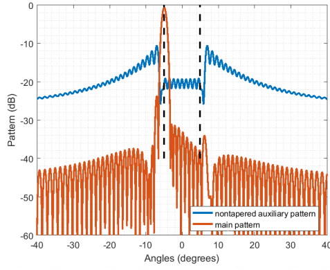
(c) Beamspace main and auxiliary patterns vs angles when D = 14
