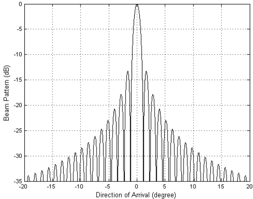
Figure 3.5: The first beamspace beam pattern of the array.
