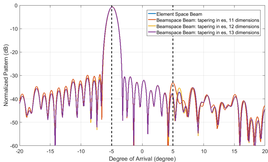
Figure 4.8: Receiver pattern of the tapering before dimension reduction method with random phase errors, \phi_s is taken as -5^\circ .
