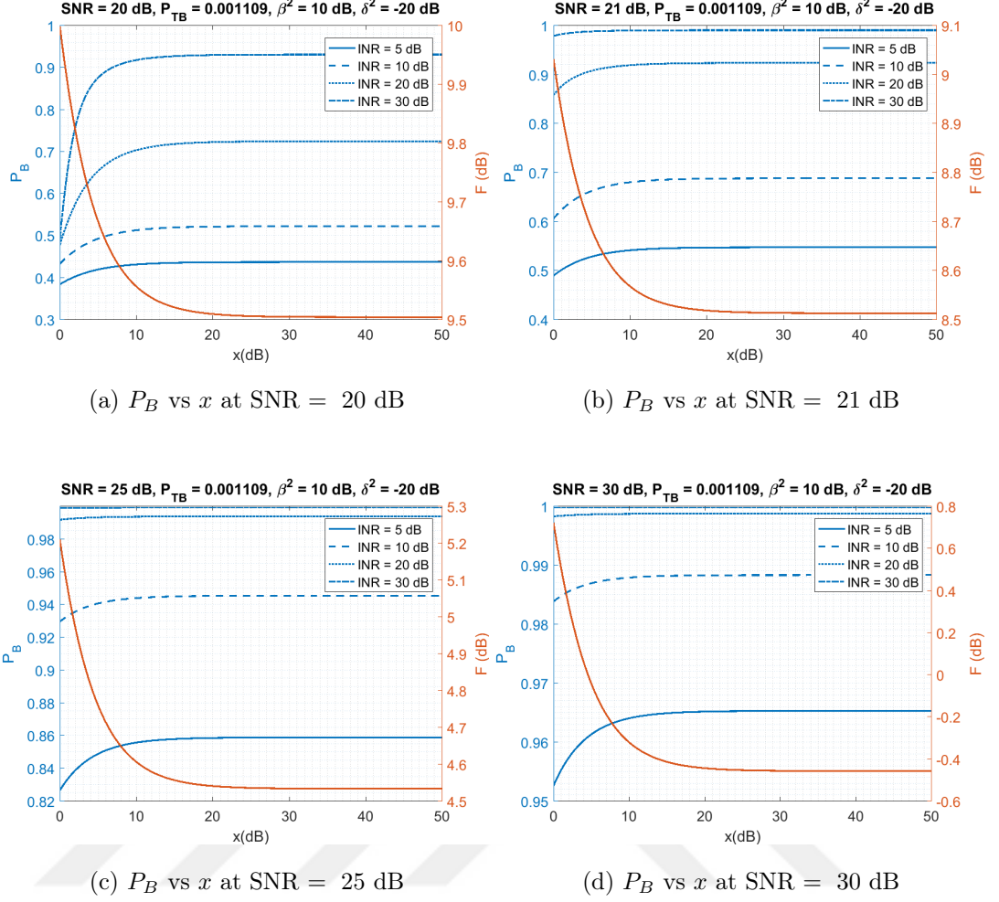
Figure 5.5: Probability of blanking, P_B , as a function of x for various INR. Left y-axes denotes the probability of blanking, P_B , and the right y-axes indicates the threshold values for the same x-axes.
