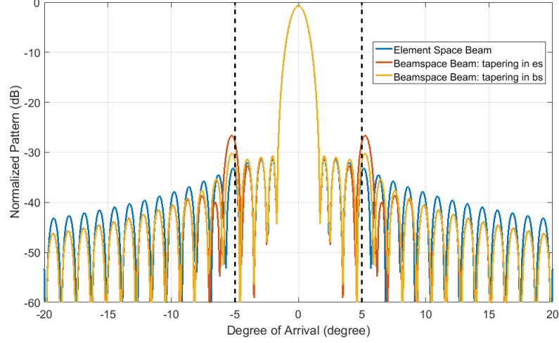
Figure 4.3: Receiver patterns of the tapering methods, \phi_s is taken as 0^\circ .
