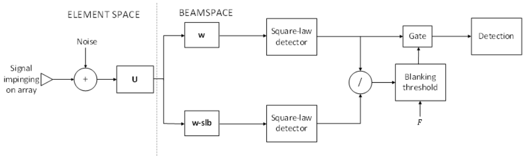
Figure 5.12: Sidelobe blanking structure in beamspace.
