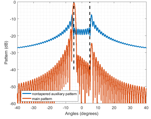
(b) Beamspace main and auxiliary patterns vs angles when D = 12
