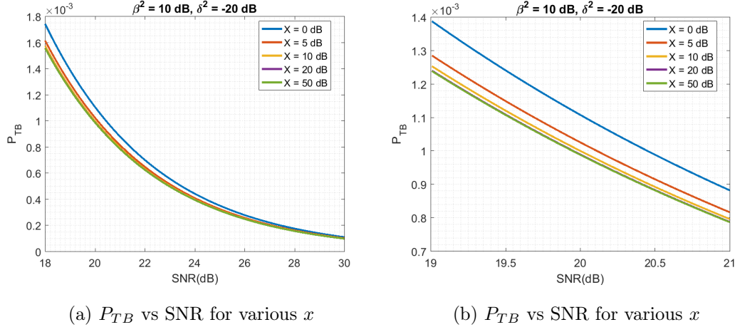
Figure 5.8: Probability of target blanking, P_{TB} , as a function of SNR, F .
