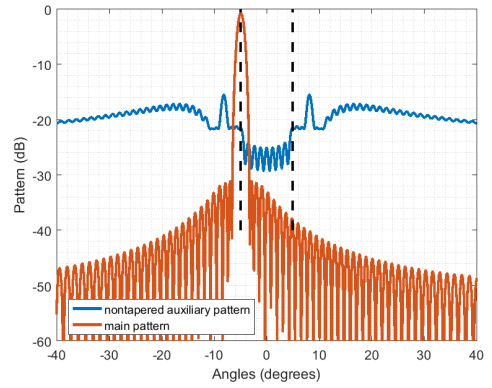
(f) Beamspace main and auxiliary patterns vs angles when D = 20
