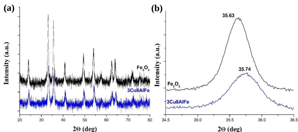
Figure 6.18. XRD diffractograms of Fe 2 O 3 and supported 3Cu8AlFe catalysts calcined at 400 °C and taken under ambient conditions as a function of 2 \Theta (a) full scan and (b) Fe 2 O 3 (110) peak
