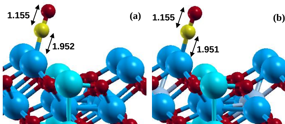
Figure 5.9. CO adsorption on the (a) Fe oct 2 terminated and the (b) Fe oct 2_Cr_ooa terminated Fe 3 O 4 (111) surface. The bond length unit is angstrom. (Fe tet : light blue, Fe oct : blue, O: red, Cr: gray, C: yellow)
