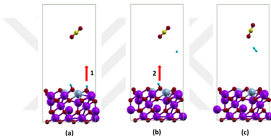
Figure 4.8. Hydrogen atom desorption for Ooct2Cr termination (a) desorption of first hydrogen atom (b) desorption of second hydrogen atom (c) final geometry (Fe: purple, O: red, Cr: gray C: yellow, H: blue)
