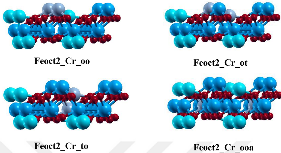
Figure 5.3. Initial structures of differently located Cr atoms in \text{Fe}_{\text{oct}2} structure (Fe tet : light blue, Fe oct : blue, O: red, Cr: gray)
