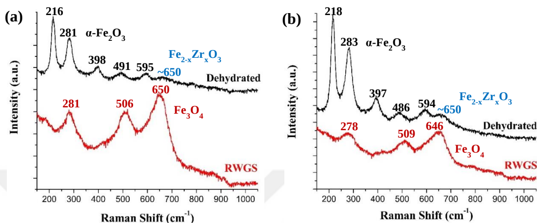
Figure 6.4. The in situ Raman spectra of (a) 8ZrFe and (b) supported 3Cu/8ZrFe catalysts under dehydration in 10% O 2 /Ar and RWGS reaction conditions (30 mL/min 5%CO 2 /Ar and 15 mL/min 10%H 2 /Ar) at 400 °C
