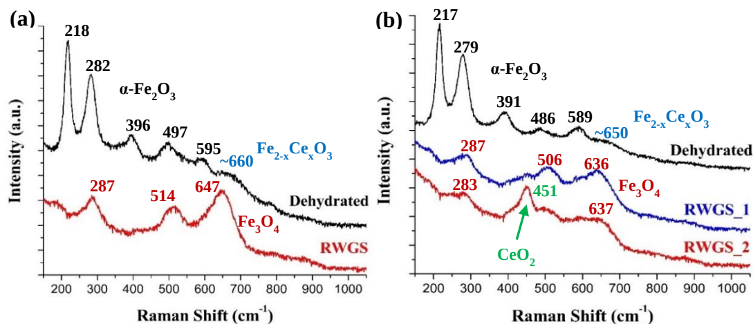
Figure 6.14. The in situ Raman spectra of (a) 8CeFe and (b) 3Cu/8CeFe catalysts under dehydration in 10% O 2 /Ar and RWGS reaction conditions (30 mL/min 5%CO 2 /Ar and 15 mL/min 10%H 2 /Ar) at 400 °C. RWGS_1 and RWGS_2 signify spectral collection from different points.
