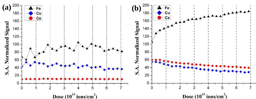
Figure 6.15. The BET surface area normalized HS-LEIS Fe, Ce, and Cu Atomic density of both (a) dehydrated, calcined and (b) activated supported 3Cu/8CeFe catalyst with the 5keV Ne ^+ dose. The vertical dashed lines indicate doses of n(1 \times 10^{15} ions/cm ^2 ), with n=1,2,3 , etc., that correspond to removal of a monolayer-equivalents from the catalyst 149
