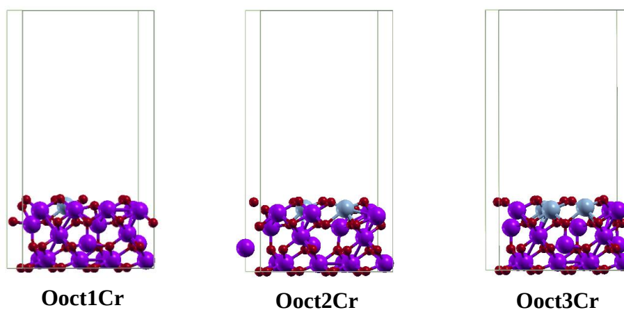
Figure 4.3. Possible chromium substitution with iron atoms on O_{oct1} termination of Fe_3O_4 (111) surface (Fe: purple, O: red, Cr: gray)
