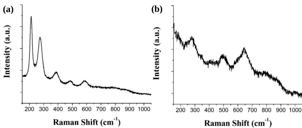
Figure A.1. In situ Raman (442nm) spectra of calcined unpromoted iron oxide catalyst at 400 °C: (a) reoxidized in 10% \text{O}_2/\text{Ar} and (b) RWGS reaction conditions (2 nd time, (30 mL/min 5% \text{CO}_2/\text{Ar} and 15 mL/min 10% \text{H}_2/\text{Ar} ))
