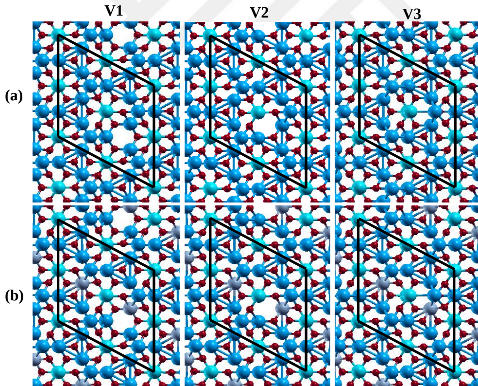
Figure 5.6. Top view of the schematic representation of the (111) surface after relaxation: (raw a) Fe oct2 and (raw b) Fe oct2 _Cr_oaa surface (Fe tet : light blue, Fe oct : blue, O: red, Cr: gray)
