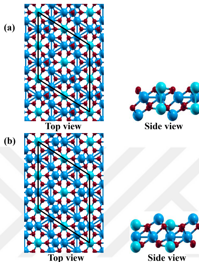
Figure 5.2. Optimized structures of (a) \text{Fe}_{\text{tet}1} and (b) \text{Fe}_{\text{oct}2} terminations ( \text{Fe}_{\text{tet}} : light blue, \text{Fe}_{\text{oct}} : blue, O: red)
