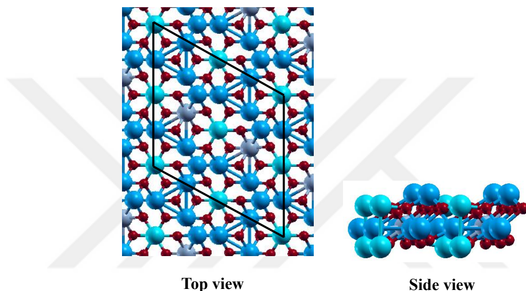
Figure 5.4. Optimized structure of Feoct2_Cr_oaa surface (Fe tet : light blue, Fe oct : blue, O: red, Cr: gray)
