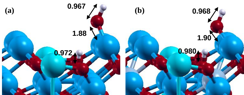
Figure 5.8. H 2 O adsorption on the (a) Fe oct2 terminated and the (b) Feoct2_Cr_ooa terminated Fe 3 O 4 (111) surface. The bond length unit is angstrom. (Fe tet : light blue, Fe oct : blue, O: red, Cr: gray, H: white)
