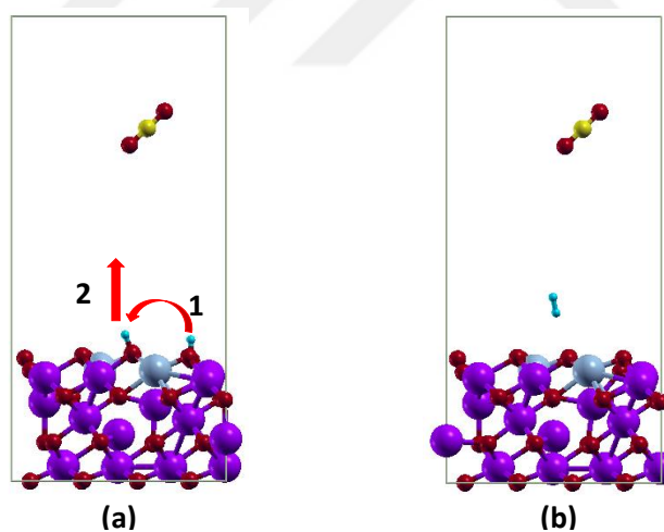
Figure 4.7. Direct hydrogen-hydrogen interaction for Ooct2Cr termination (a) initial geometry (b) final geometry (Fe: purple, O: red, Cr: gray, C: yellow, H: blue)
