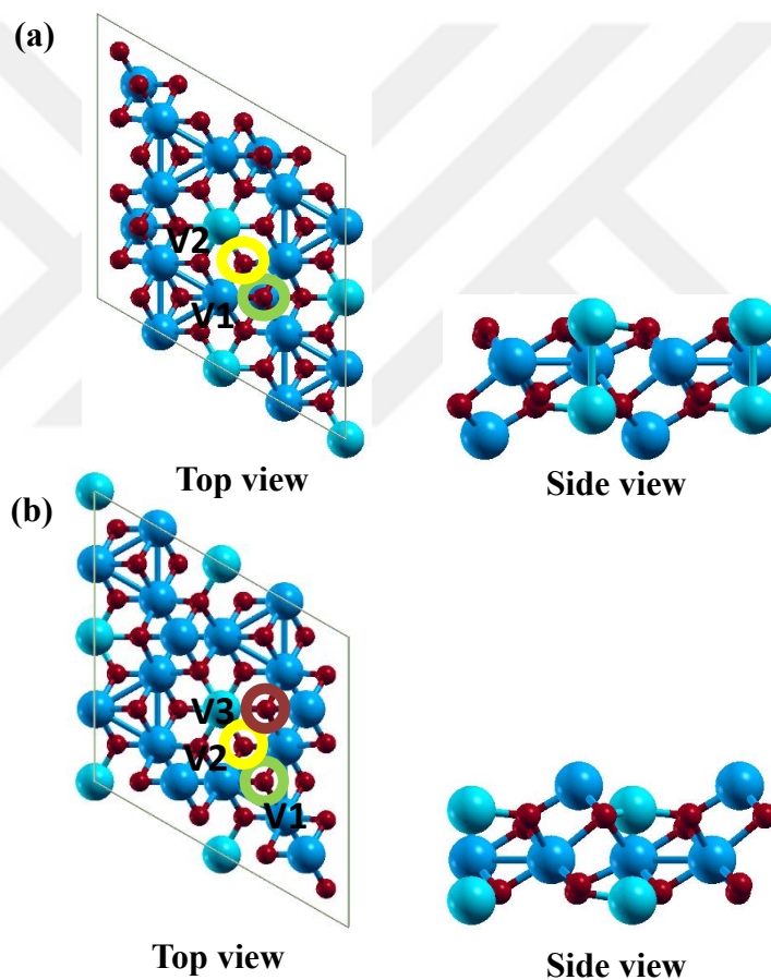
Figure 5.5. Possible oxygen sites on (a) Fe tet1 surface and (b) Fe oct2 surface (Fe tet : light blue, Fe oct : blue, O: red)
