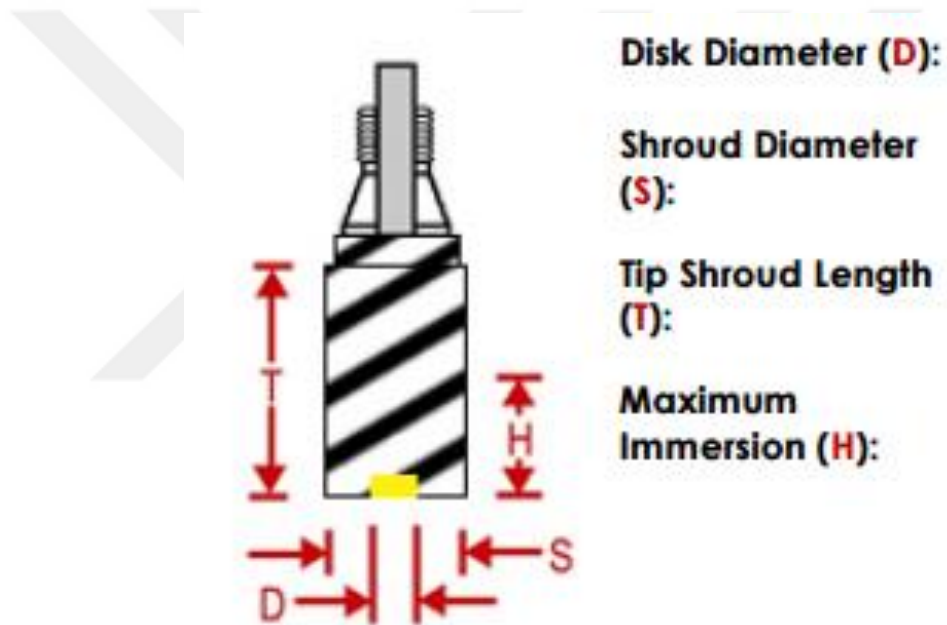
Figure 3.3 The schematic of Pt-RDE [51]
