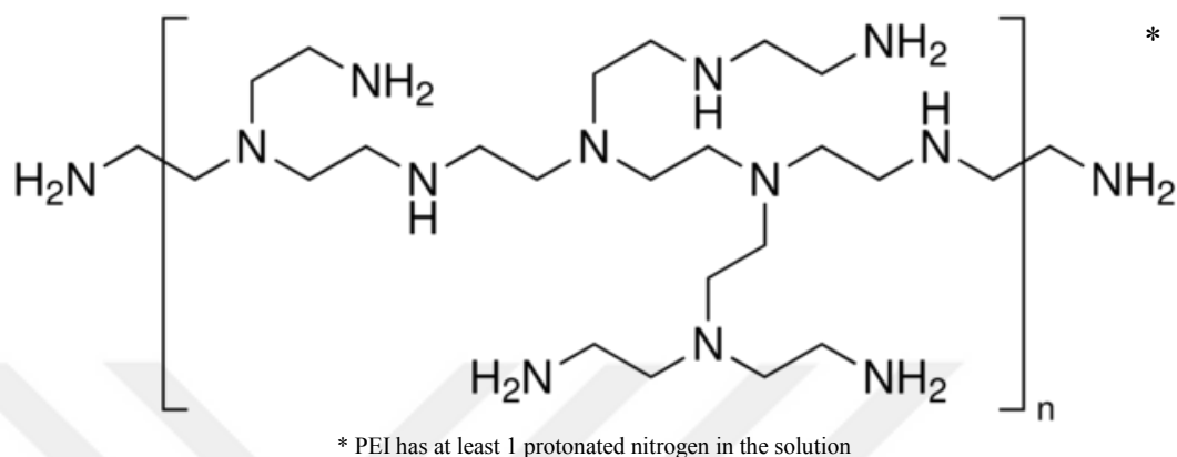
Figure 2.3 The chemical structure of PEI [31]
