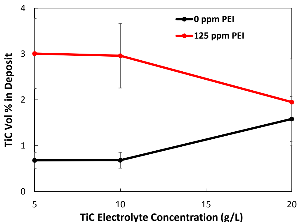
Figure 4.8 TiC vol.% in the deposit for different TiC electrolyte concentrations in a Watts bath containing 0 and 125 ppm PEI at a current density of -50 mA cm -2 . The RDE rotation speed is adjusted to 100 rpm for all cases.
