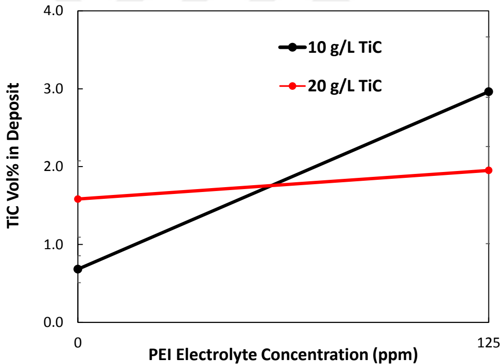
Figure 4.7 TiC vol.% in the deposit for different PEI electrolyte concentrations in a Watts bath containing 10 \text{ g L}^{-1} and 20 \text{ g L}^{-1} TiC at a current density of -50 \text{ mA cm}^{-2} . The rotation speed is adjusted to 100 rpm for all cases.
