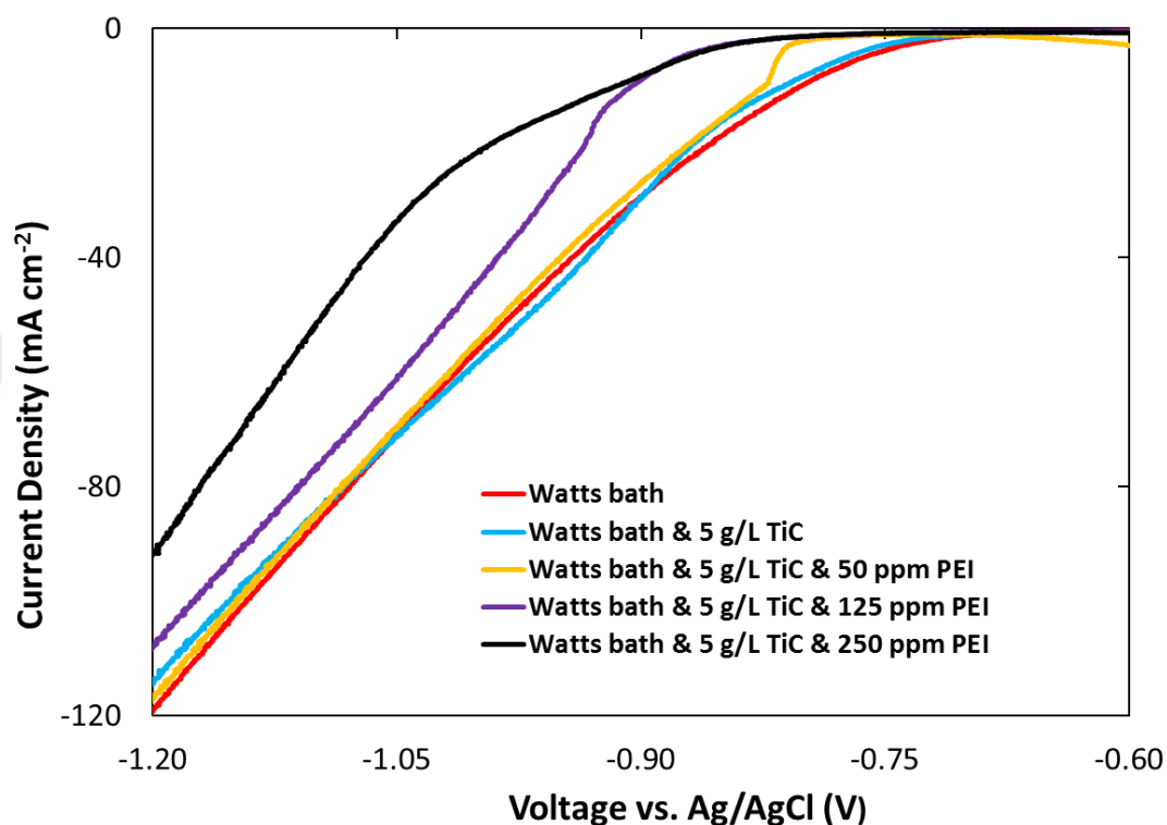
Figure 4.2 Polarization curves for pure Watts solution and Watts solution containing 5 g L -1 TiC and different PEI concentrations. The RDE rotation speed is adjusted to 2500 rpm for all cases.
