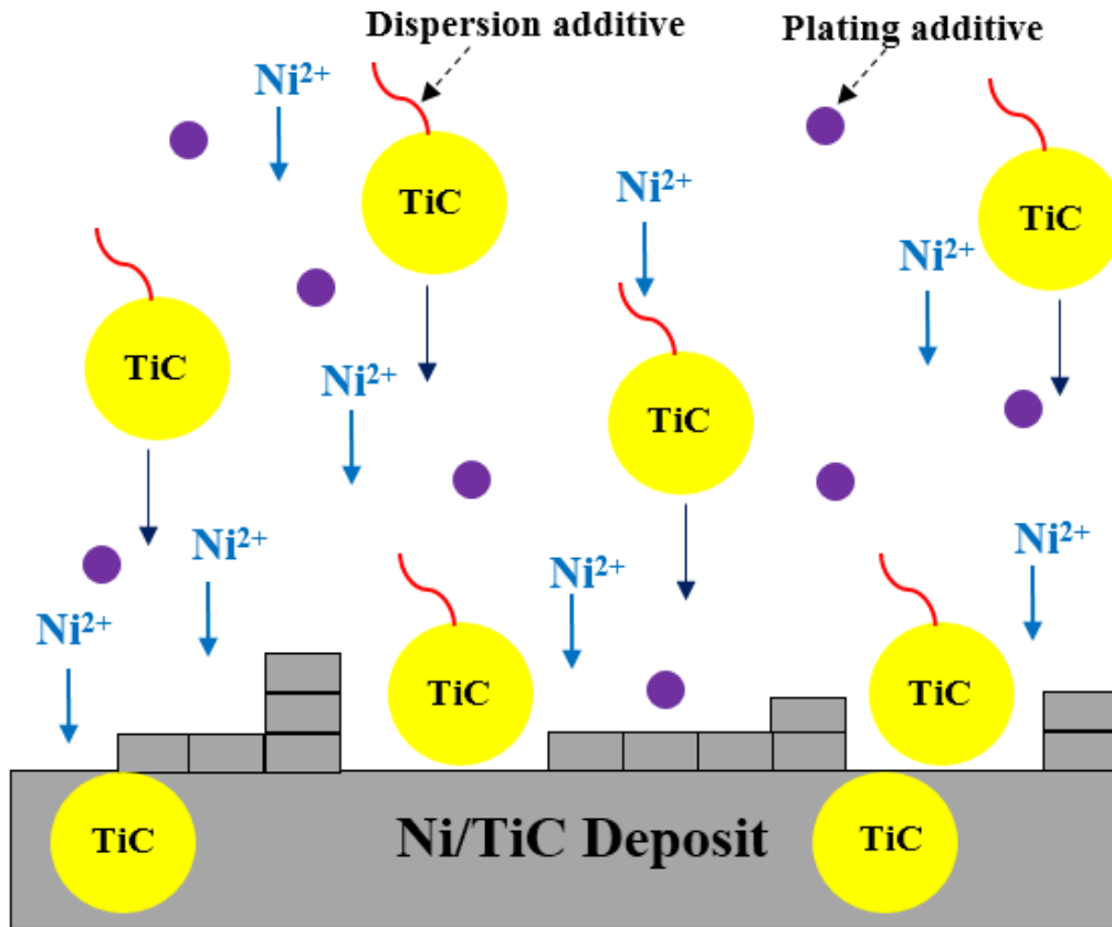
Figure 1.2 Schematic diagram of Ni/TiC electrodeposition (adapted from [5])
