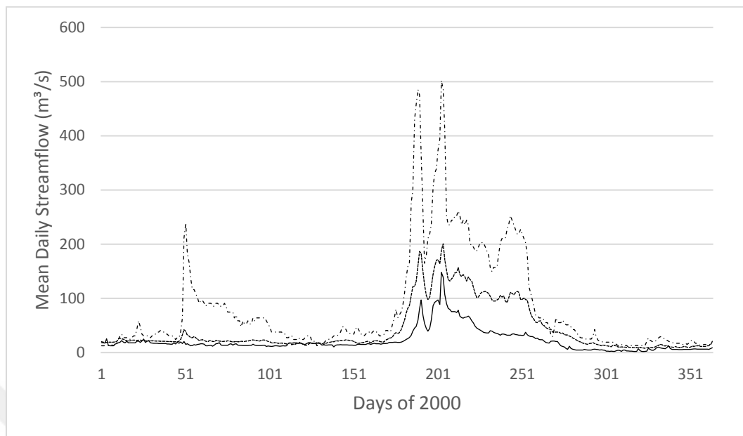
Figure 101: Hydrograph of streamgage 2323
