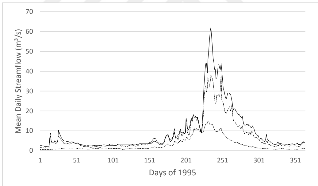
Figure 106: Hydrograph of streamgage 2342
