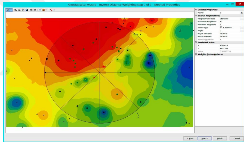
Figure 8: Parameters of IDW
