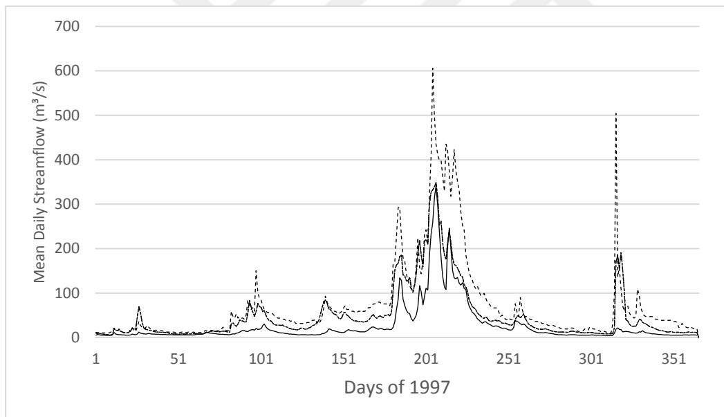
Figure 83: Hydrograph of streamgage 1307
