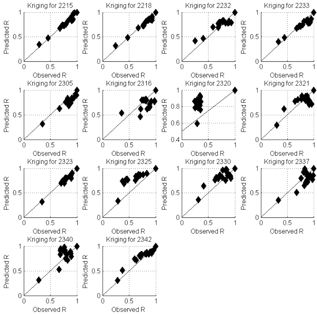
Figure 77: Evaluation of Correlation Estimations with Ordinary Ordinary Kriging for Coruh Region
