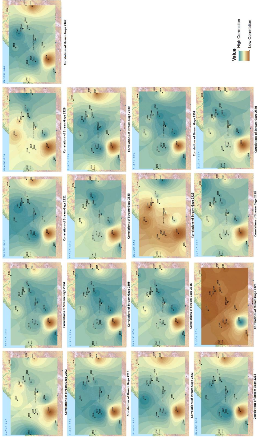
Figure 63: Correlation maps for Coruh Basin where streamgauge number 2218 is assumed to be unengaged (Created with IDW)
