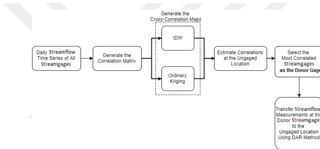
Figure 5: Workflow of MCM (Modified from Ocal and Kentel, 2017)
