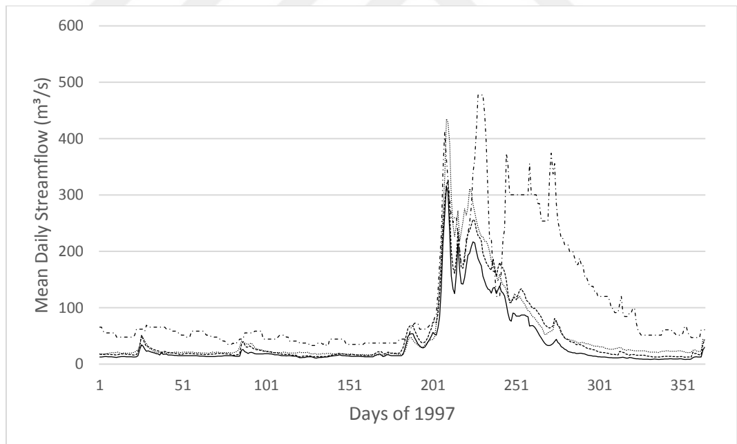
Figure 98: Hydrograph of streamgage 2316
