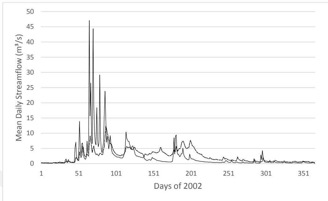
Figure 89: Hydrograph of streamgage 1338
