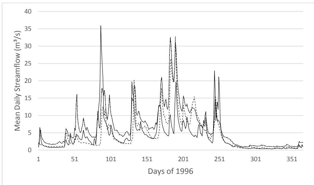
Figure 83: Hydrograph of streamgage 1307
