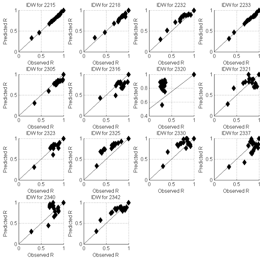
Figure 76: Evaluation of Correlation Estimations with IDW for Coruh Region
