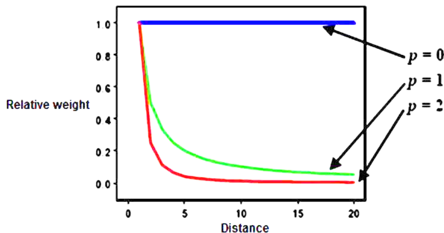
Figure 7: Decrease of weight with distance (ESRI Development Team, 2010)
