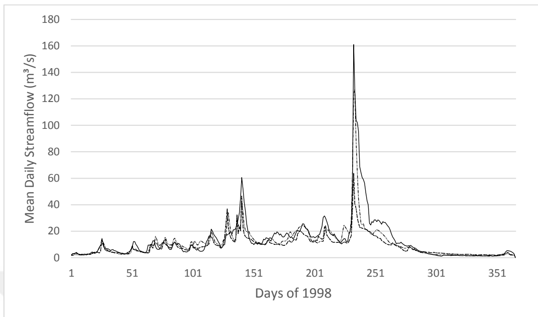
Figure 85: Hydrograph of streamgage 1319
