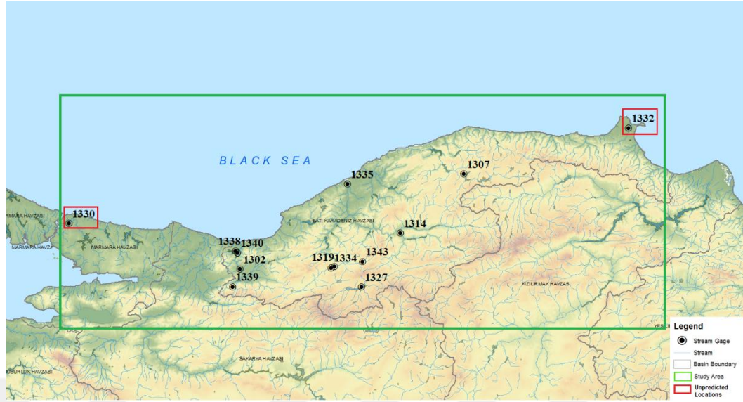
Figure 39: Unpredicted Locations in Western Black Sea Region
