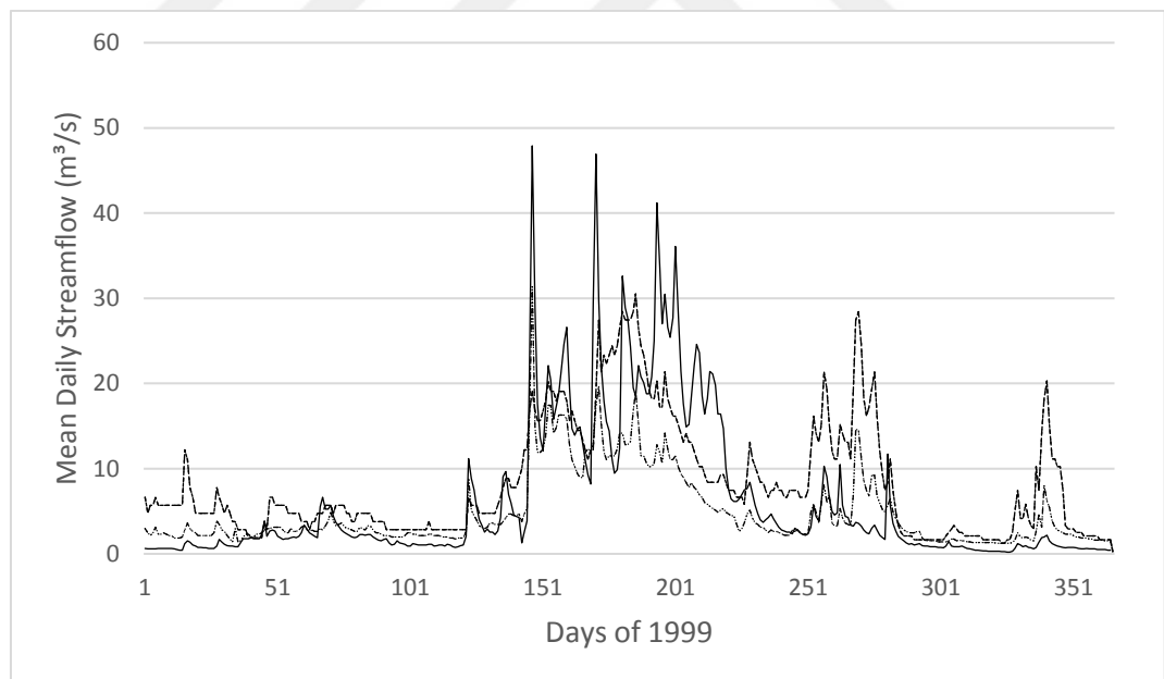
Figure 86: Hydrograph of streamgage 1327
