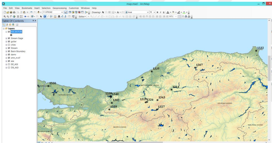
Figure 38: Digital elevation model, streamgages, dams at Western Black Sea Region
