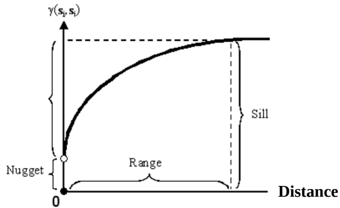
Figure 11: Example of a semi-variogram
