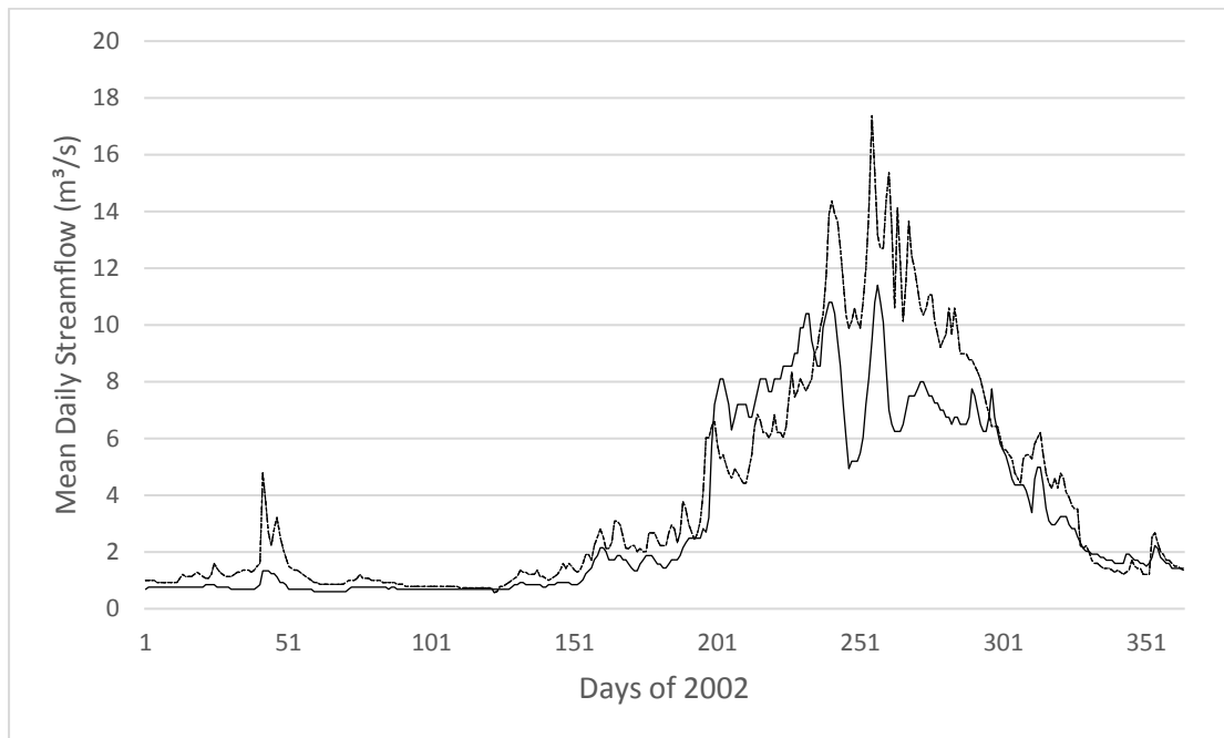
Figure 103: Hydrograph of streamgage 2330
