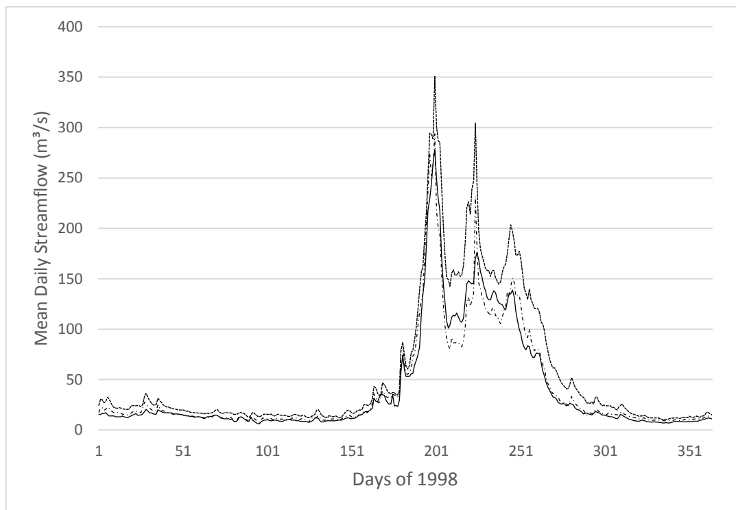
Figure 99: Hydrograph of streamgage 2320
