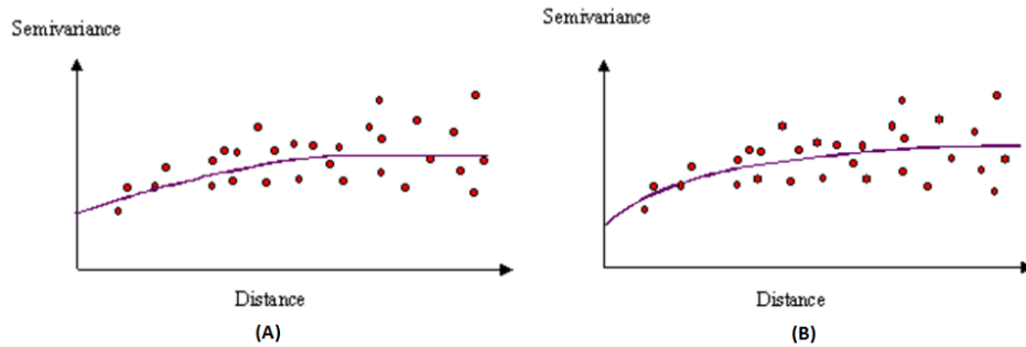
Figure 12: Different types of variogram models. (A) shows a spherical model while (B) shows an exponential model (ESRI Development Team, 2010)
