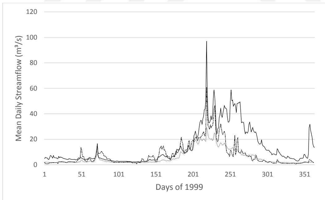
Figure 100: Hydrograph of streamgage 2321
