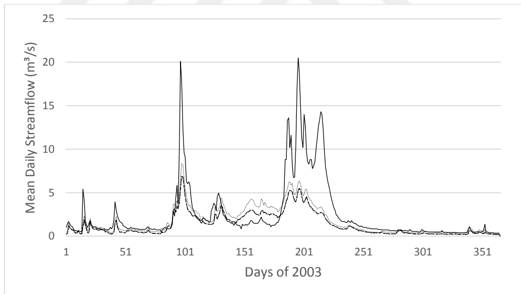
Figure 90: Hydrograph of streamgage 1339
