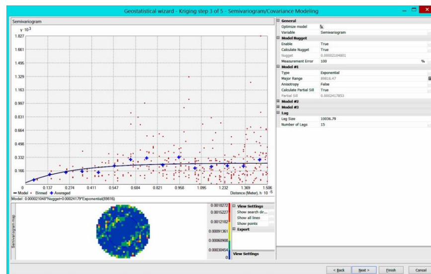
Figure 13: Step 3 - Semivariogram modeling
