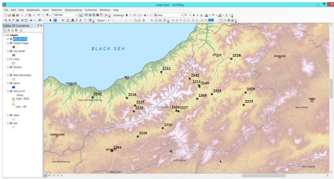
Figure 61: Digital elevation model, streamgages, dams at Coruh Region
