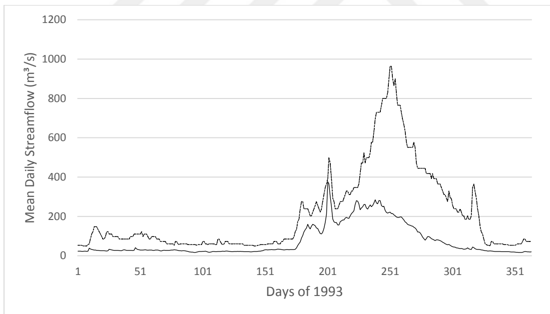
Figure 104: Hydrograph of streamgage 2337
