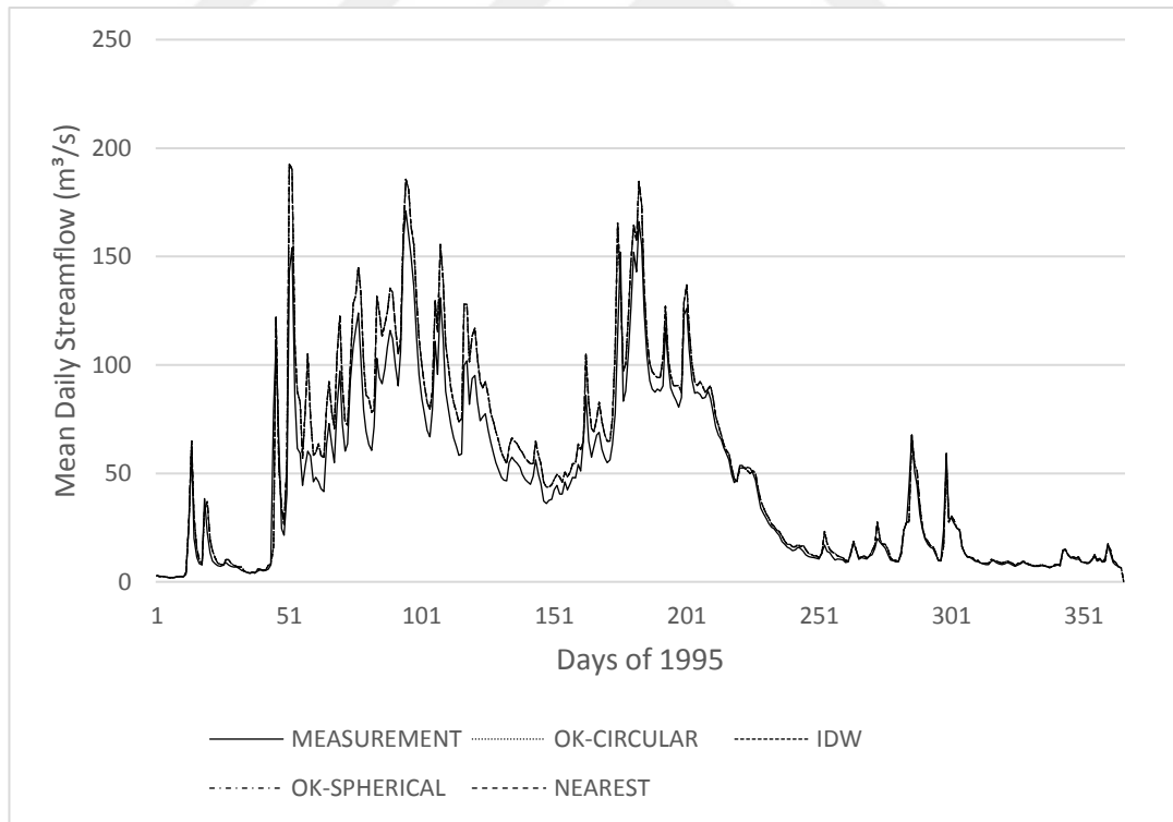
Figure 82: Hydrograph of streamgage 1302
