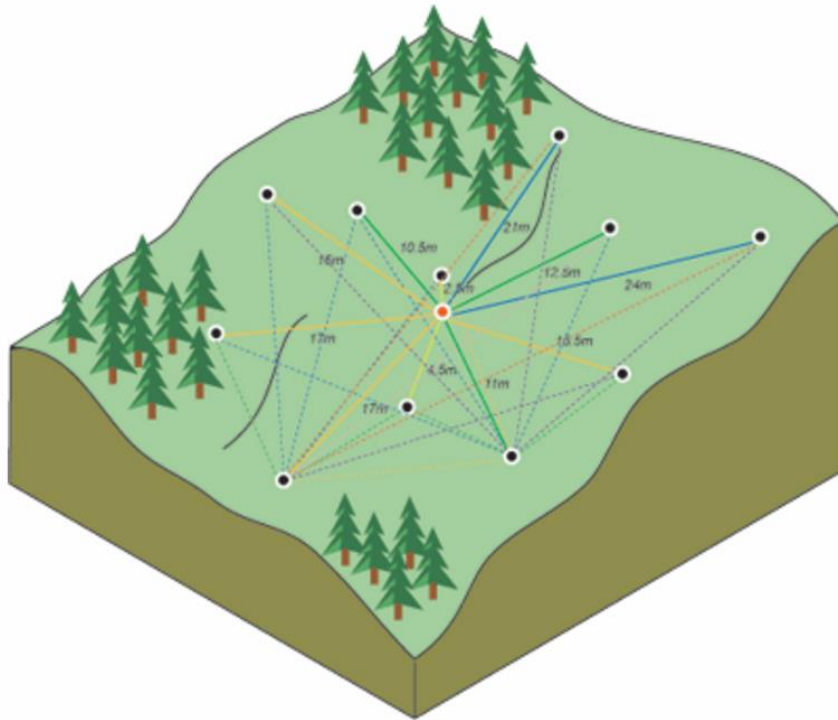
Figure 10: Variogram calculation on sample data. (ESRI Development Team, 2010)
