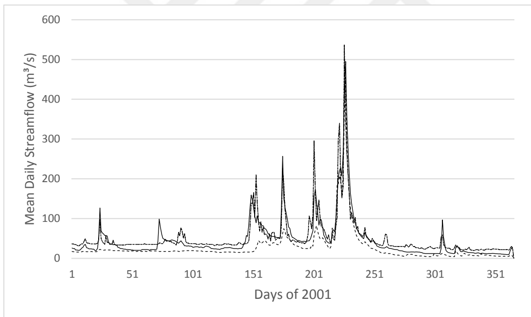
Figure 88: Hydrograph of streamgage 1335
