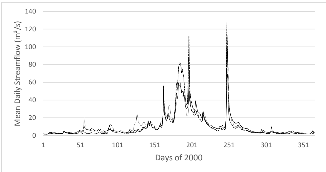
Figure 87: Hydrograph of streamgage 1334
