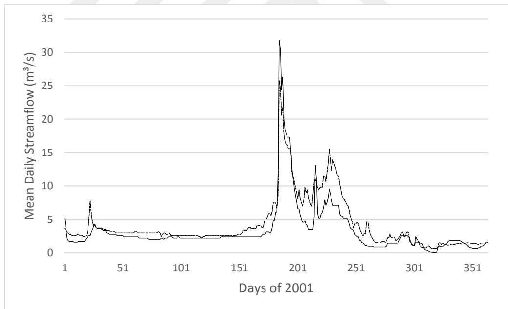
Figure 102: Hydrograph of streamgage 2325
