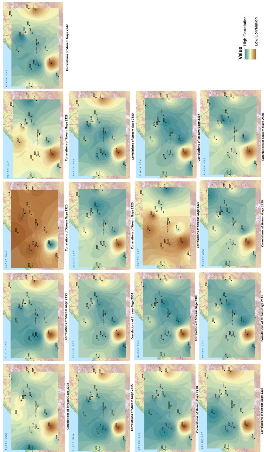
Figure 69: Correlation maps for Coruh Basin where streamgauge number 2321 is assumed to be unengaged (Created with IDW)
