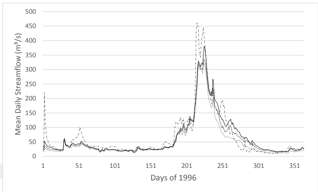
Figure 97: Hydrograph of streamgage 2305
