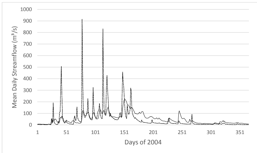
Figure 91: Hydrograph of streamgage 1340
