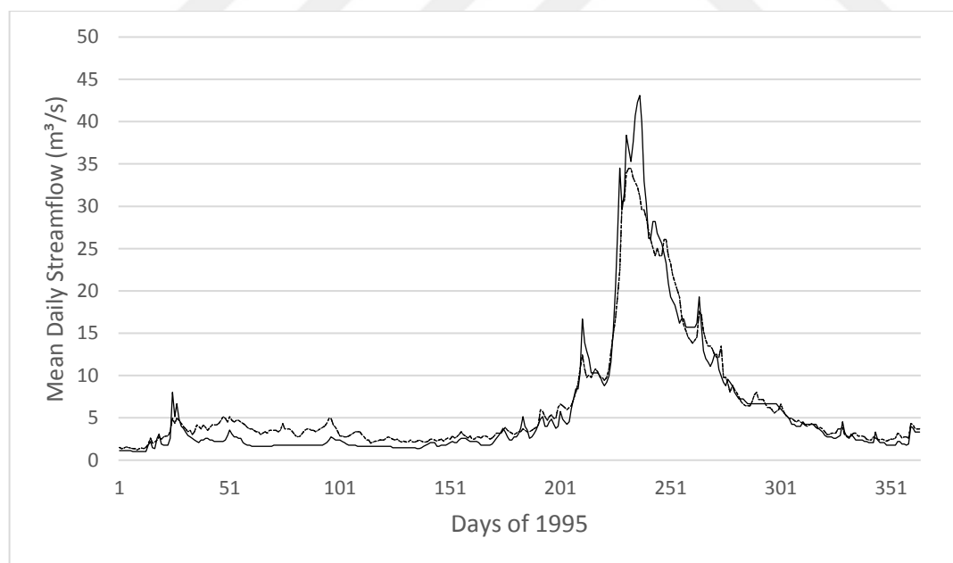
Figure 96: Hydrograph of streamgage 2233
