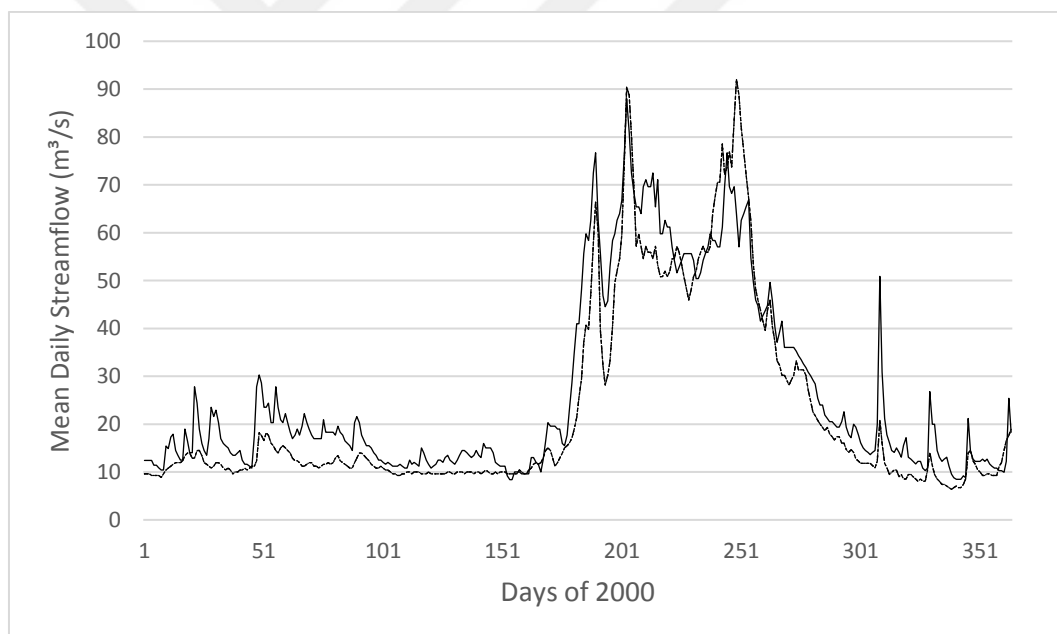
Figure 93: Hydrograph of streamgage 2215
