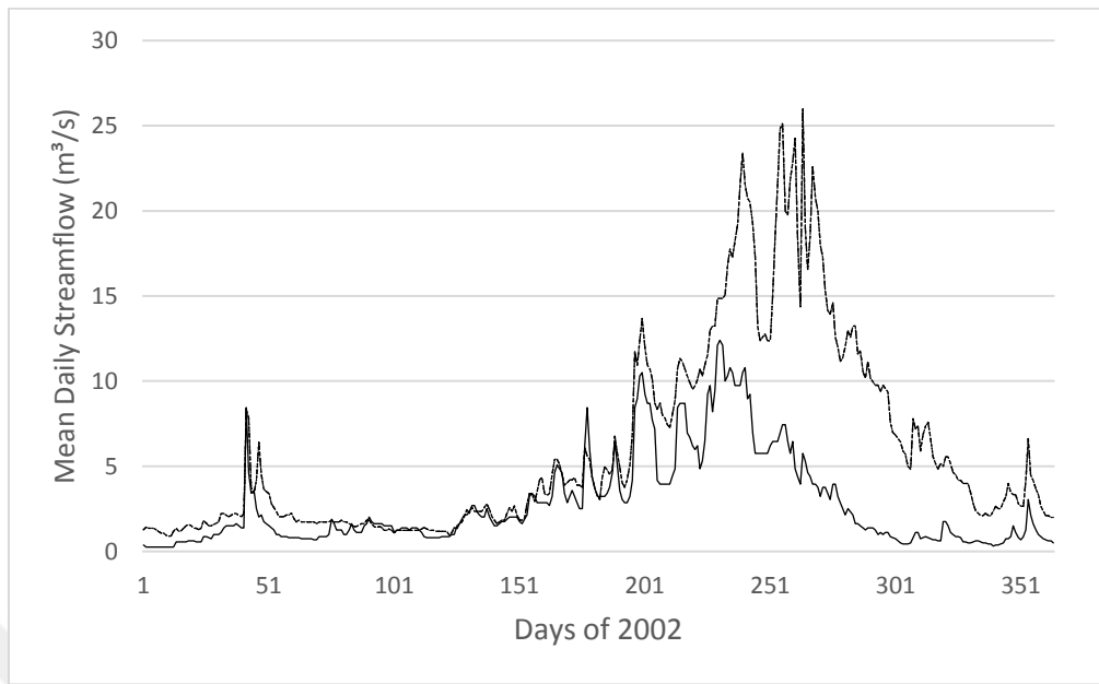
Figure 105: Hydrograph of streamgage 2340
