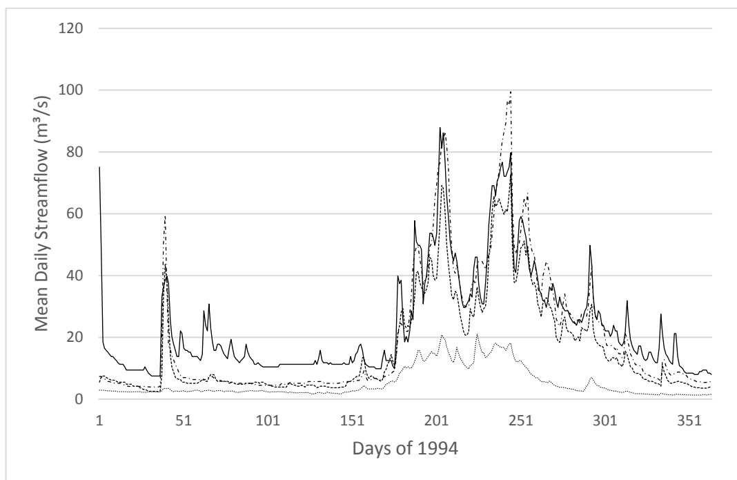
Figure 95: Hydrograph of streamgage 2232
