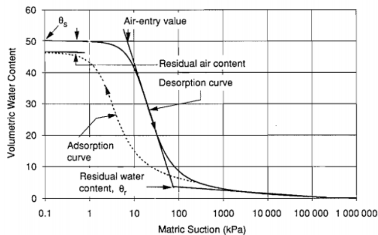
Figure 3-1: The typical soil water characteristic curve of silty soil (Fredlund and Xing 1994)
