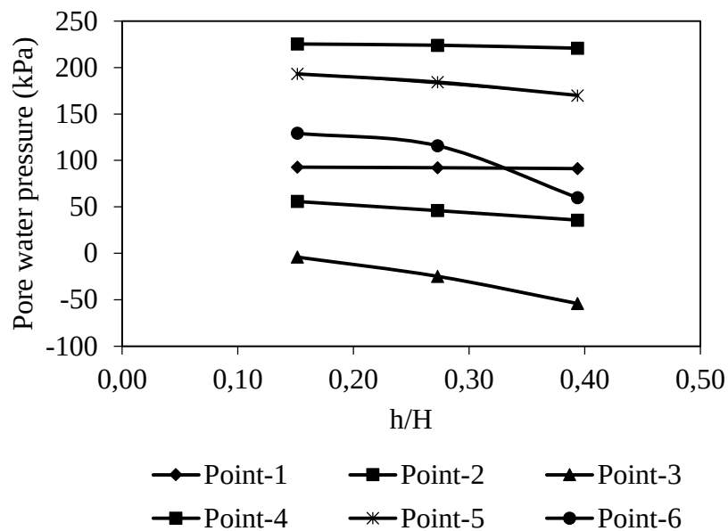
Figure 4-42: The graphical representation of the pore water pressure variation for the toe drain without an internal drainage
