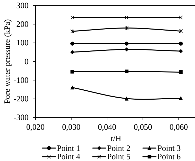
Figure 4-21: The variation of the pore water pressures with respect to t/H
