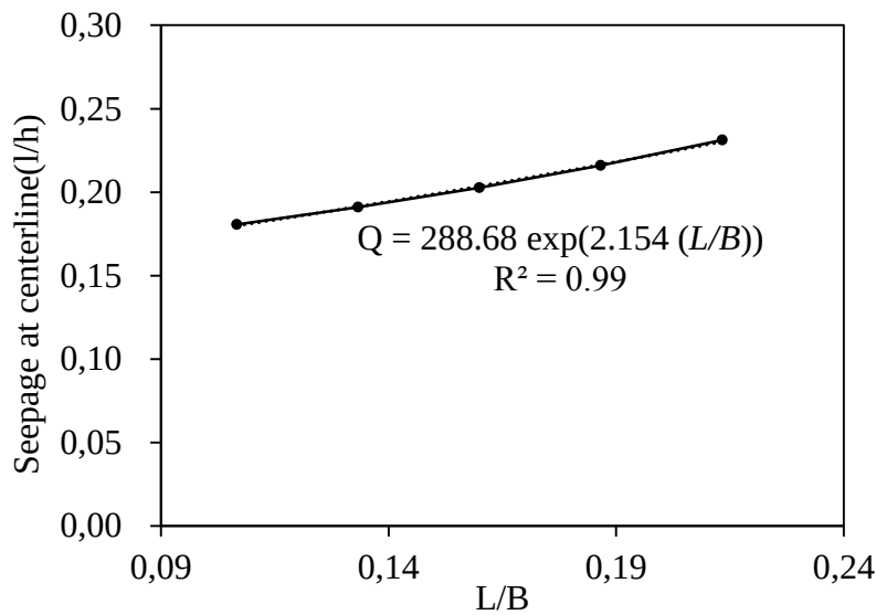
Figure 4-15: Graphical representation of seepage flows at the centerline with respect to L/B .
