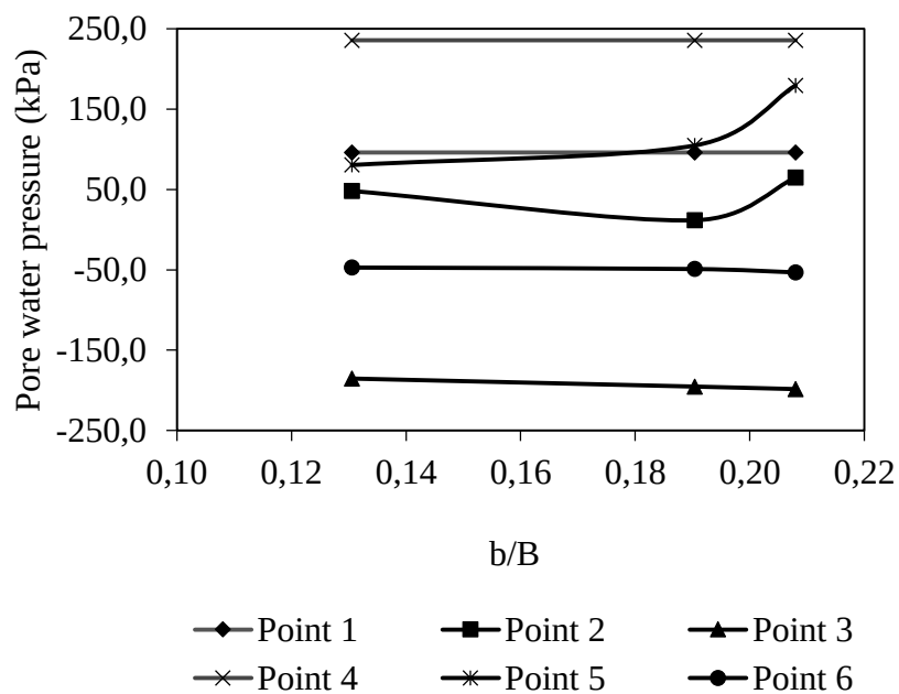
Figure 4-31: The graphical representation of pore water pressures for varied downstream slopes of core with respect to b/B
