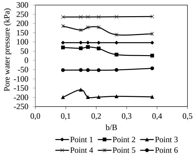
Figure 4-29: The graphical representation of pore water pressures with respect to b/B
