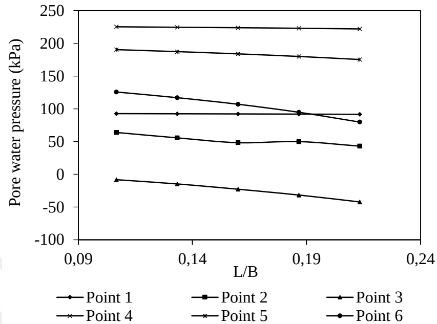
Figure 4-14: Pore water pressures at predefined points with respect to L/B
