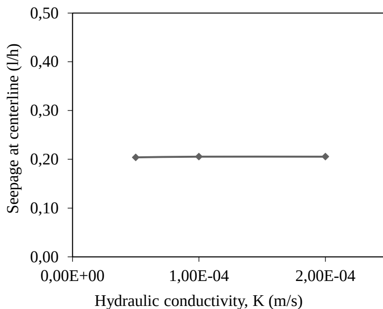
Figure 4-46: The graphical representation of the seepage rate at the dam centerline with respect to various hydraulic conductivities of the toe drain
