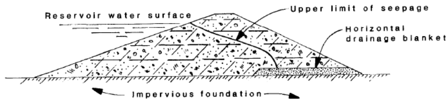
Figure 2-1: Typical cross-section of blanket drain in homogenous earth-fill dam (USBR 1987)
