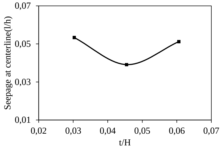
Figure 4-22: The graphical representation of seepage rates at centerline with respect to t/H
