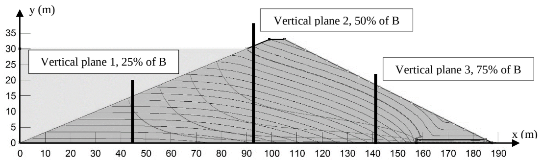
Figure 4-6: Selected vertical planes for different x/B values
