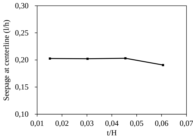
Figure 4-18: The graphical representation of seepage rates at centerline with respect to t/H
