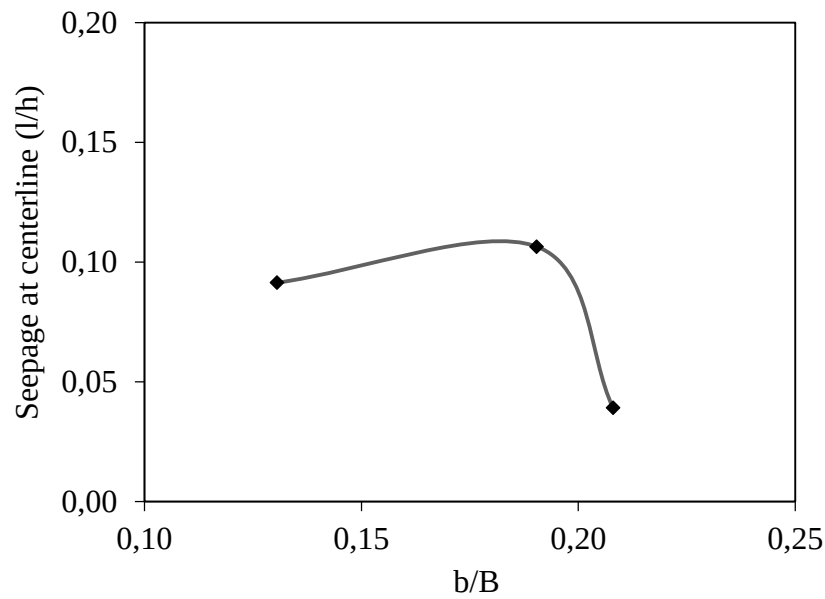
Figure 4-34: The graphical representation of the seepage flows at the centerline for varied downstream slopes of core with respect to b/B
