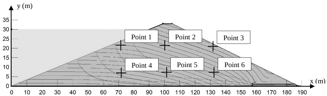
Figure 4-2: The defined points for determination of pore water pressure values
