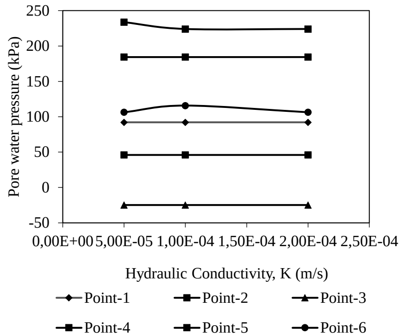
Figure 4-45: The graphical representation of the pore water pressure variation with respect to various hydraulic conductivities of the toe drain without an internal drainage
