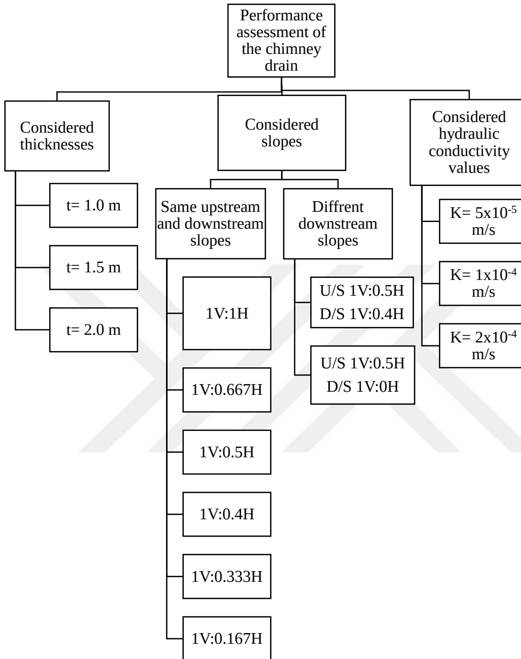
Figure 4-19: Investigated cases for the performance assessment of the chimney drain
