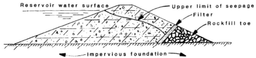
Figure 2-4: Typical cross-section of toe drain in homogenous earth-fill dam (USBR 1987)
