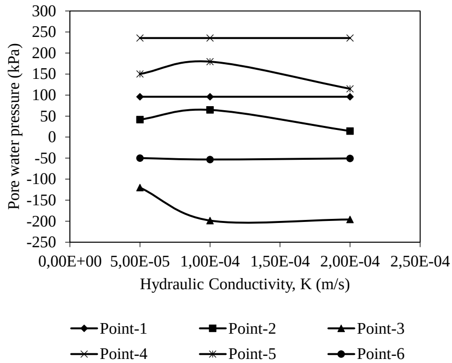
Figure 4-36: The pore water pressure values for various hydraulic conductivity values
