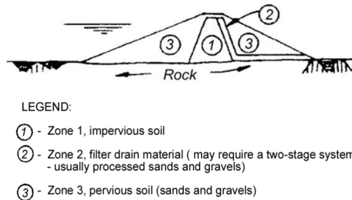
Figure 2-2: Typical cross-section of the chimney drain in a central core zoned type earth-fill dam (USBR 2012)
