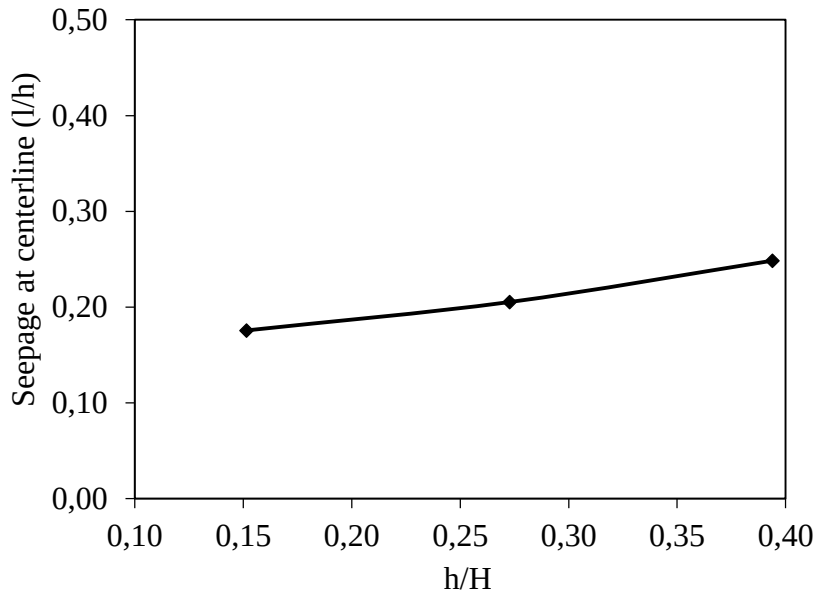
Figure 4-43: The graphical representation of the seepage rate at the dam centerline with respect to toe drain height
