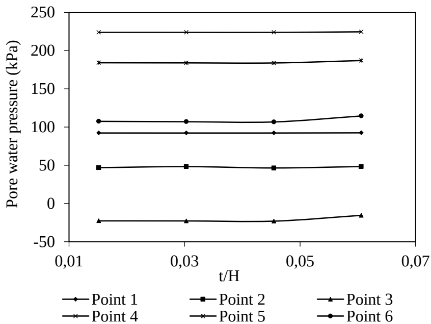
Figure 4-16: Pore water pressures at predefined points with respect to t/H
