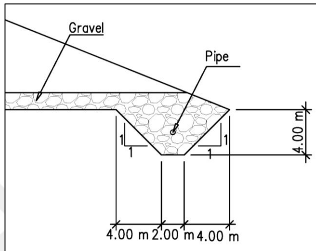
Figure 4-47: The detailed geometry of the toe drain with an internal drainage The toe drain is applied along with blanket and chimney drains and seepage analyses are conducted. The phreatic lines of the cases having blanket with and without a toe drain are given in Figure 4-48. The pore water pressures at predefined points for these two cases are provided in Table 4-30. According to the results, when a toe drain is applied under the blanket drain, the phreatic line slightly moves towards upstream and the pore water pressures slightly decrease. It may be resulted that the toe drain increases the effectiveness of the blanket drain.
