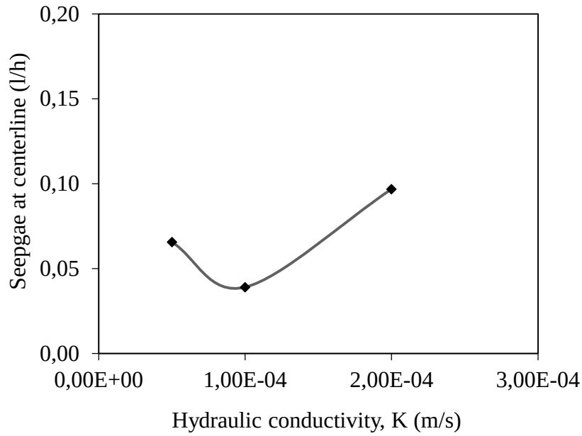
Figure 4-37: The graphical representation of the seepage flows at centerline for various hydraulic conductivity values of the chimney drain
