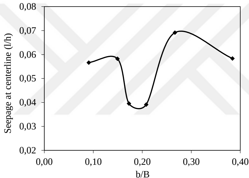
Figure 4-30: The graphical representation of seepage rates at the centerline with respect to b/B
