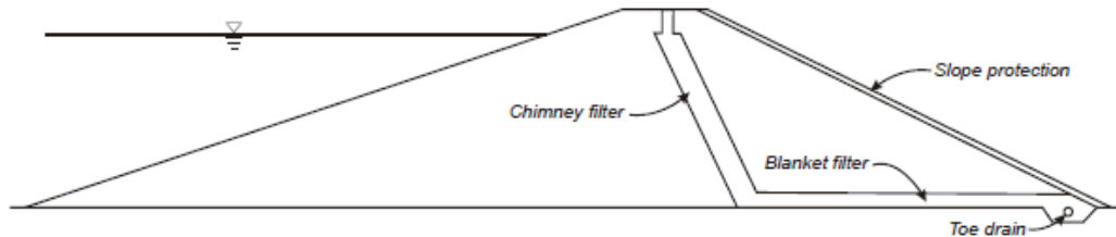
Figure 2-3: Typical cross-section of toe drain with internal drainage systems in homogenous earth-fill dam (FEMA 2011)
