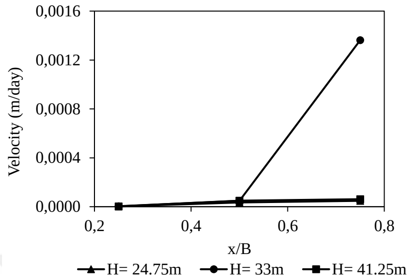
Figure 4-8: Average velocities with respect to x/B in the simple zoned type earth-fill dam
