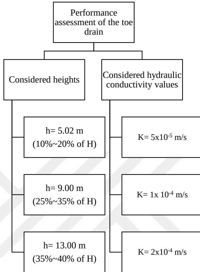
Figure 4-40: Investigated cases for the performance assessment of the toe drain
