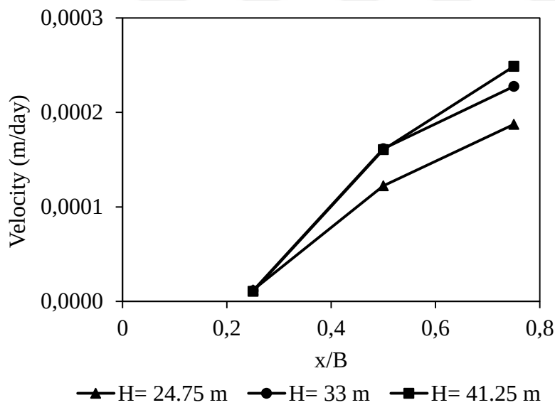
Figure 4-7: Average velocities with respect to x/B in the homogenous type earth-fill dam
